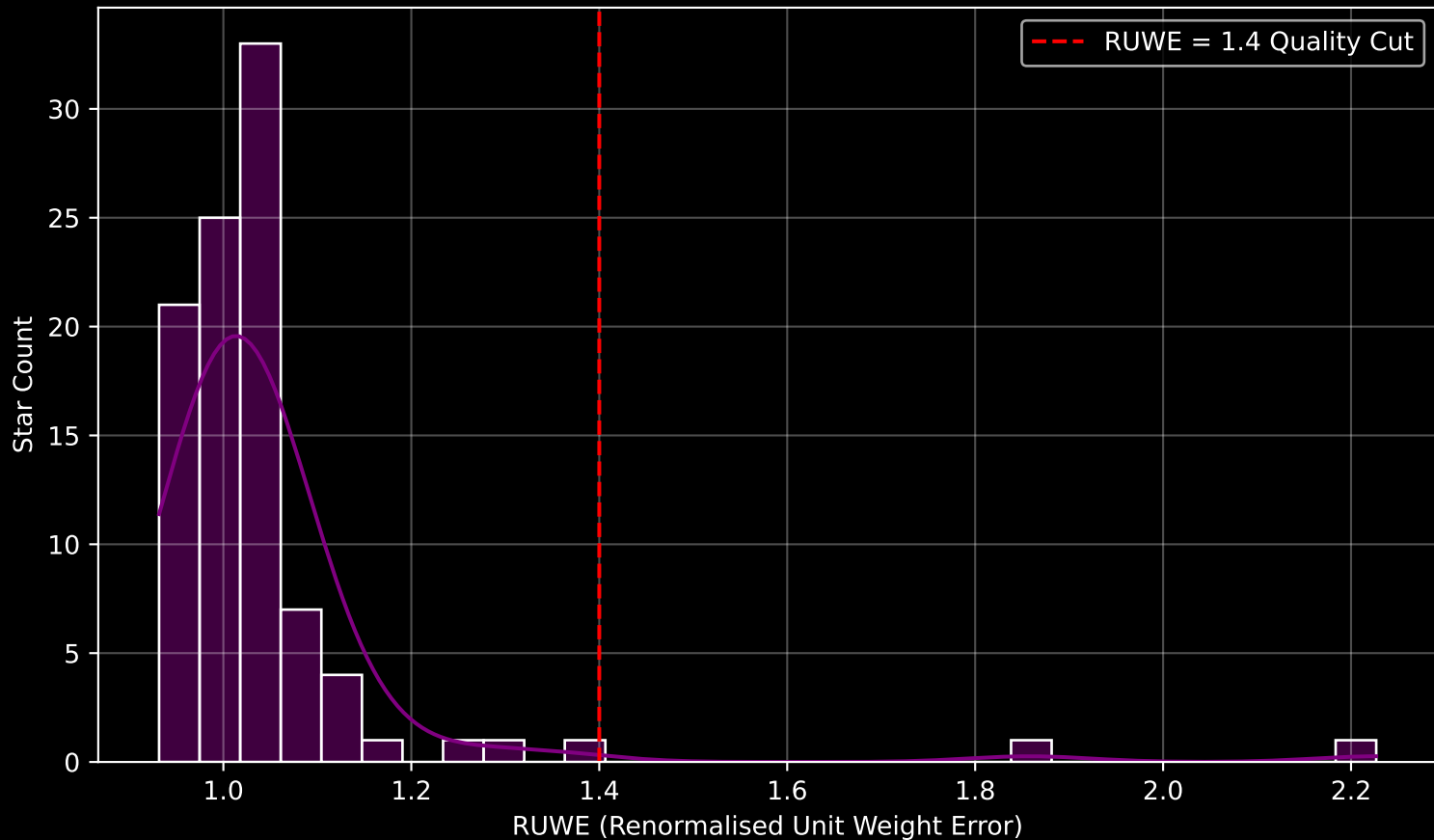
Gaia Cluster: [Gulliver_57] RUWE Distribution (n= 96)
