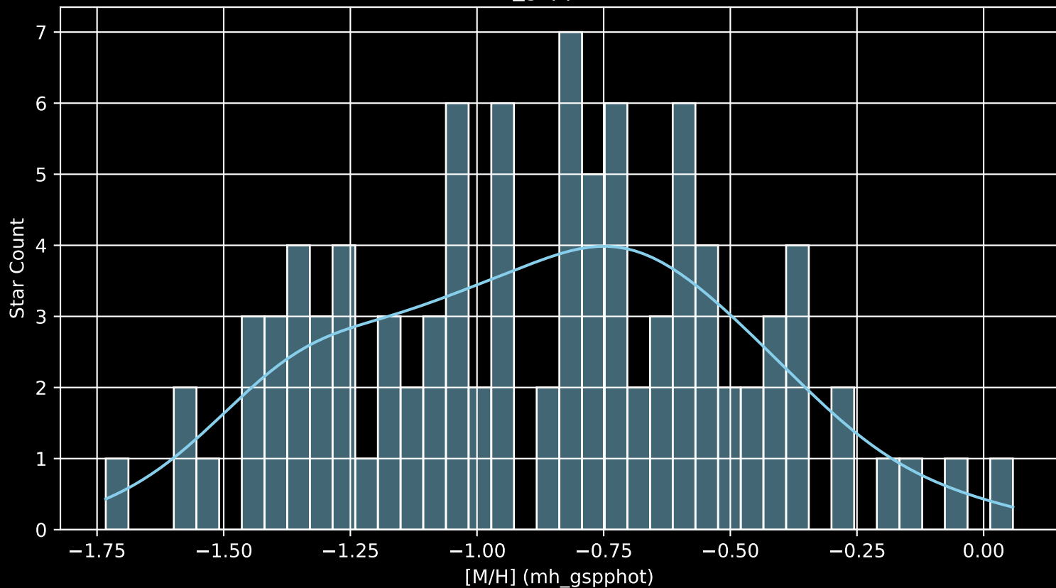
Gaia Cluster: [Gulliver_57 [M/H] (mh_gspphot) (n= 96)
