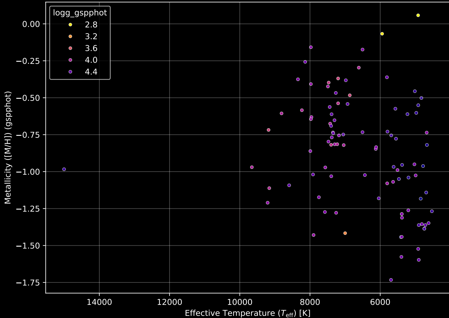
Gaia Cluster: [Gulliver_57] Stellar Population Parameters (n= 96)
