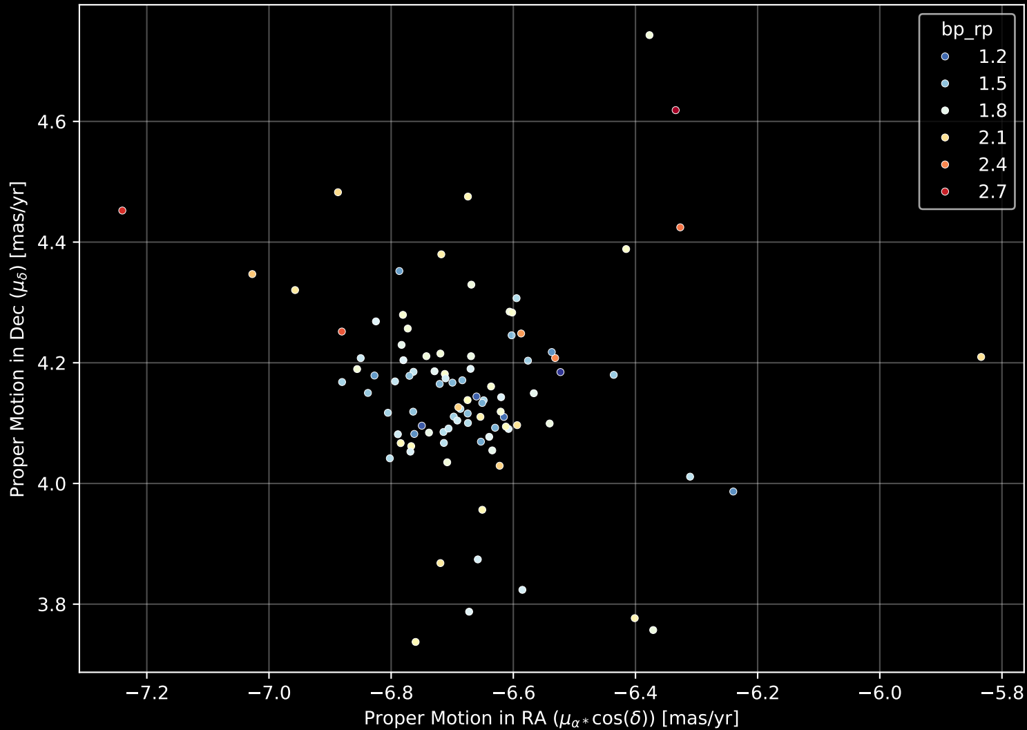
Gaia Cluster: [Gulliver_57] Proper Motion Diagram (n= 96)
