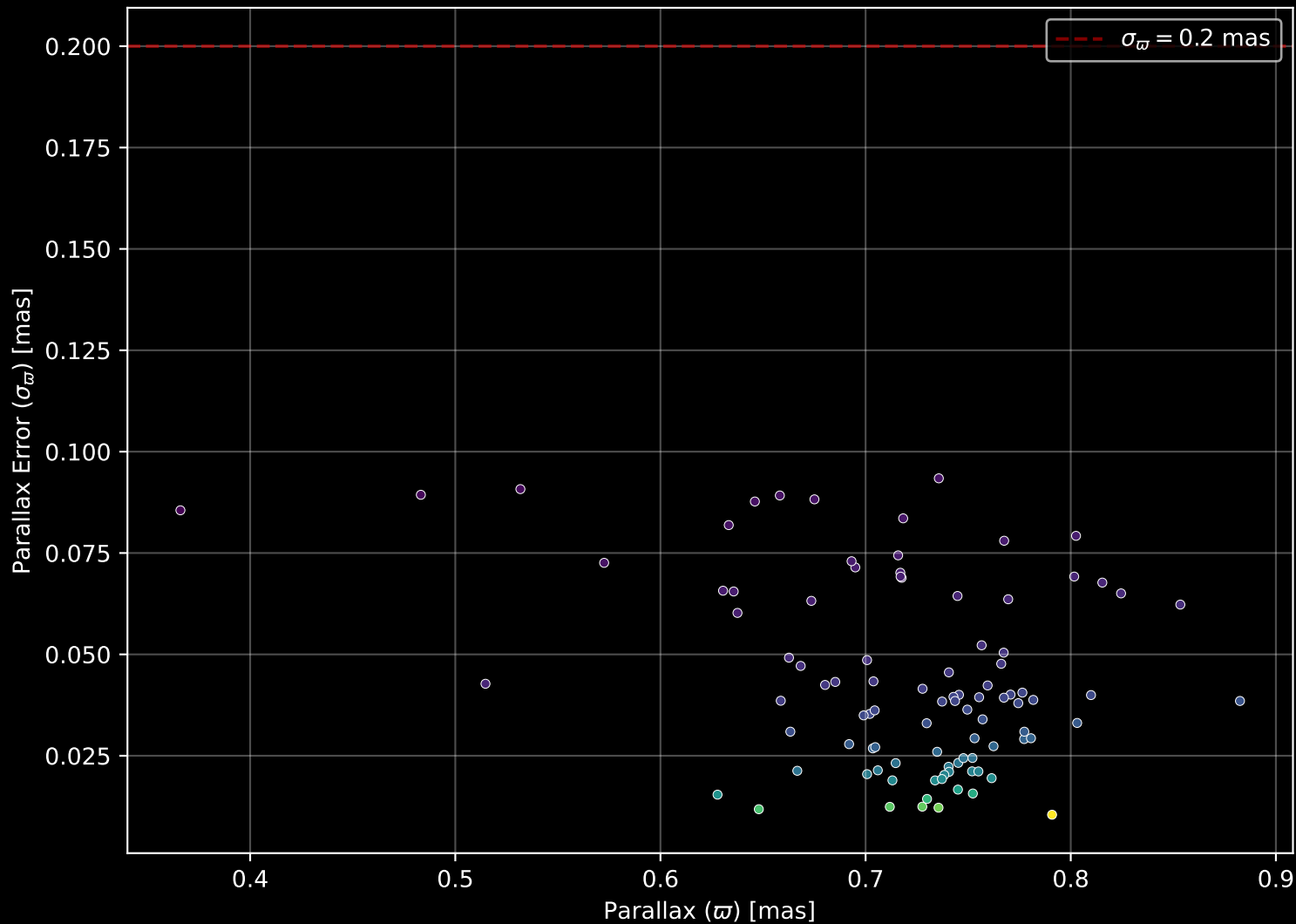
Gaia Cluster: [Gulliver_57] Parallax Quality (n= 96)
