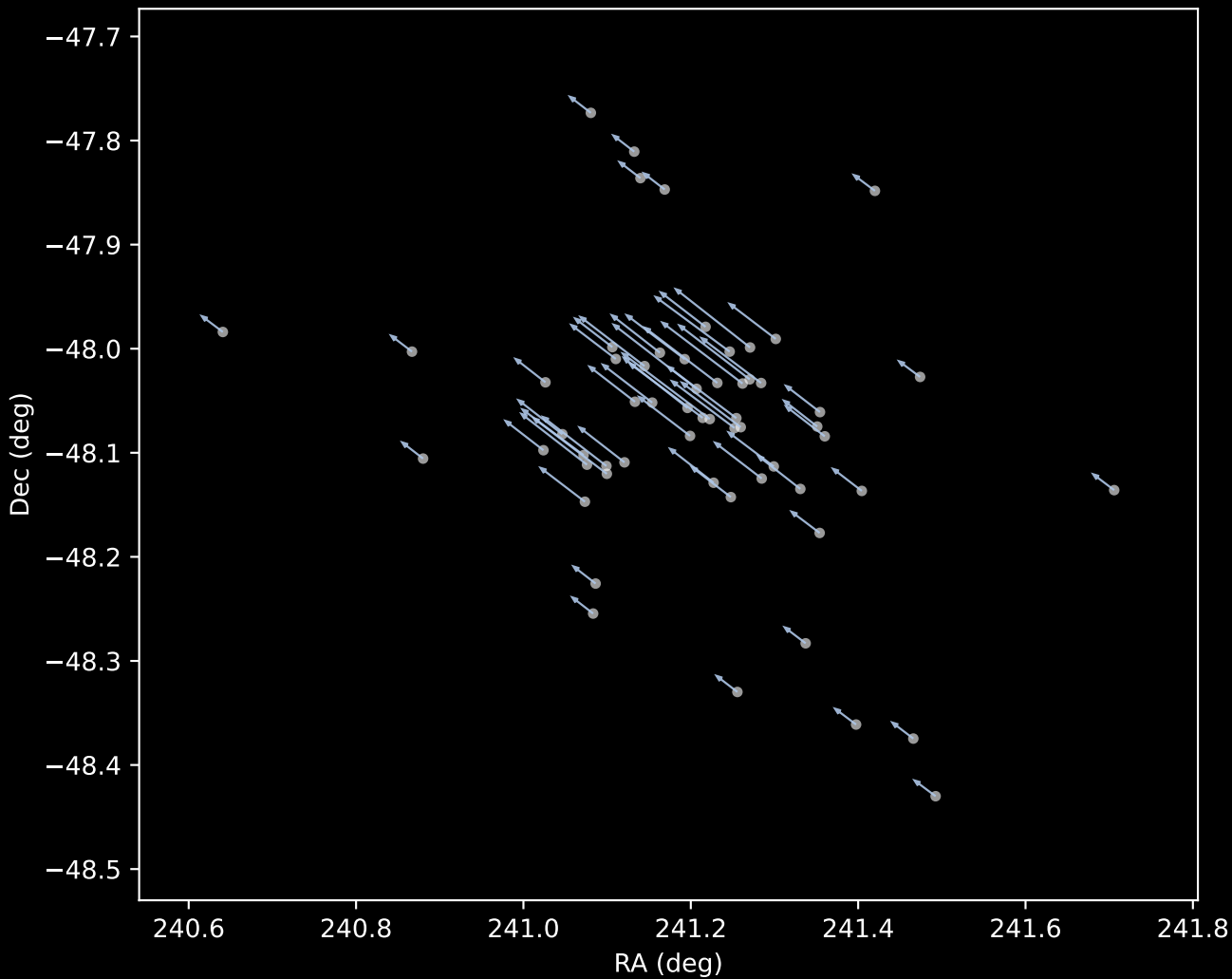
Gaia DR3 Cluster 1 Proper Motion Vectors (n=59)
