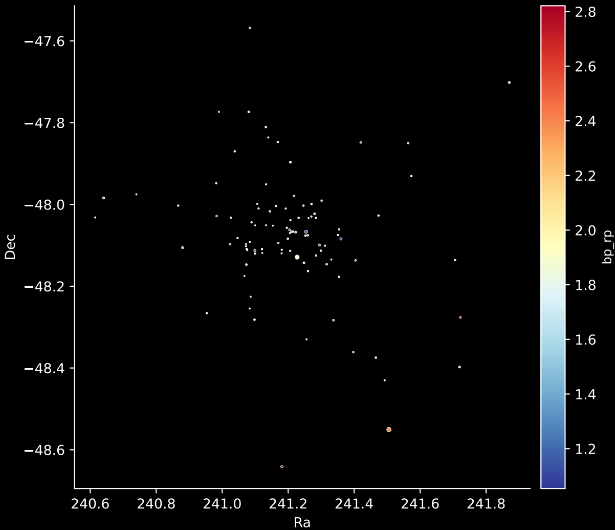
Gaia Cluster: [Gulliver_57] Stars: 96
