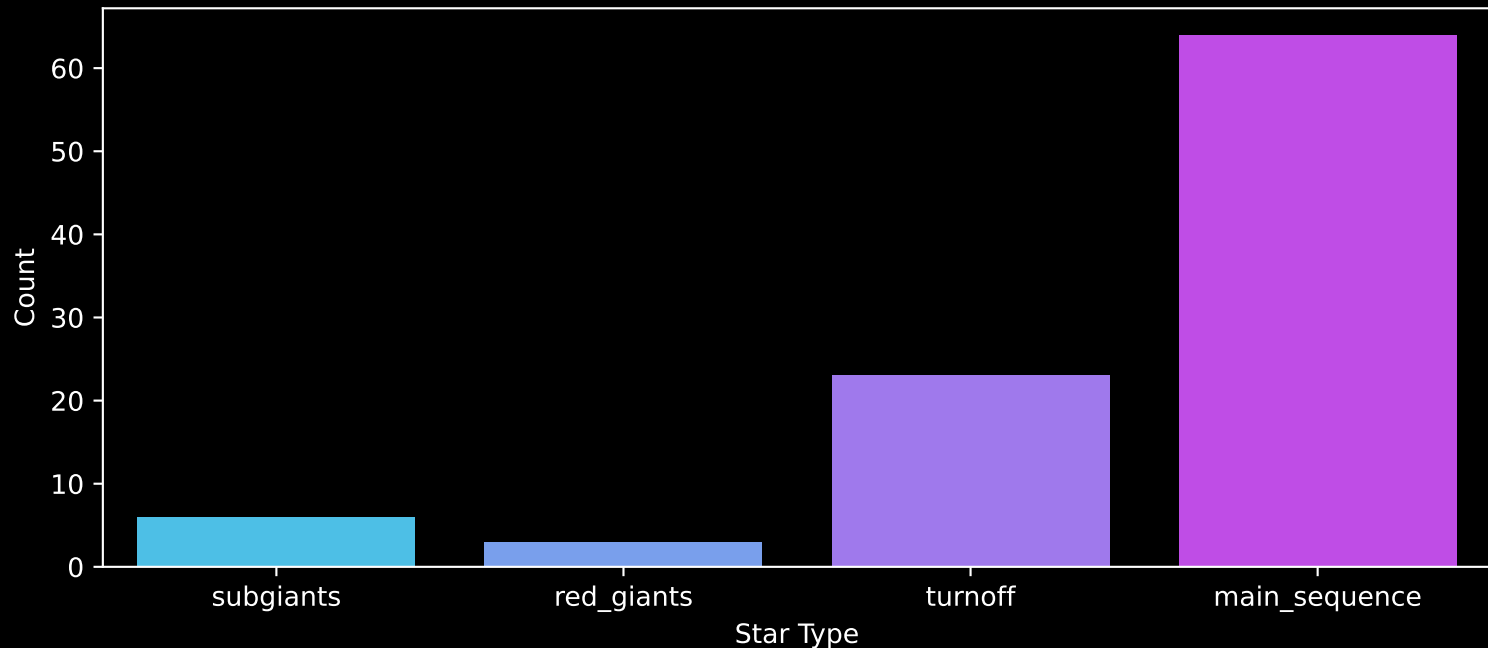
Gaia Cluster: [Gulliver_57] Count plot of Star Type
