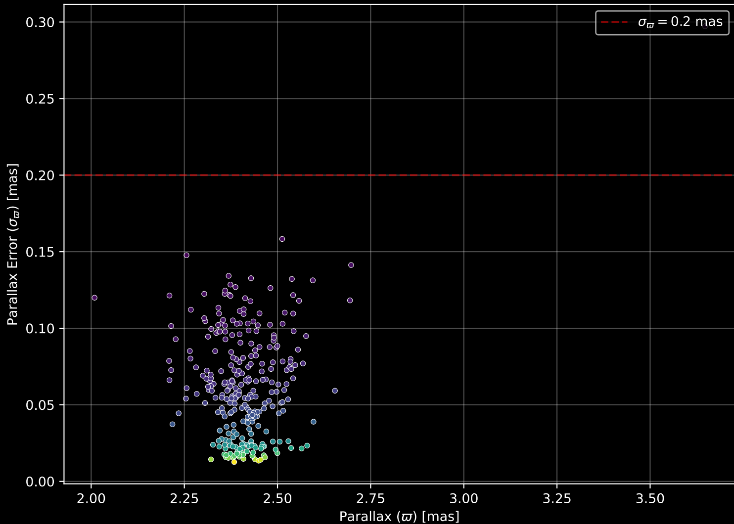
Gaia Cluster: [Gulliver_6] Parallax Quality (n= 284)
