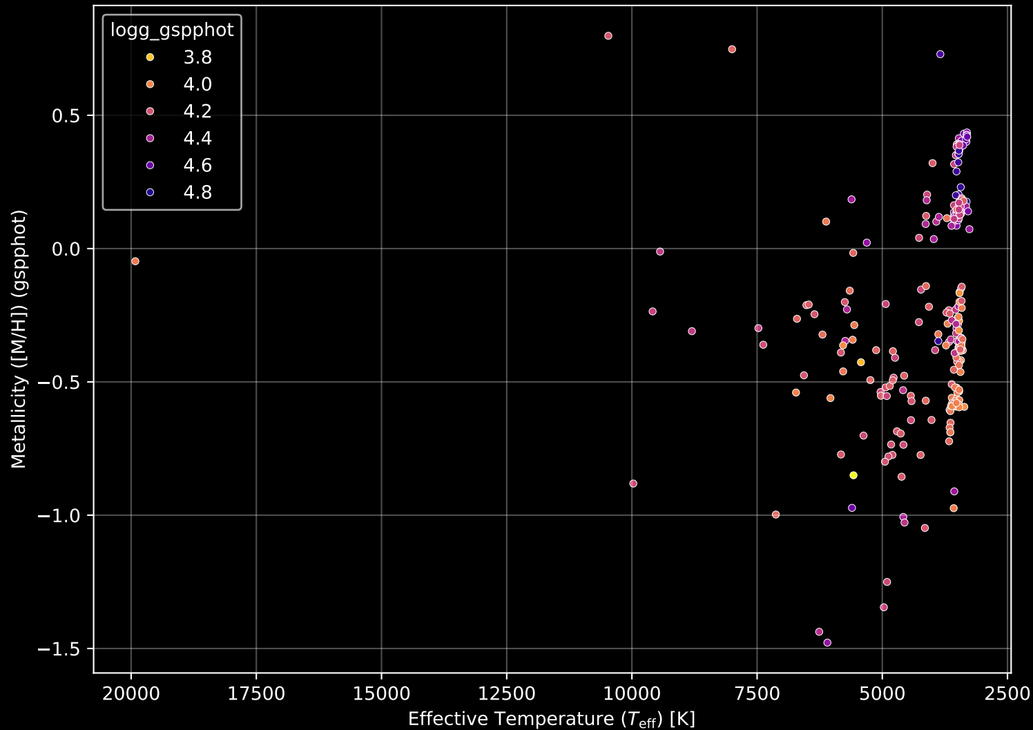
Gaia Cluster: [Gulliver_6] Stellar Population Parameters (n= 284)
