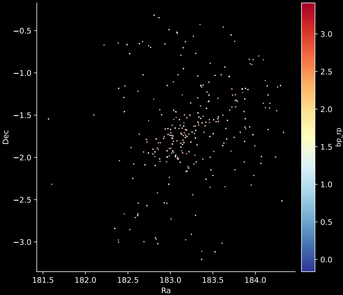
Gaia Cluster: [Gulliver_6] Stars: 284
