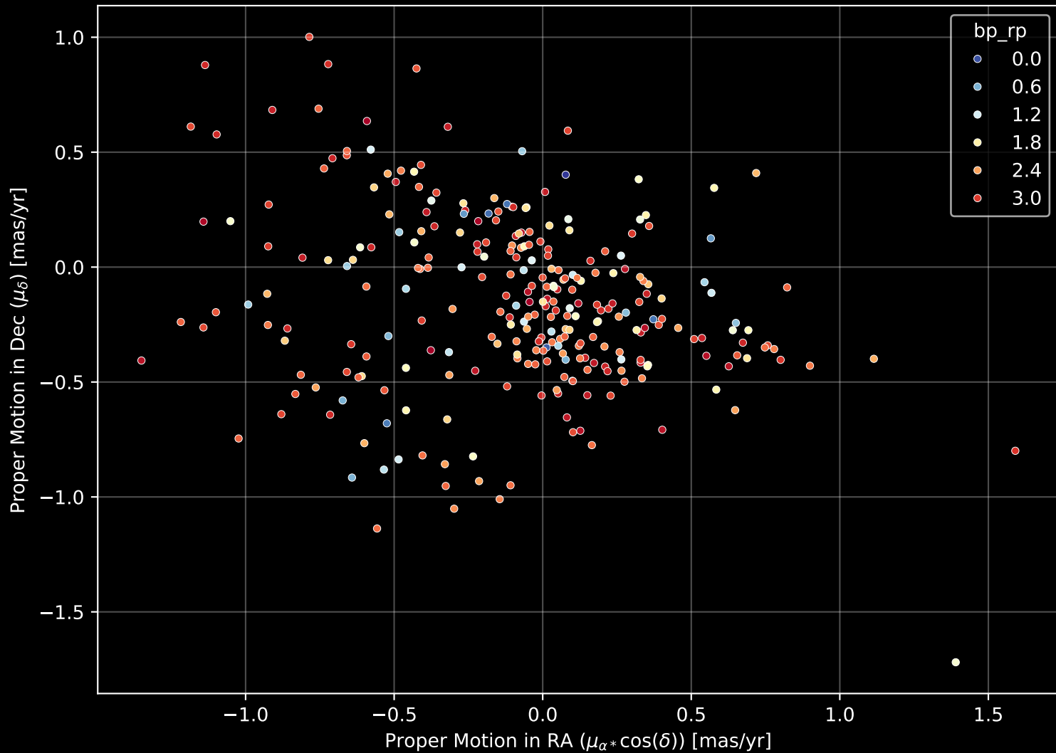
Gaia Cluster: [Gulliver_6] Proper Motion Diagram (n= 284)
