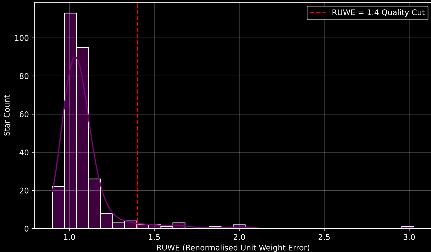
Gaia Cluster: [Gulliver_6] RUWE Distribution (n= 283)
