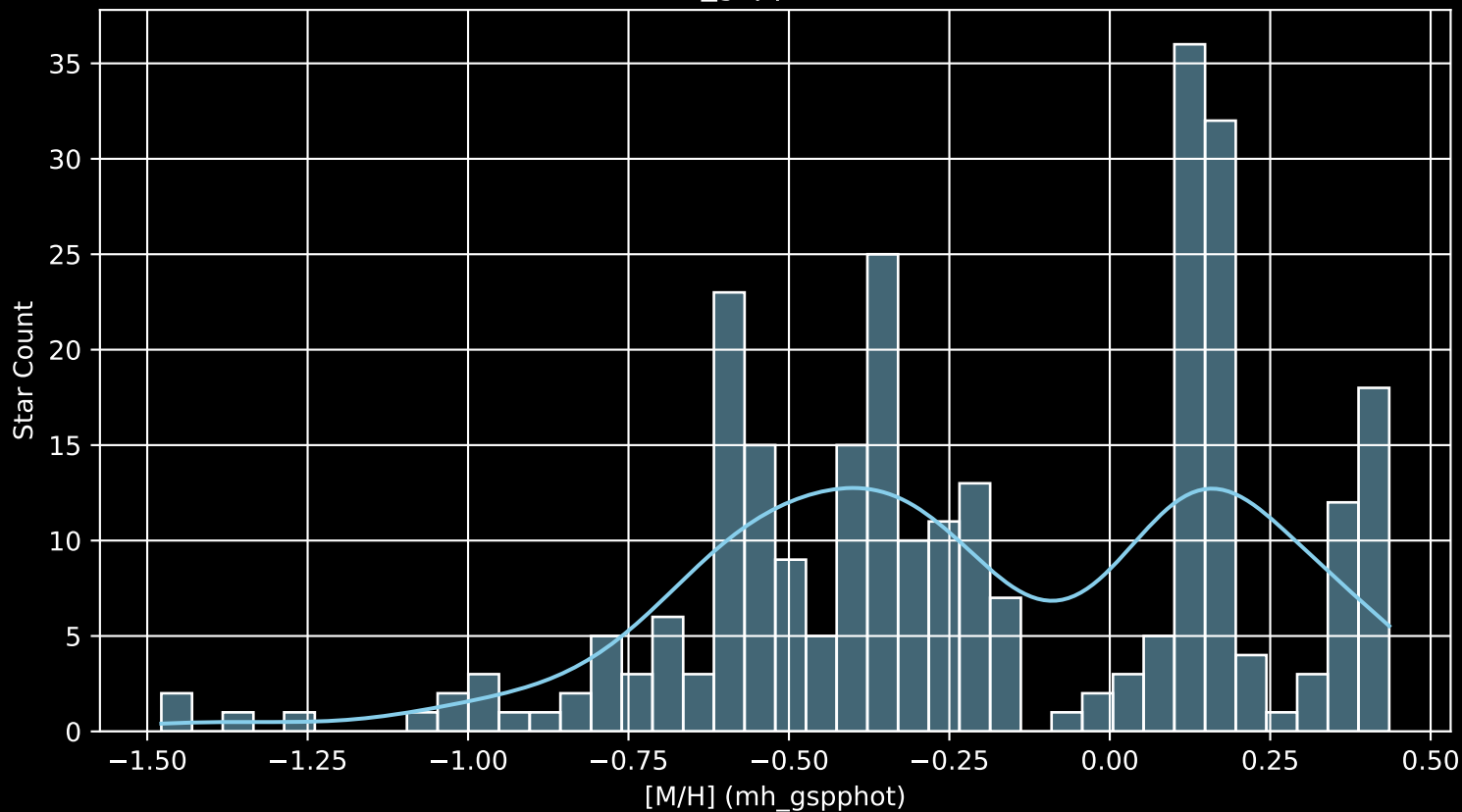
Gaia Cluster: [Gulliver_6 [M/H] (mh_gspphot) (n= 281)
