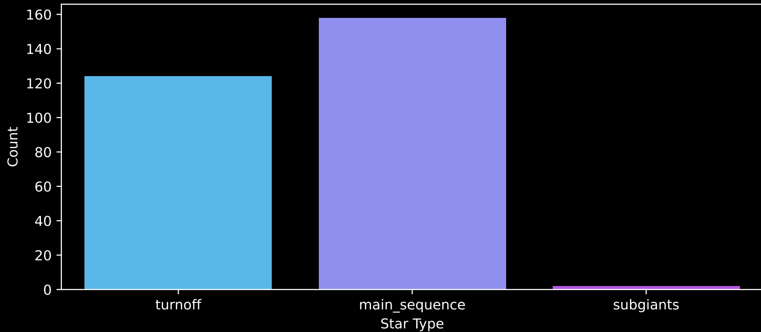
Gaia Cluster: [Gulliver_6] Count plot of Star Type
