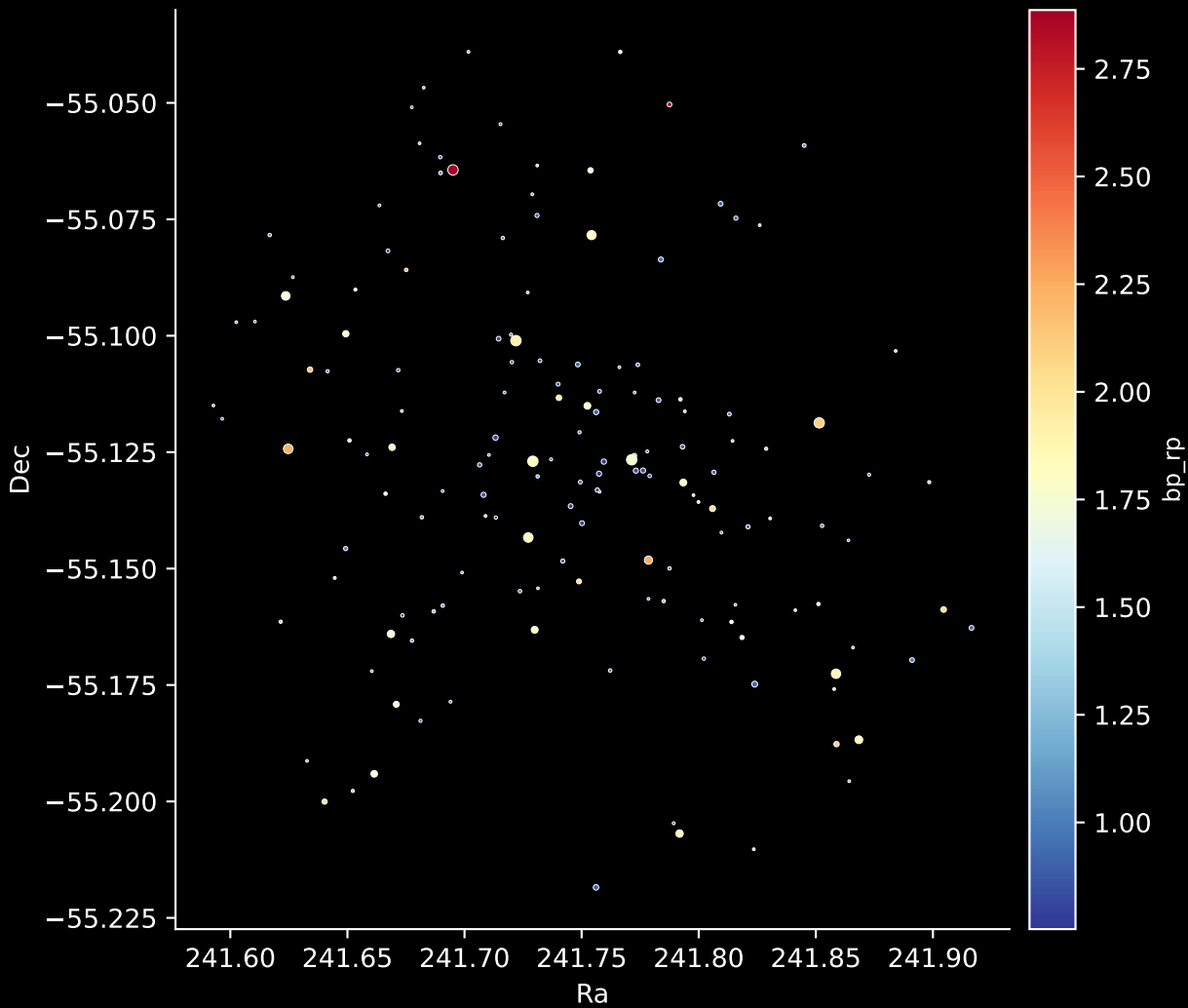
Gaia Cluster: [Gulliver_7] Stars: 153
