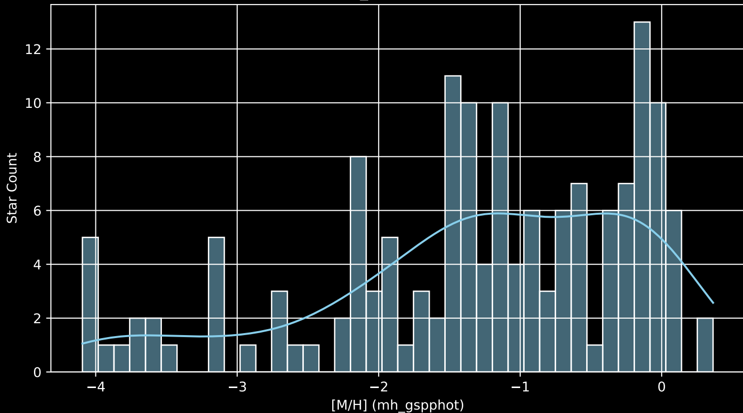
Gaia Cluster: [Gulliver_7 [M/H] (mh_gspphot) (n= 153)
