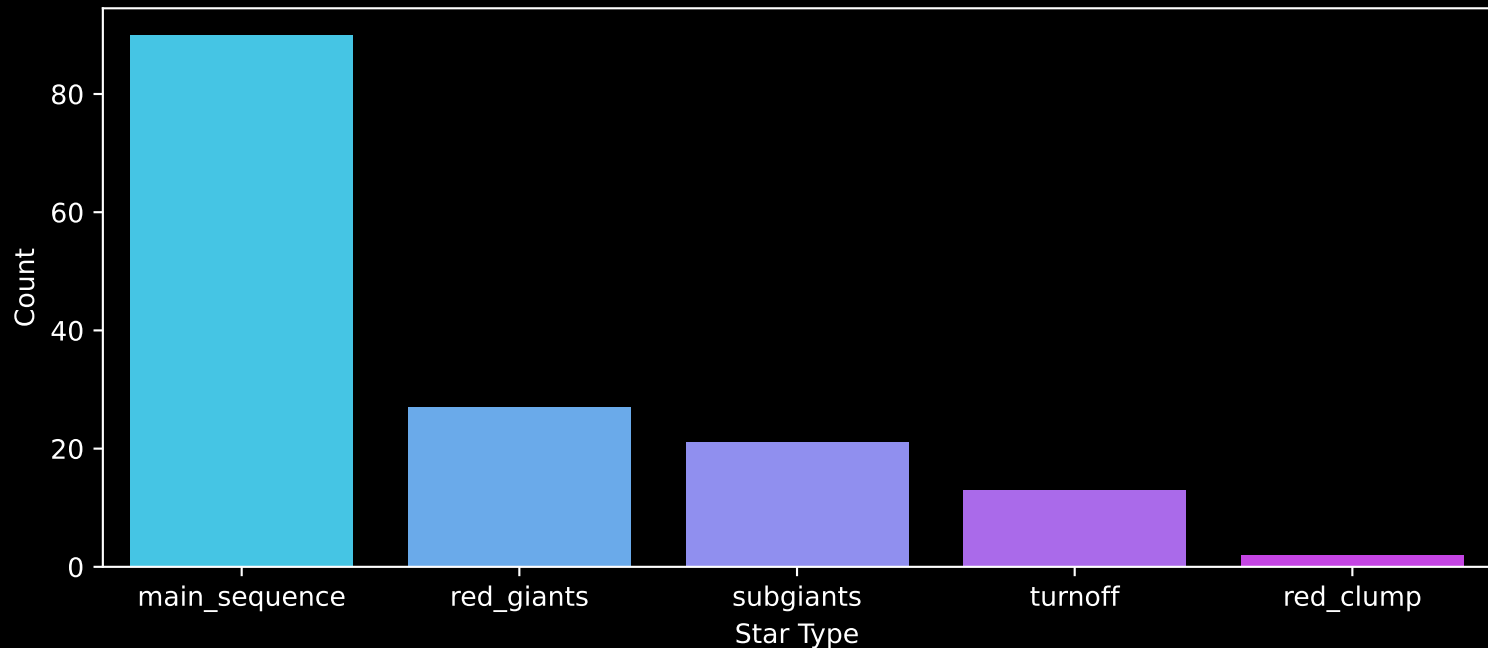
Gaia Cluster: [Gulliver_7] Count plot of Star Type
