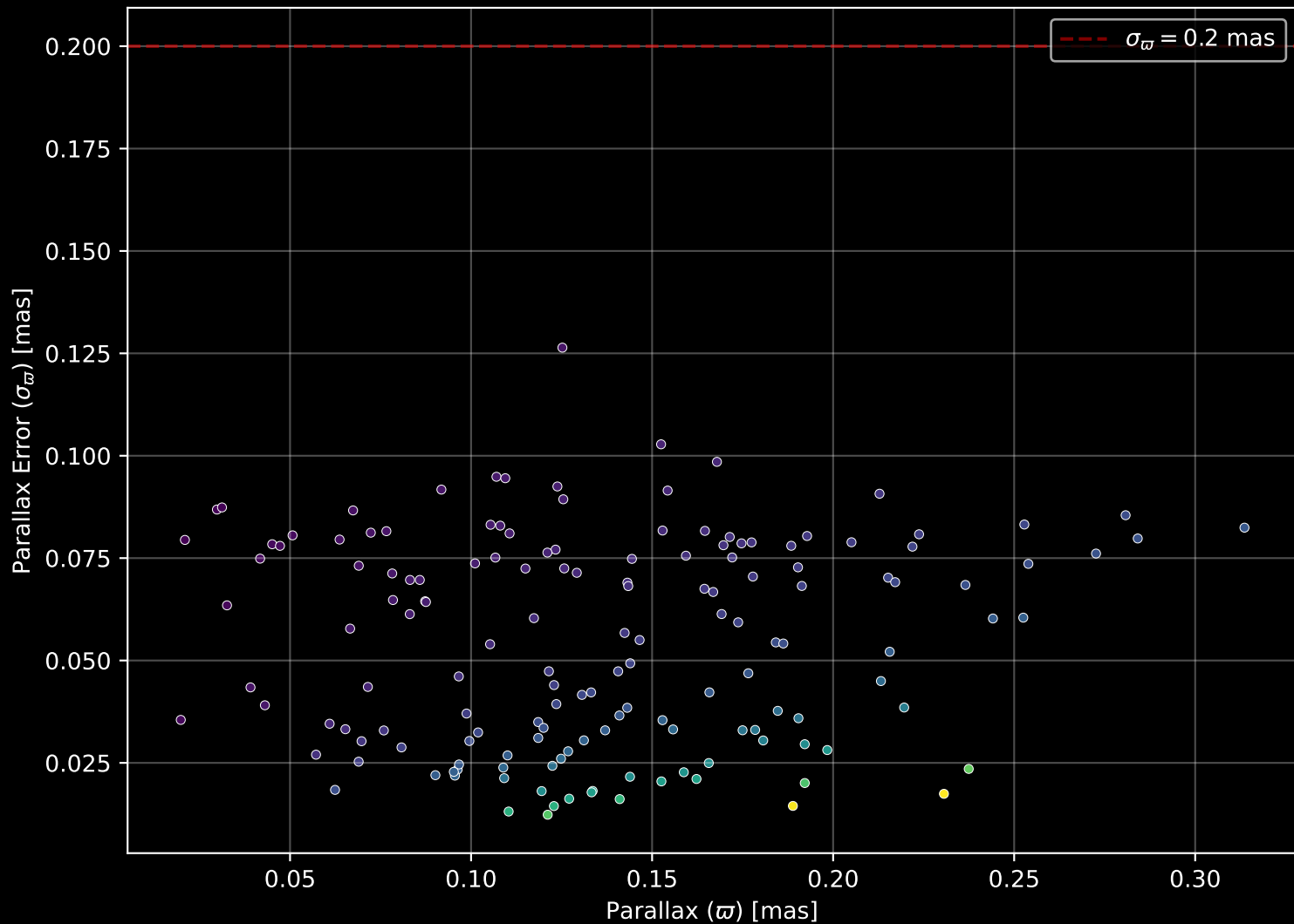
Gaia Cluster: [Gulliver_7] Parallax Quality (n= 153)
