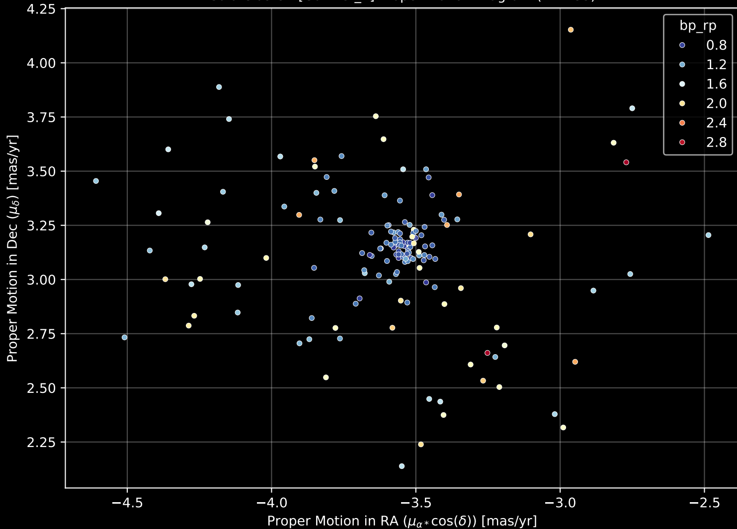
Gaia Cluster: [Gulliver_7] Proper Motion Diagram (n= 153)
