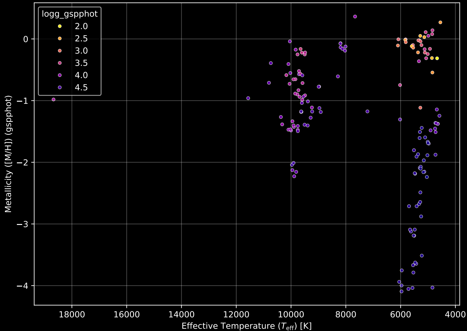
Gaia Cluster: [Gulliver_7] Stellar Population Parameters (n= 153)
