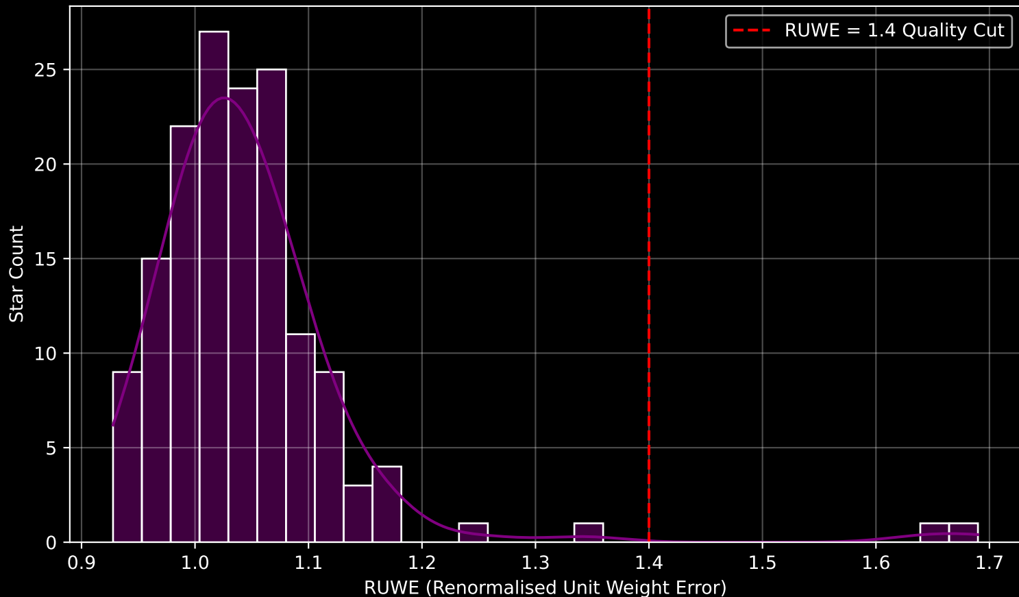
Gaia Cluster: [Gulliver_7] RUWE Distribution (n= 153)
