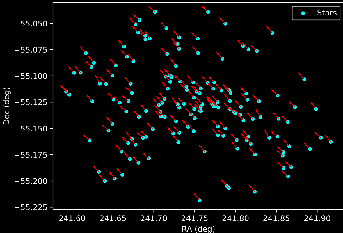
Gaia Cluster: [Gulliver_7] Proper Motion Vectors for Gaia Star Field (n= 153)
