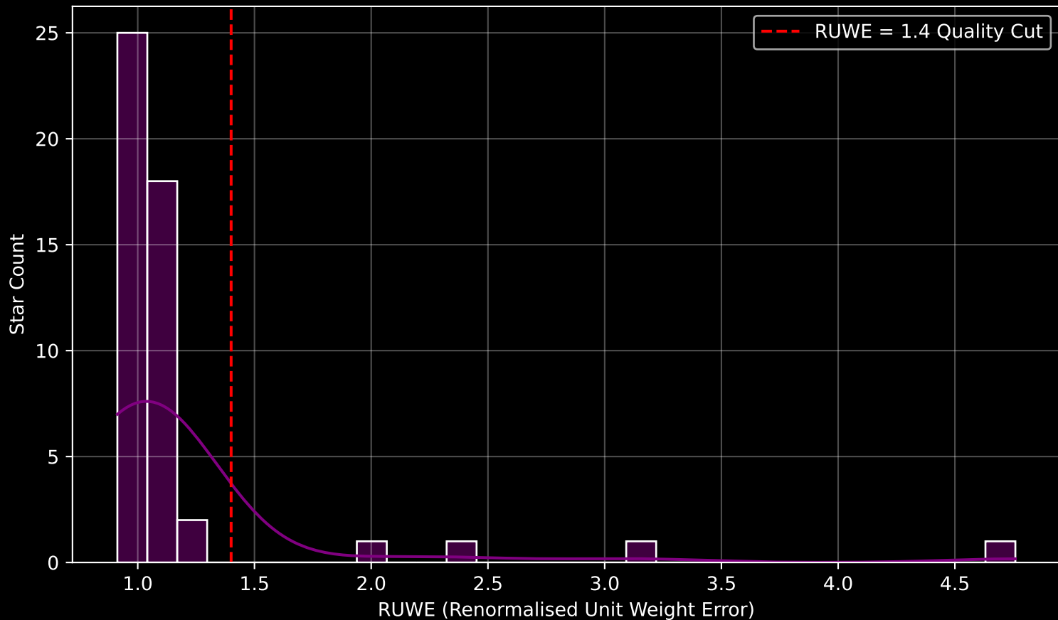
Gaia Cluster: [Gulliver_8] RUWE Distribution (n= 49)
