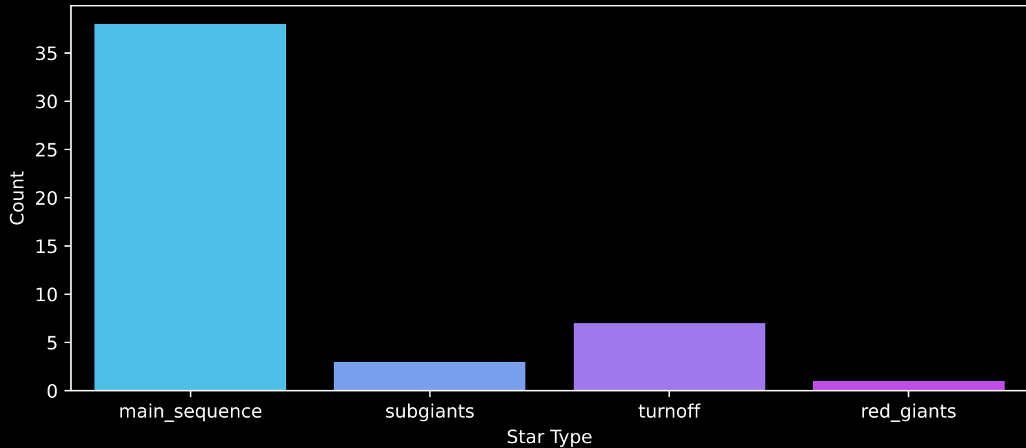
Gaia Cluster: [Gulliver_8] Count plot of Star Type
