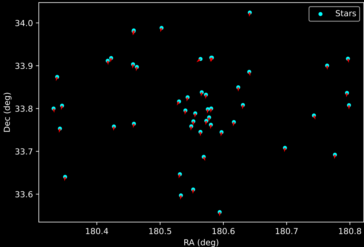
Gaia Cluster: [Gulliver_8] Proper Motion Vectors for Gaia Star Field (n= 49)
