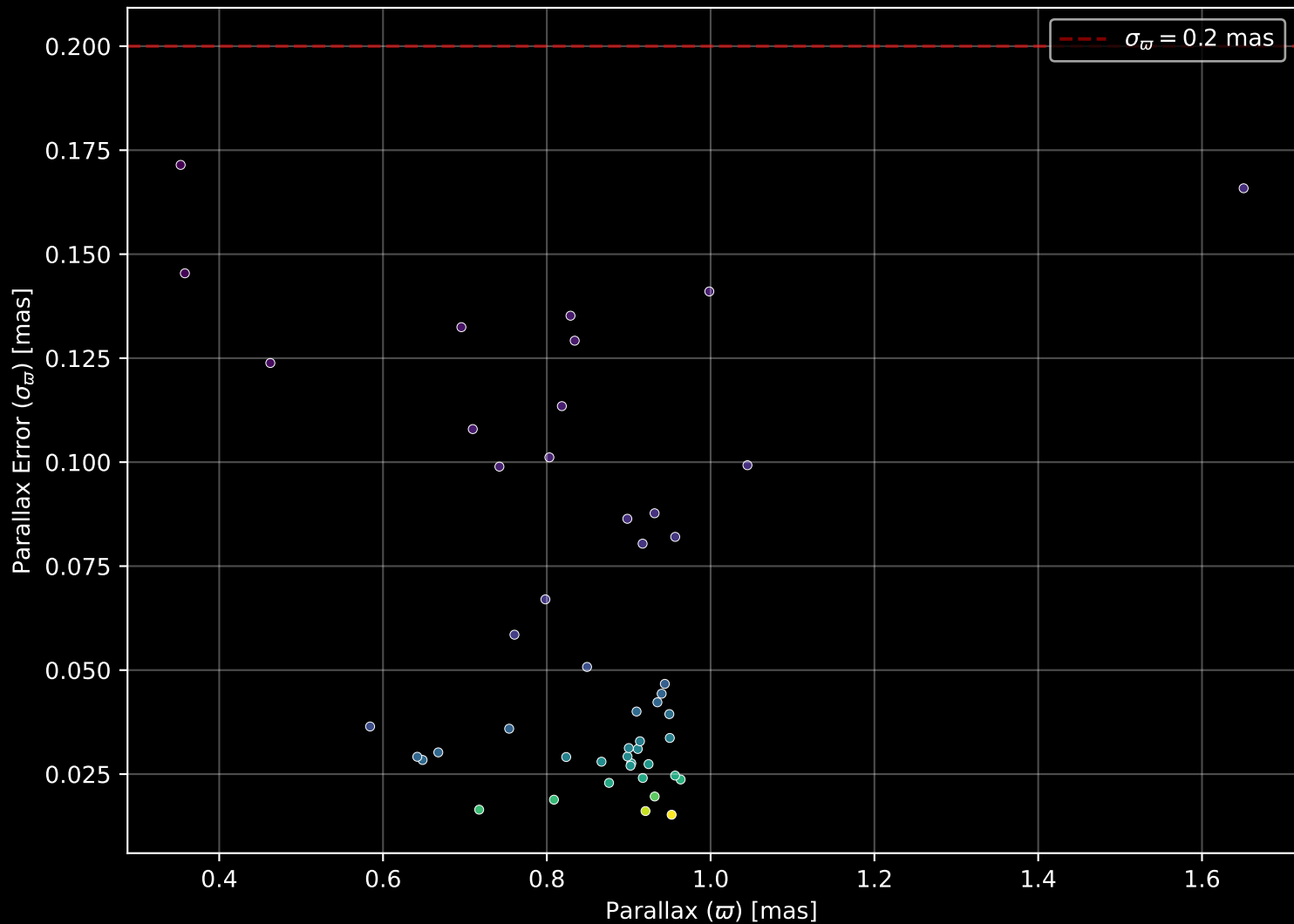
Gaia Cluster: [Gulliver_8] Parallax Quality (n= 49)
