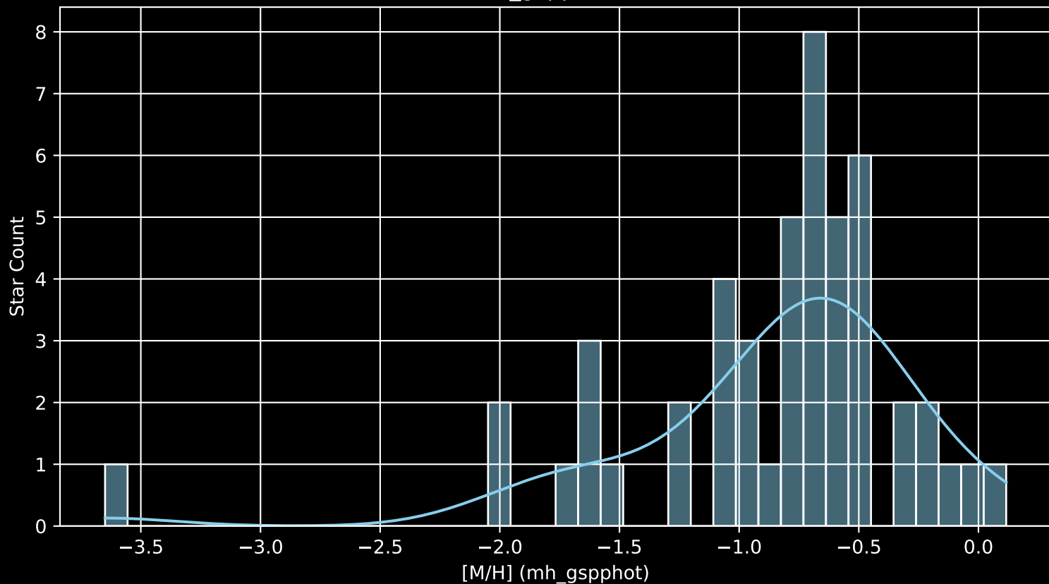
Gaia Cluster: [Gulliver_8 [M/H] (mh_gspphot) (n= 49)
