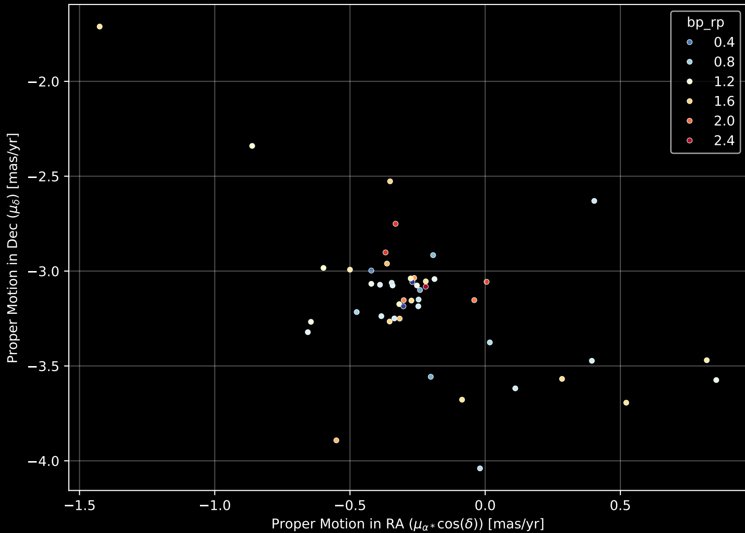
Gaia Cluster: [Gulliver_8] Proper Motion Diagram (n= 49)
