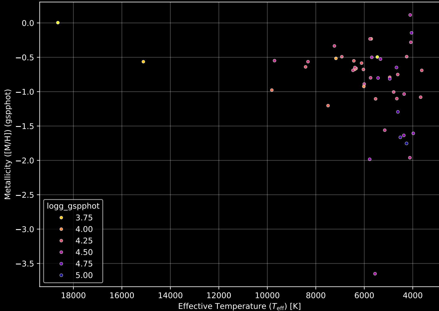
Gaia Cluster: [Gulliver_8] Stellar Population Parameters (n= 49)
