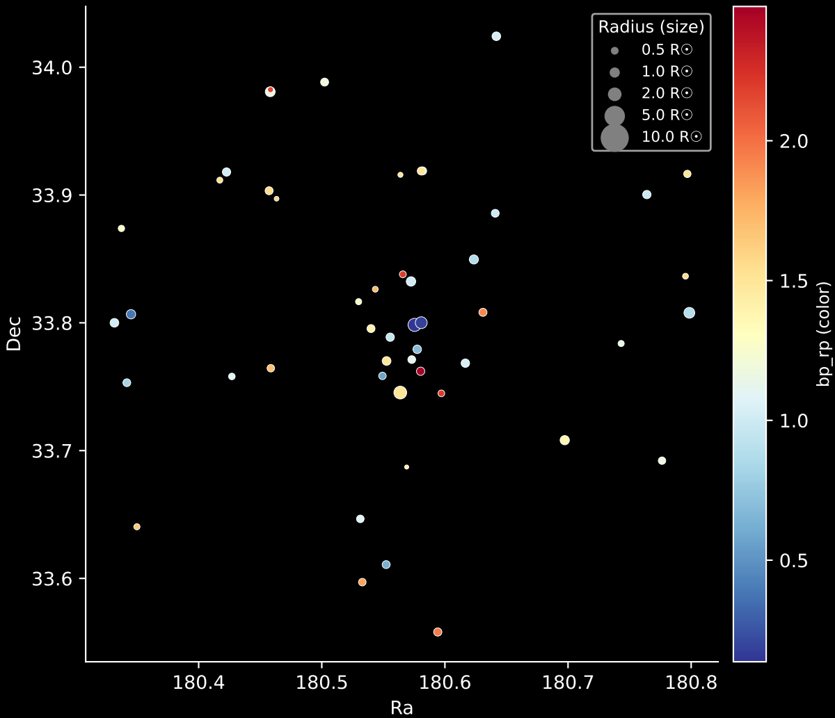
Gaia Cluster: [Gulliver_8] Stars: 49
