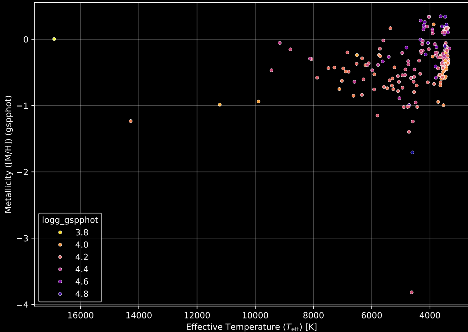
Gaia Cluster: [Gulliver_9] Stellar Population Parameters (n= 254)
