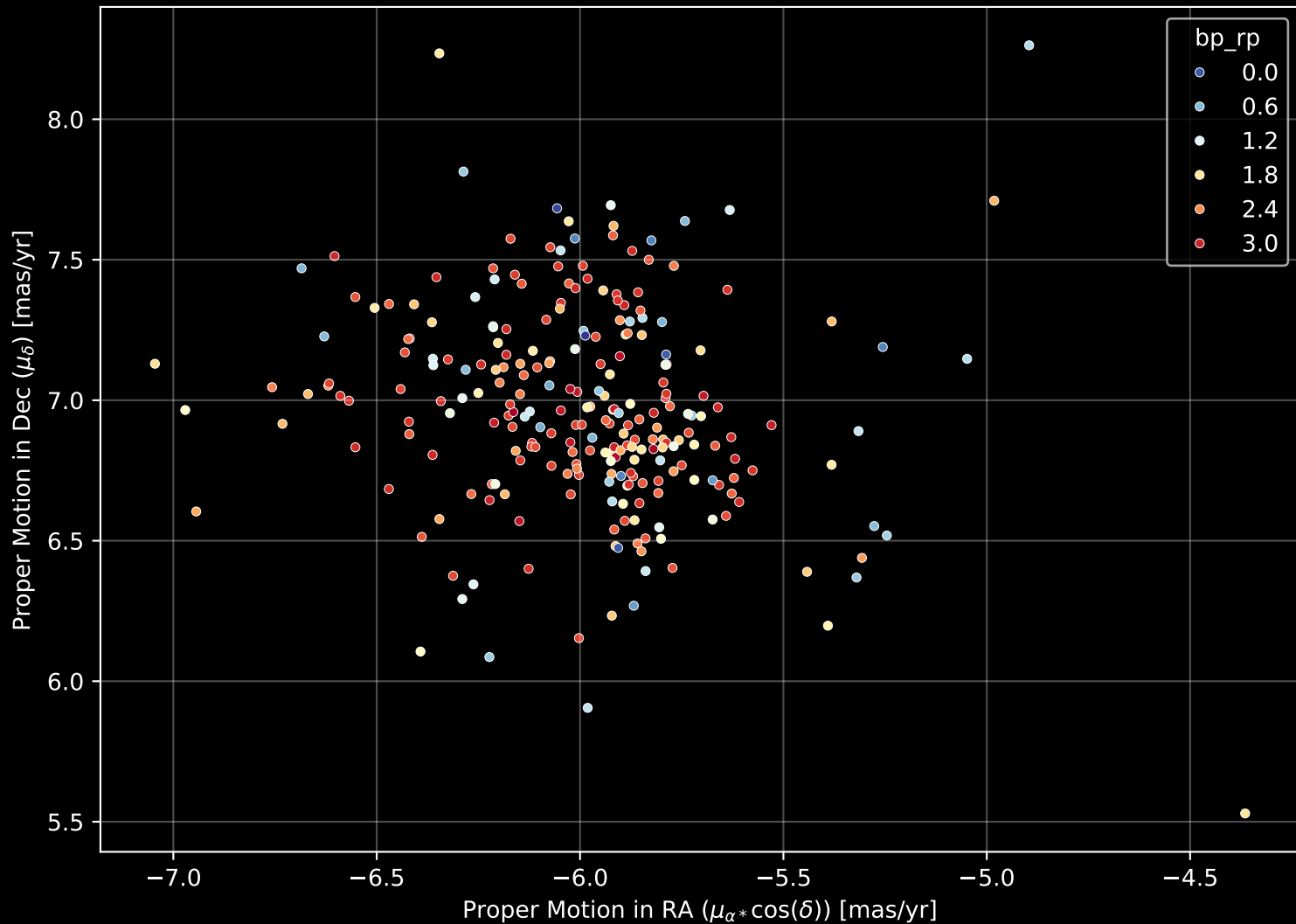
Gaia Cluster: [Gulliver_9] Proper Motion Diagram (n= 254)
