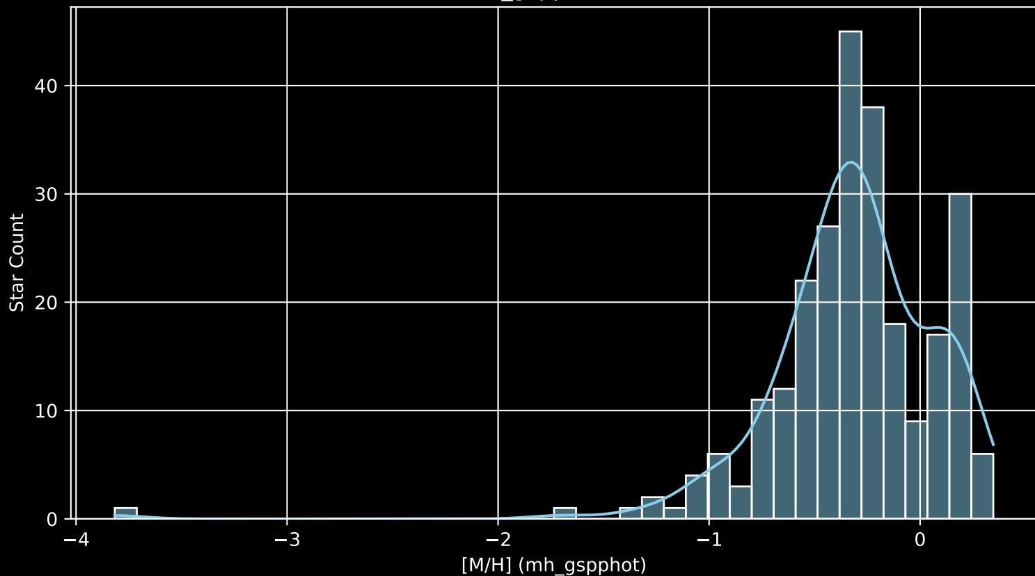
Gaia Cluster: [Gulliver_9 [M/H] (mh_gspphot) (n= 254)
