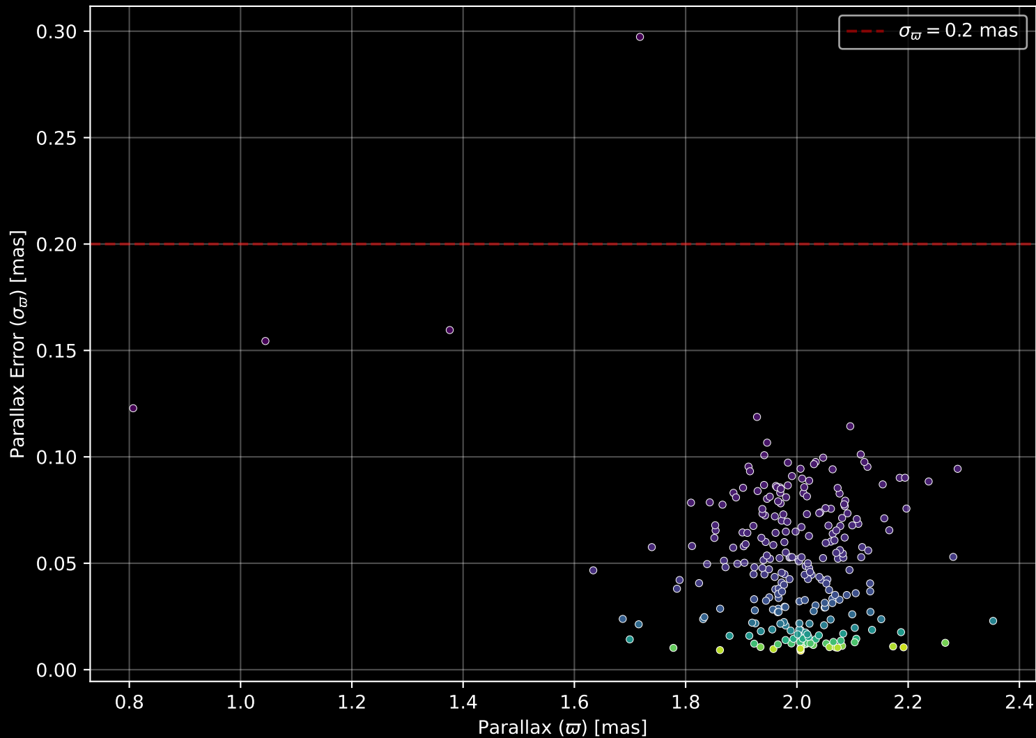
Gaia Cluster: [Gulliver_9] Parallax Quality (n= 254)
