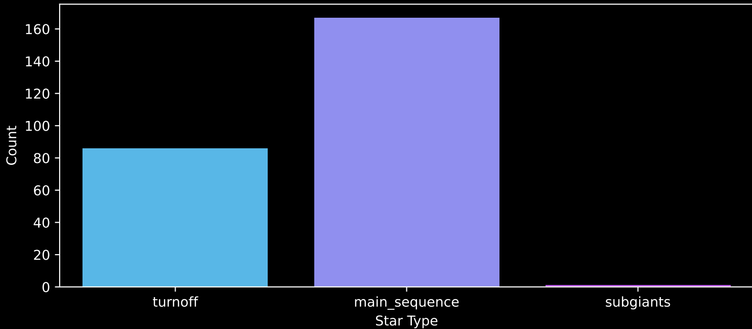
Gaia Cluster: [Gulliver_9] Count plot of Star Type
