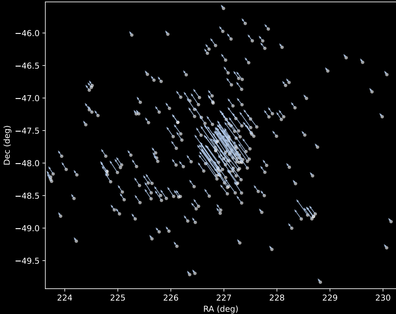
Gaia DR3 Cluster 1 Proper Motion Vectors (n=234)
