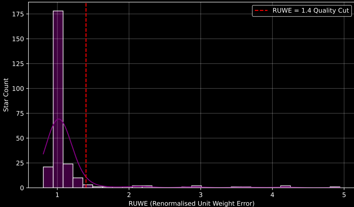
Gaia Cluster: [Gulliver_9] RUWE Distribution (n= 251)
