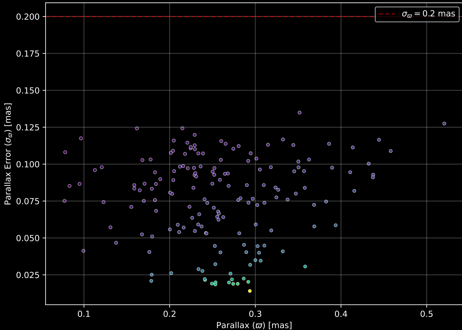
Gaia Cluster: [Haffner_10] Parallax Quality (n= 165)
