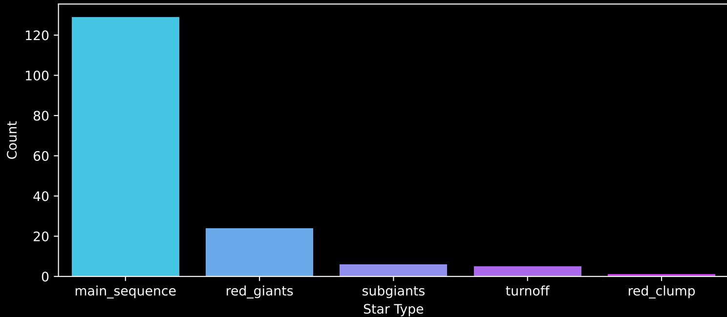
Gaia Cluster: [Haffner_10] Count plot of Star Type
