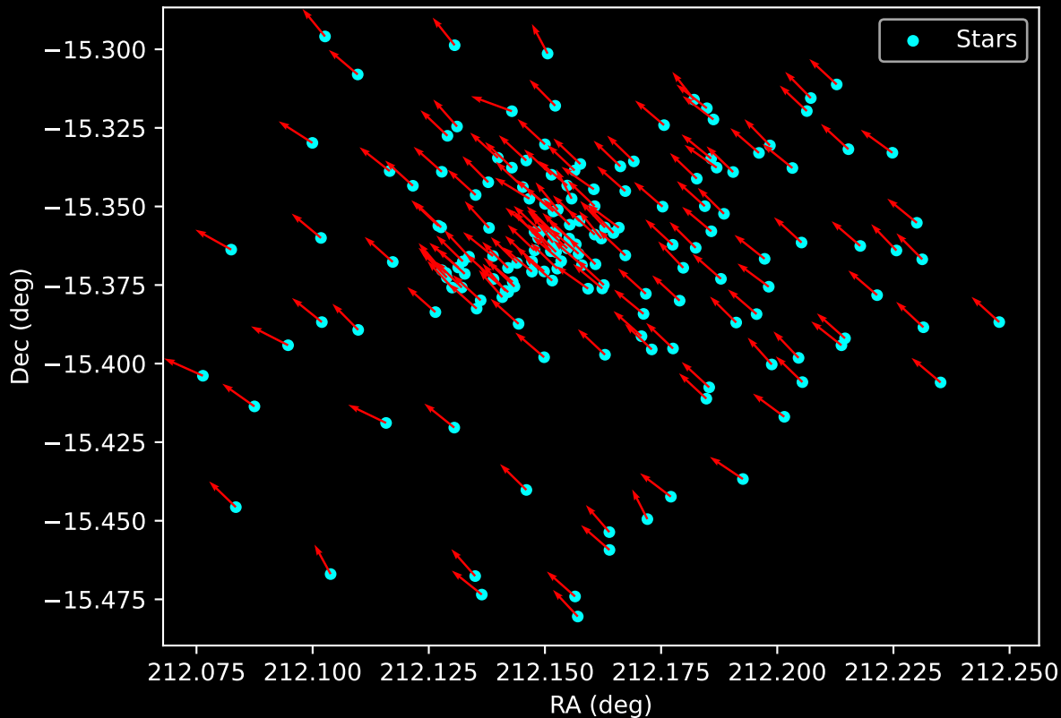
Gaia Cluster: [Haffner_10] Proper Motion Vectors for Gaia Star Field (n= 165)
