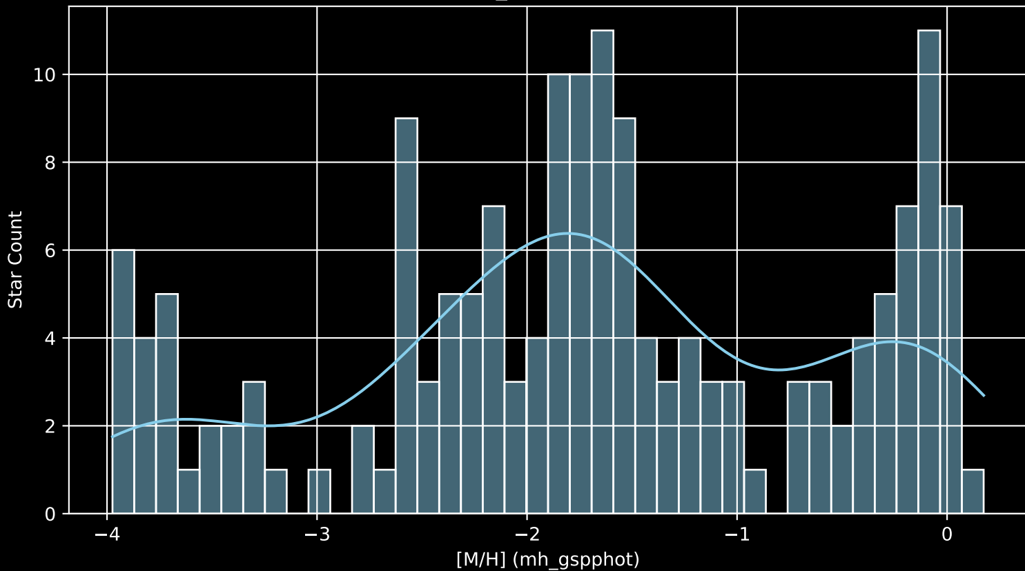
Gaia Cluster: [Haffner_10 [M/H] (mh_gspphot) (n= 165)
