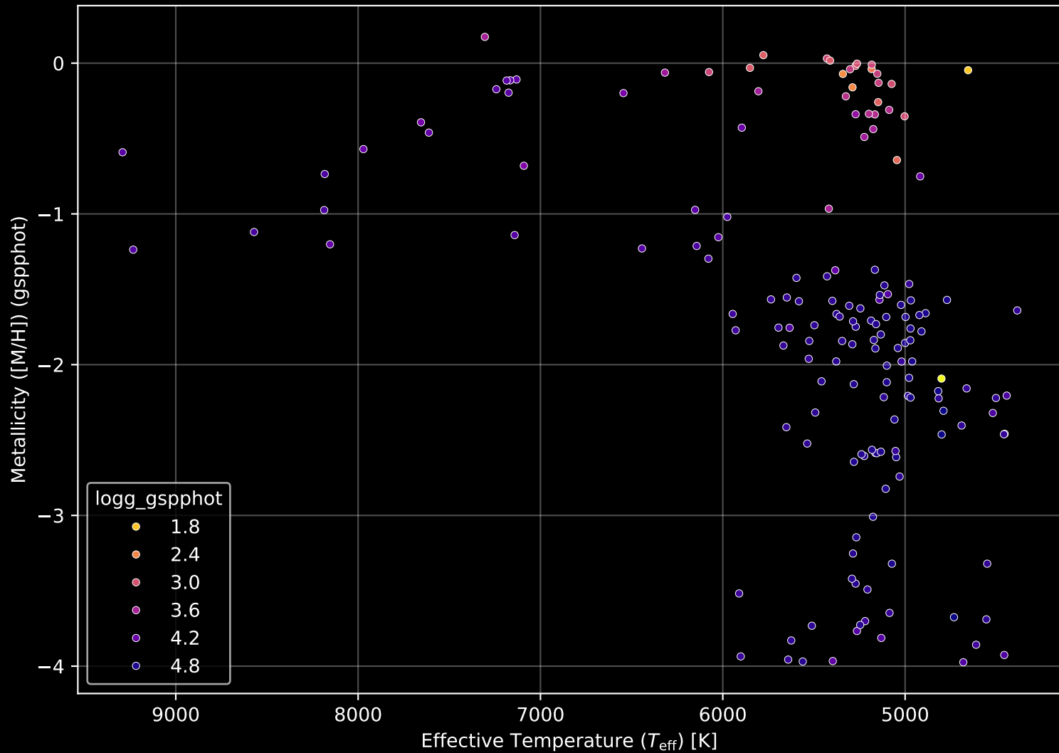
Gaia Cluster: [Haffner_10] Stellar Population Parameters (n= 165)
