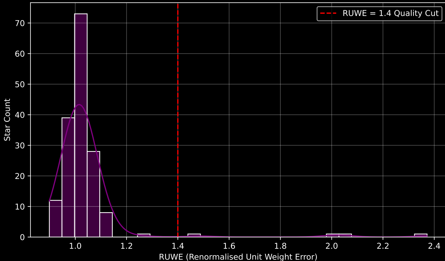
Gaia Cluster: [Haffner_10] RUWE Distribution (n= 165)
