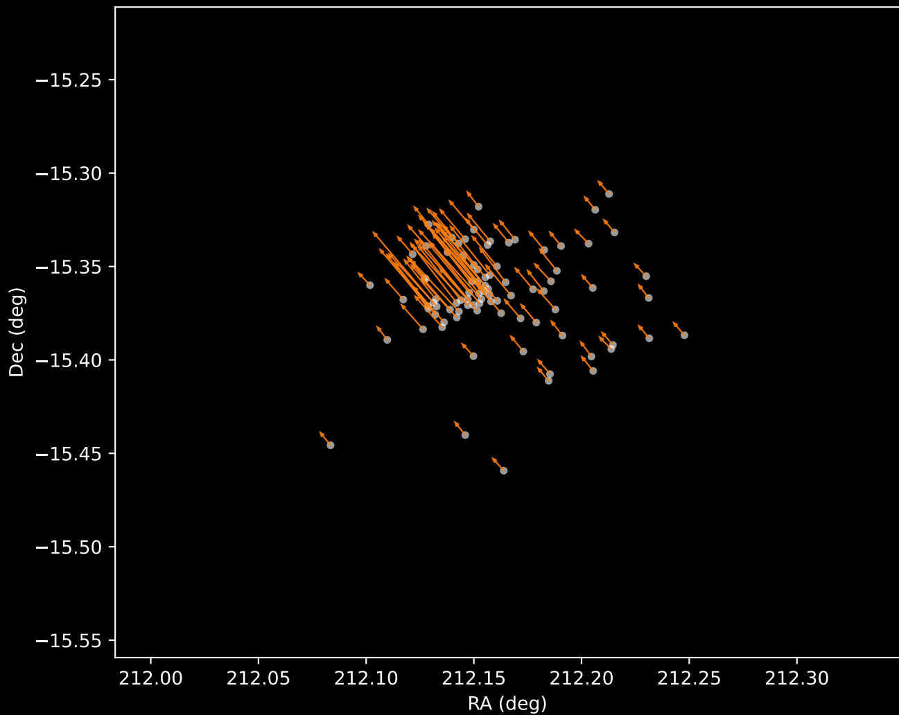
Gaia DR3 Cluster 2 Proper Motion Vectors (n=87)
