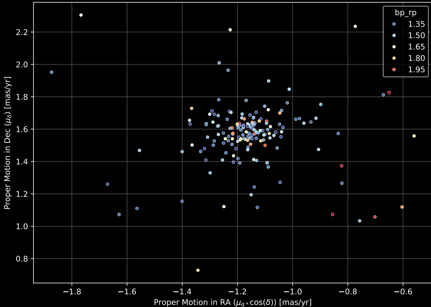
Gaia Cluster: [Haffner_10] Proper Motion Diagram (n= 165)
