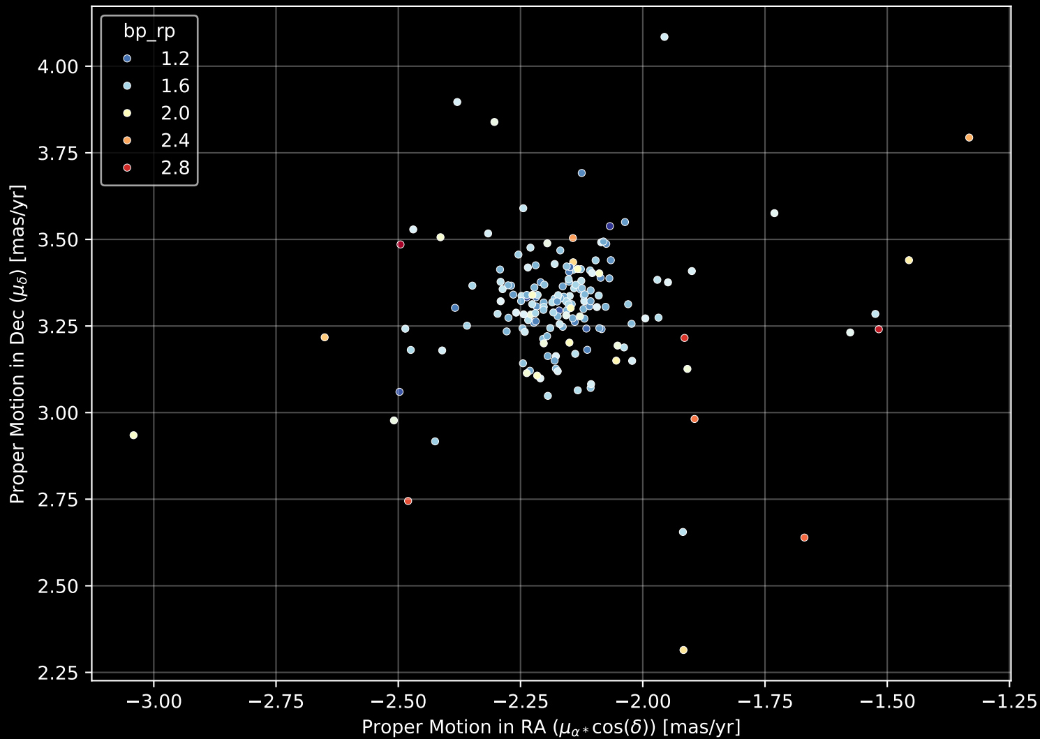
Gaia Cluster: [Haffner_15] Proper Motion Diagram (n= 175)
