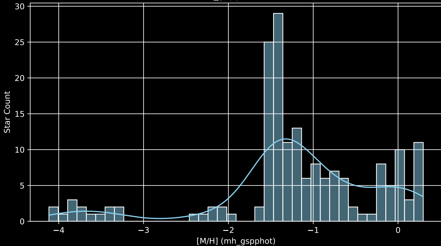
Gaia Cluster: [Haffner_15 [M/H] (mh_gspphot) (n= 175)
