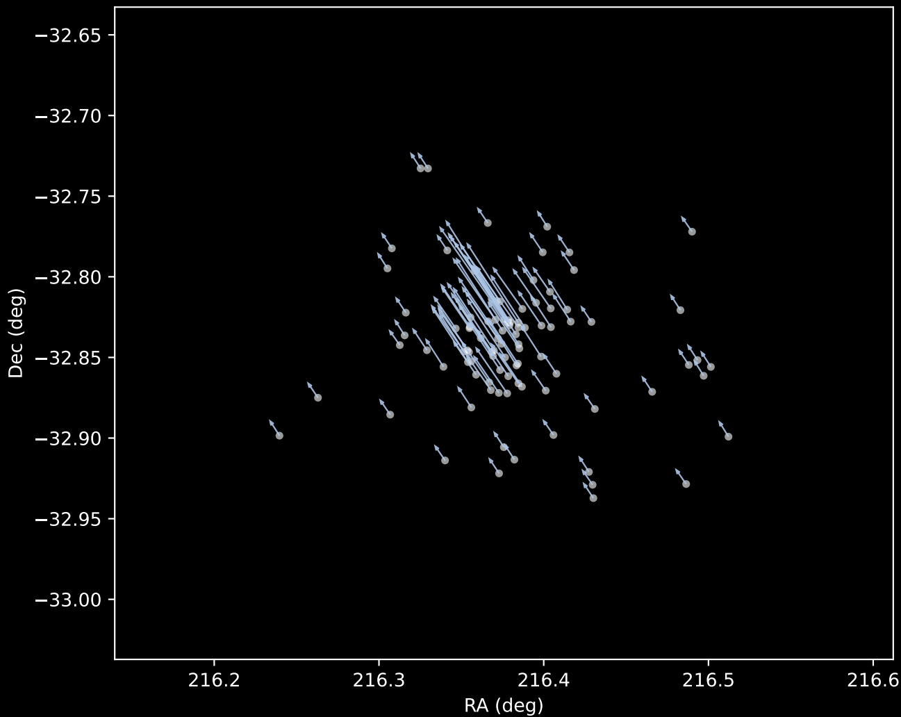
Gaia DR3 Cluster 1 Proper Motion Vectors (n=94)
