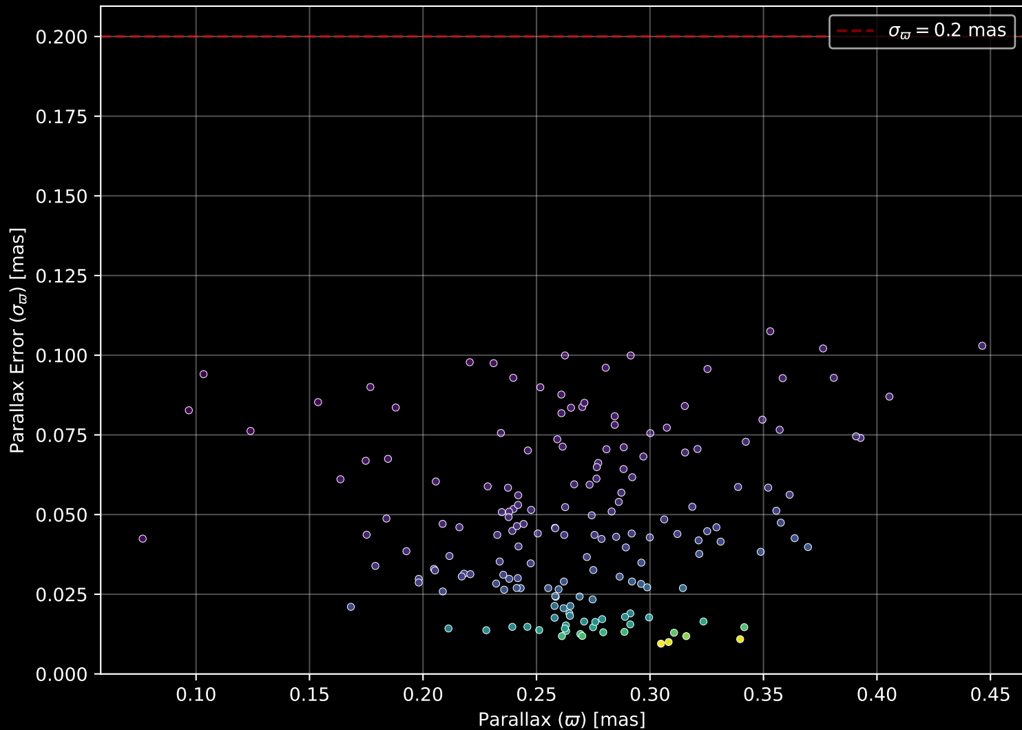
Gaia Cluster: [Haffner_15] Parallax Quality (n= 175)
