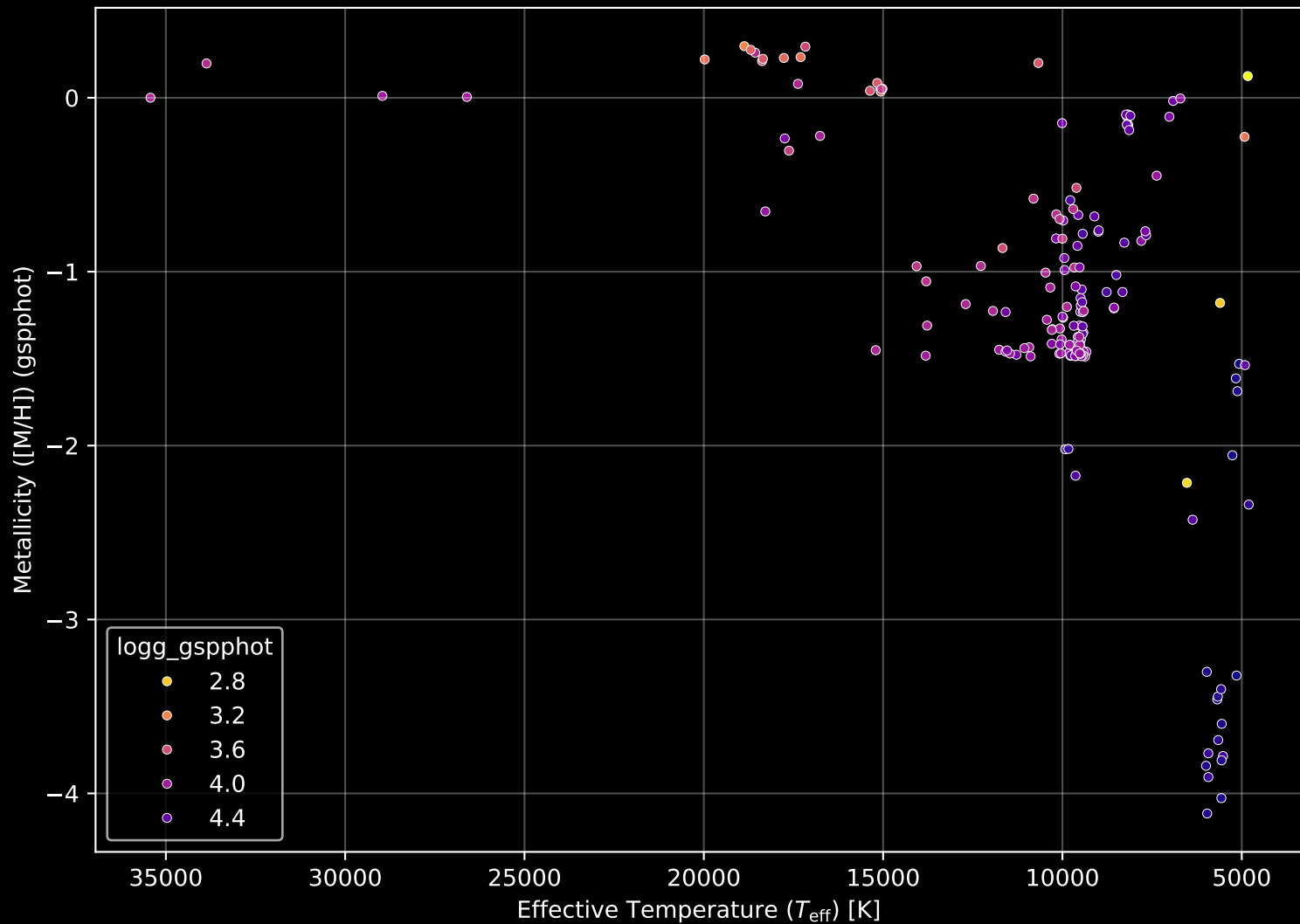
Gaia Cluster: [Haffner_15] Stellar Population Parameters (n= 175)
