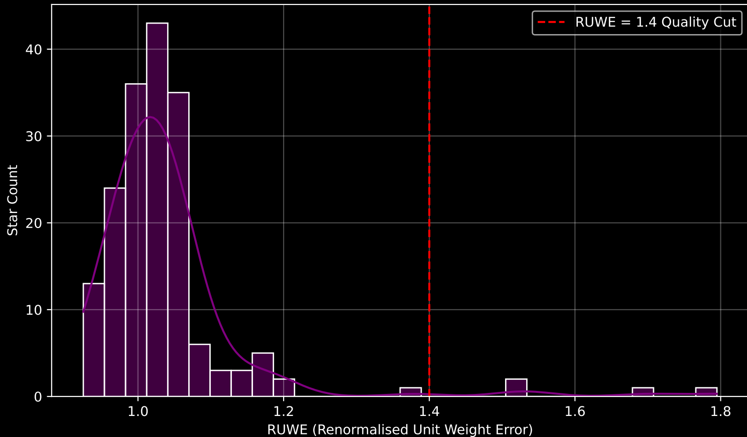
Gaia Cluster: [Haffner_15] RUWE Distribution (n= 175)
