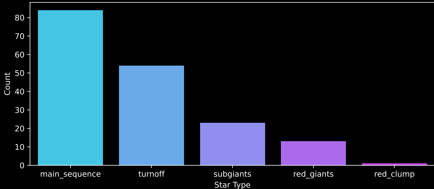
Gaia Cluster: [Haffner_15] Count plot of Star Type
