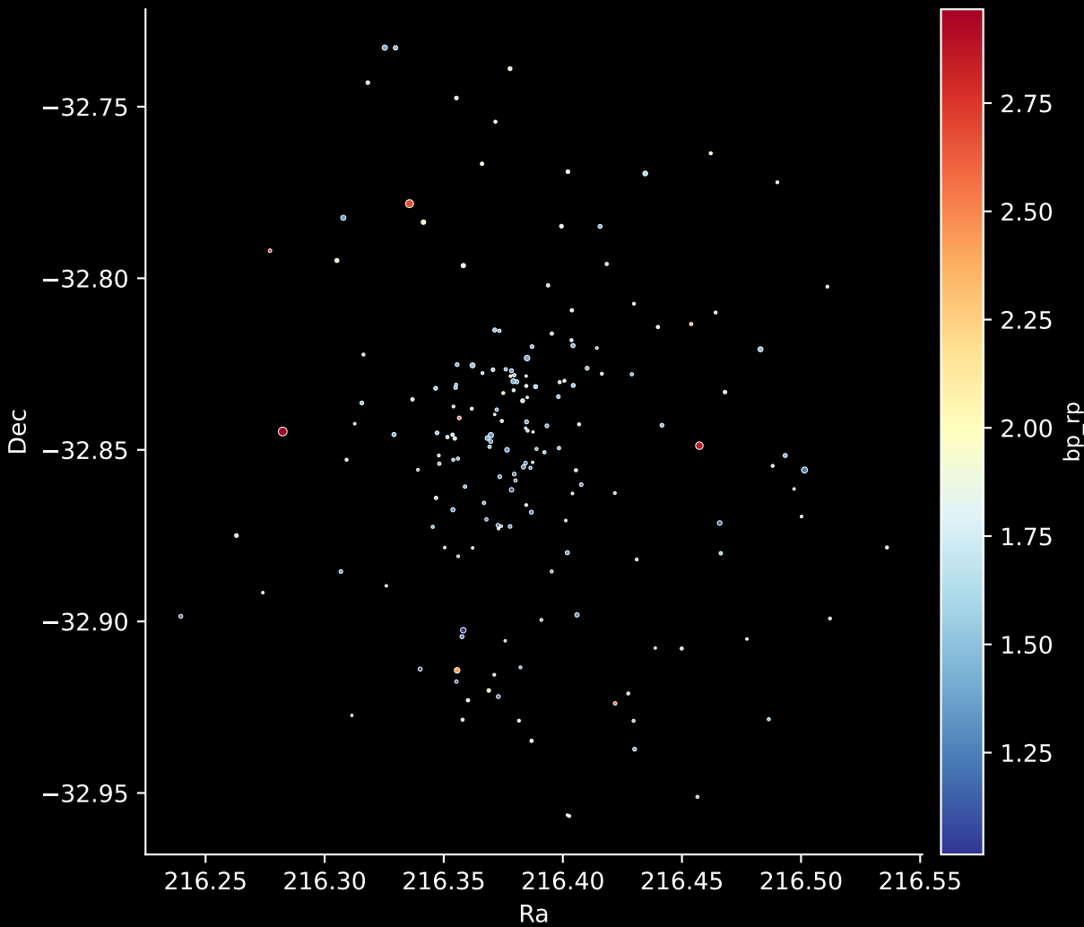
Gaia Cluster: [Haffner_15] Stars: 175
