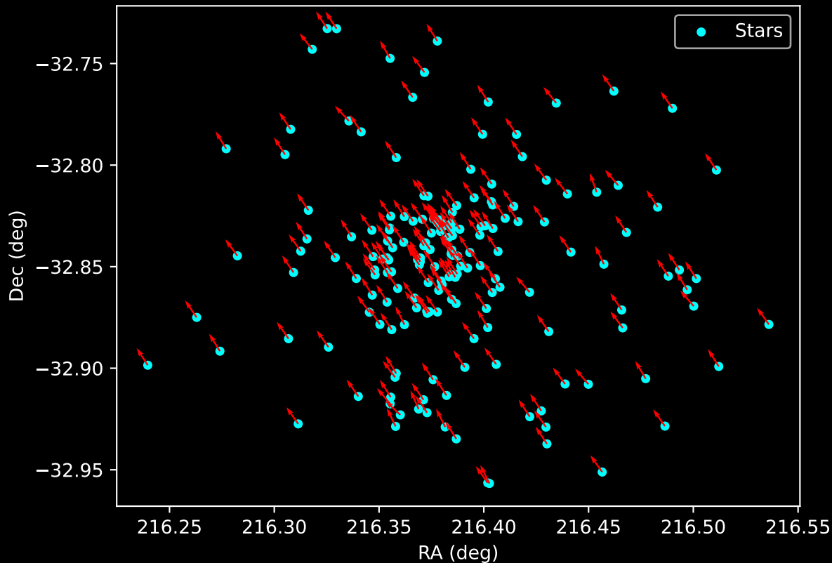
Gaia Cluster: [Haffner_15] Proper Motion Vectors for Gaia Star Field (n= 175)
