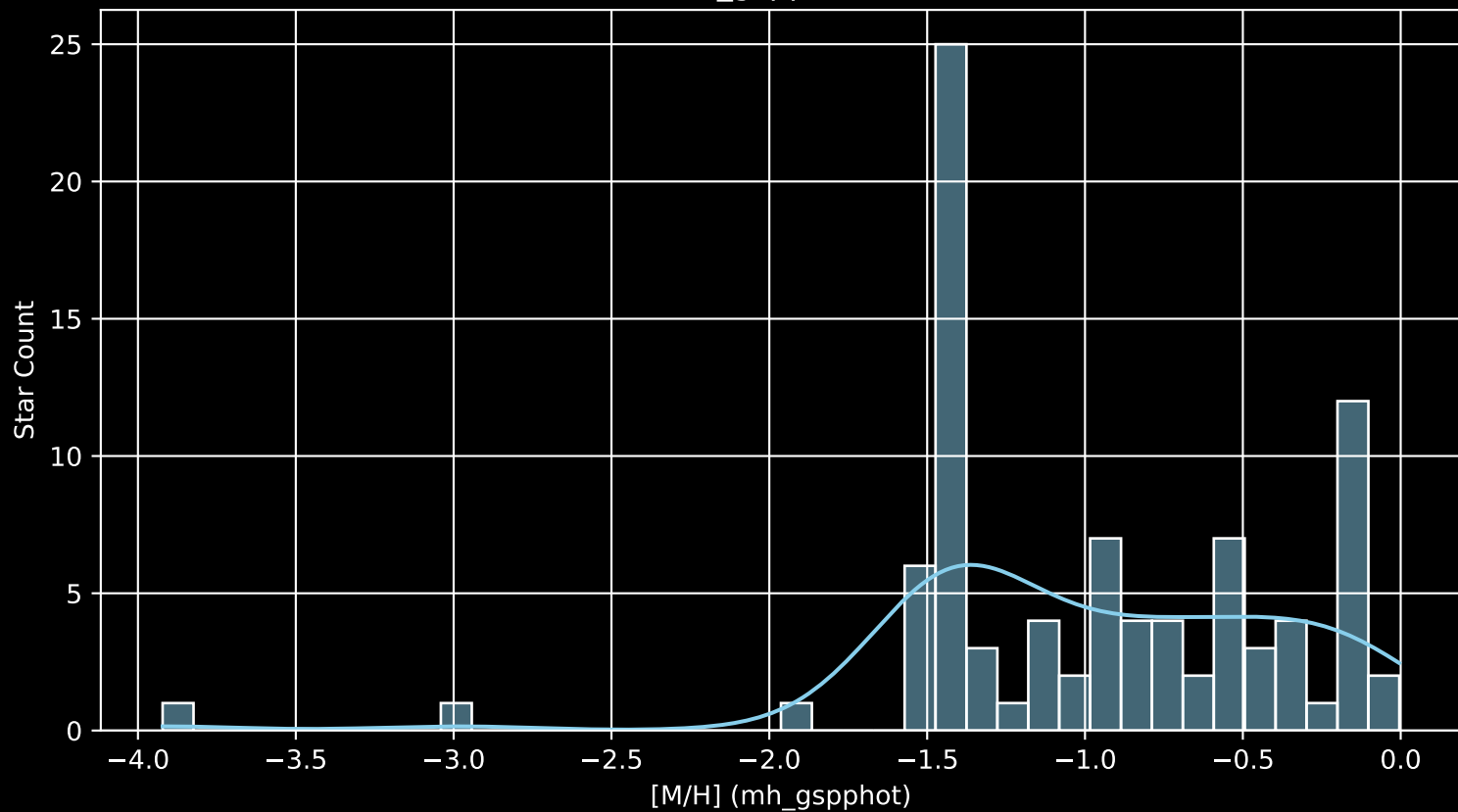
Gaia Cluster: [Haffner_17 [M/H] (mh_gspphot) (n= 90)
