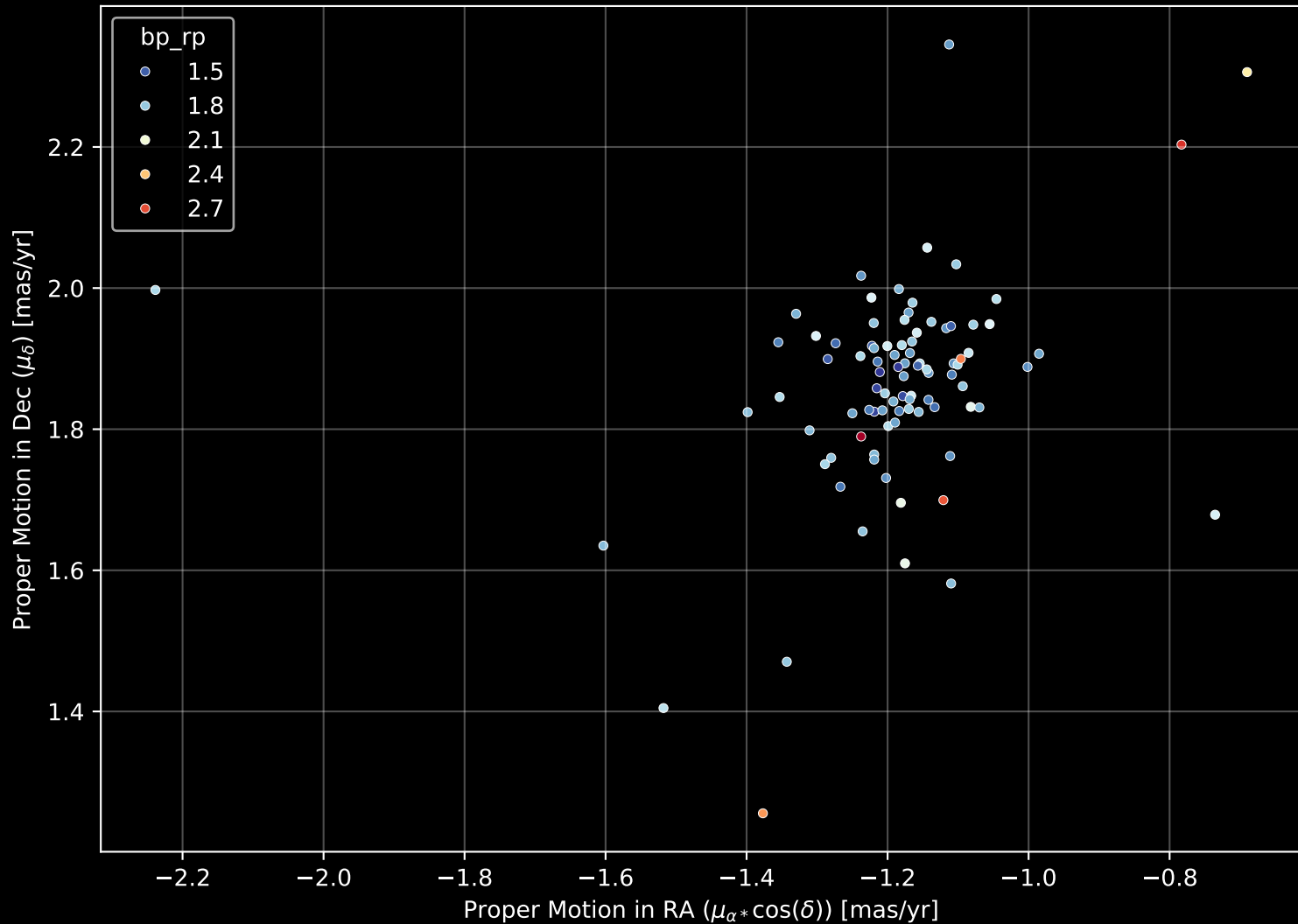
Gaia Cluster: [Haffner_17] Proper Motion Diagram (n= 90)
