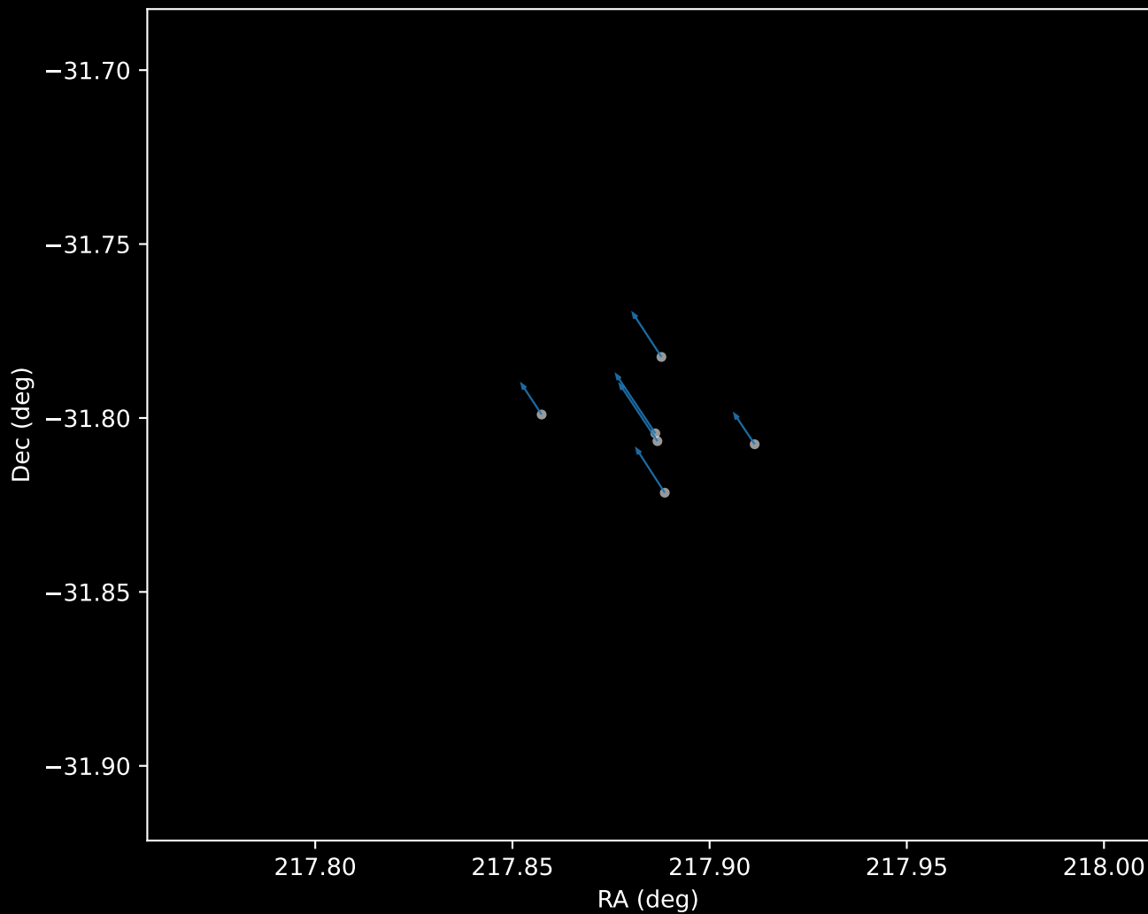
Gaia DR3 Cluster 0 Proper Motion Vectors (n=6)
