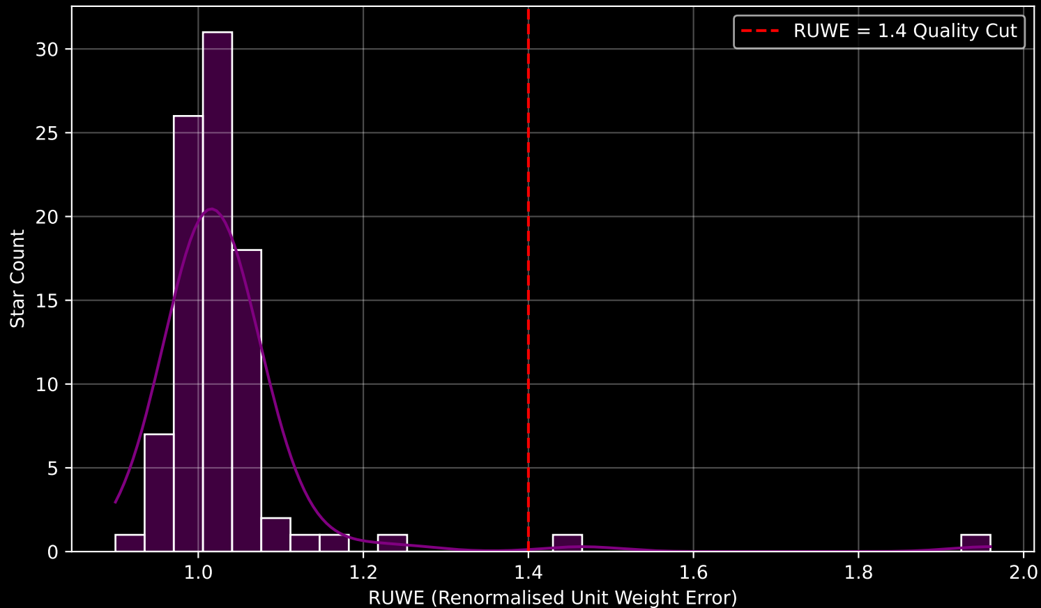
Gaia Cluster: [Haffner_17] RUWE Distribution (n= 90)
