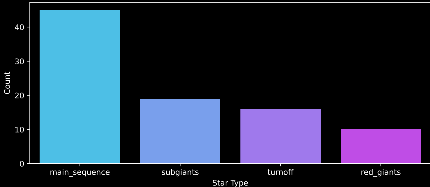
Gaia Cluster: [Haffner_17] Count plot of Star Type
