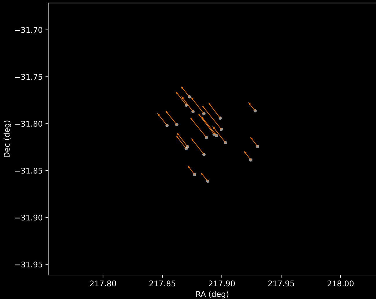
Gaia DR3 Cluster 2 Proper Motion Vectors (n=20)
