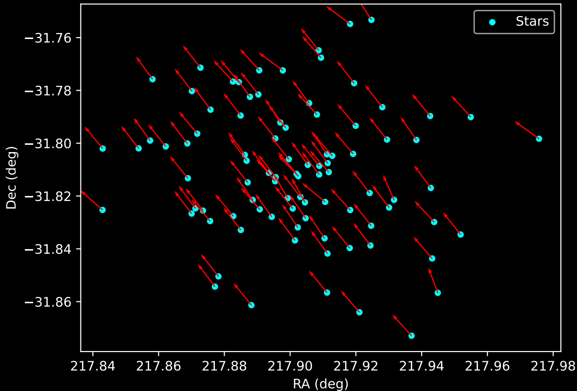
Gaia Cluster: [Haffner_17] Proper Motion Vectors for Gaia Star Field (n= 90)
