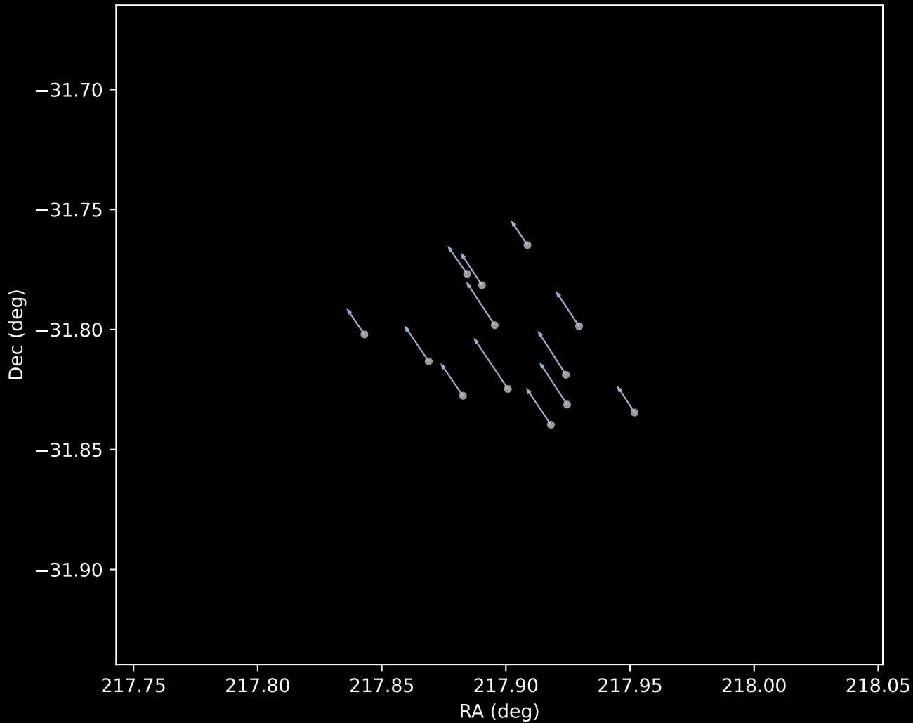
Gaia DR3 Cluster 1 Proper Motion Vectors (n=13)
