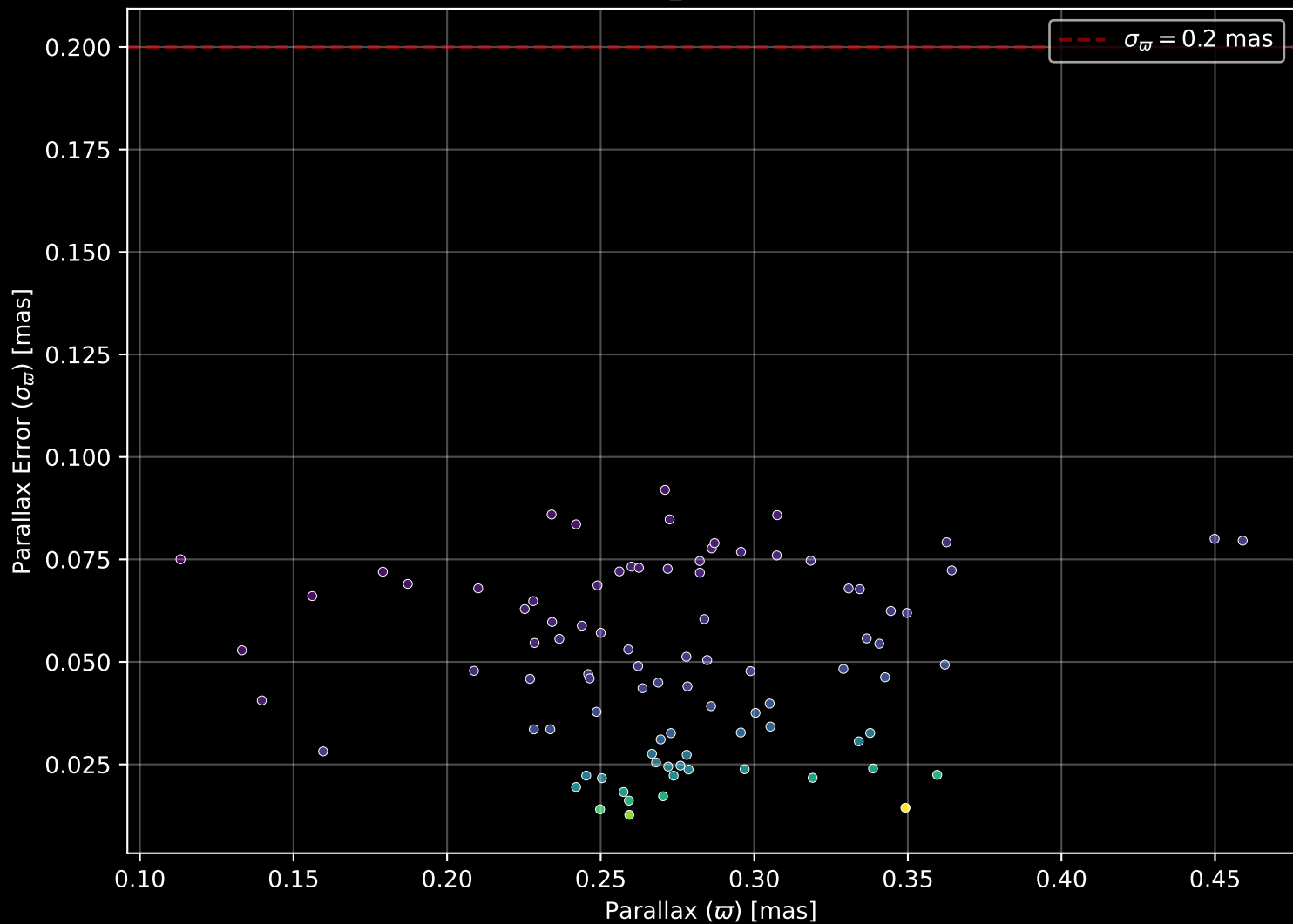
Gaia Cluster: [Haffner_17] Parallax Quality (n= 90)
