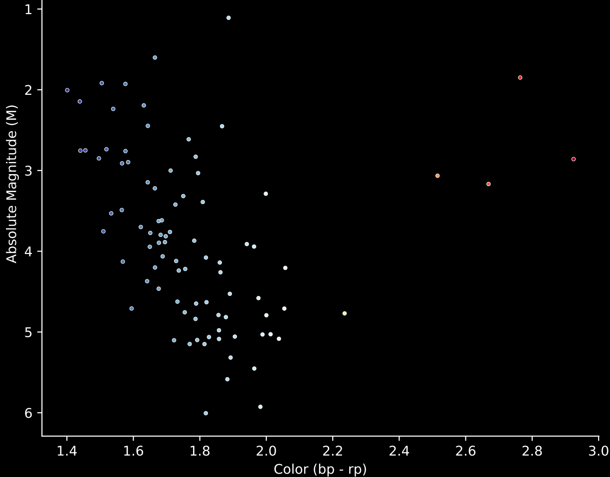
Gaia Cluster: [Haffner_17] Stars (n= 90) Hertzsprung-Russel Diagram
