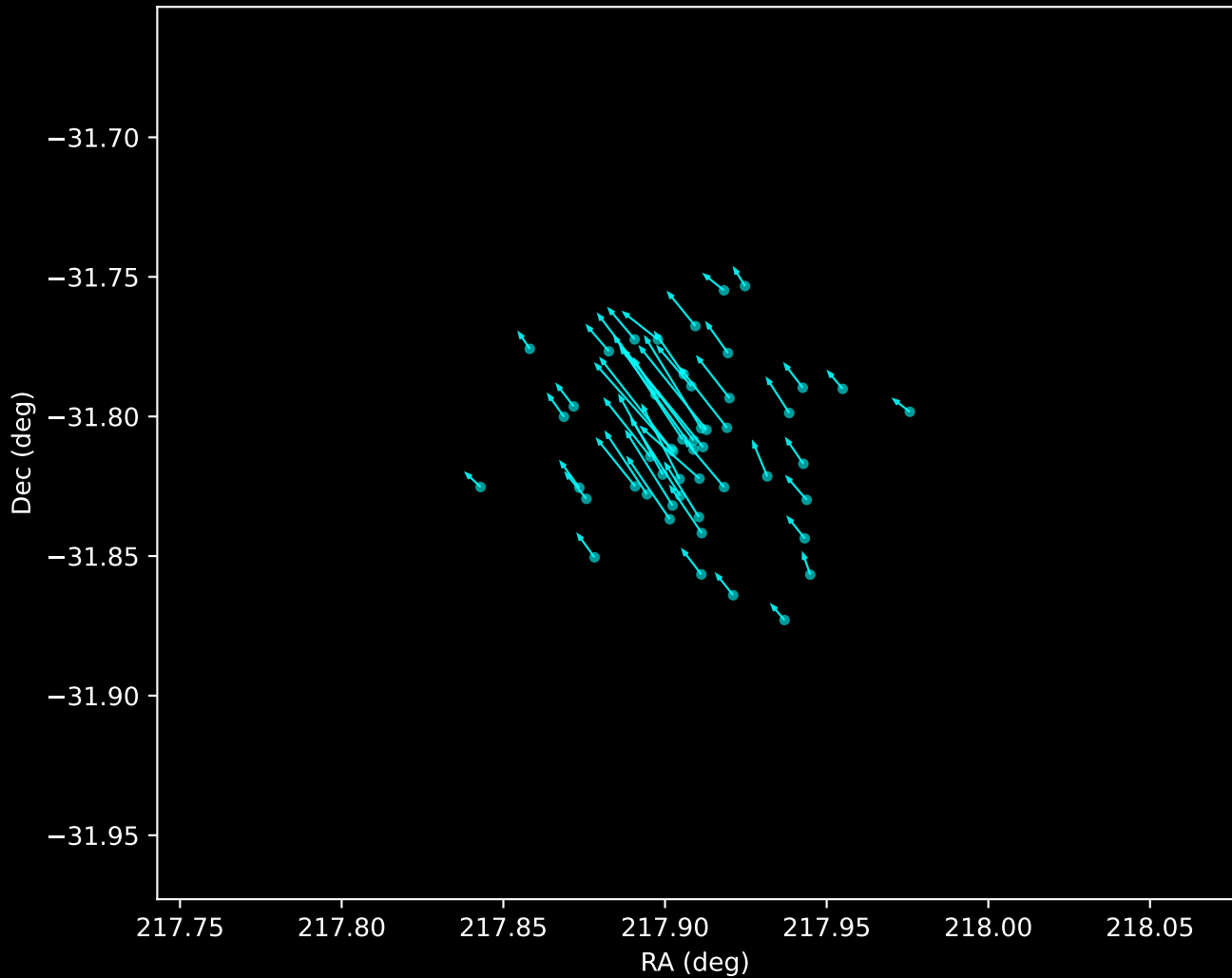
Gaia DR3 Noise Stream Proper Motion Vectors (n=51)
