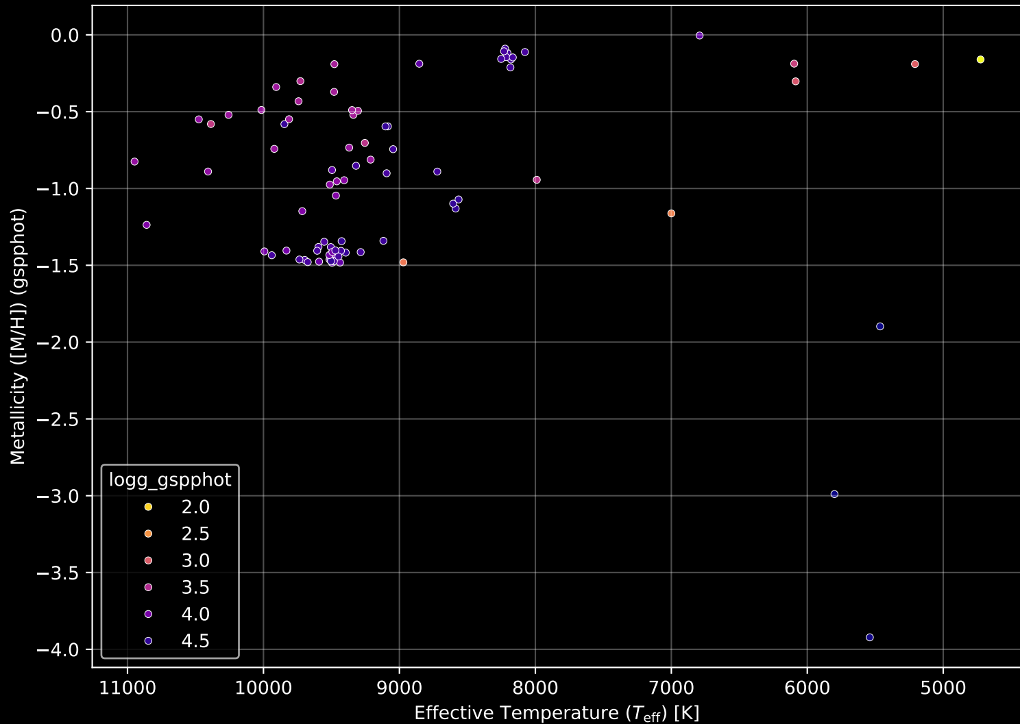
Gaia Cluster: [Haffner_17] Stellar Population Parameters (n= 90)
