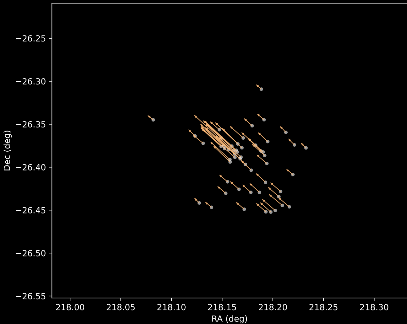
Gaia DR3 Cluster 3 Proper Motion Vectors (n=53)
