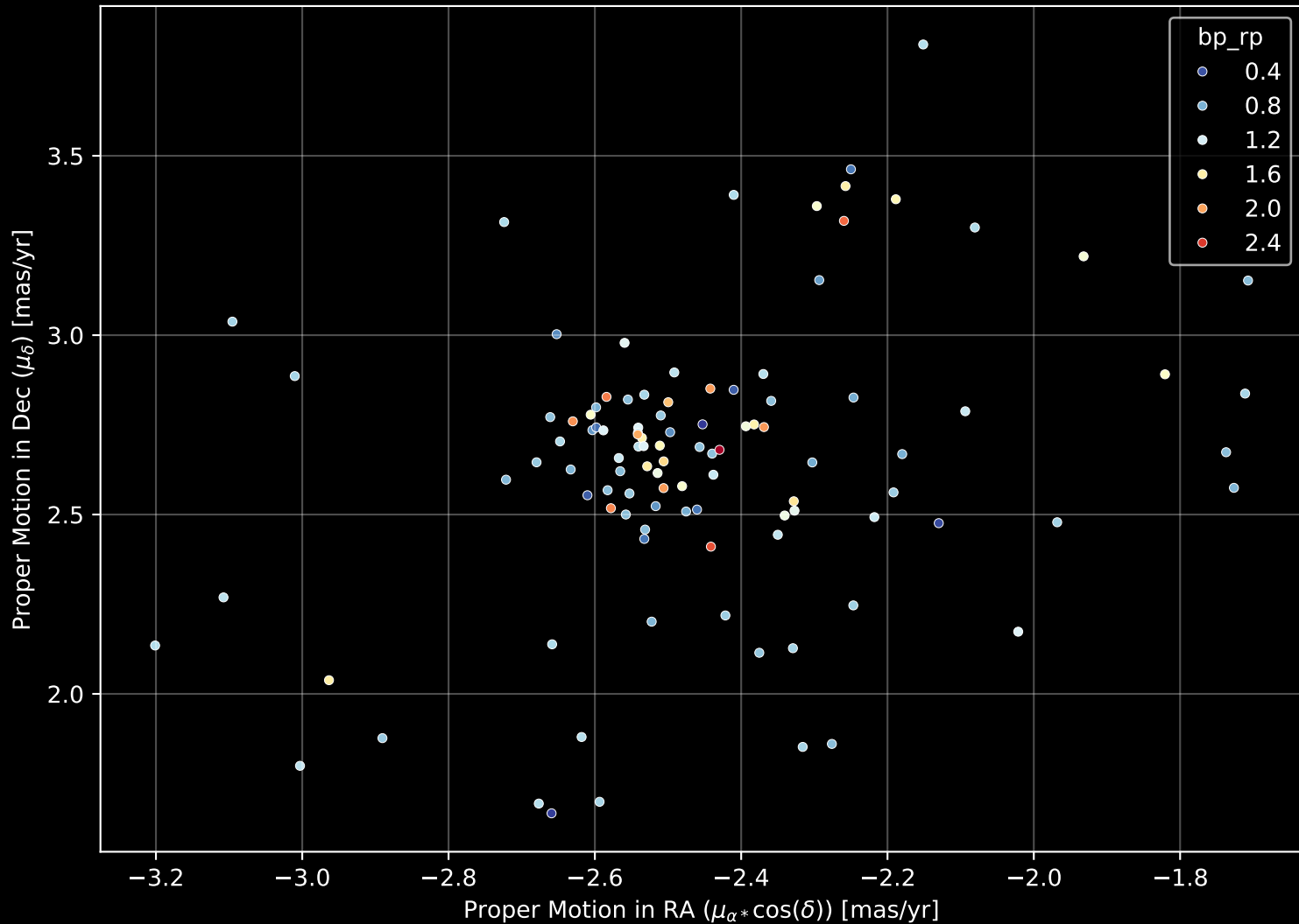
Gaia Cluster: [Haffner_18] Proper Motion Diagram (n= 105)
