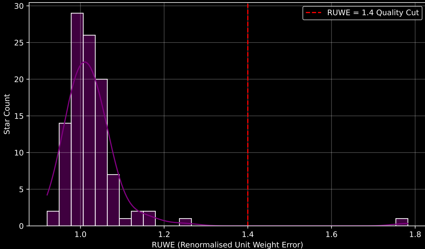
Gaia Cluster: [Haffner_18] RUWE Distribution (n= 105)
