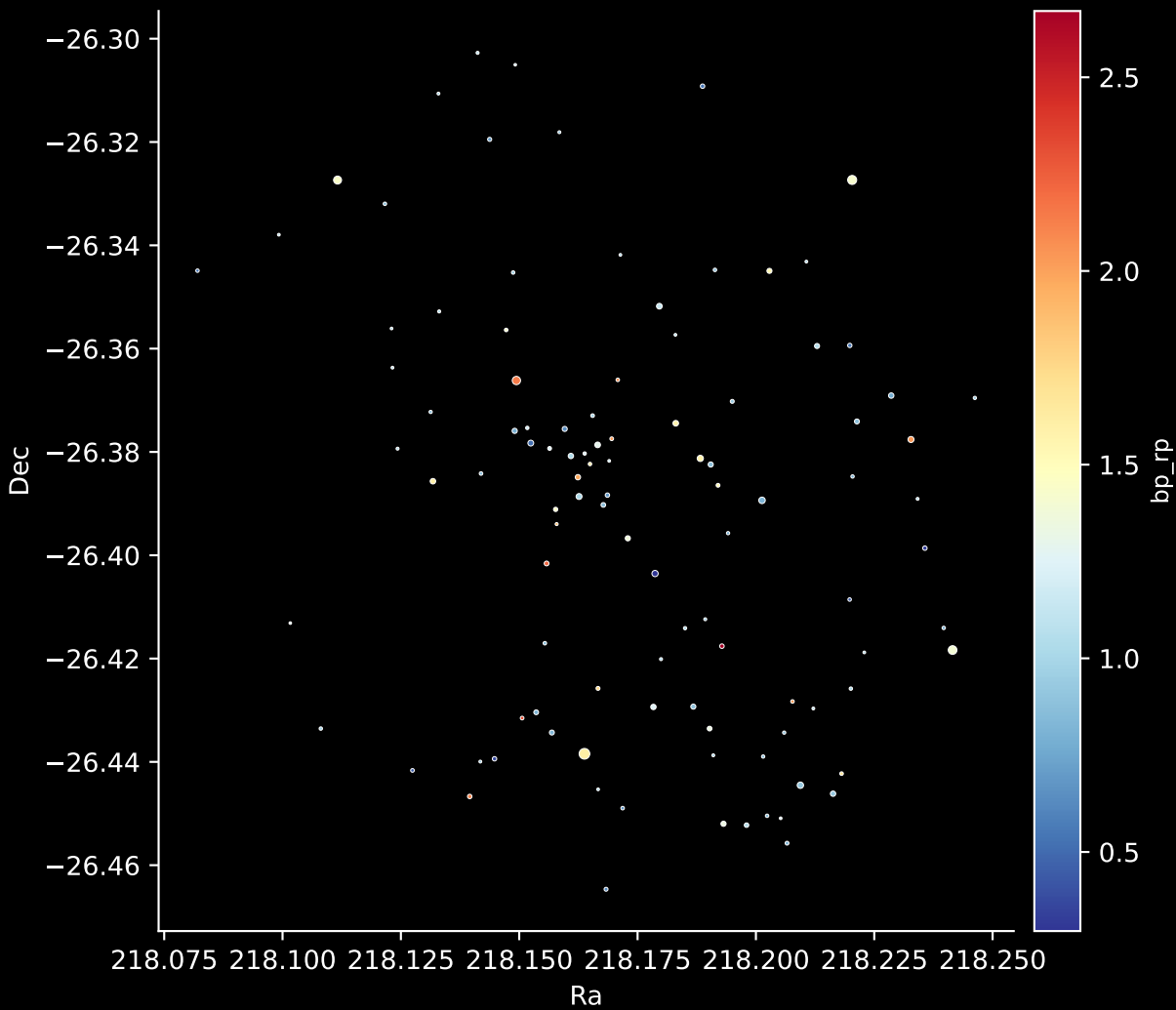
Gaia Cluster: [Haffner_18] Stars: 105
