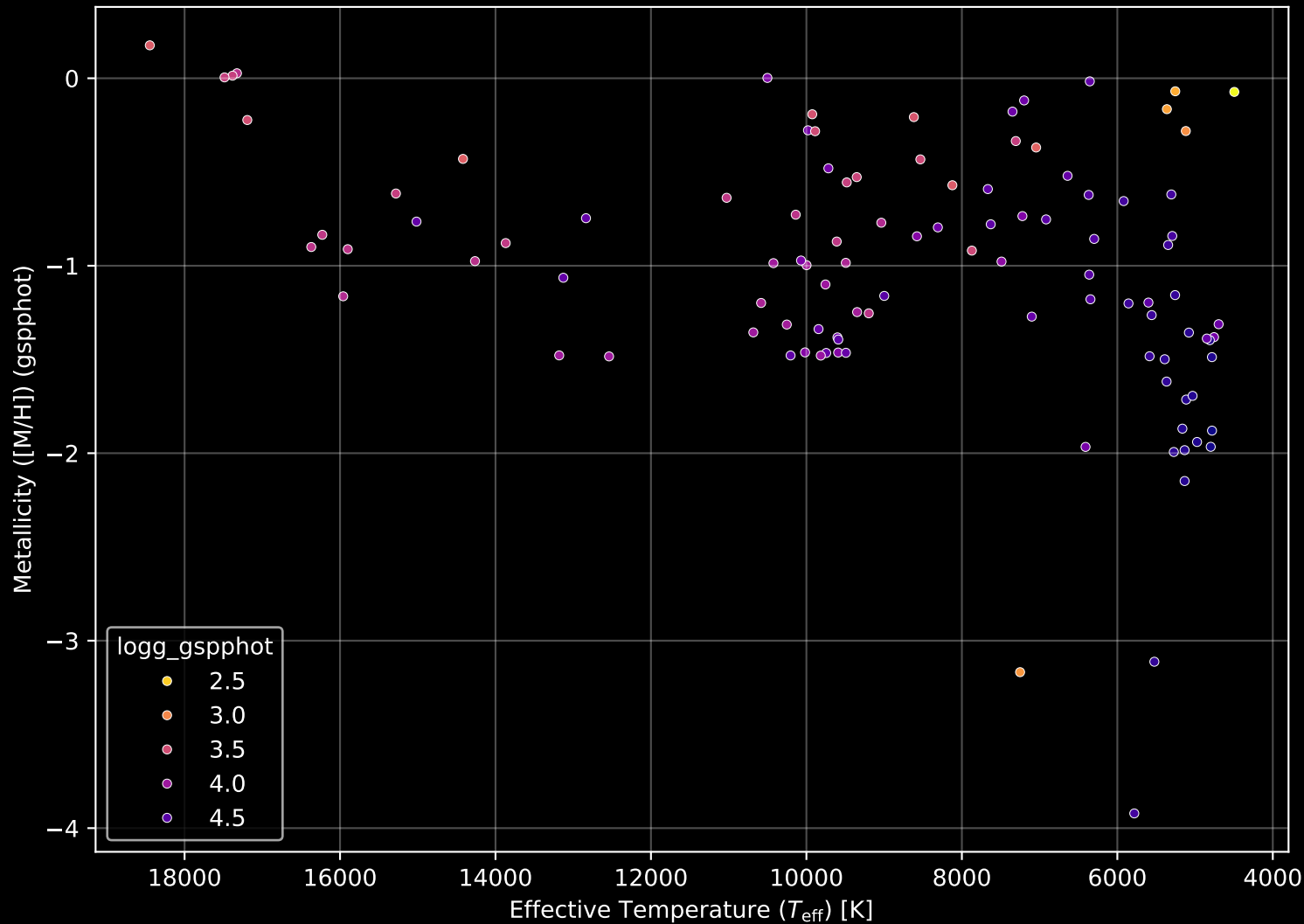
Gaia Cluster: [Haffner_18] Stellar Population Parameters (n= 105)
