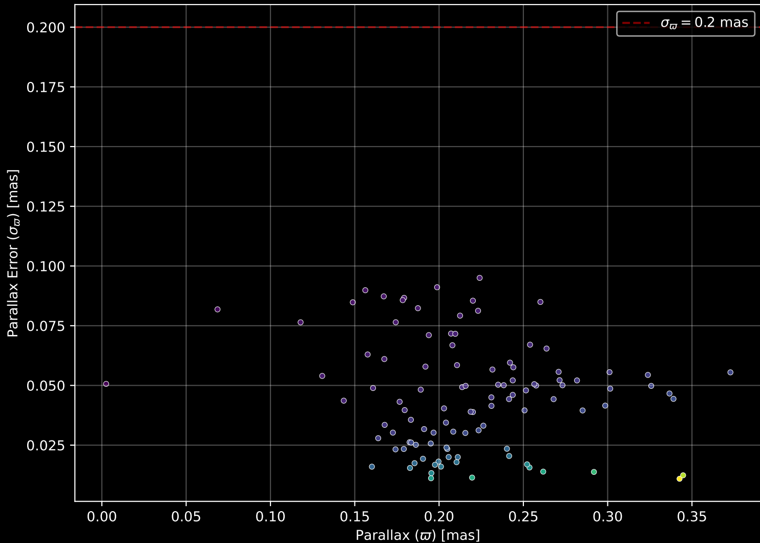
Gaia Cluster: [Haffner_18] Parallax Quality (n= 105)
