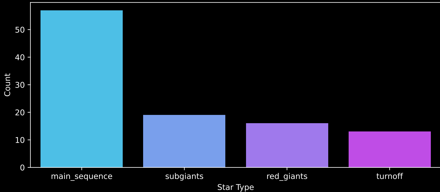
Gaia Cluster: [Haffner_18] Count plot of Star Type
