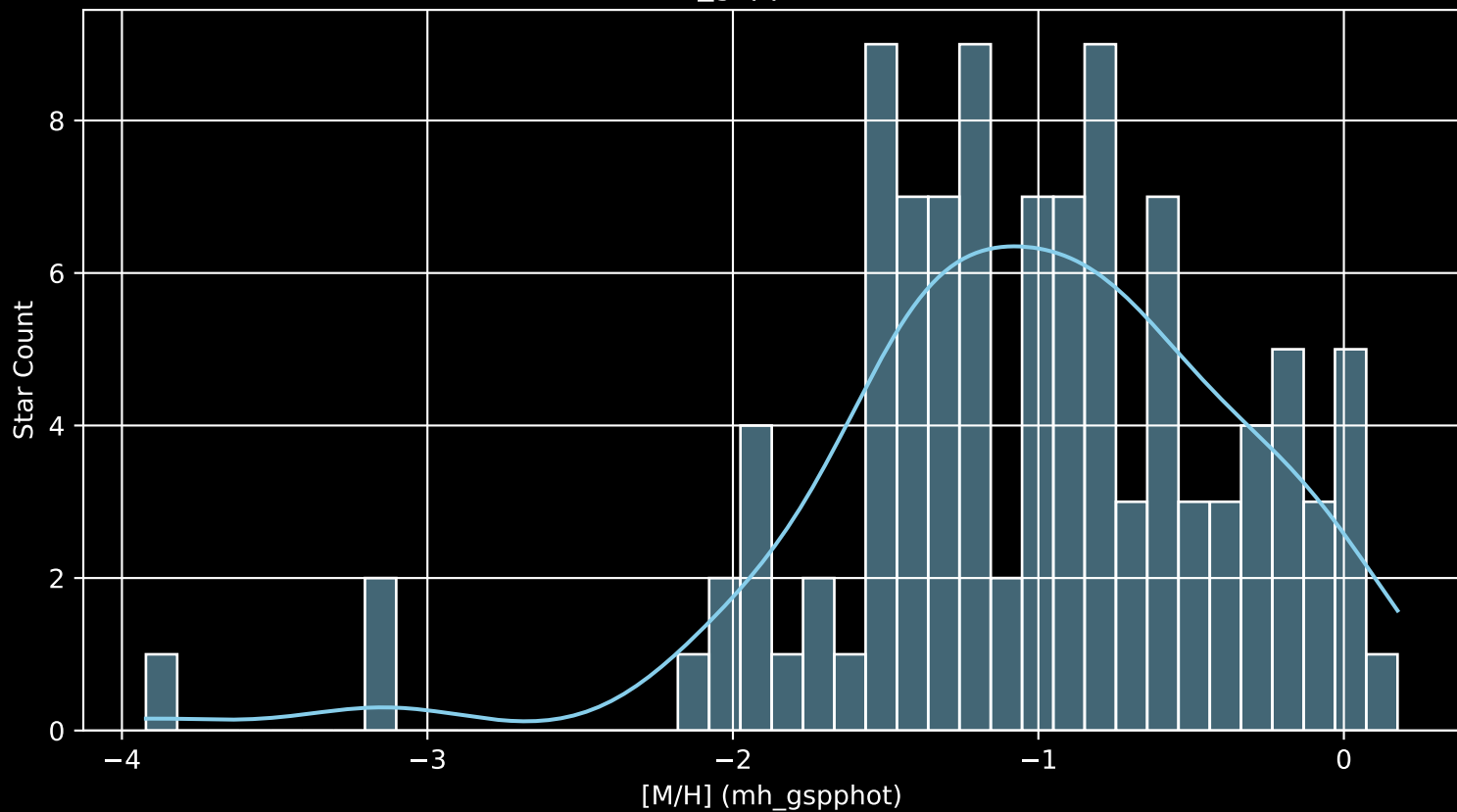
Gaia Cluster: [Haffner_18 [M/H] (mh_gspphot) (n= 105)
