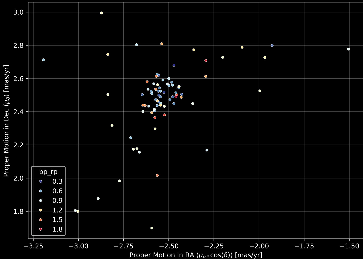
Gaia Cluster: [Haffner_19] Proper Motion Diagram (n= 82)
