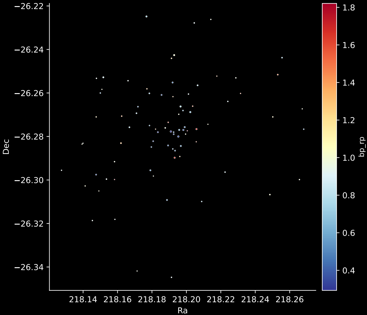
Gaia Cluster: [Haffner_19] Stars: 82
