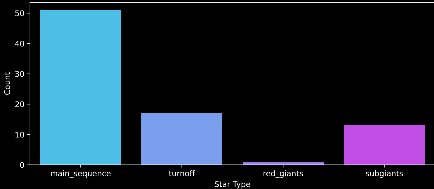
Gaia Cluster: [Haffner_19] Count plot of Star Type
