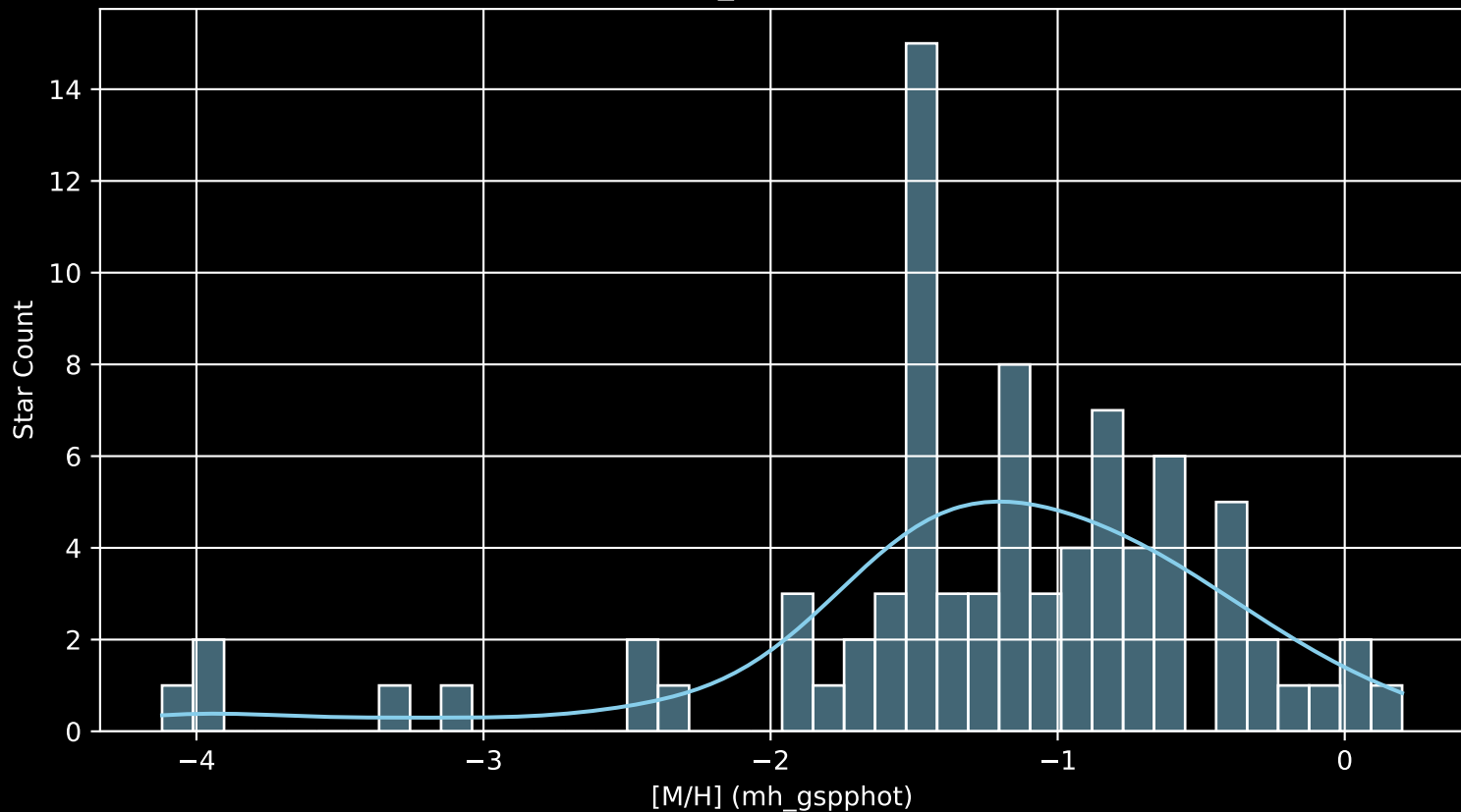
Gaia Cluster: [Haffner_19 [M/H] (mh_gspphot) (n= 82)
