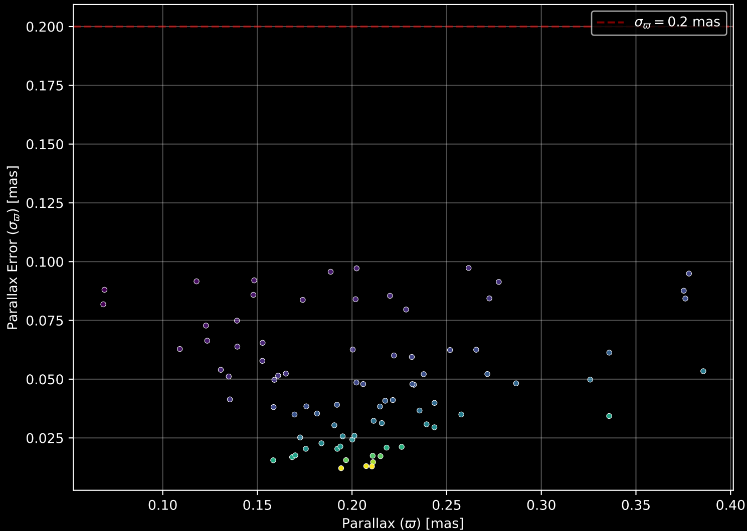
Gaia Cluster: [Haffner 19] Parallax Quality (n= 82)
