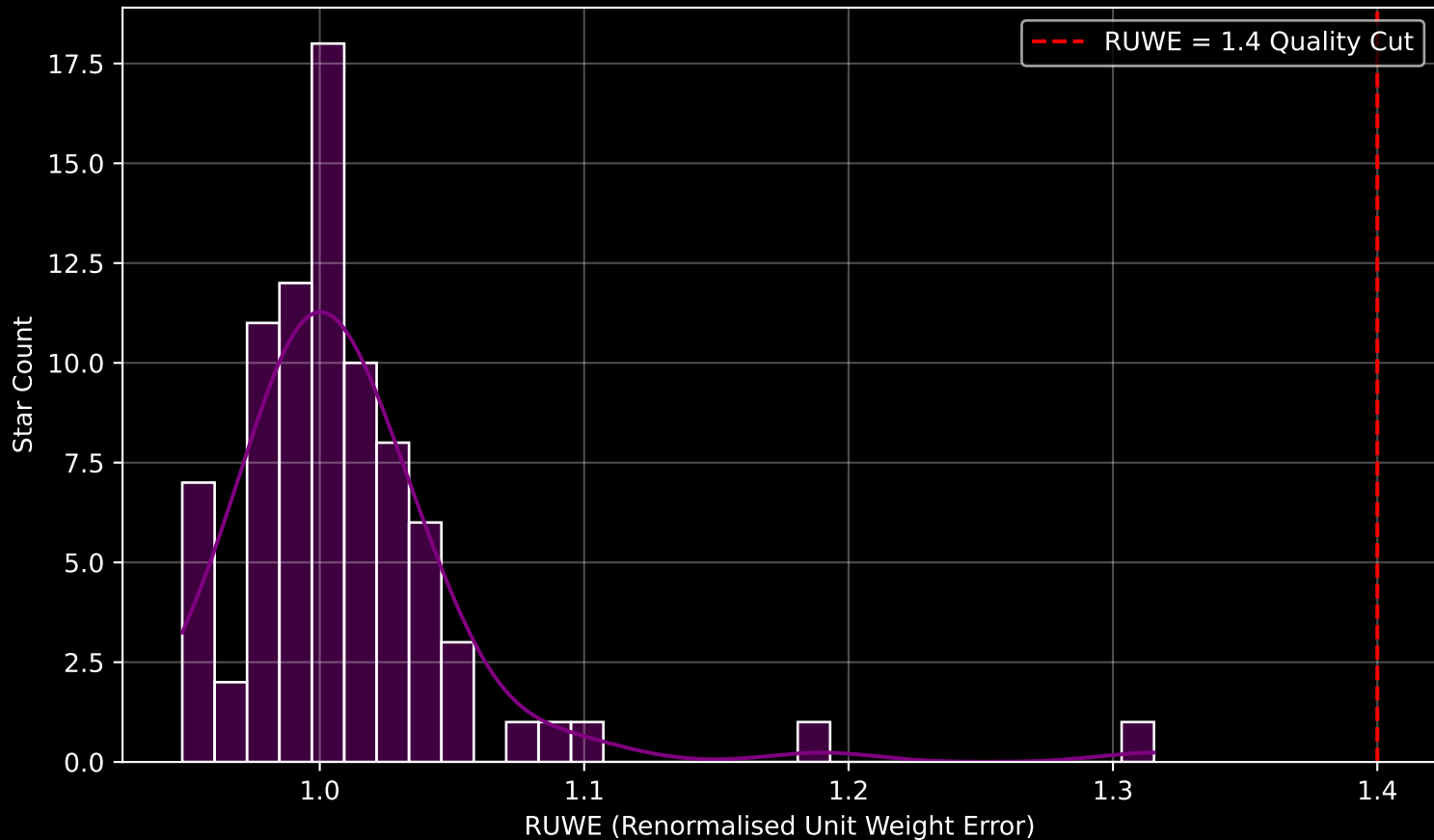
Gaia Cluster: [Haffner_19] RUWE Distribution (n= 82)
