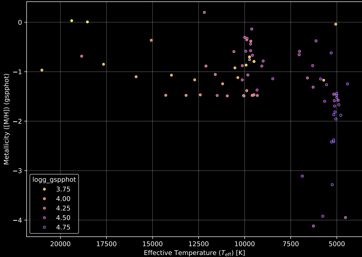
Gaia Cluster: [Haffner_19] Stellar Population Parameters (n= 82)
