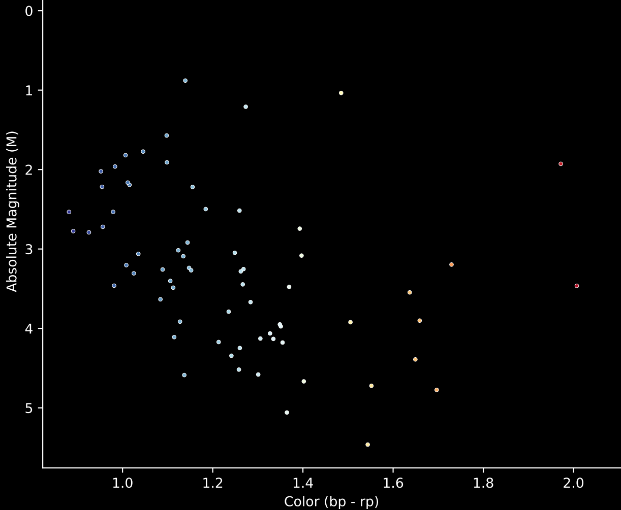
Gaia Cluster: [Haffner_20] Stars (n= 69) Hertzsprung-Russel Diagram
