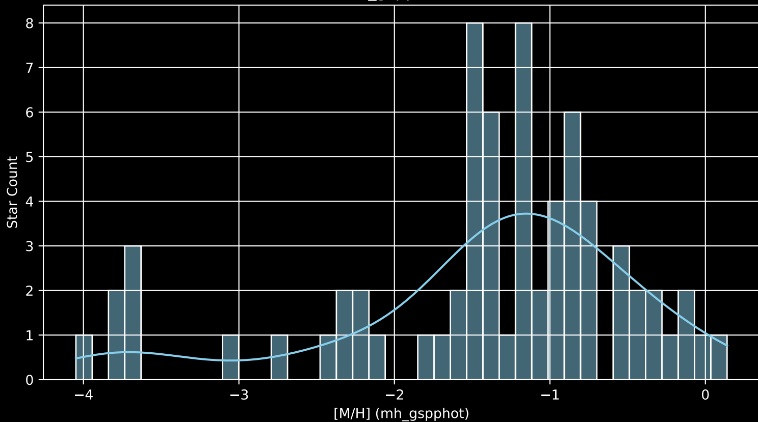
Gaia Cluster: [Haffner_20 [M/H] (mh_gspphot) (n= 69)
