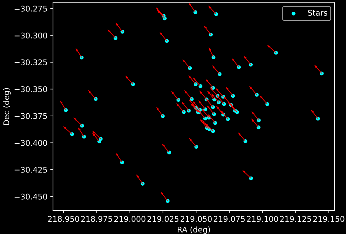
Gaia Cluster: [Haffner_20] Proper Motion Vectors for Gaia Star Field (n= 69)
