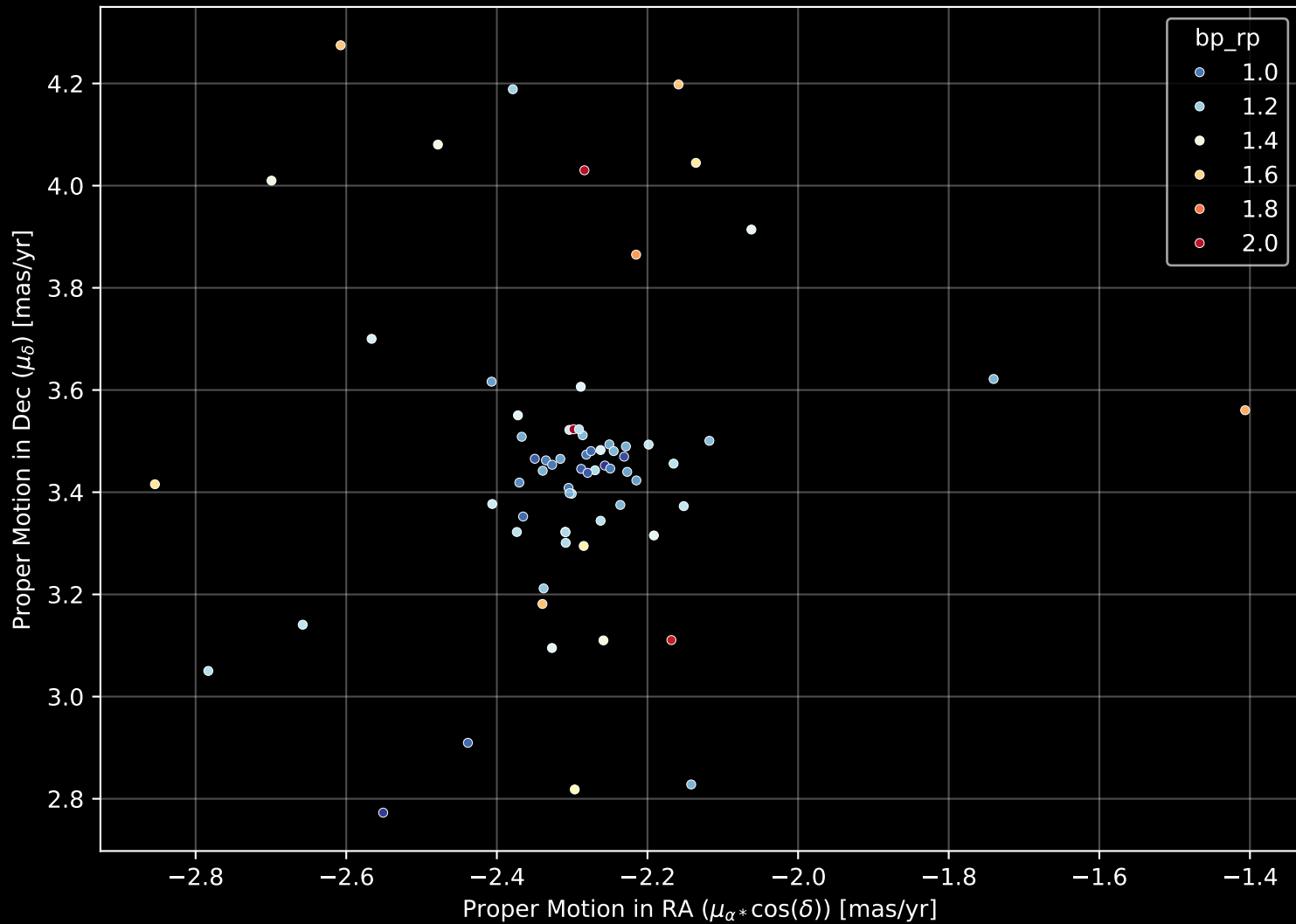
Gaia Cluster: [Haffner_20] Proper Motion Diagram (n= 69)
