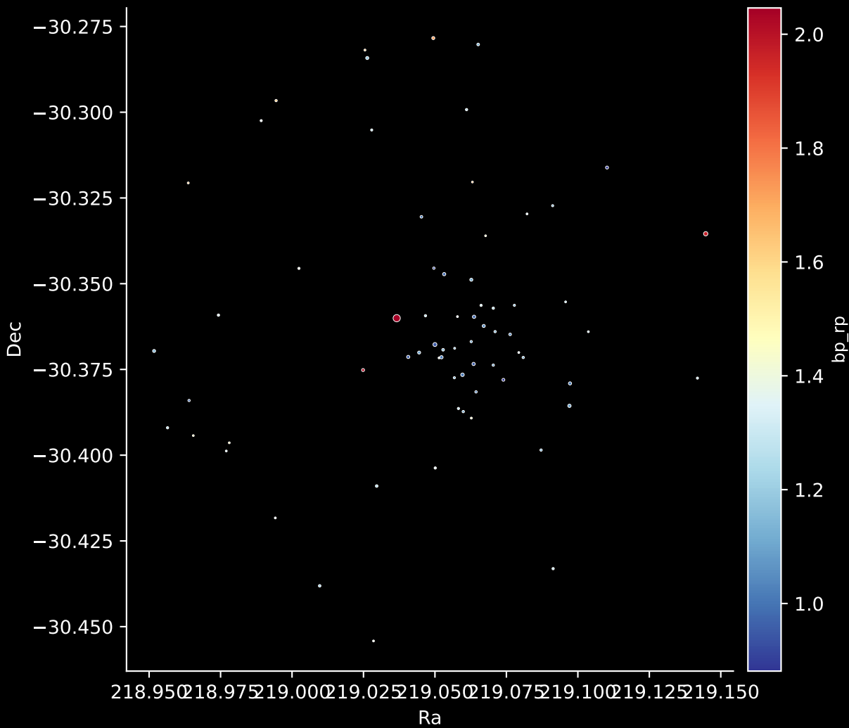
Gaia Cluster: [Haffner_20] Stars: 69
