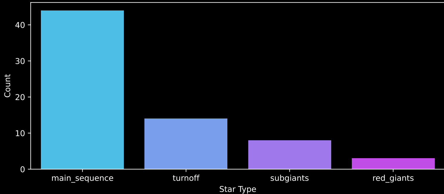
Gaia Cluster: [Haffner_20] Count plot of Star Type
