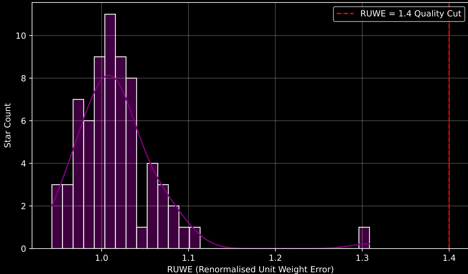
Gaia Cluster: [Haffner_20] RUWE Distribution (n= 69)
