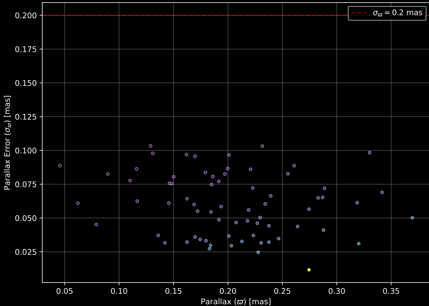
Gaia Cluster: [Haffner_20] Parallax Quality (n= 69)
