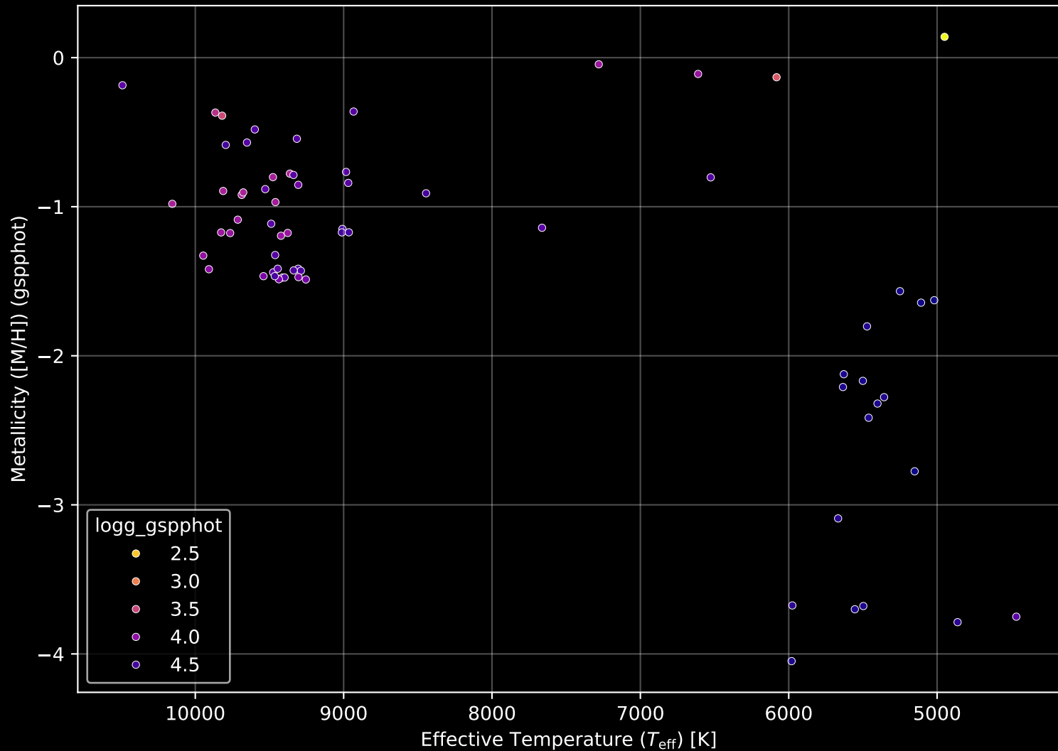
Gaia Cluster: [Haffner_20] Stellar Population Parameters (n= 69)
