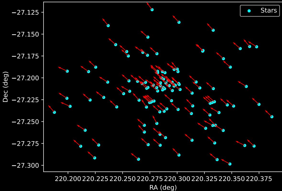
Gaia Cluster: [Haffner_21] Proper Motion Vectors for Gaia Star Field (n= 114)
