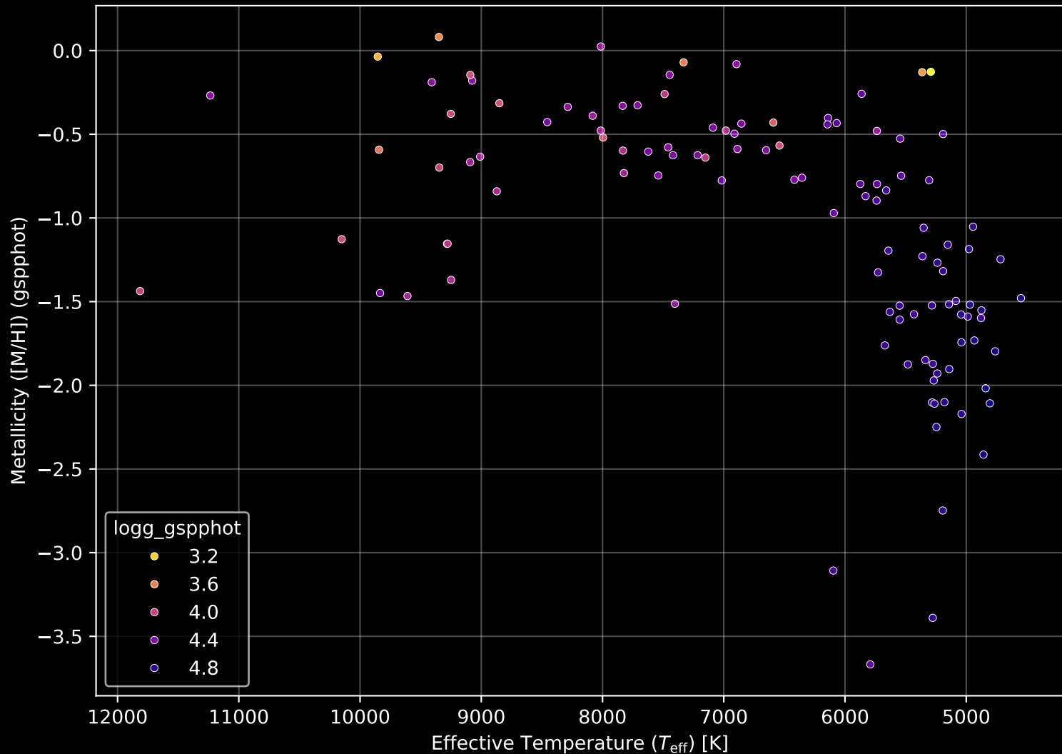
Gaia Cluster: [Haffner_21] Stellar Population Parameters (n= 114)
