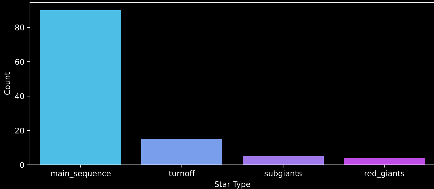
Gaia Cluster: [Haffner_21] Count plot of Star Type
