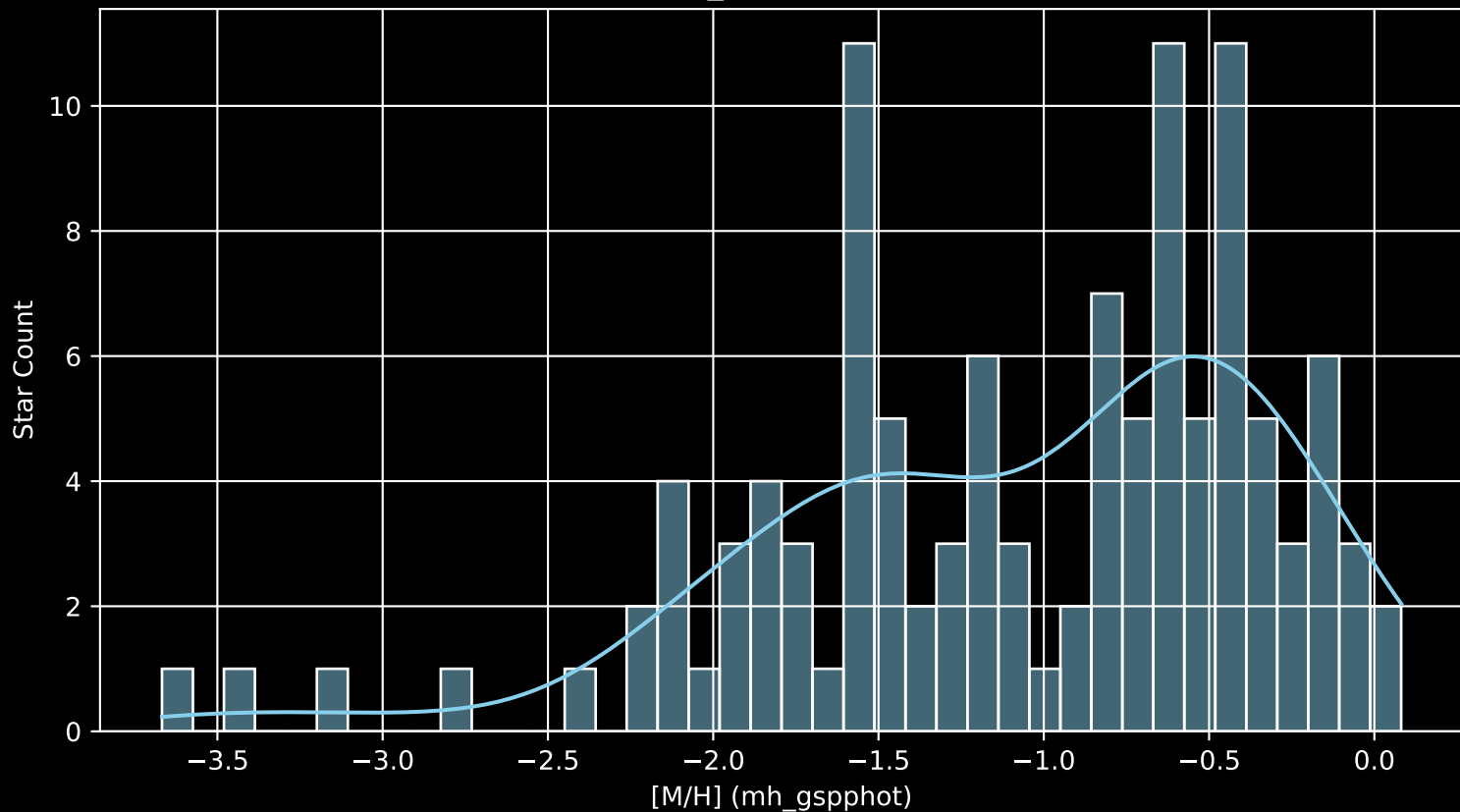
Gaia Cluster: [Haffner_21 [M/H] (mh_gspphot) (n= 114)
