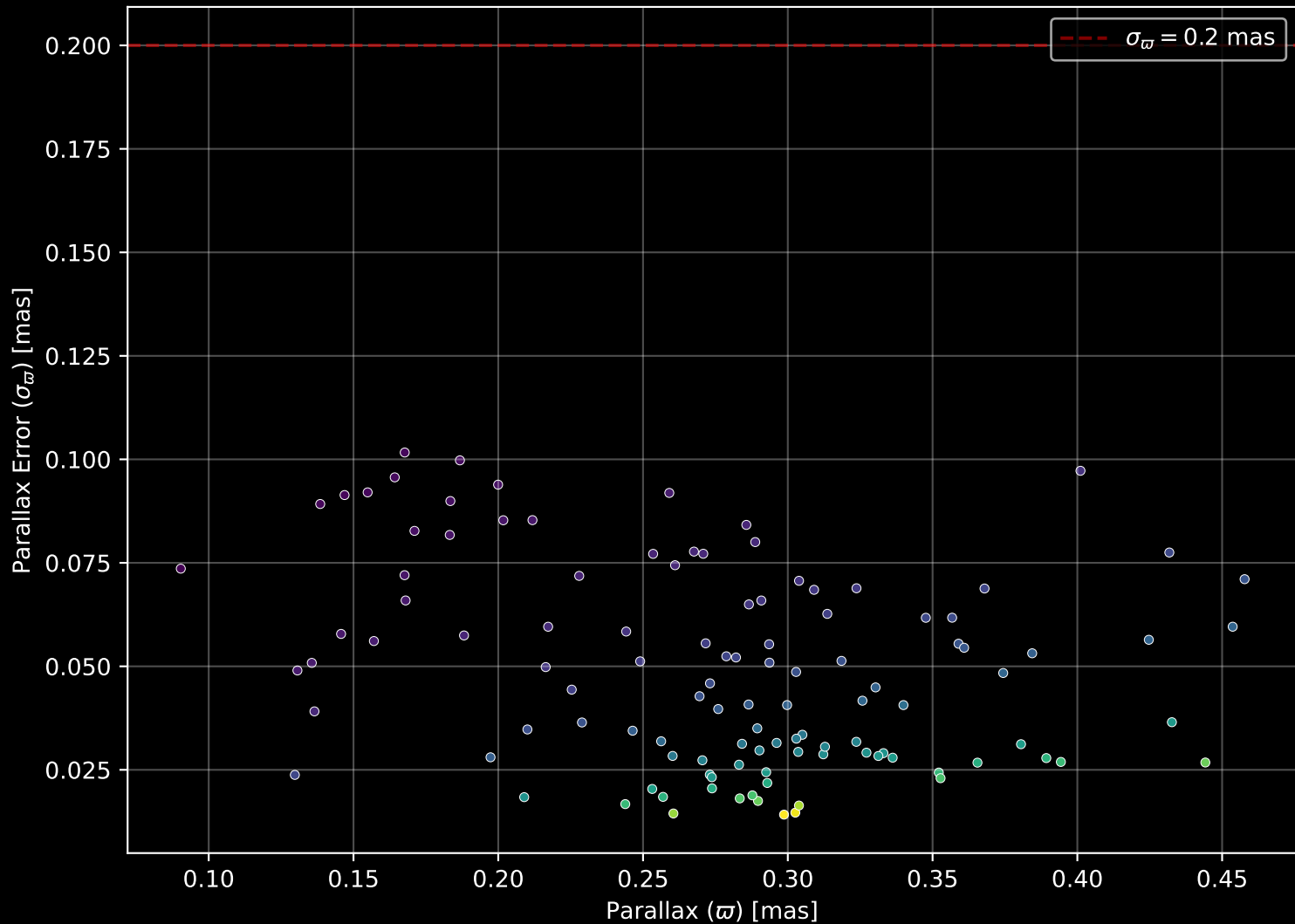
Gaia Cluster: [Haffner_21] Parallax Quality (n= 114)
