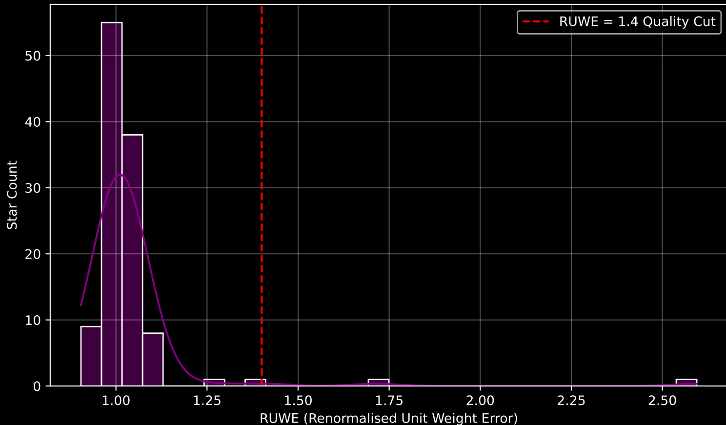
Gaia Cluster: [Haffner_21] RUWE Distribution (n= 114)
