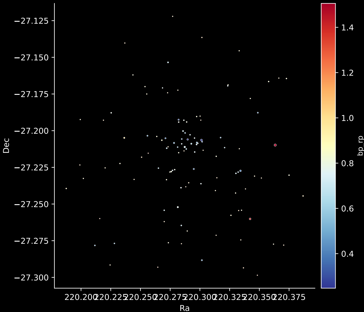
Gaia Cluster: [Haffner_21] Stars: 114
