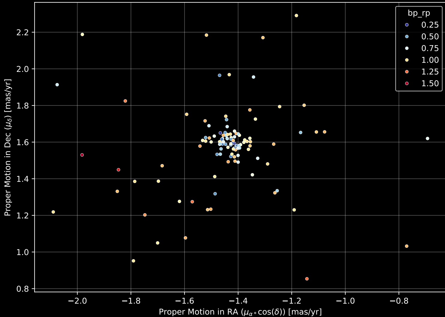
Gaia Cluster: [Haffner_21] Proper Motion Diagram (n= 114)
