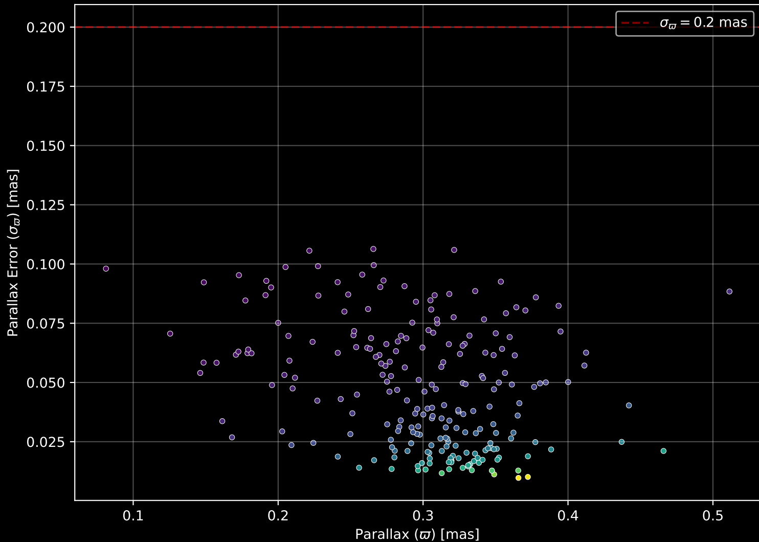
Gaia Cluster: [Haffner_26] Parallax Quality (n= 228)
