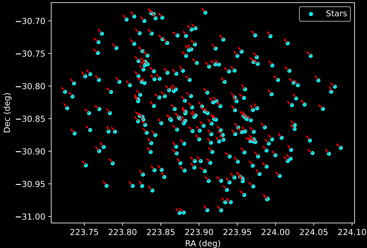
Gaia Cluster: [Haffner_26] Proper Motion Vectors for Gaia Star Field (n= 228)
