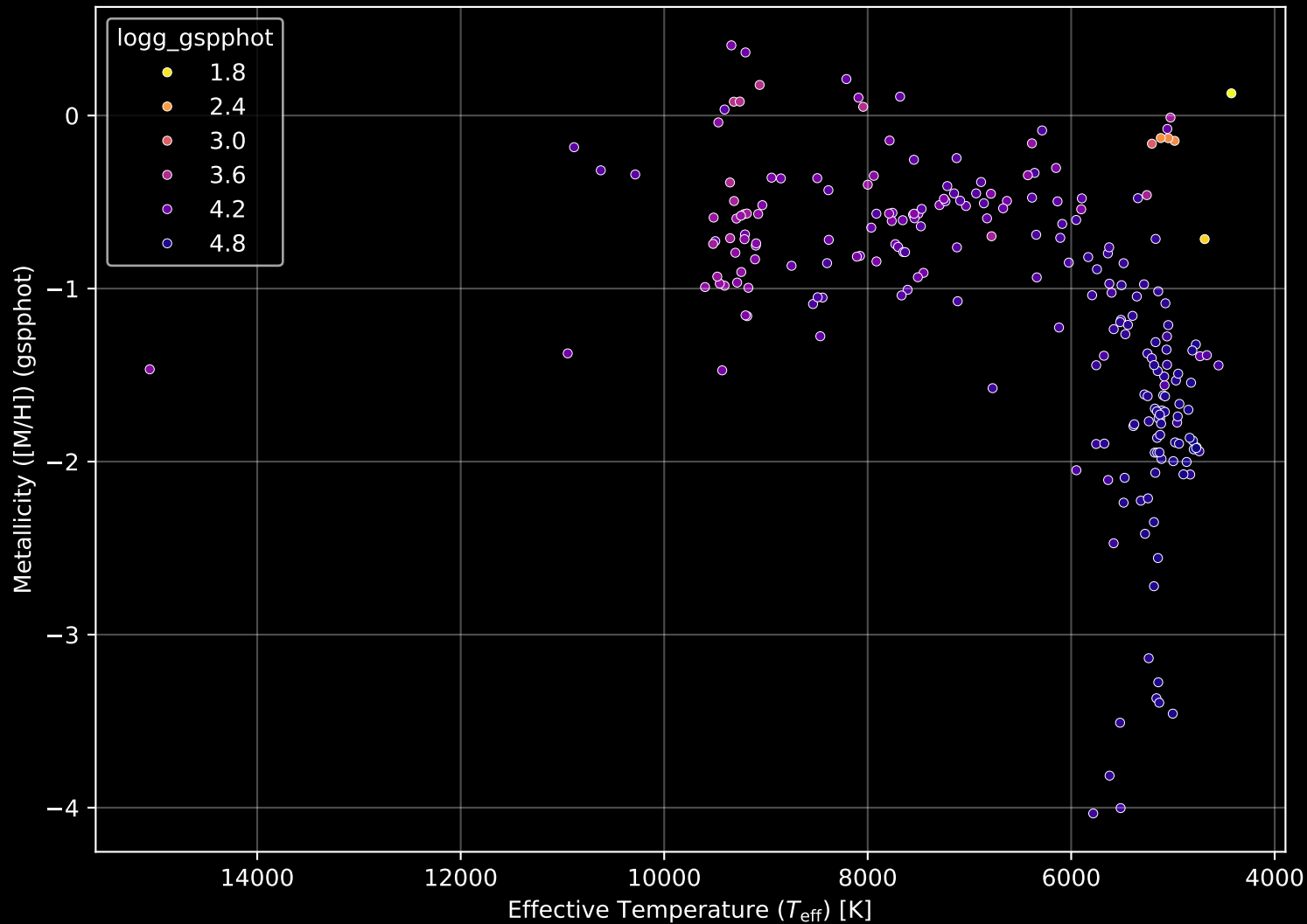
Gaia Cluster: [Haffner_26] Stellar Population Parameters (n= 228)
