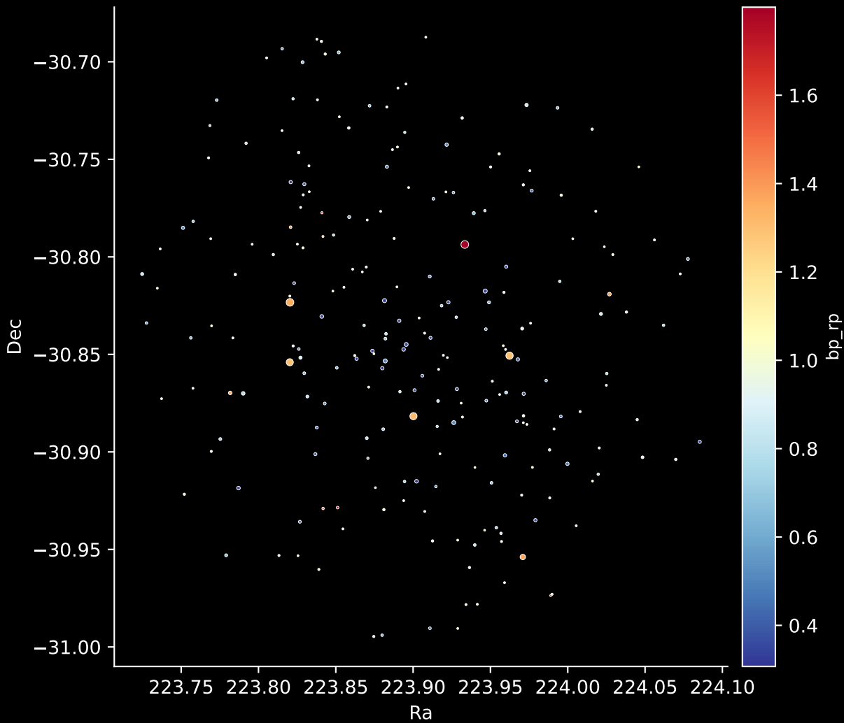
Gaia Cluster: [Haffner_26] Stars: 228
