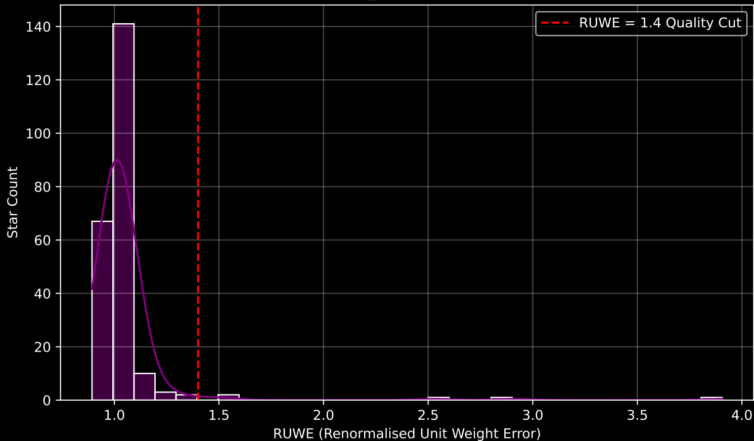
Gaia Cluster: [Haffner_26] RUWE Distribution (n= 228)
