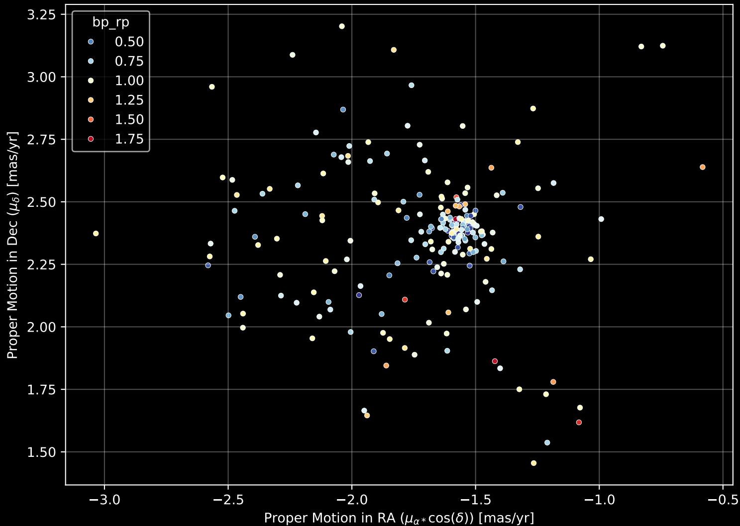
Gaia Cluster: [Haffner_26] Proper Motion Diagram (n= 228)
