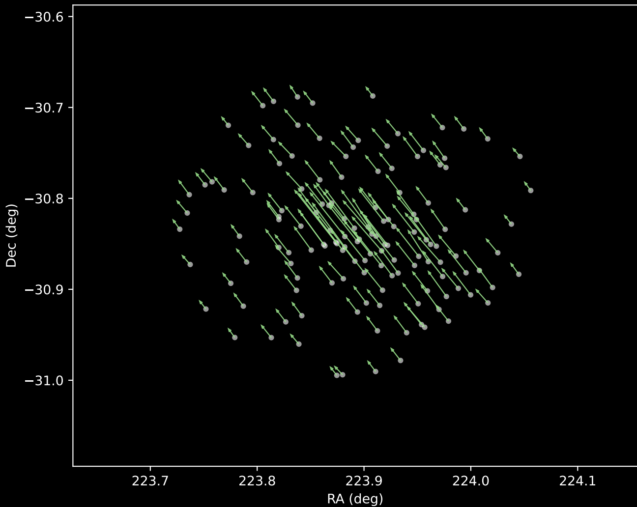
Gaia DR3 Cluster 5 Proper Motion Vectors (n=138)
