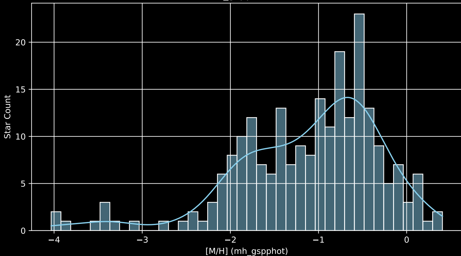
Gaia Cluster: [Haffner_26 [M/H] (mh_gspphot) (n= 228)
