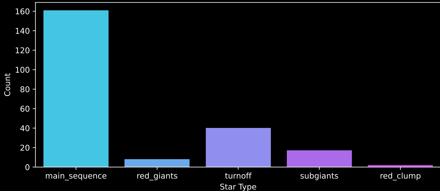
Gaia Cluster: [Haffner_26] Count plot of Star Type
