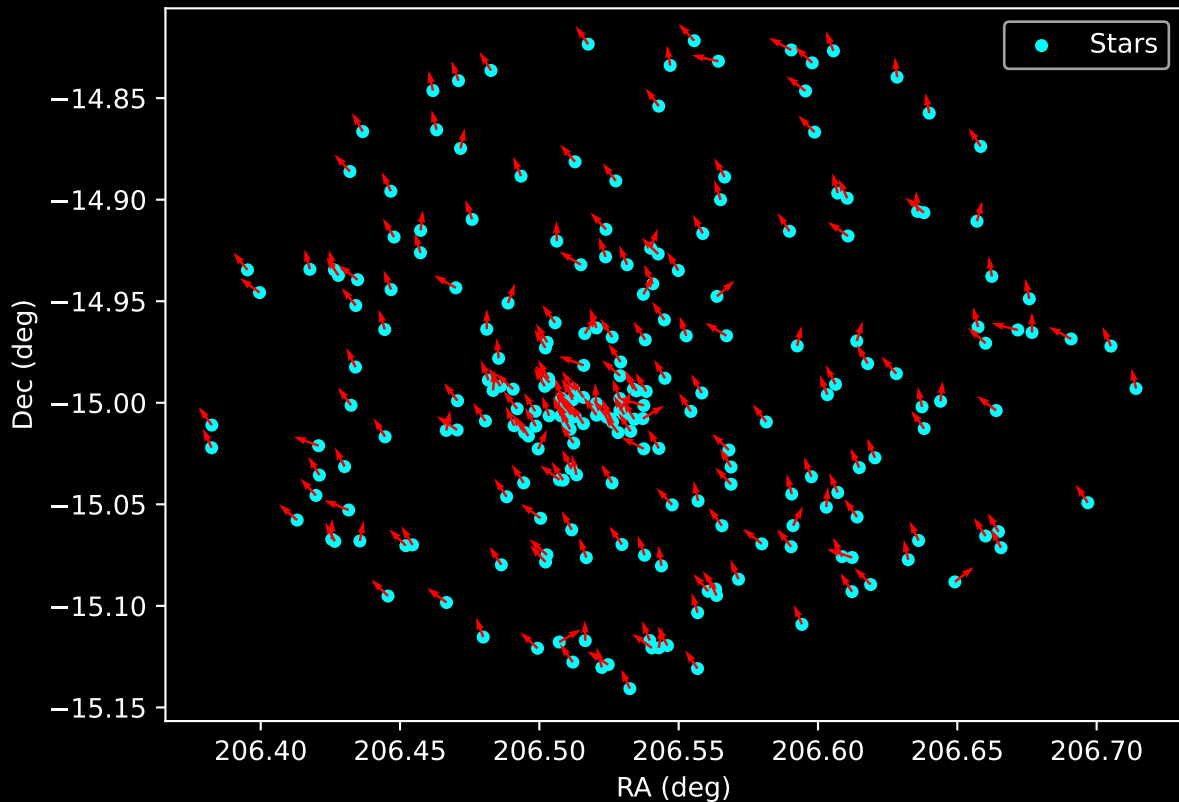
Gaia Cluster: [Haffner_4] Proper Motion Vectors for Gaia Star Field (n= 230)
