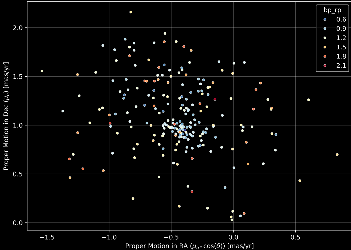
Gaia Cluster: [Haffner_4] Proper Motion Diagram (n= 230)
