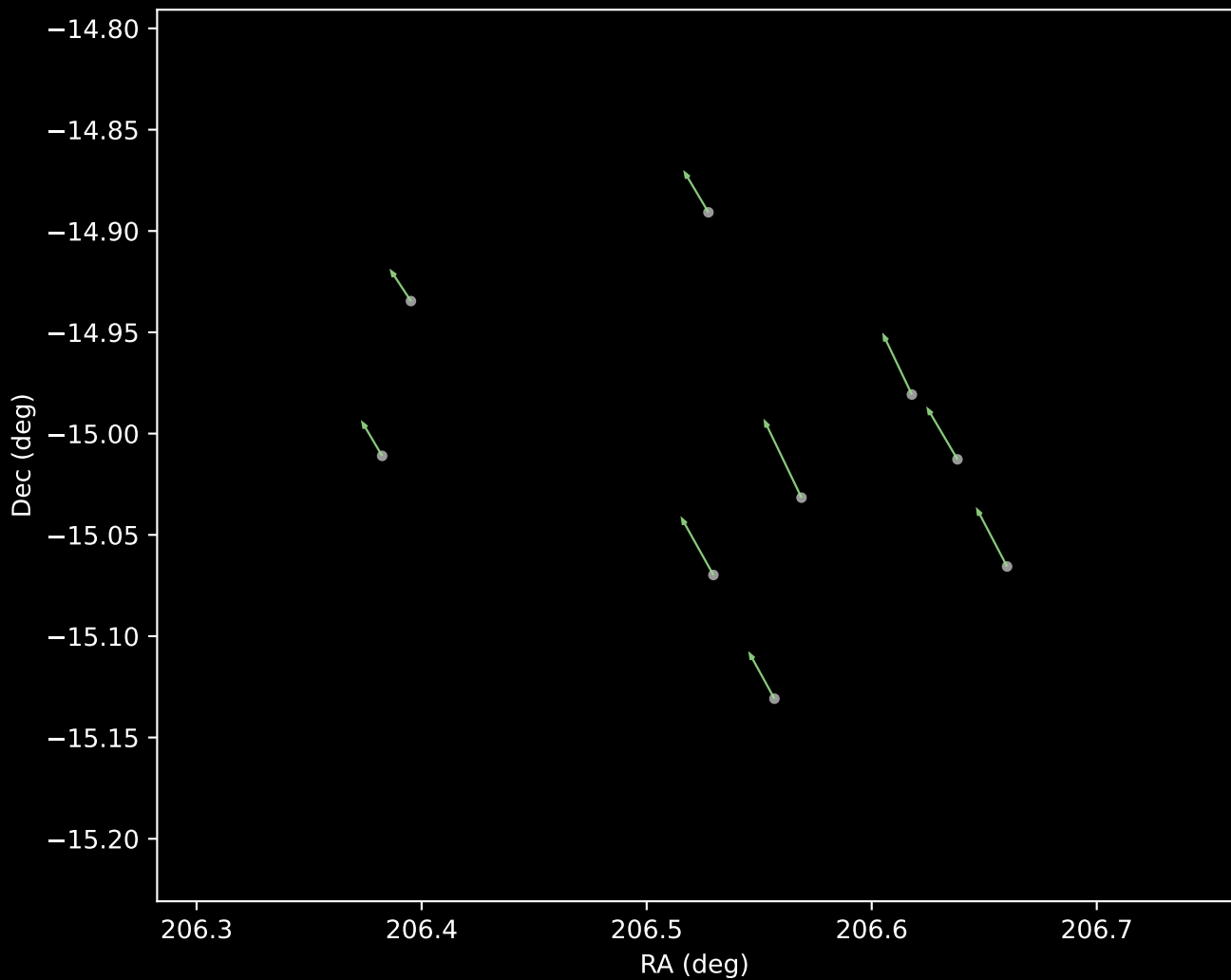
Gaia DR3 Cluster 5 Proper Motion Vectors (n=9)
