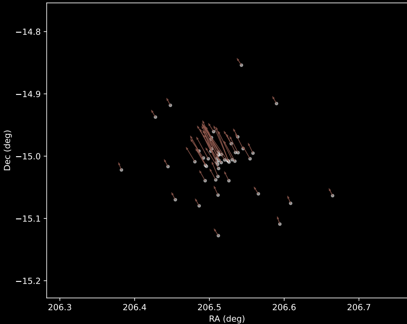
Gaia DR3 Cluster 10 Proper Motion Vectors (n=52)
