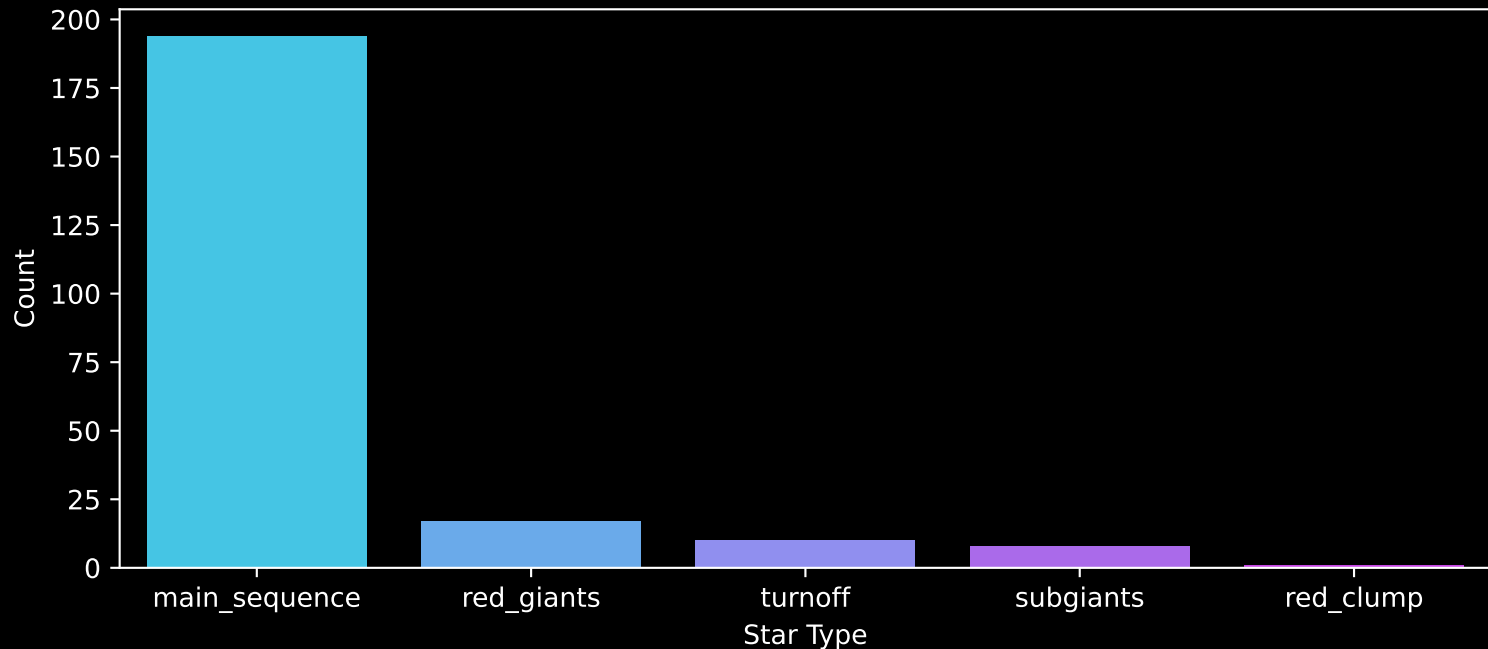
Gaia Cluster: [Haffner_4] Count plot of Star Type
