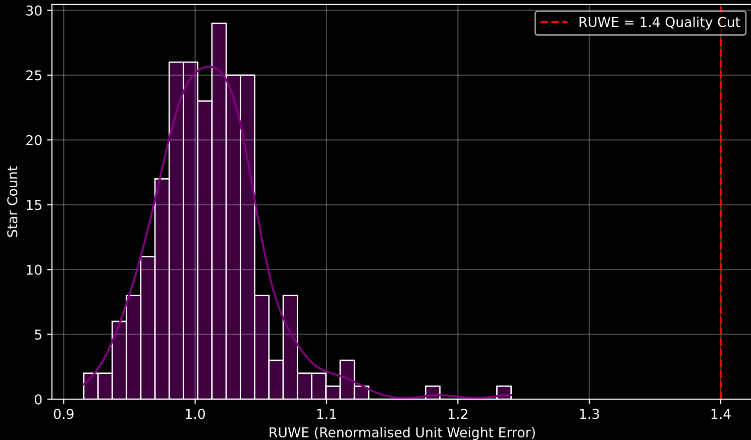
Gaia Cluster: [Haffner_4] RUWE Distribution (n= 230)
