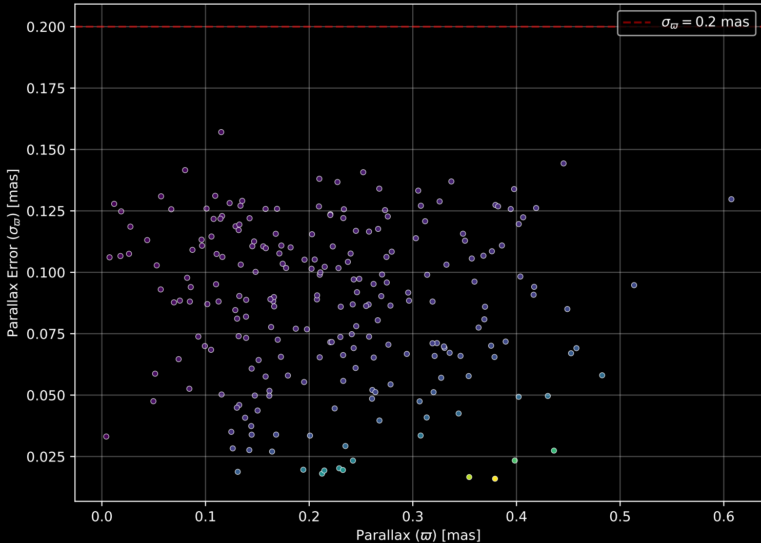
Gaia Cluster: [Haffner_4] Parallax Quality (n= 230)
