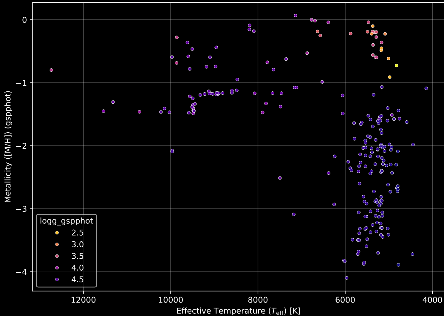
Gaia Cluster: [Haffner_4] Stellar Population Parameters (n= 230)
