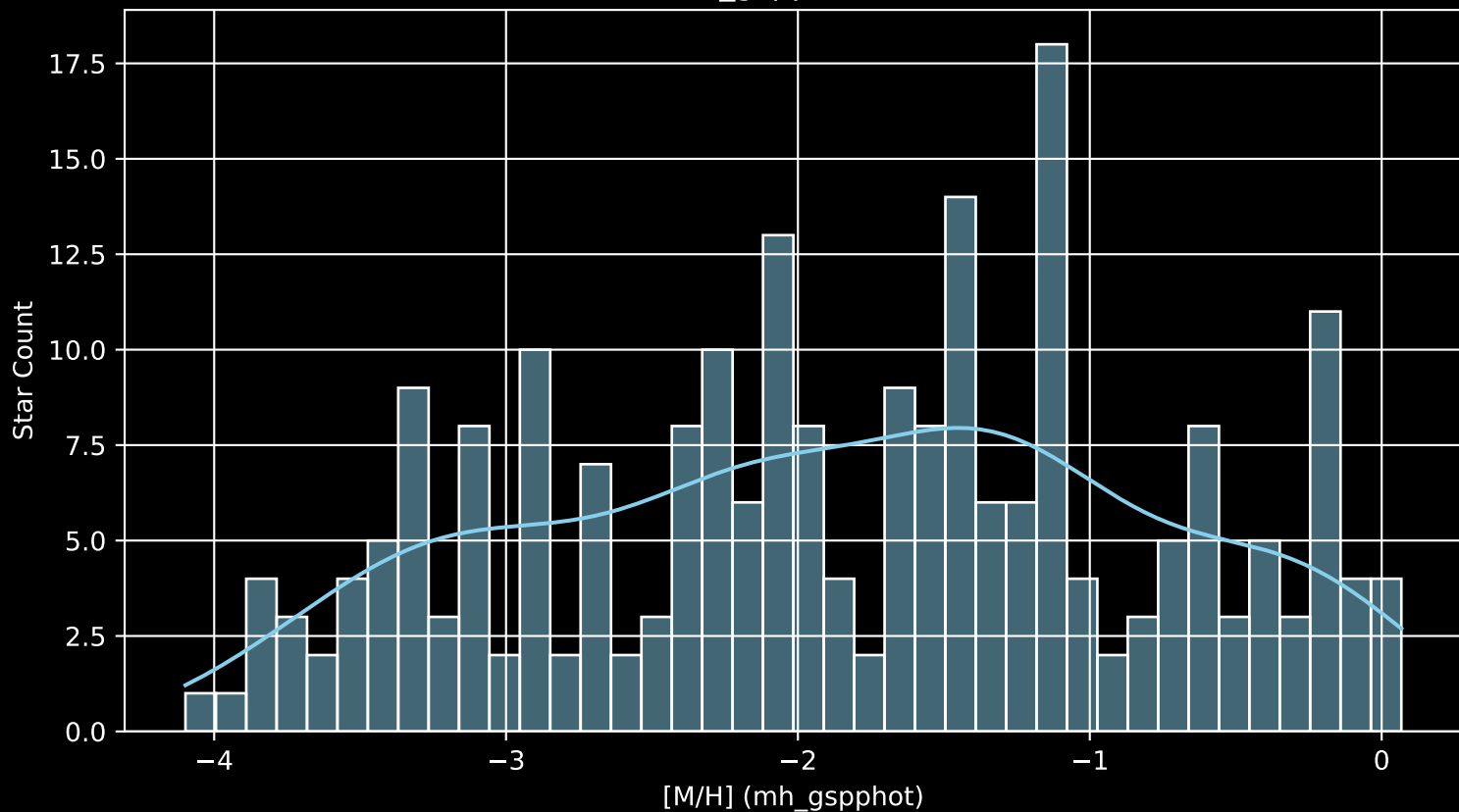
Gaia Cluster: [Haffner_4 [M/H] (mh_gspphot) (n= 230)
