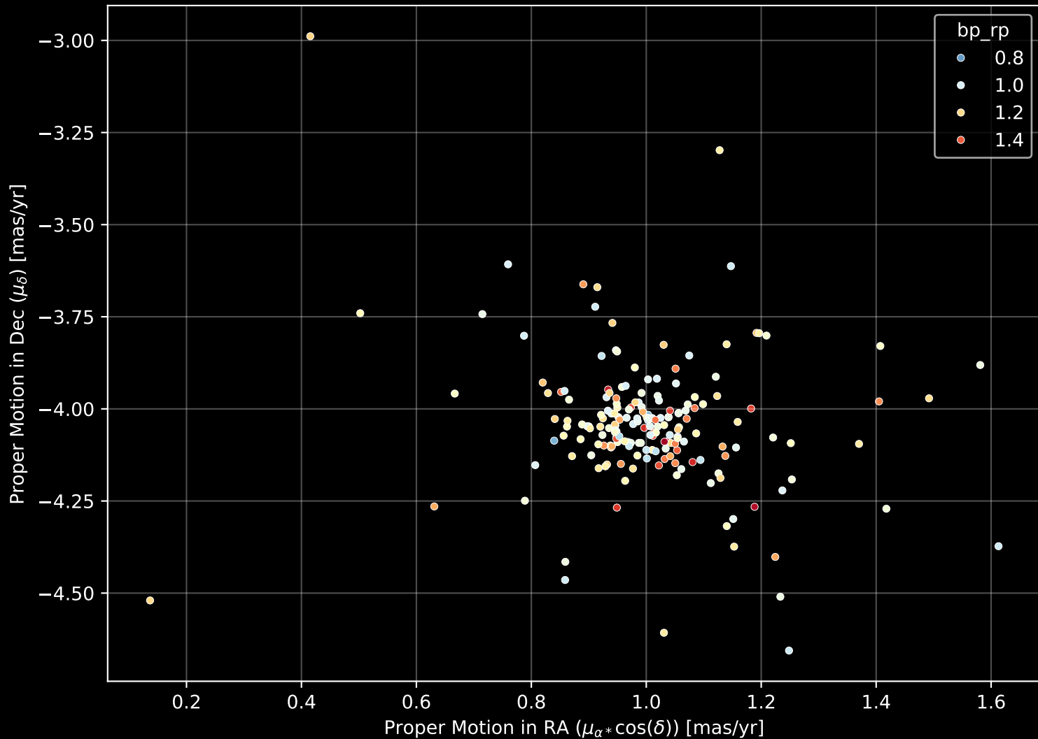
Gaia Cluster: [Haffner_5] Proper Motion Diagram (n= 192)
