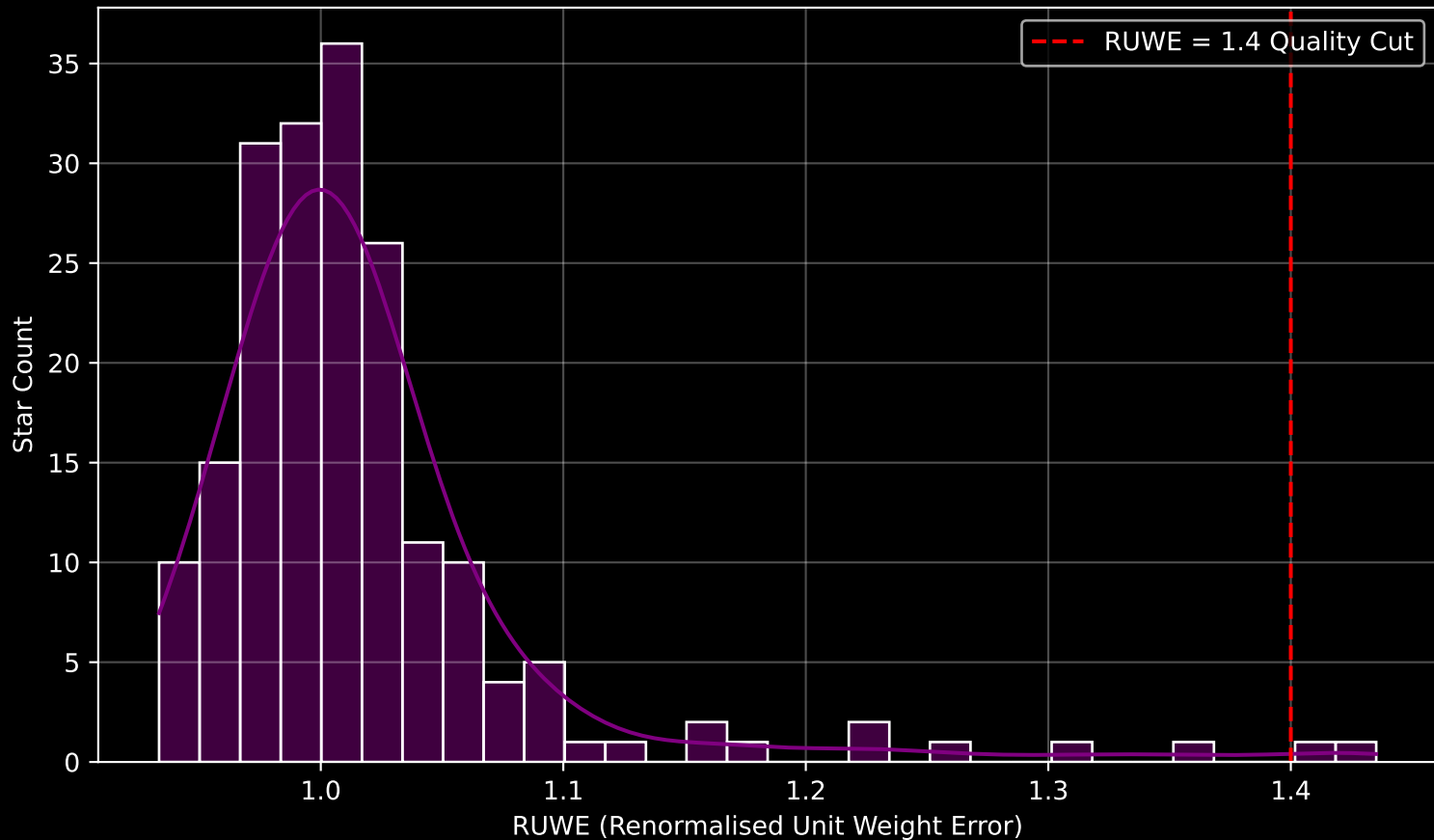
Gaia Cluster: [Haffner_5] RUWE Distribution (n= 192)
