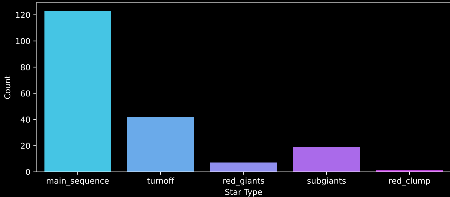
Gaia Cluster: [Haffner_5] Count plot of Star Type
