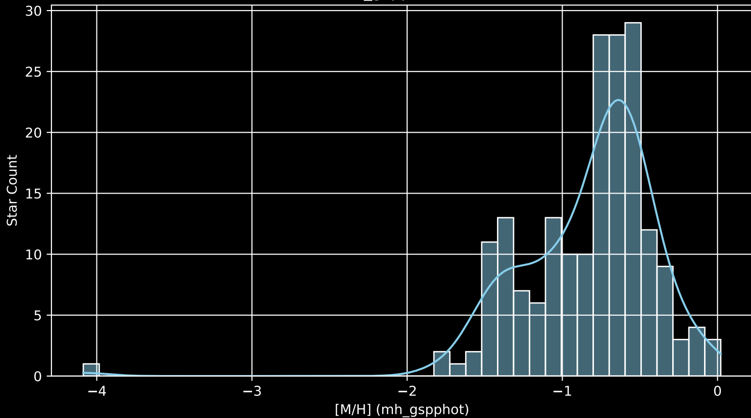
Gaia Cluster: [Haffner_5 [M/H] (mh_gspphot) (n= 192)
