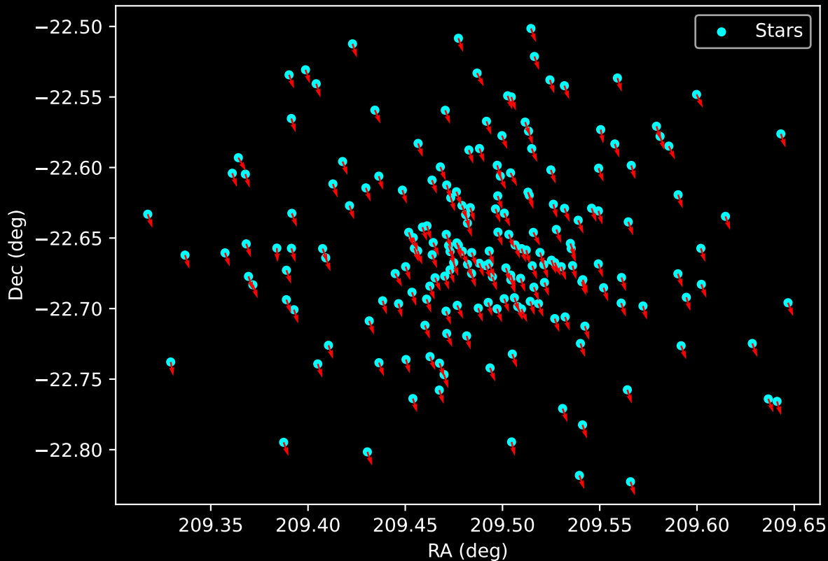
Gaia Cluster: [Haffner_5] Proper Motion Vectors for Gaia Star Field (n= 192)
