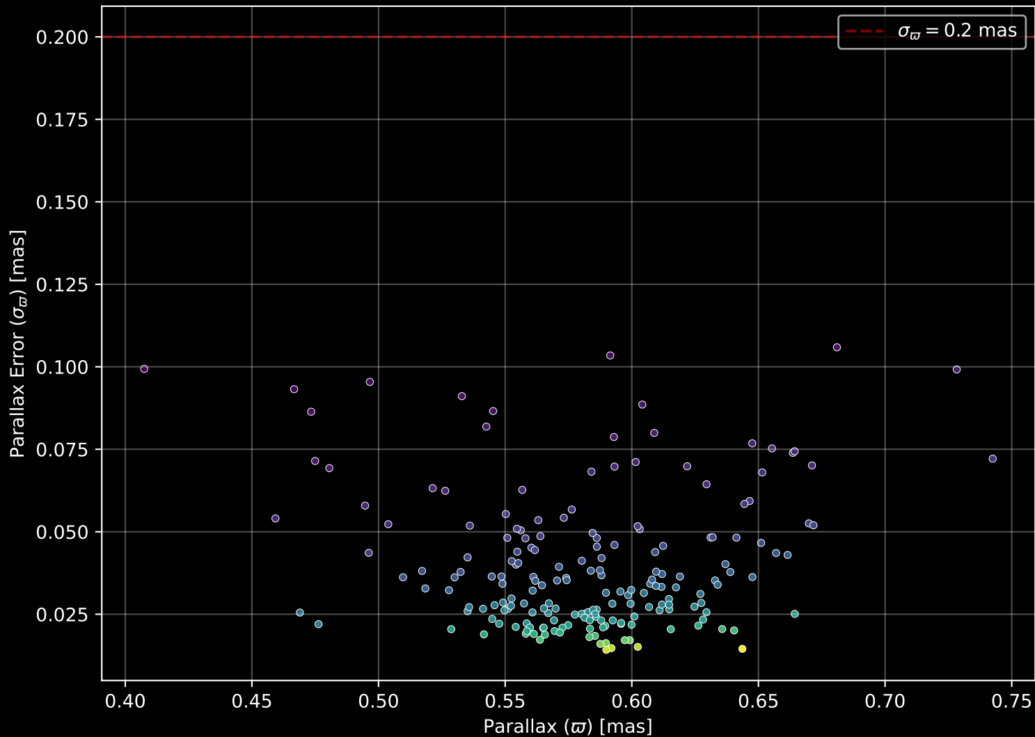
Gaia Cluster: [Haffner_5] Parallax Quality (n= 192)
