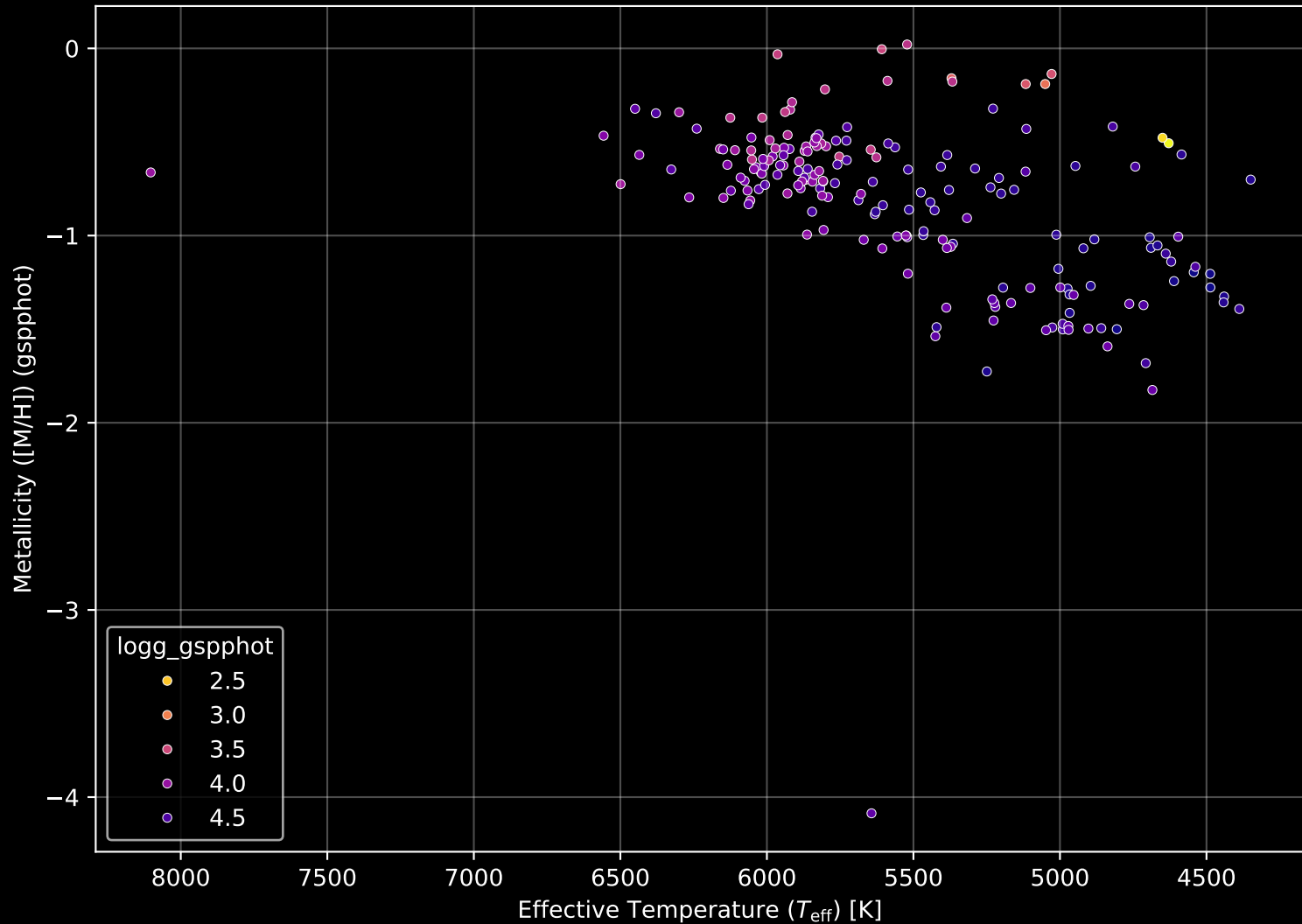
Gaia Cluster: [Haffner_5] Stellar Population Parameters (n= 192)
