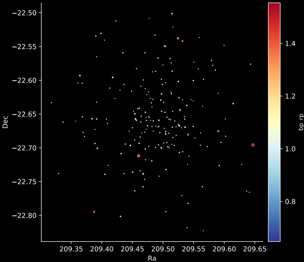
Gaia Cluster: [Haffner_5] Stars: 192
