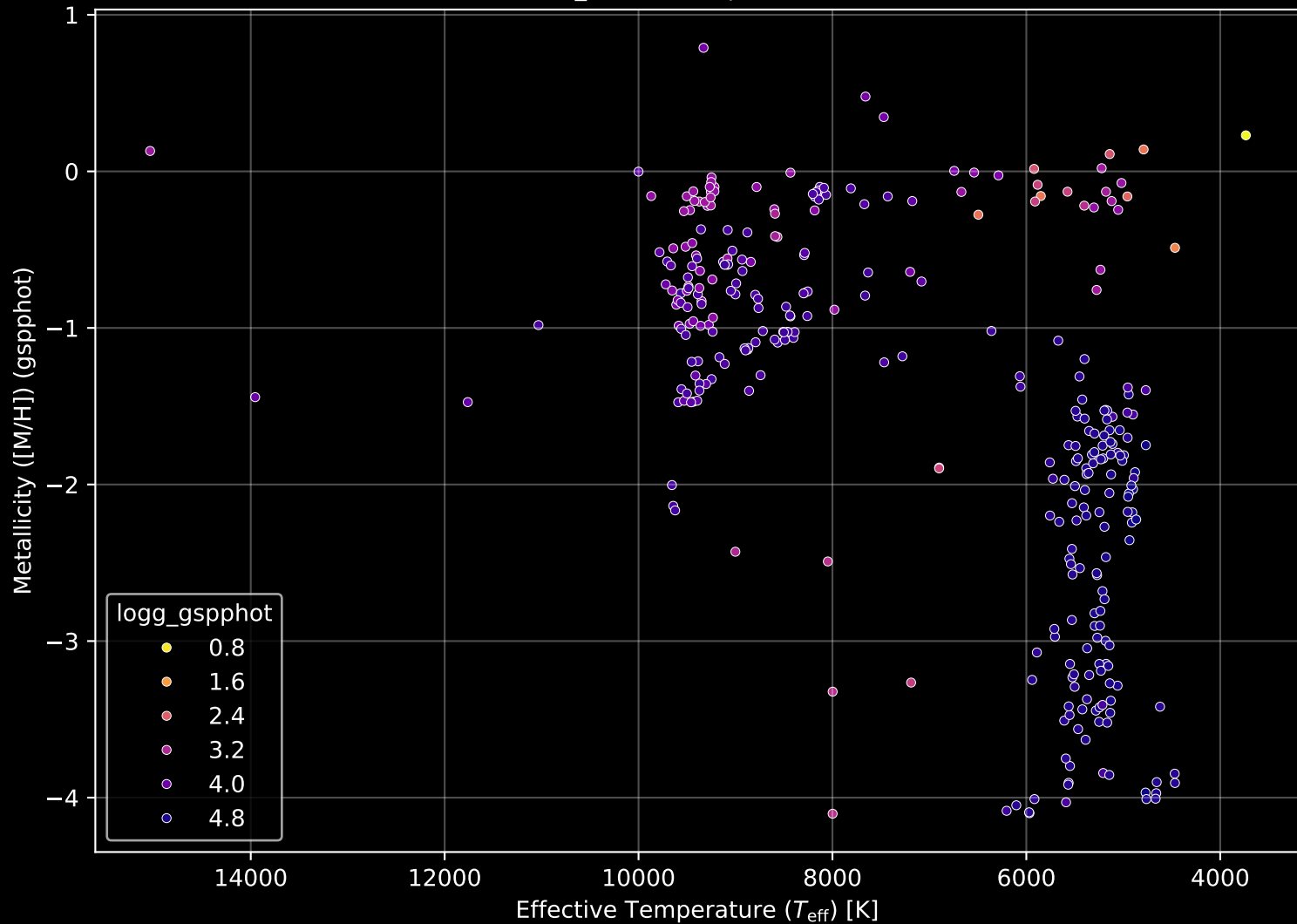
Gaia Cluster: [Haffner_6] Stellar Population Parameters (n= 322)
