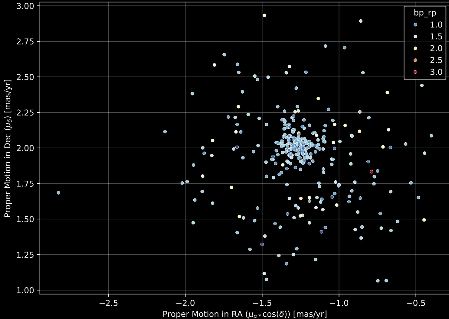
Gaia Cluster: [Haffner_6] Proper Motion Diagram (n= 322)
