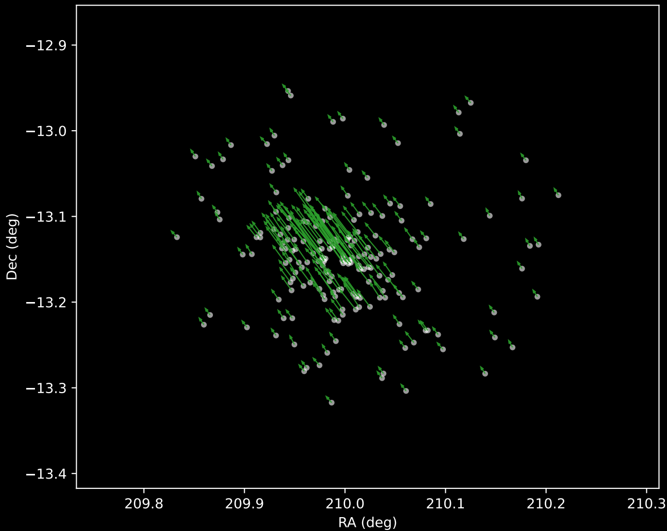
Gaia DR3 Cluster 4 Proper Motion Vectors (n=190)
