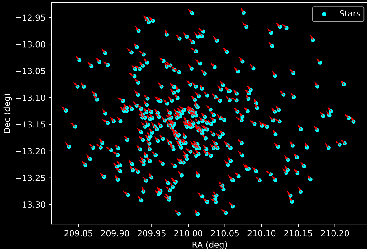
Gaia Cluster: [Haffner_6] Proper Motion Vectors for Gaia Star Field (n= 322)
