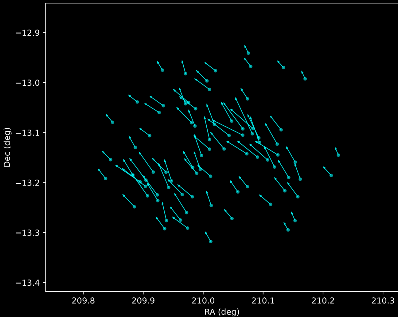
Gaia DR3 Noise Stream Proper Motion Vectors (n=81)
