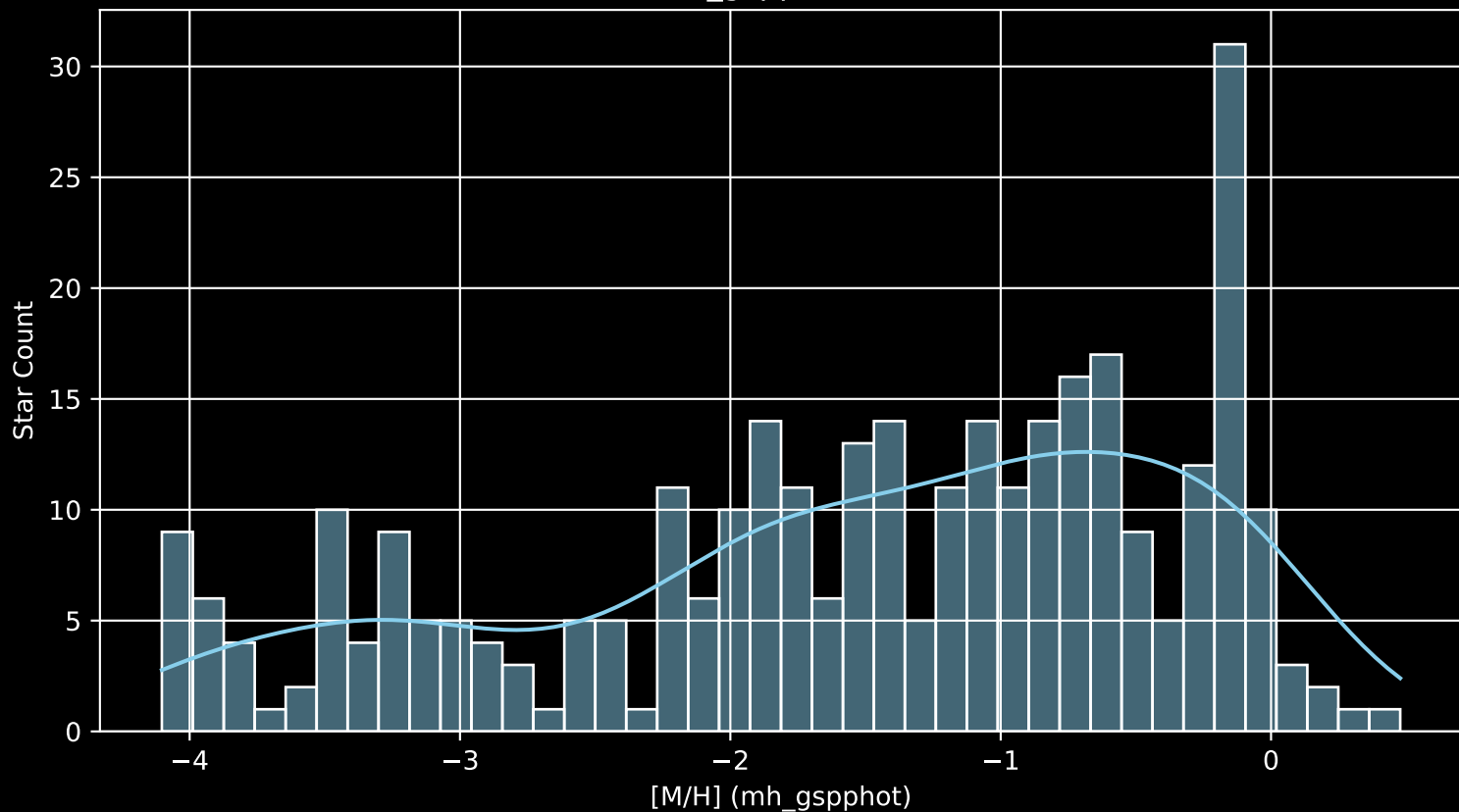
Gaia Cluster: [Haffner_6 [M/H] (mh_gspphot) (n= 321)
