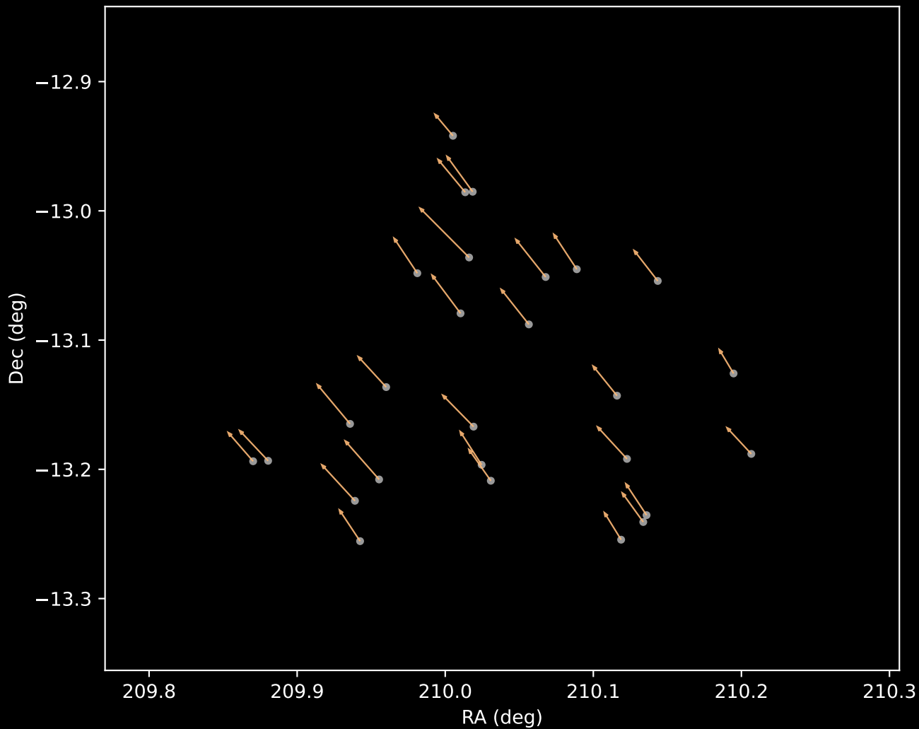
Gaia DR3 Cluster 3 Proper Motion Vectors (n=27)
