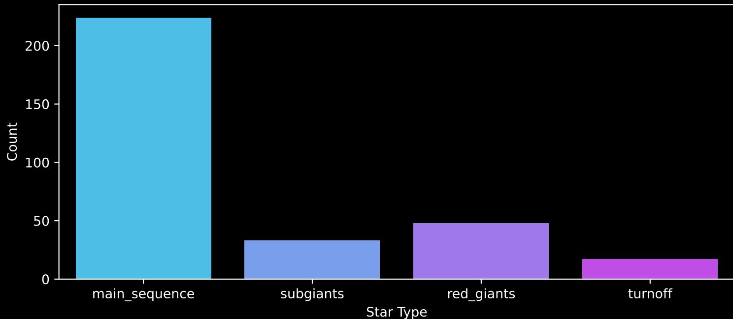
Gaia Cluster: [Haffner_6] Count plot of Star Type
