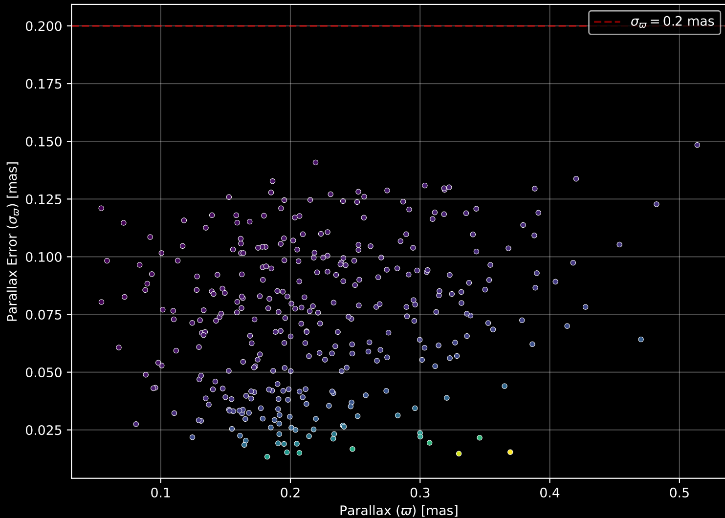
Gaia Cluster: [Haffner_6] Parallax Quality (n= 322)
