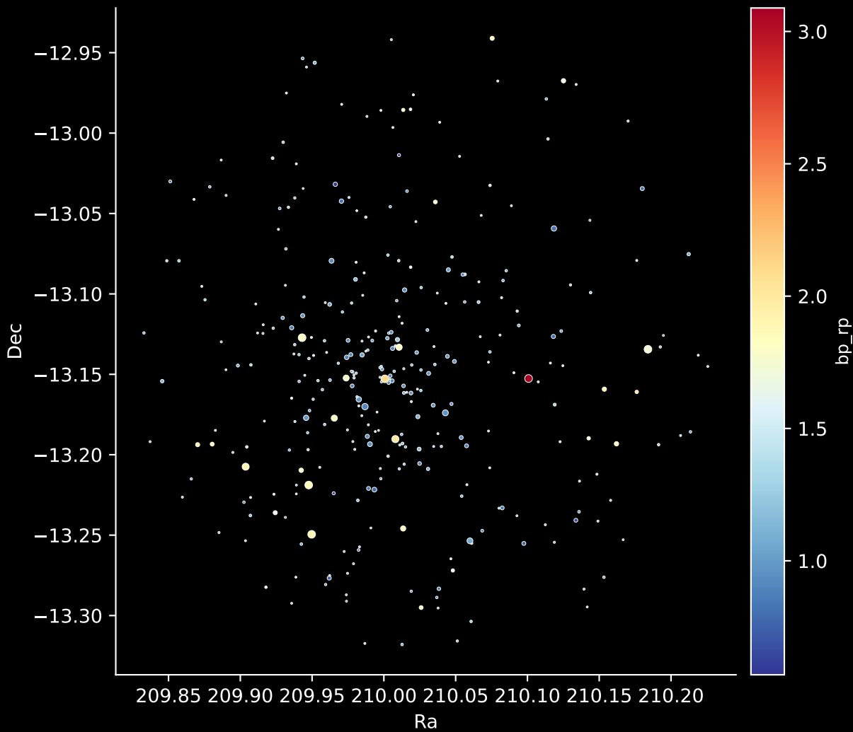
Gaia Cluster: [Haffner_6] Stars: 322
