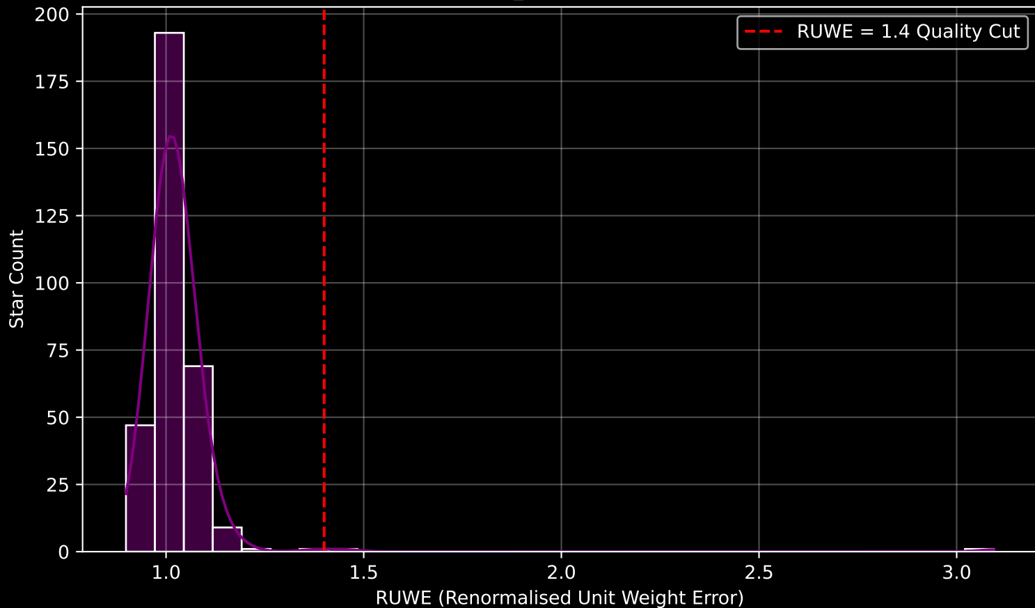
Gaia Cluster: [Haffner_6] RUWE Distribution (n= 322)
