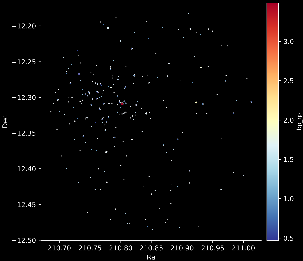
Gaia Cluster: [Haffner_8] Stars: 222
