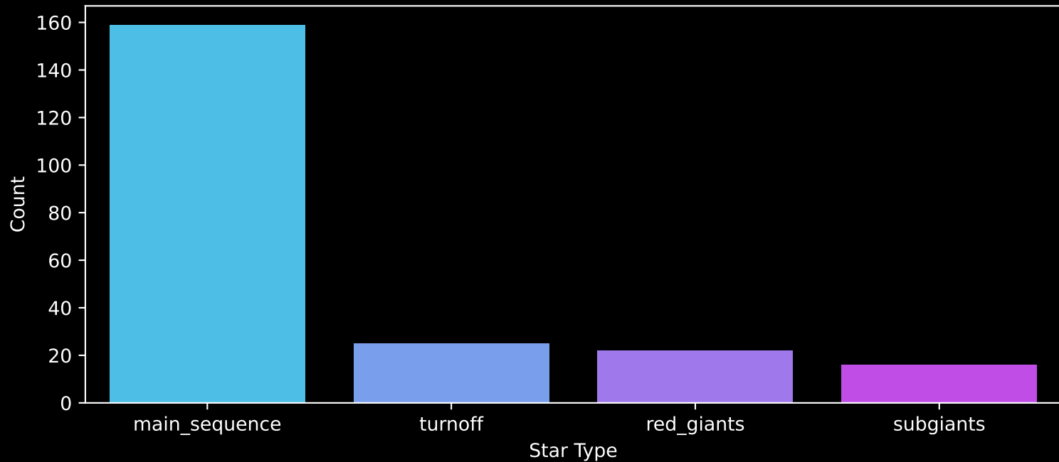
Gaia Cluster: [Haffner_8] Count plot of Star Type
