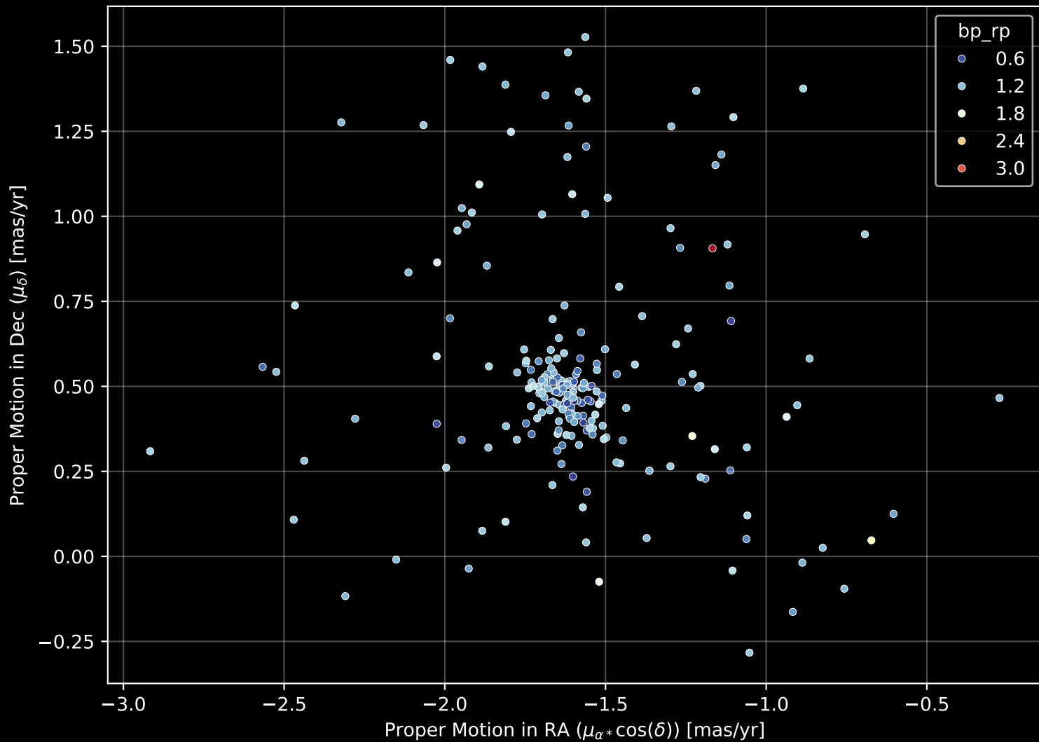
Gaia Cluster: [Haffner_8] Proper Motion Diagram (n= 222)
