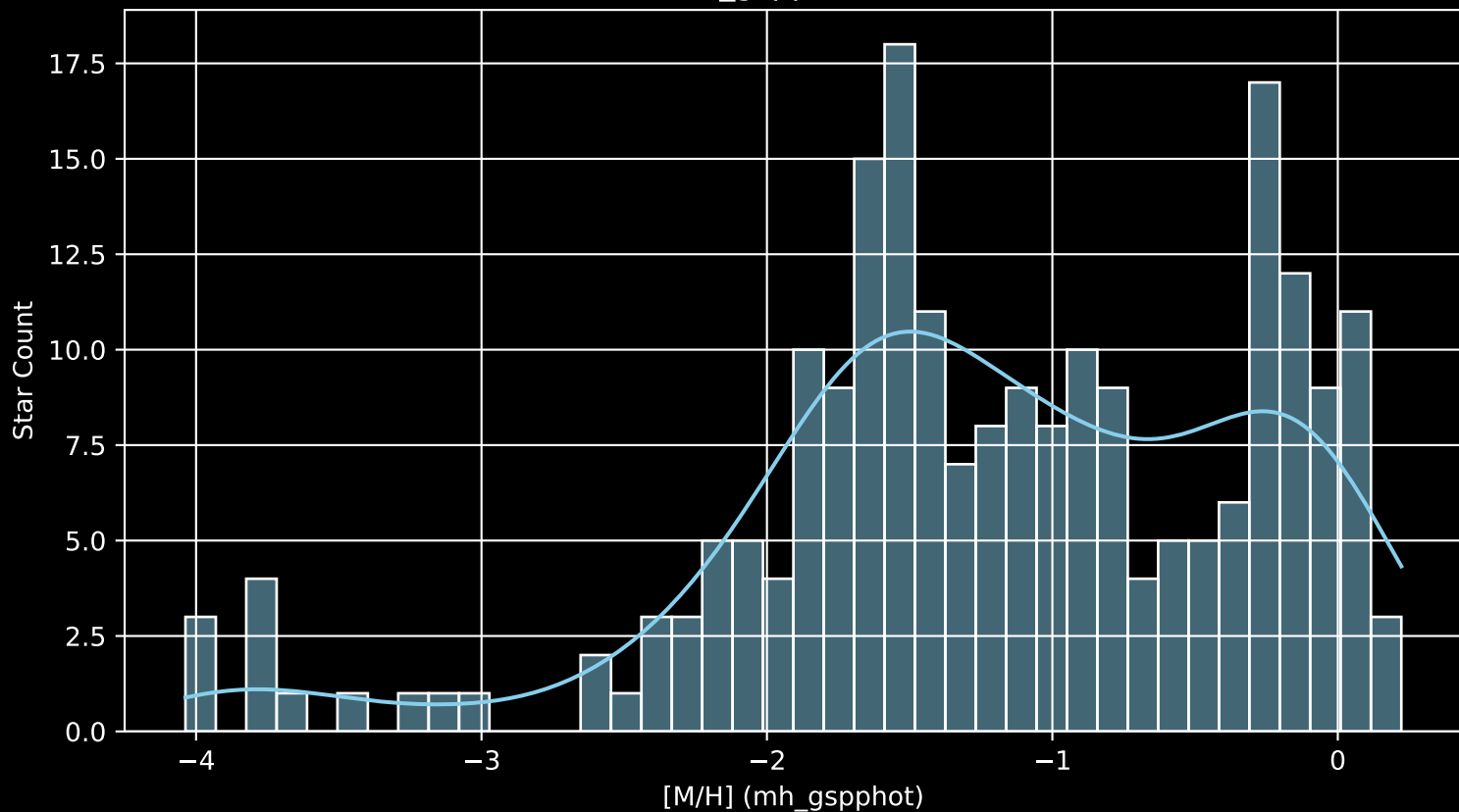
Gaia Cluster: [Haffner_8 [M/H] (mh_gspphot) (n= 221)
