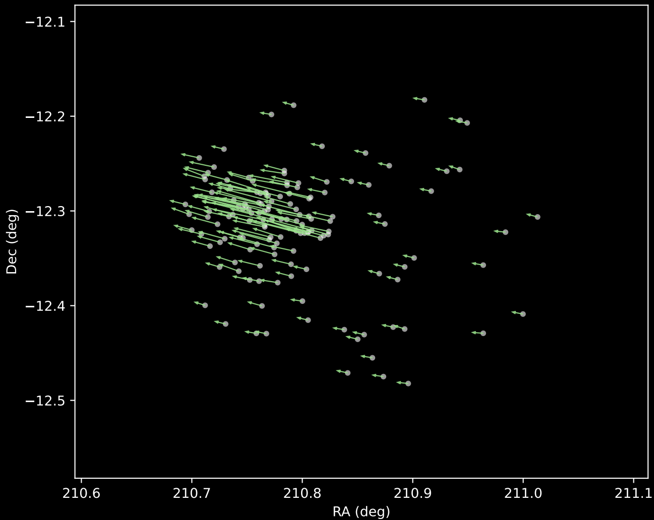
Gaia DR3 Cluster 5 Proper Motion Vectors (n=141)
