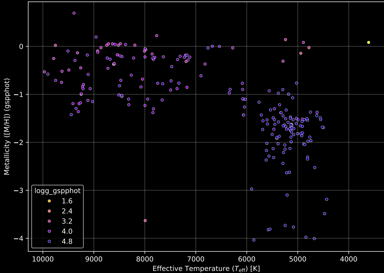
Gaia Cluster: [Haffner_8] Stellar Population Parameters (n= 222)
