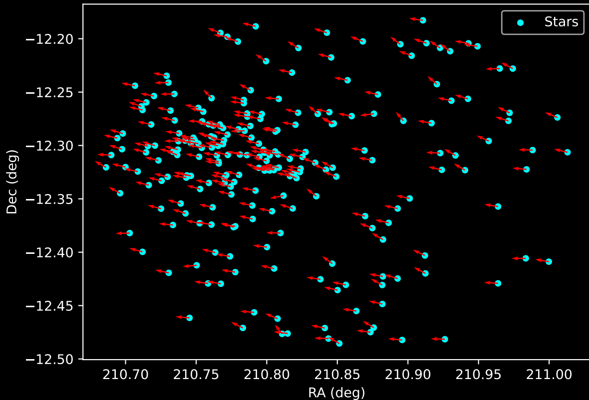
Gaia Cluster: [Haffner_8] Proper Motion Vectors for Gaia Star Field (n= 222)
