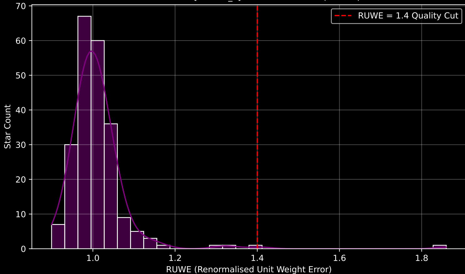
Gaia Cluster: [Haffner_8] RUWE Distribution (n= 222)
