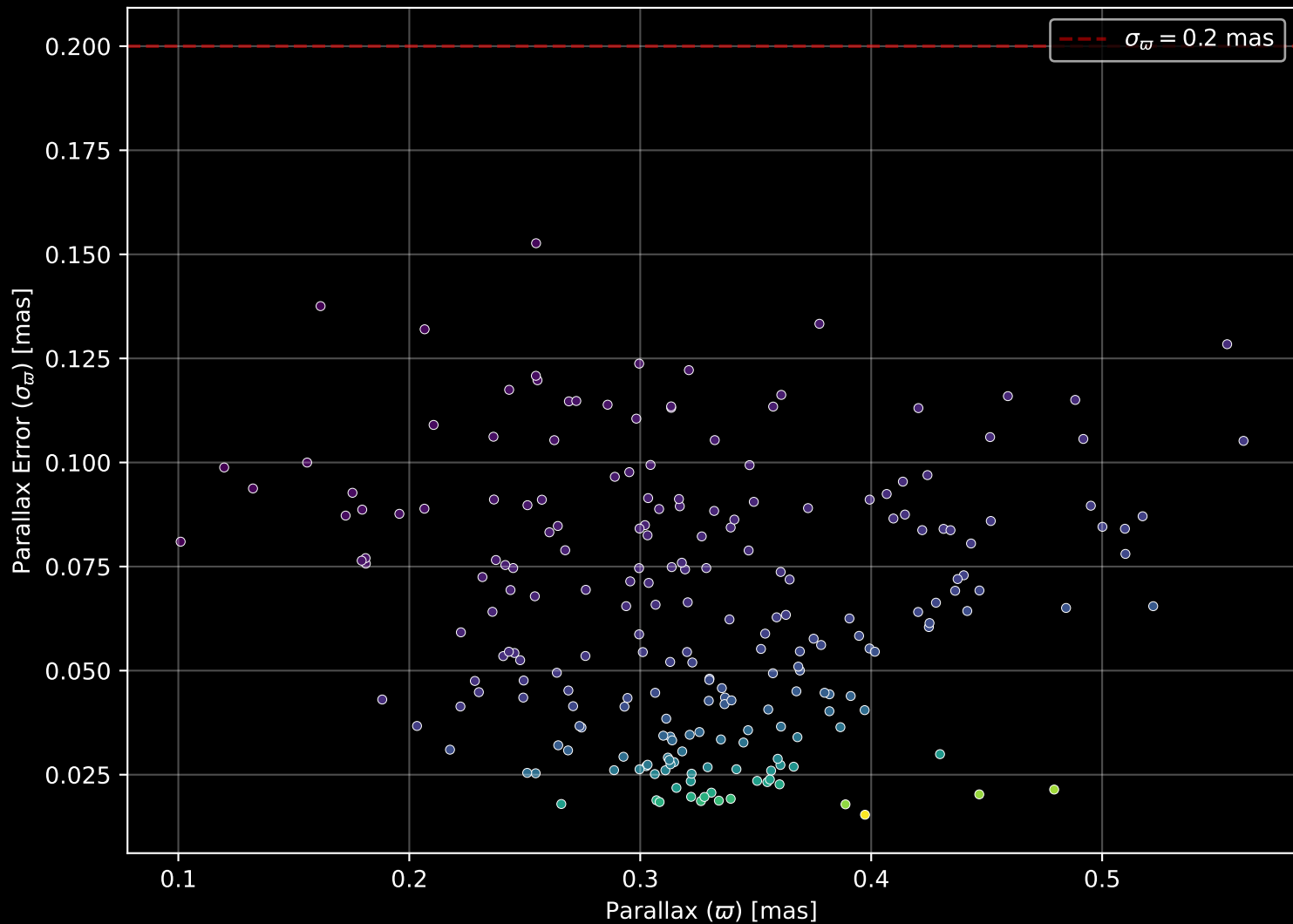
Gaia Cluster: [Haffner_8] Parallax Quality (n= 222)
