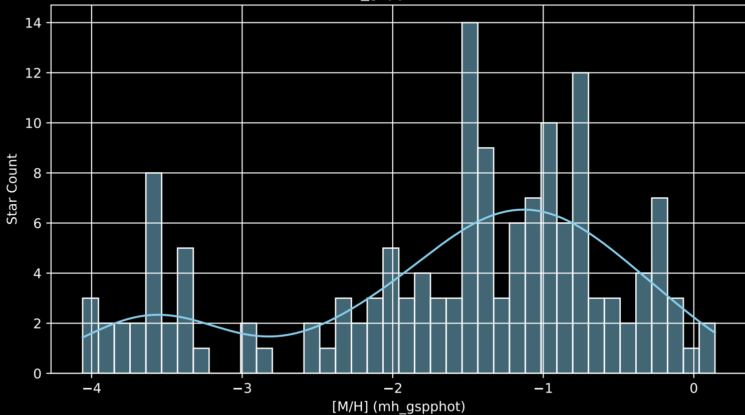
Gaia Cluster: [Haffner_9 [M/H] (mh_gspphot) (n= 149)
