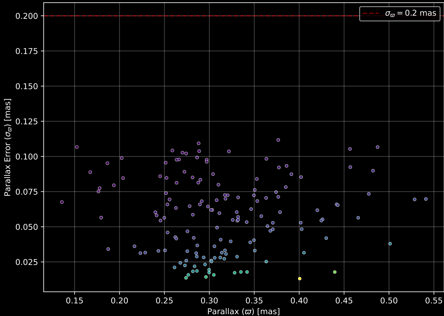
Gaia Cluster: [Haffner_9] Parallax Quality (n= 149)
