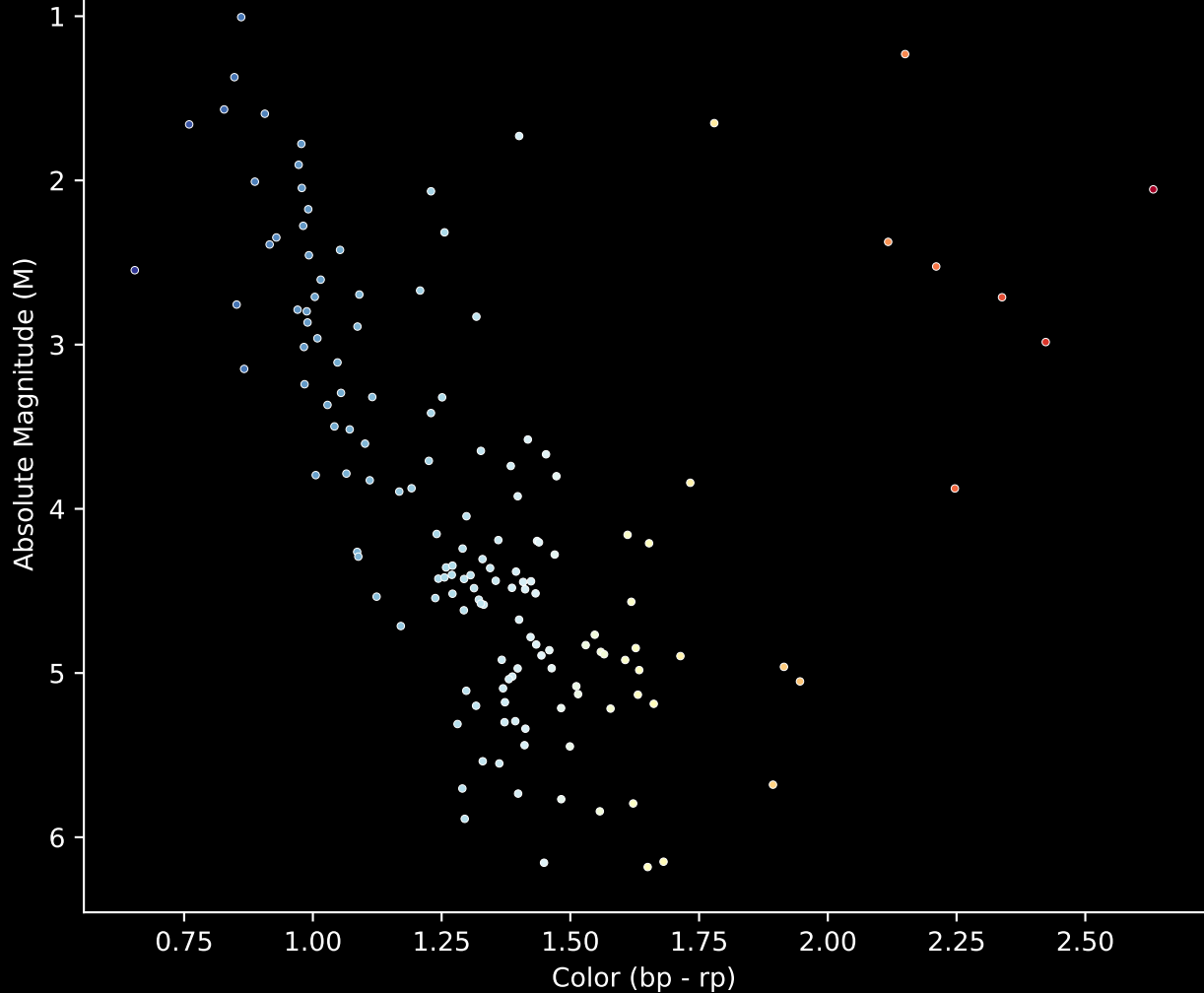
Gaia Cluster: [Haffner_9] Stars (n= 149) Hertzsprung-Russel Diagram
