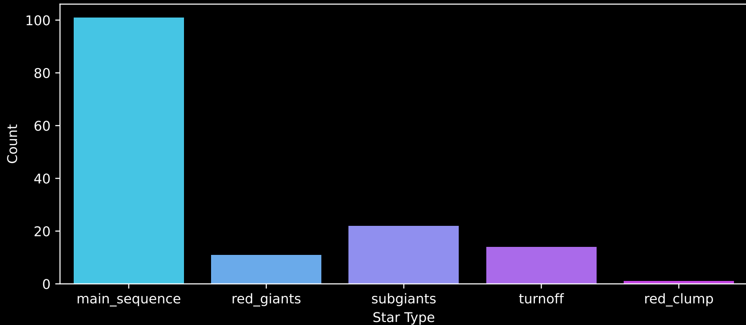
Gaia Cluster: [Haffner_9] Count plot of Star Type
