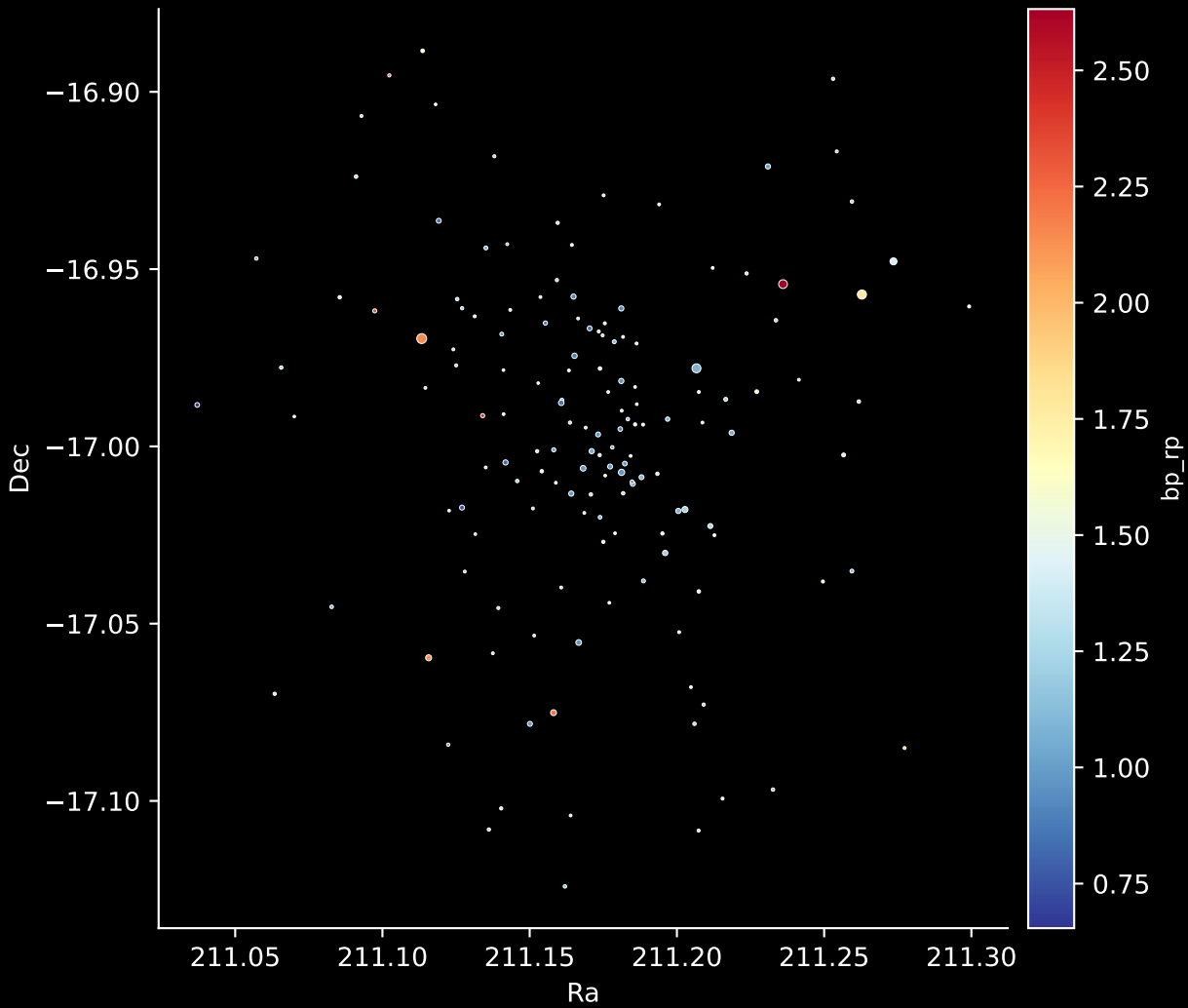
Gaia Cluster: [Haffner_9] Stars: 149
