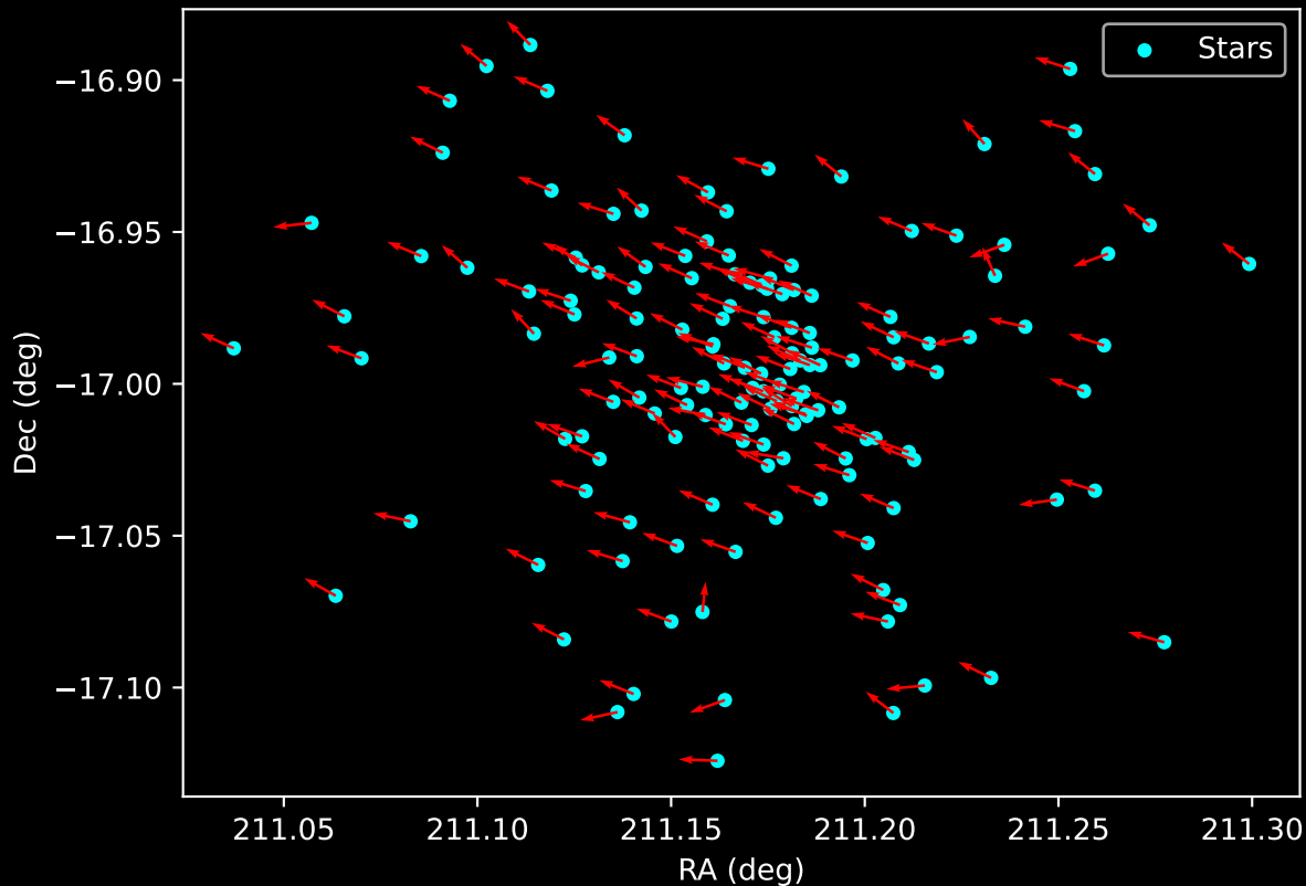
Gaia Cluster: [Haffner_9] Proper Motion Vectors for Gaia Star Field (n= 149)
