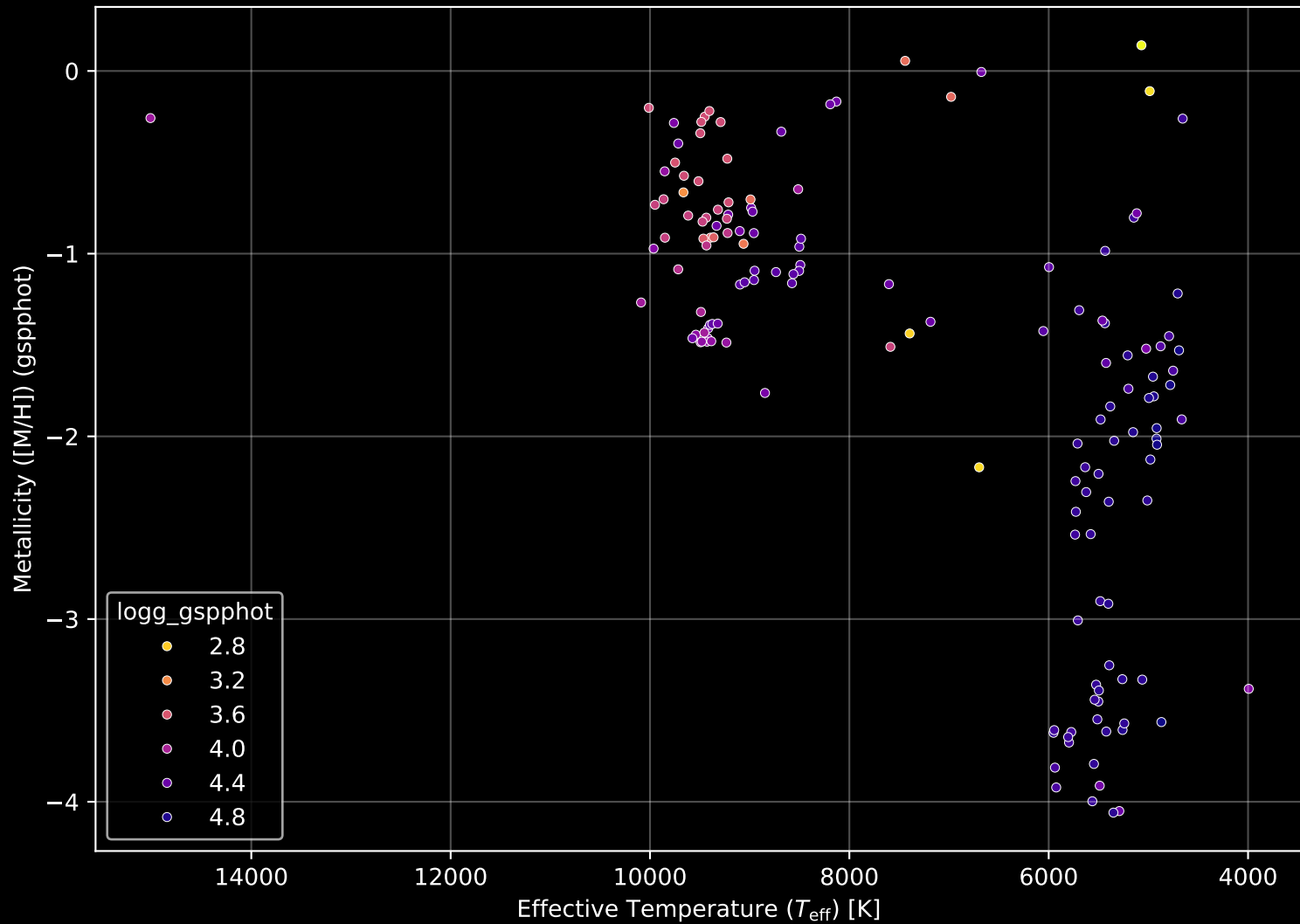
Gaia Cluster: [Haffner_9] Stellar Population Parameters (n= 149)
