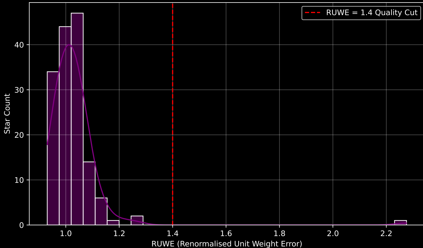
Gaia Cluster: [Haffner_9] RUWE Distribution (n= 149)
