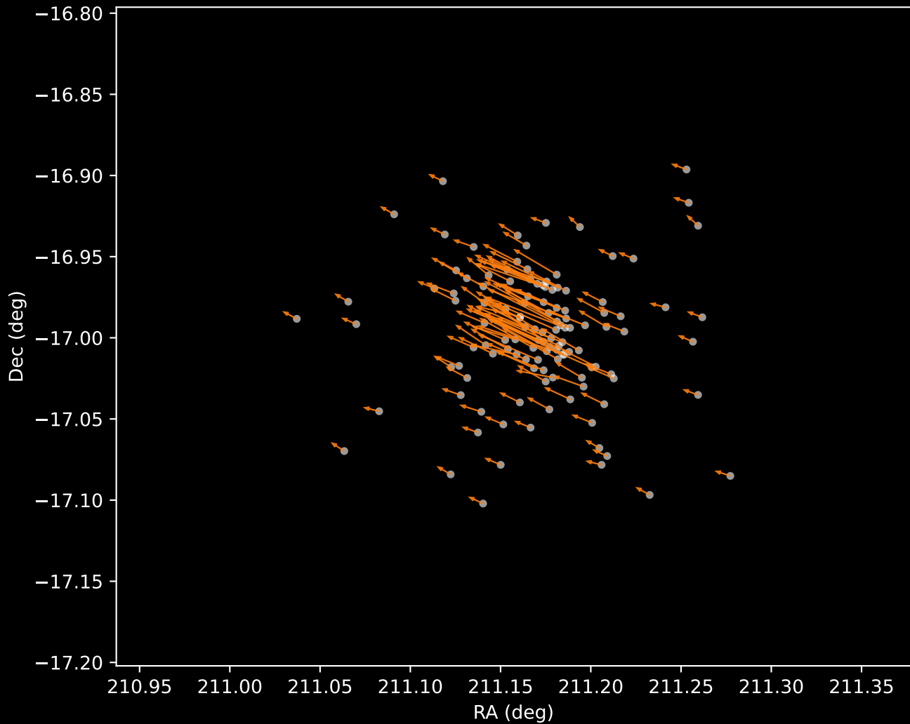
Gaia DR3 Cluster 2 Proper Motion Vectors (n=122)
