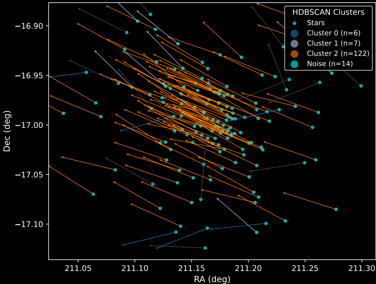
Gaia Cluster: [Haffner_9] Proper Motion Vectors with HDBSCAN (n=149)
