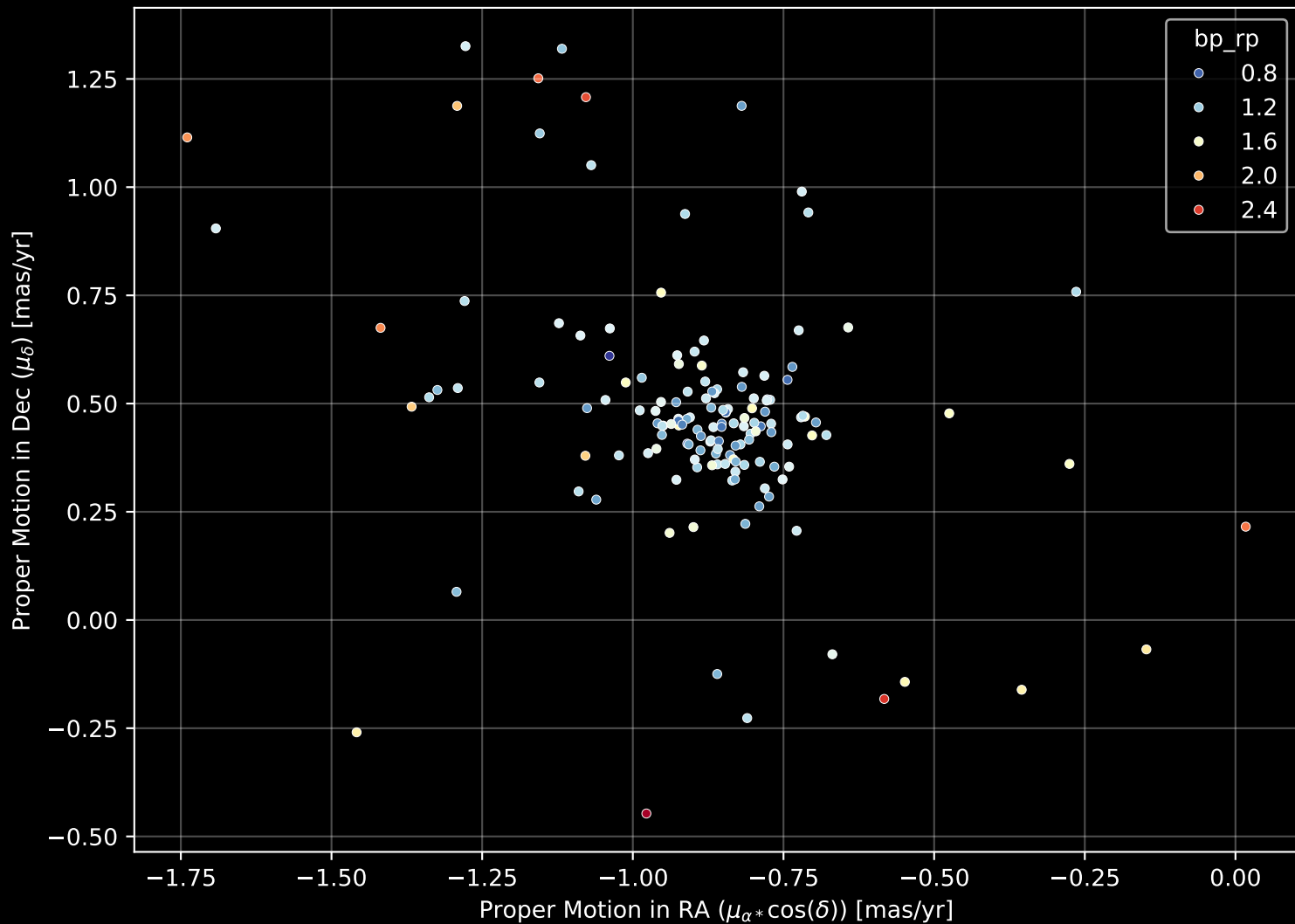
Gaia Cluster: [Haffner_9] Proper Motion Diagram (n= 149)
