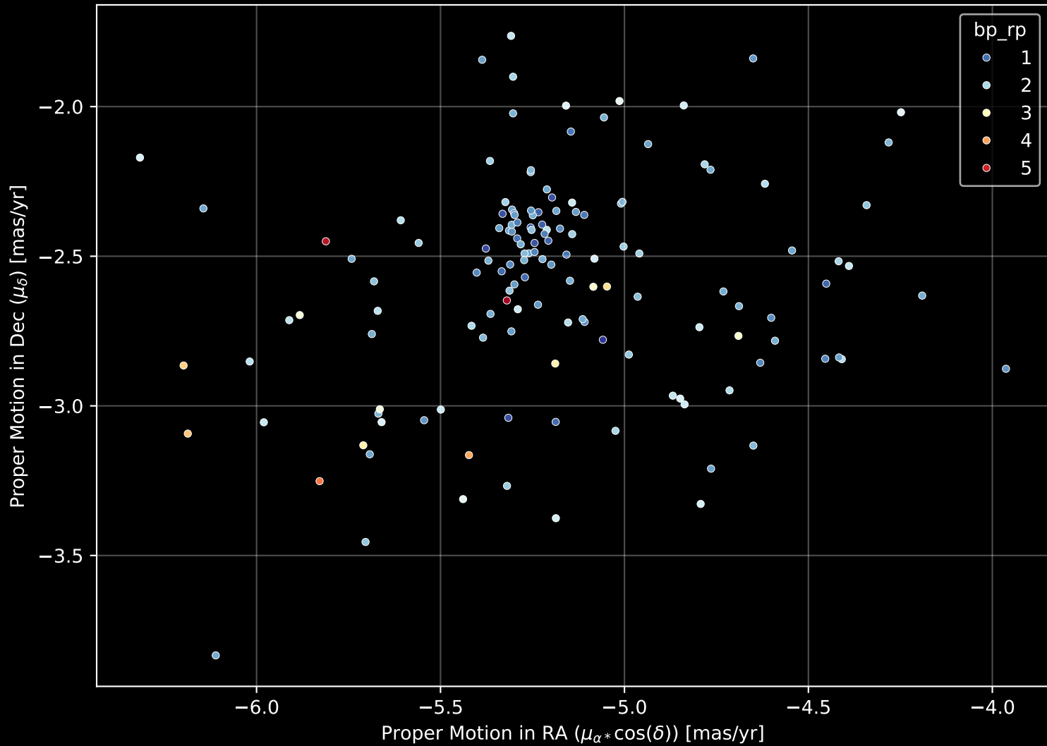
Gaia Cluster: [Hogg_17] Proper Motion Diagram (n= 142)
