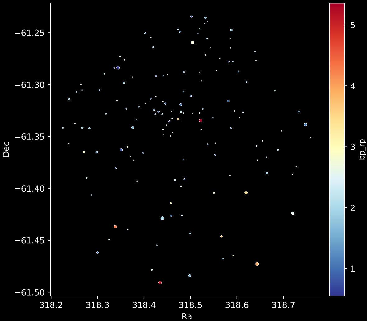
Gaia Cluster: [Hogg_17] Stars: 142
