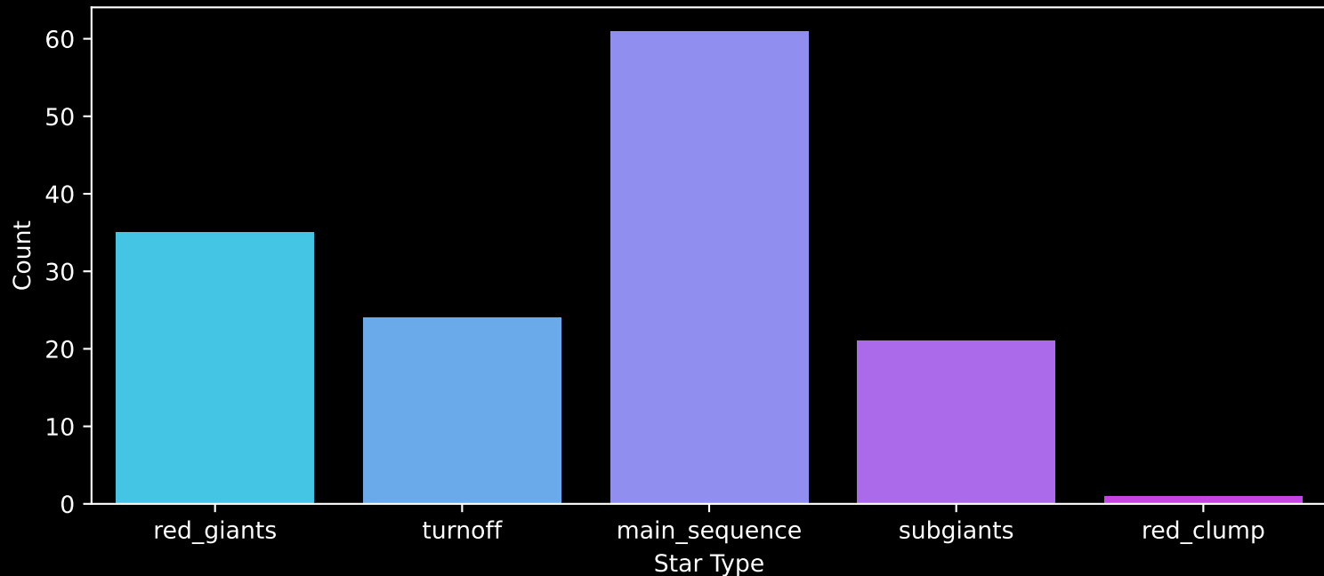
Gaia Cluster: [Hogg_17] Count plot of Star Type
