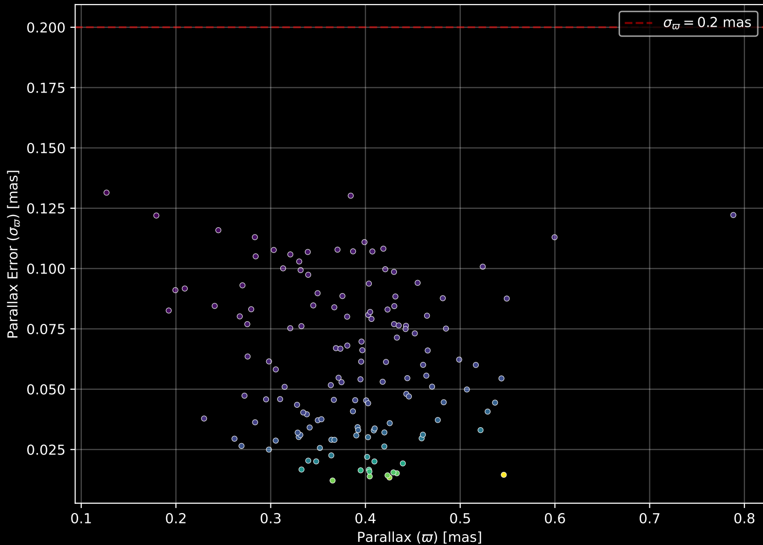
Gaia Cluster: [Hogg_17] Parallax Quality (n= 142)
