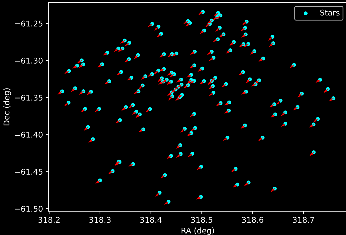
Gaia Cluster: [Hogg_17] Proper Motion Vectors for Gaia Star Field (n= 142)
