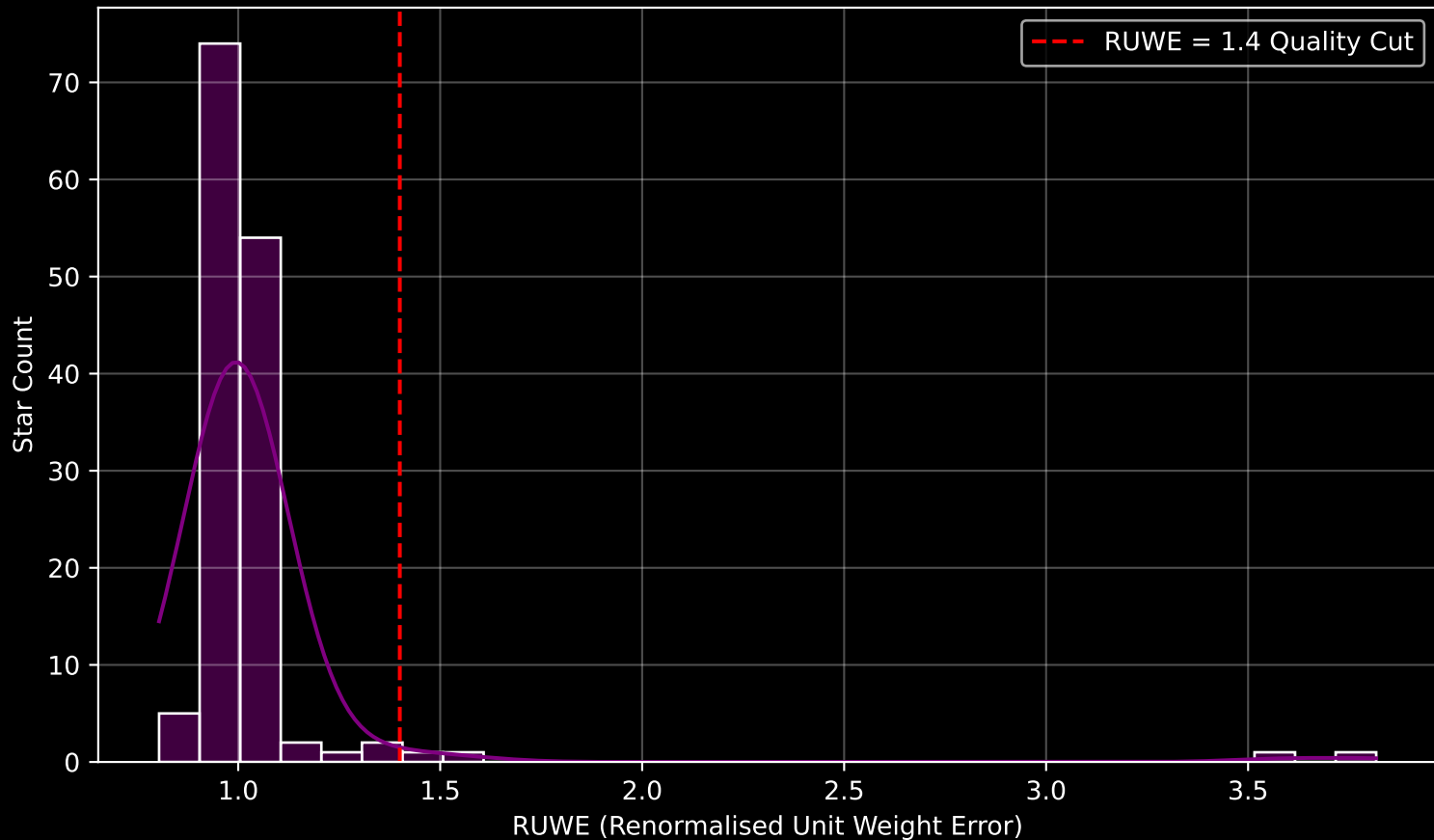
Gaia Cluster: [Hogg_17] RUWE Distribution (n= 142)
