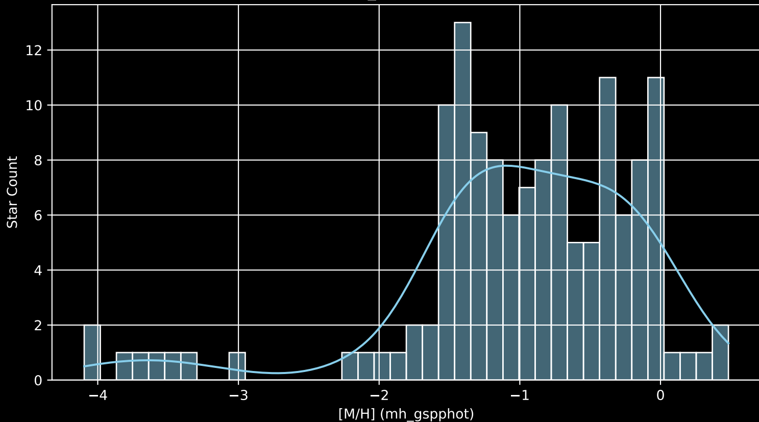
Gaia Cluster: [Hogg_17 [M/H] (mh_gspphot) (n= 138)
