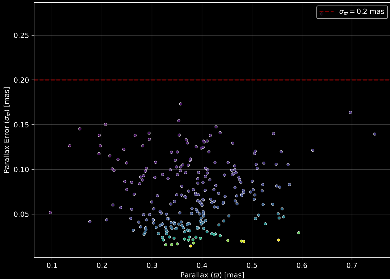
Gaia Cluster: [Hogg_21] Parallax Quality (n= 252)
