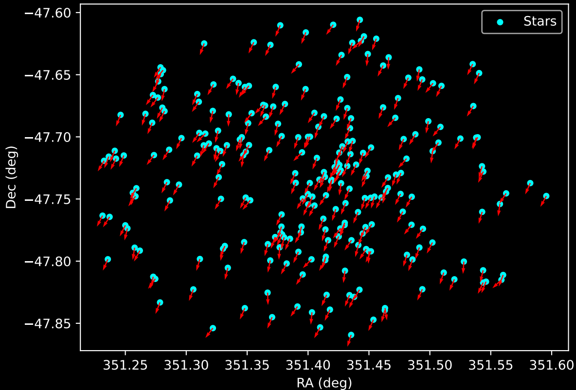
Gaia Cluster: [Hogg_21] Proper Motion Vectors for Gaia Star Field (n= 252)
