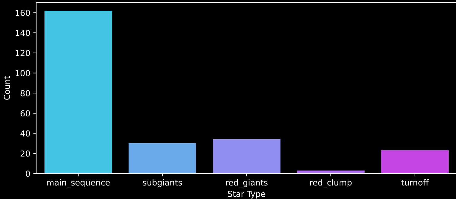
Gaia Cluster: [Hogg_21] Count plot of Star Type
