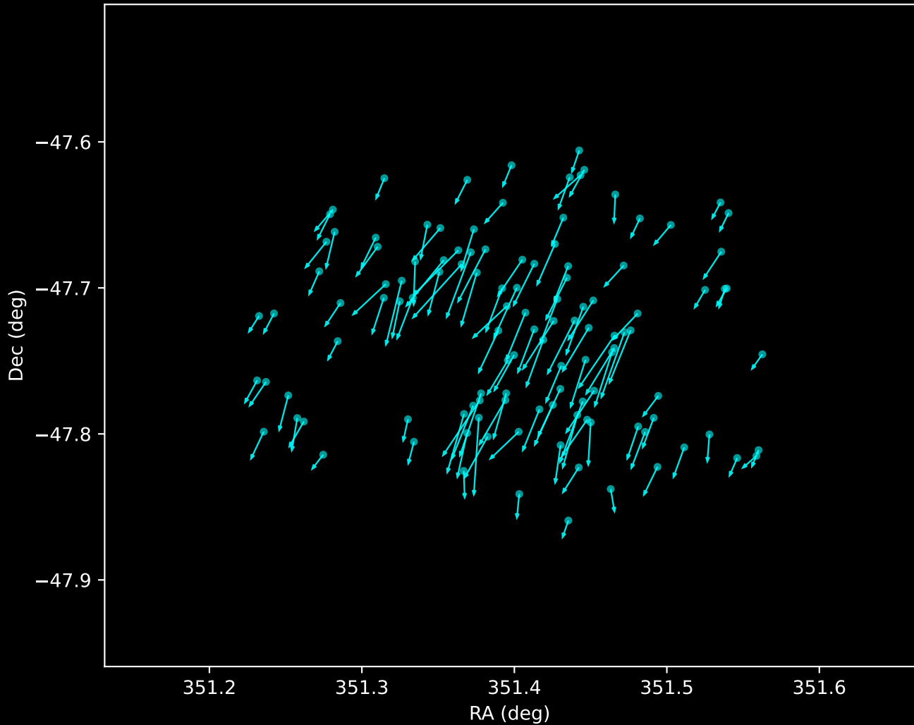
Gaia DR3 Noise Stream Proper Motion Vectors (n=118)
