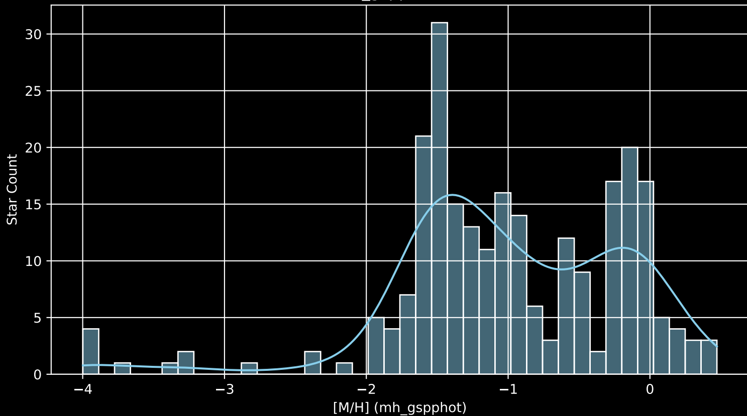
Gaia Cluster: [Hogg_21 [M/H] (mh_gspphot) (n= 250)
