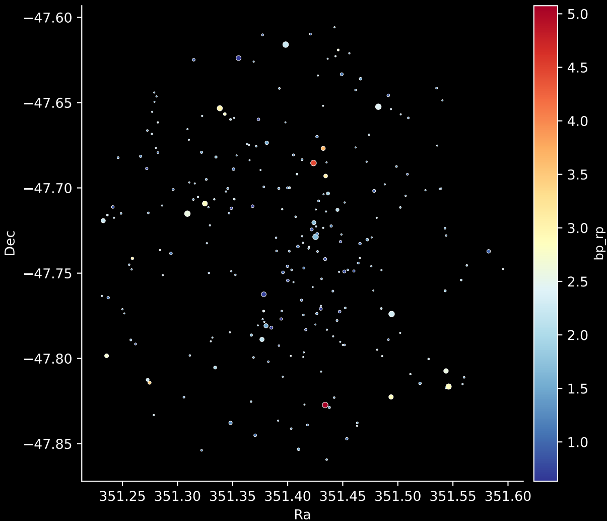
Gaia Cluster: [Hogg_21] Stars: 252
