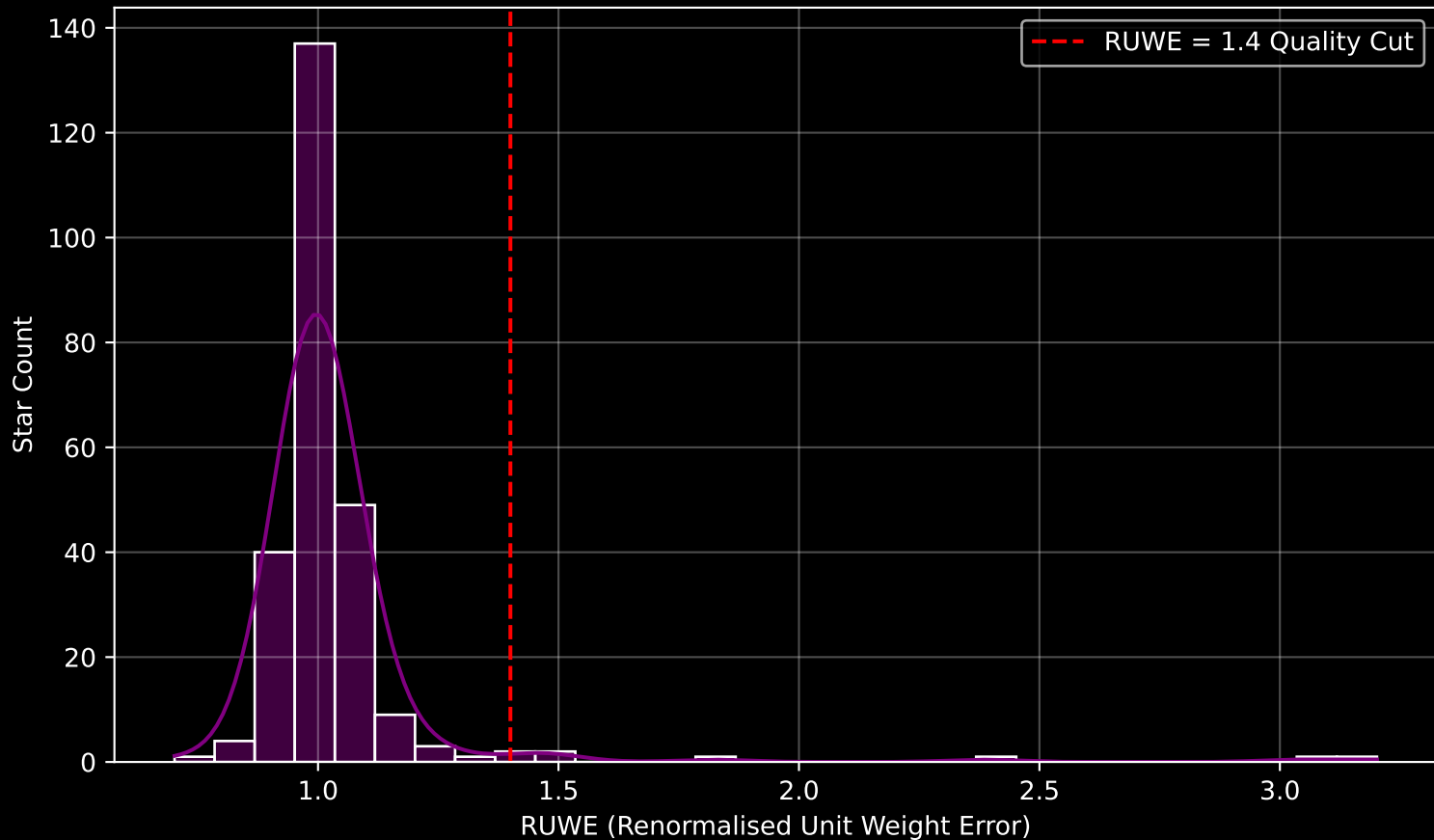
Gaia Cluster: [Hogg_21] RUWE Distribution (n= 252)
