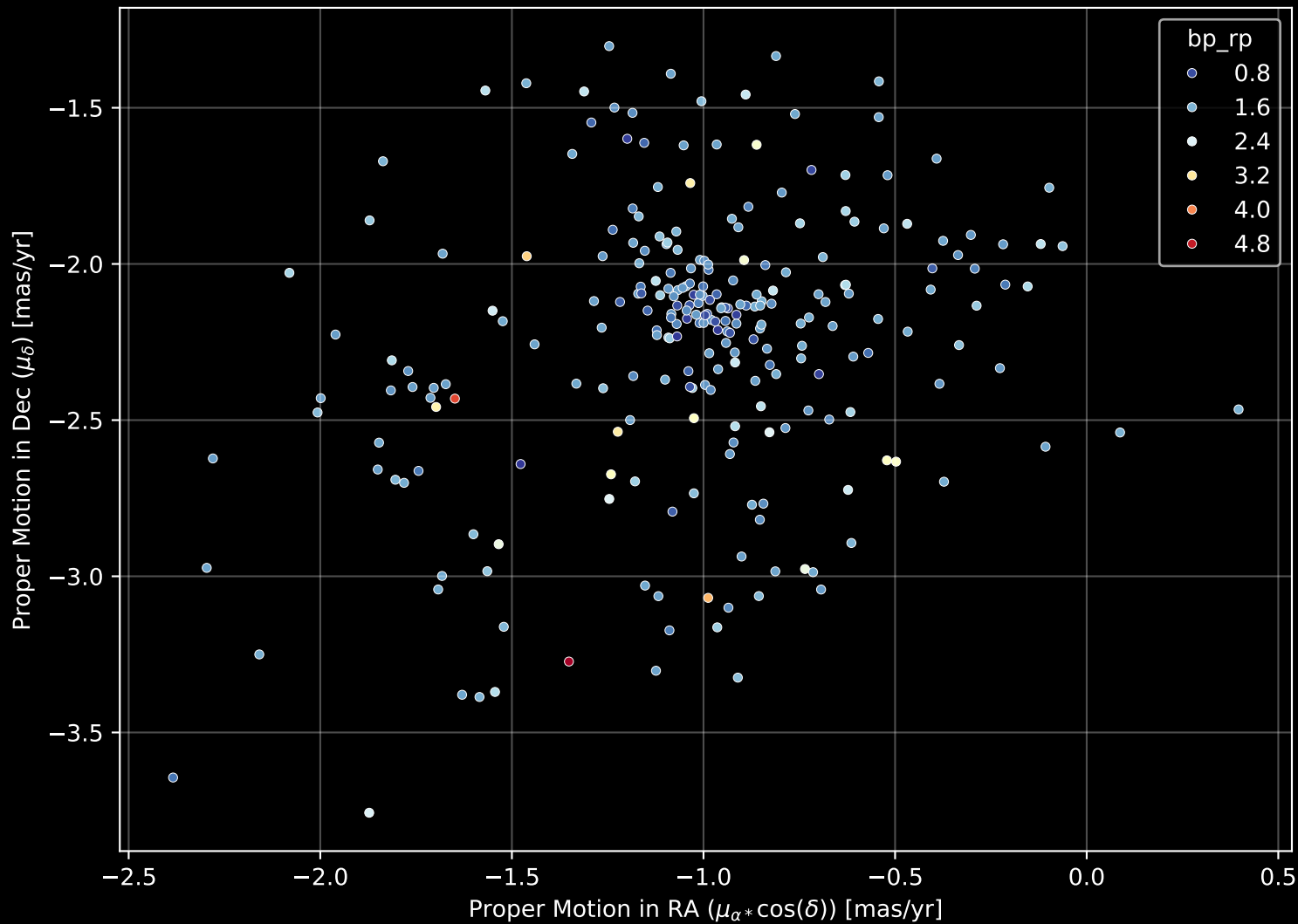
Gaia Cluster: [Hogg_21] Proper Motion Diagram (n= 252)
