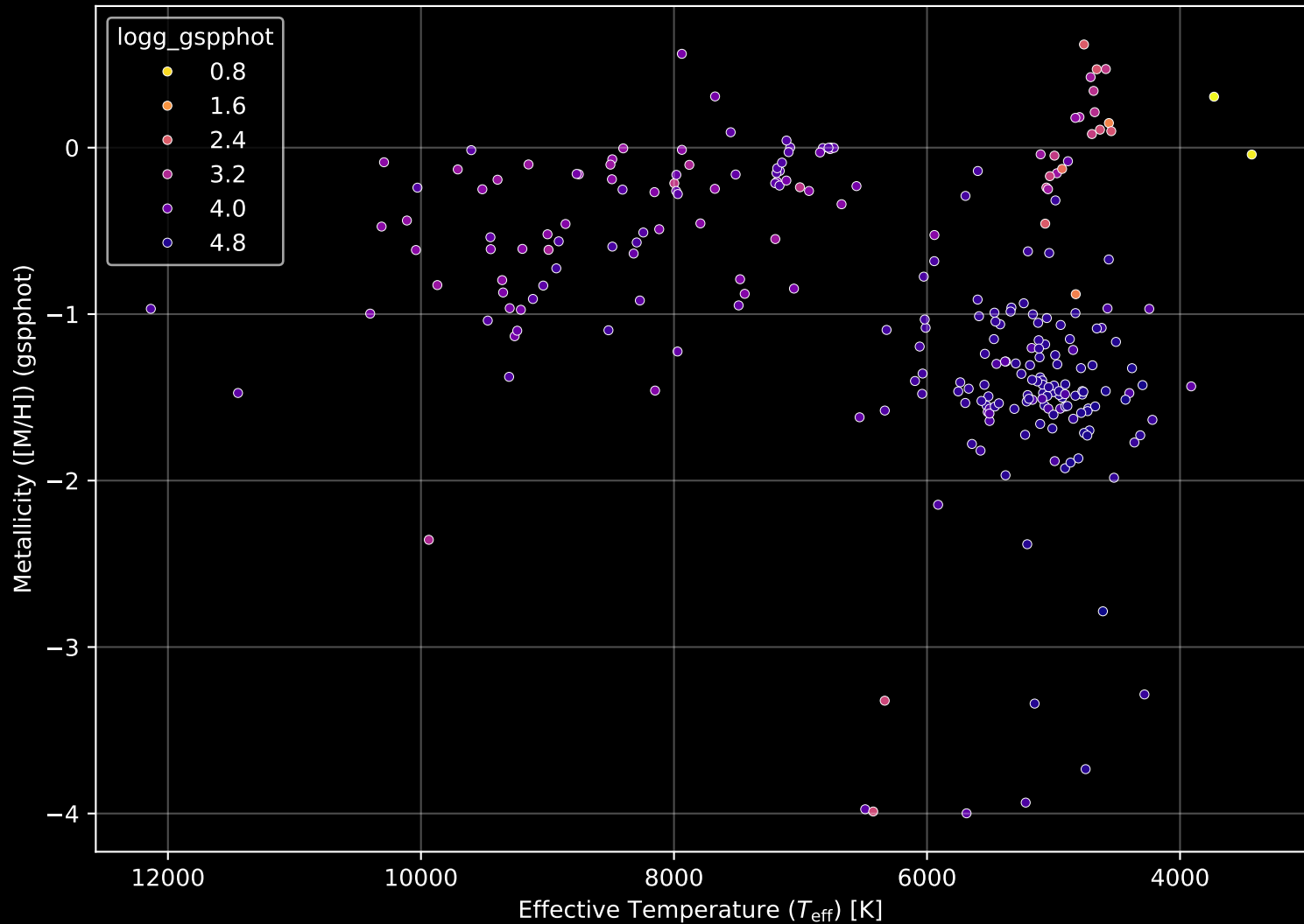
Gaia Cluster: [Hogg_21] Stellar Population Parameters (n= 252)
