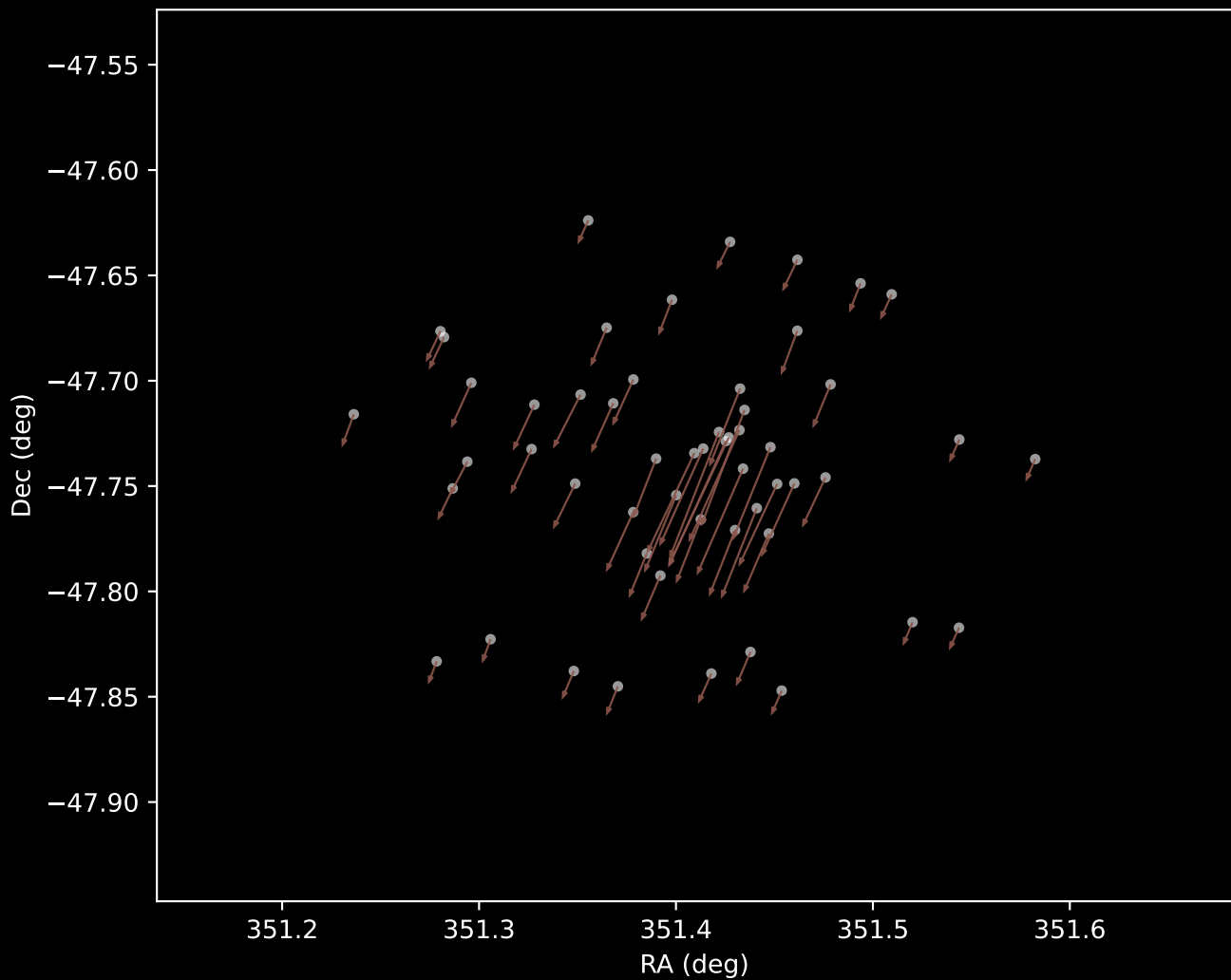
Gaia DR3 Cluster 10 Proper Motion Vectors (n=54)
