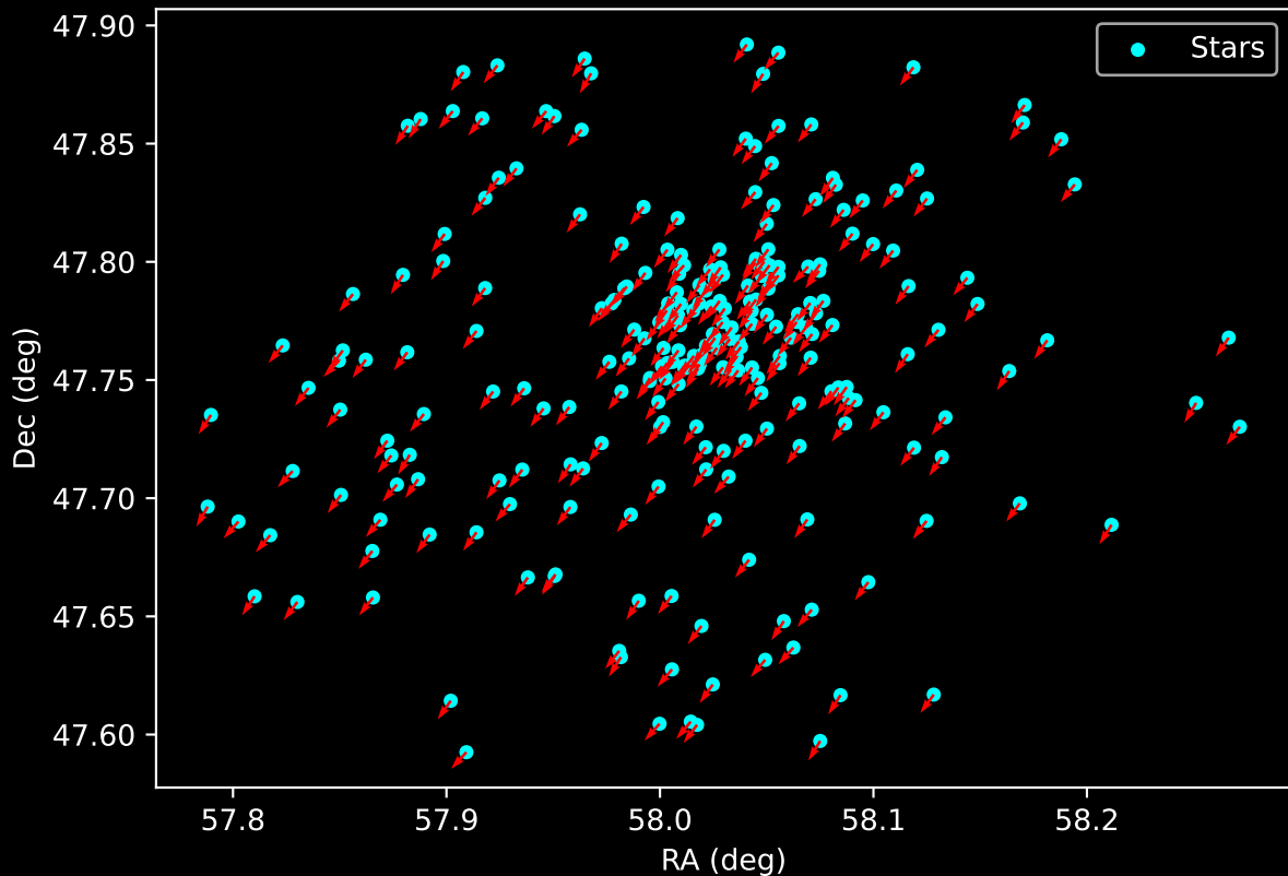
Gaia Cluster: [IC_1369] Proper Motion Vectors for Gaia Star Field (n= 250)
