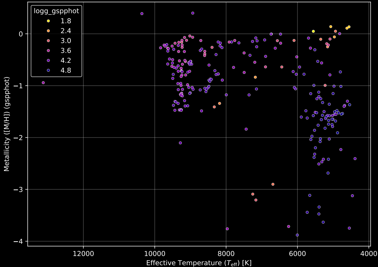
Gaia Cluster: [IC_1369] Stellar Population Parameters (n= 250)
