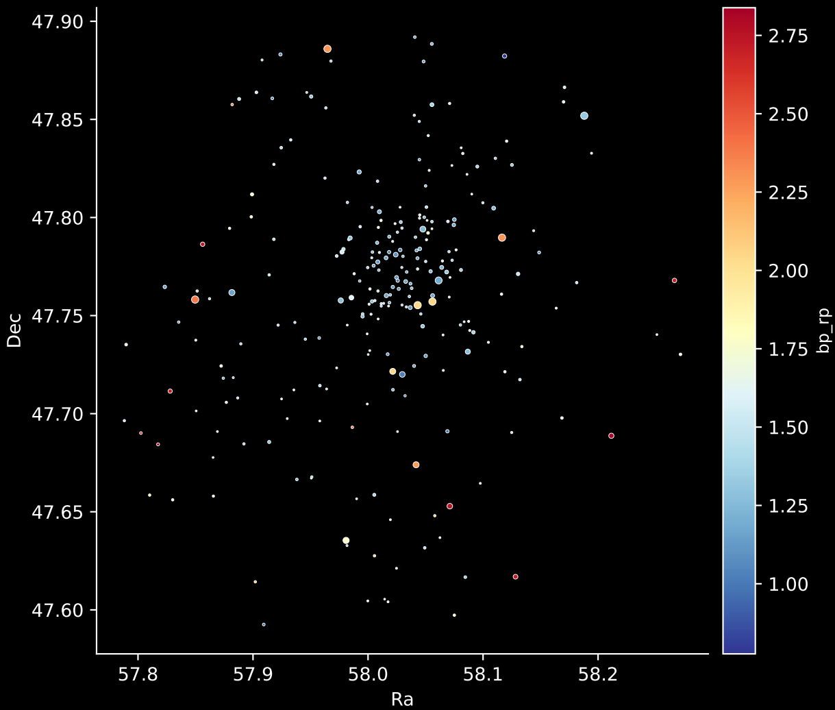
Gaia Cluster: [IC_1369] Stars: 250
