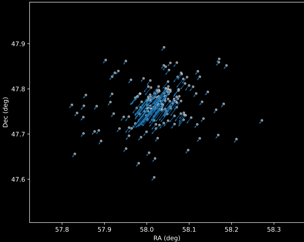
Gaia DR3 Cluster 0 Proper Motion Vectors (n=176)
