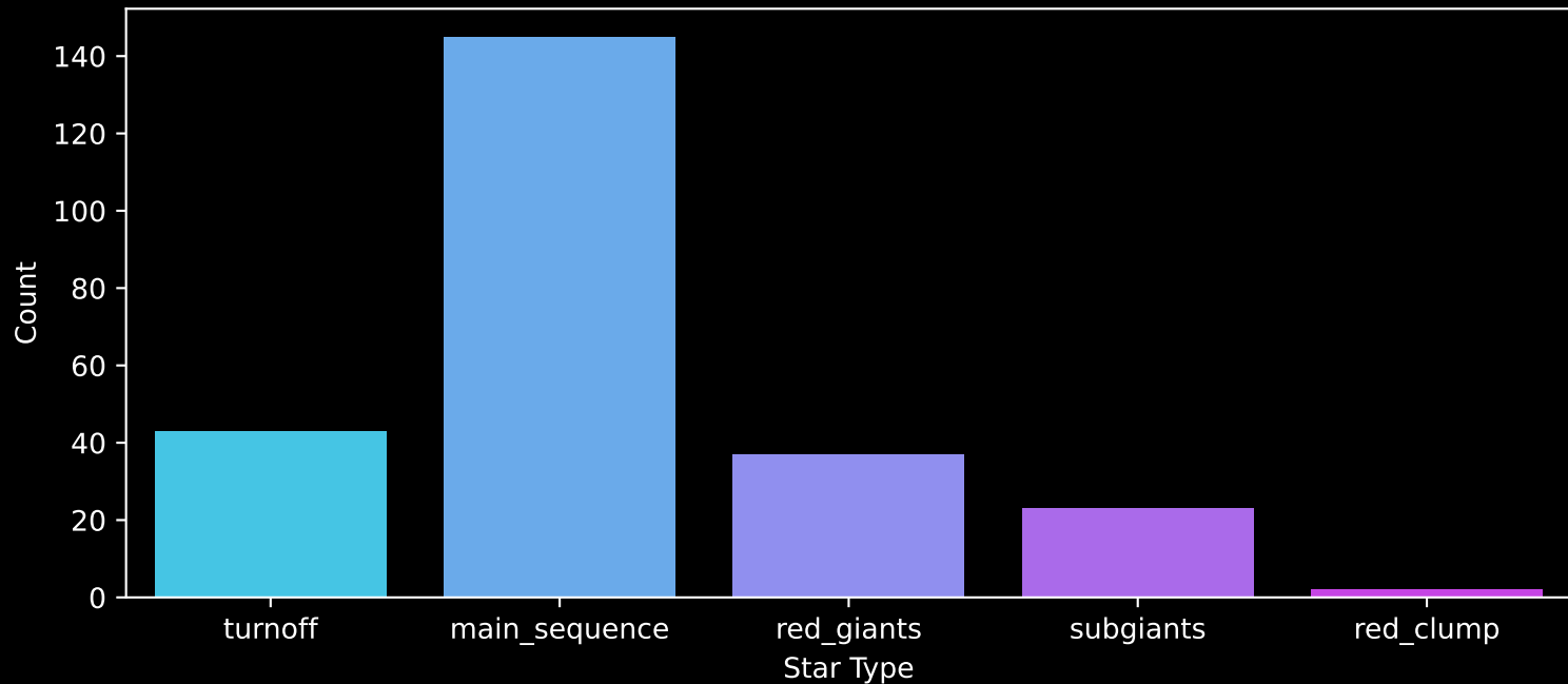
Gaia Cluster: [IC_1369] Count plot of Star Type
