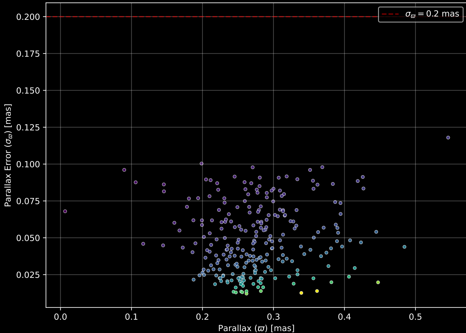
Gaia Cluster: [IC_1369] Parallax Quality (n= 250)
