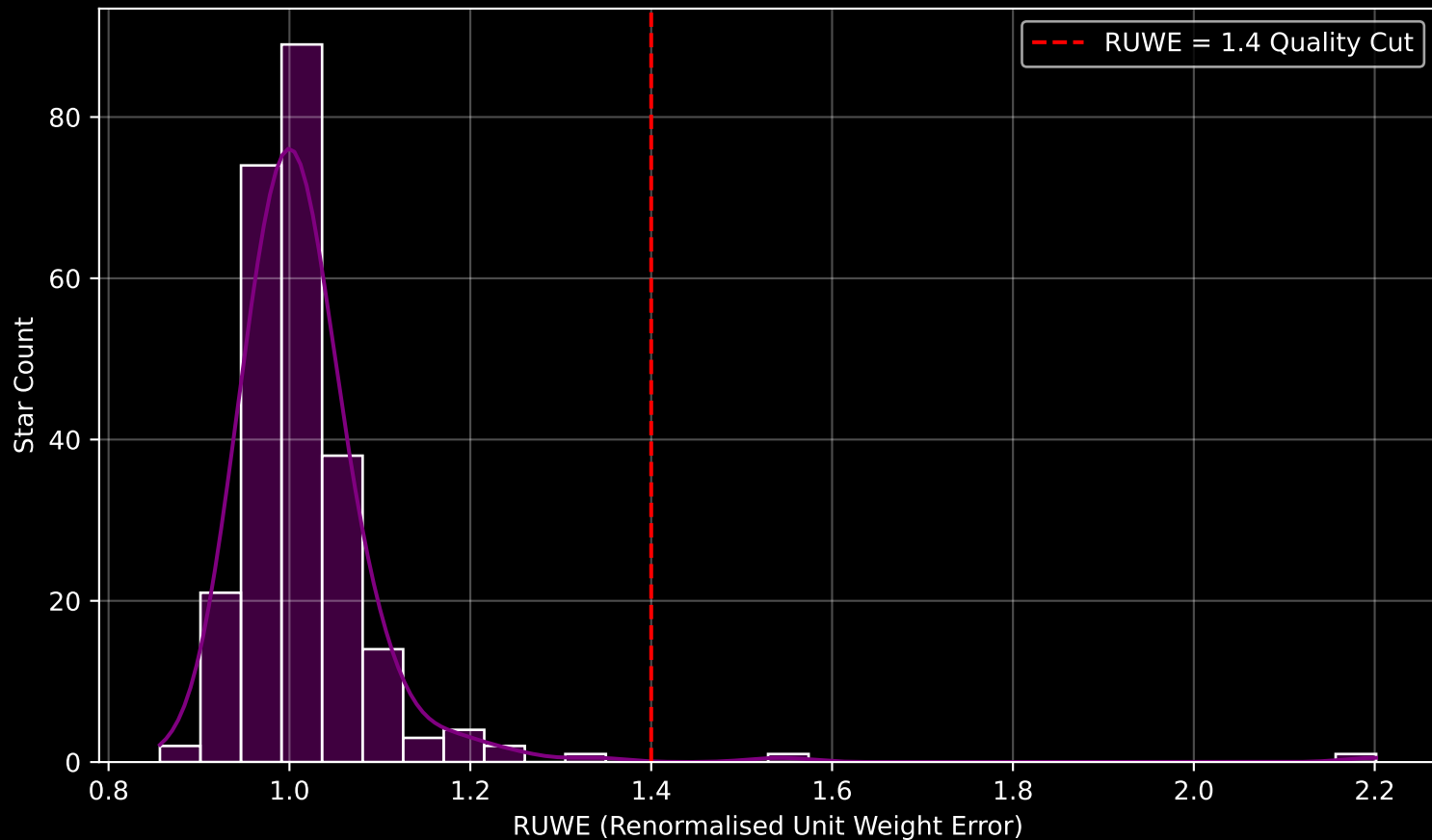
Gaia Cluster: [IC_1369] RUWE Distribution (n= 250)
