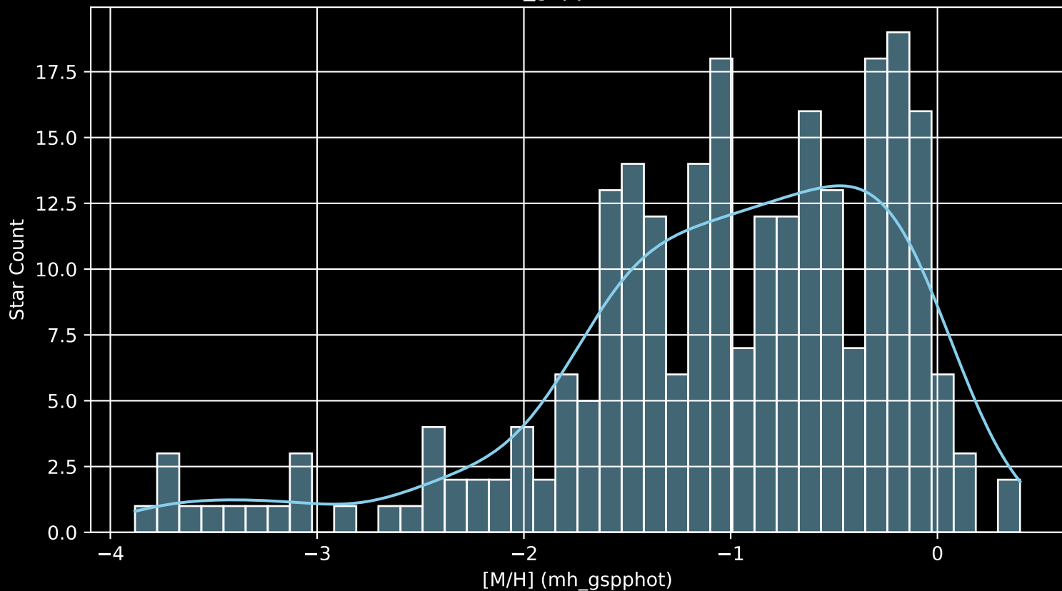
Gaia Cluster: [IC_1369 [M/H] (mh_gspphot) (n= 250)
