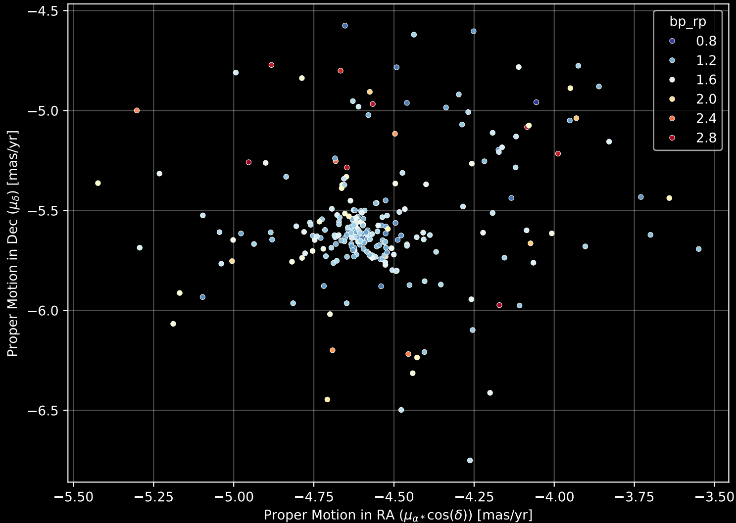
Gaia Cluster: [IC_1369] Proper Motion Diagram (n= 250)
