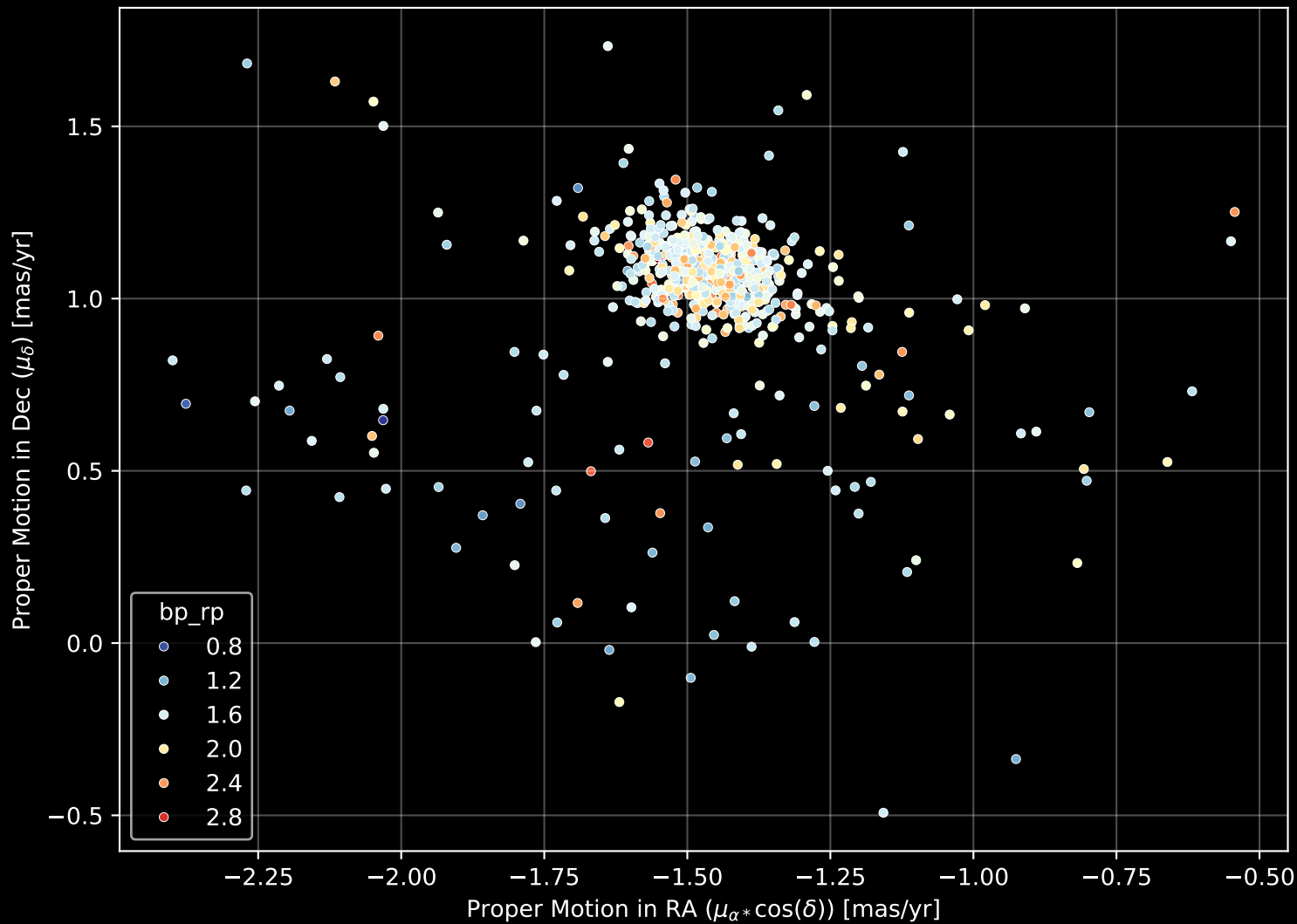
Gaia Cluster: [IC_166] Proper Motion Diagram (n= 656)
