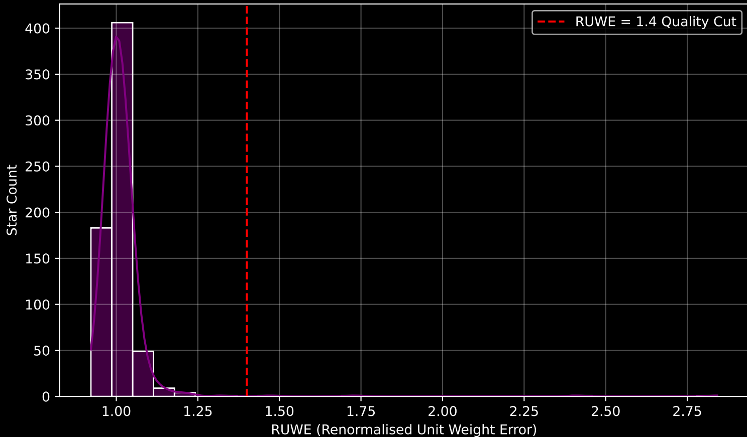
Gaia Cluster: [IC_166] RUWE Distribution (n= 656)
