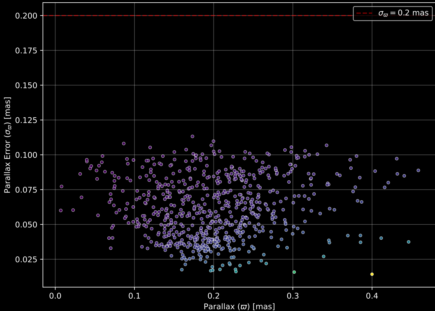
Gaia Cluster: [IC_166] Parallax Quality (n= 656)
