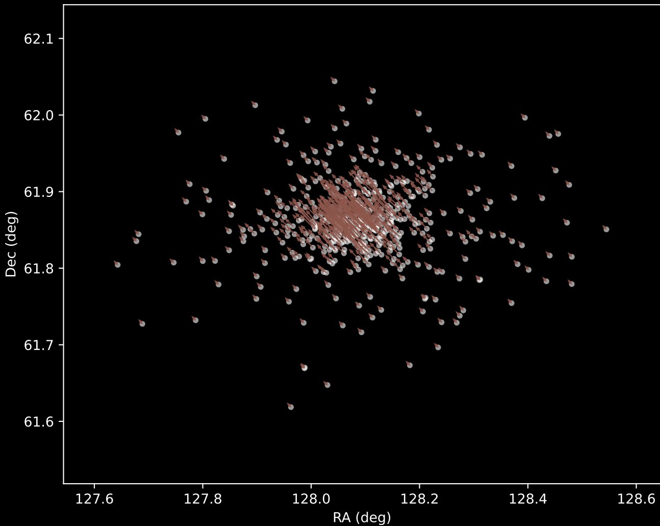
Gaia DR3 Cluster 10 Proper Motion Vectors (n=488)
