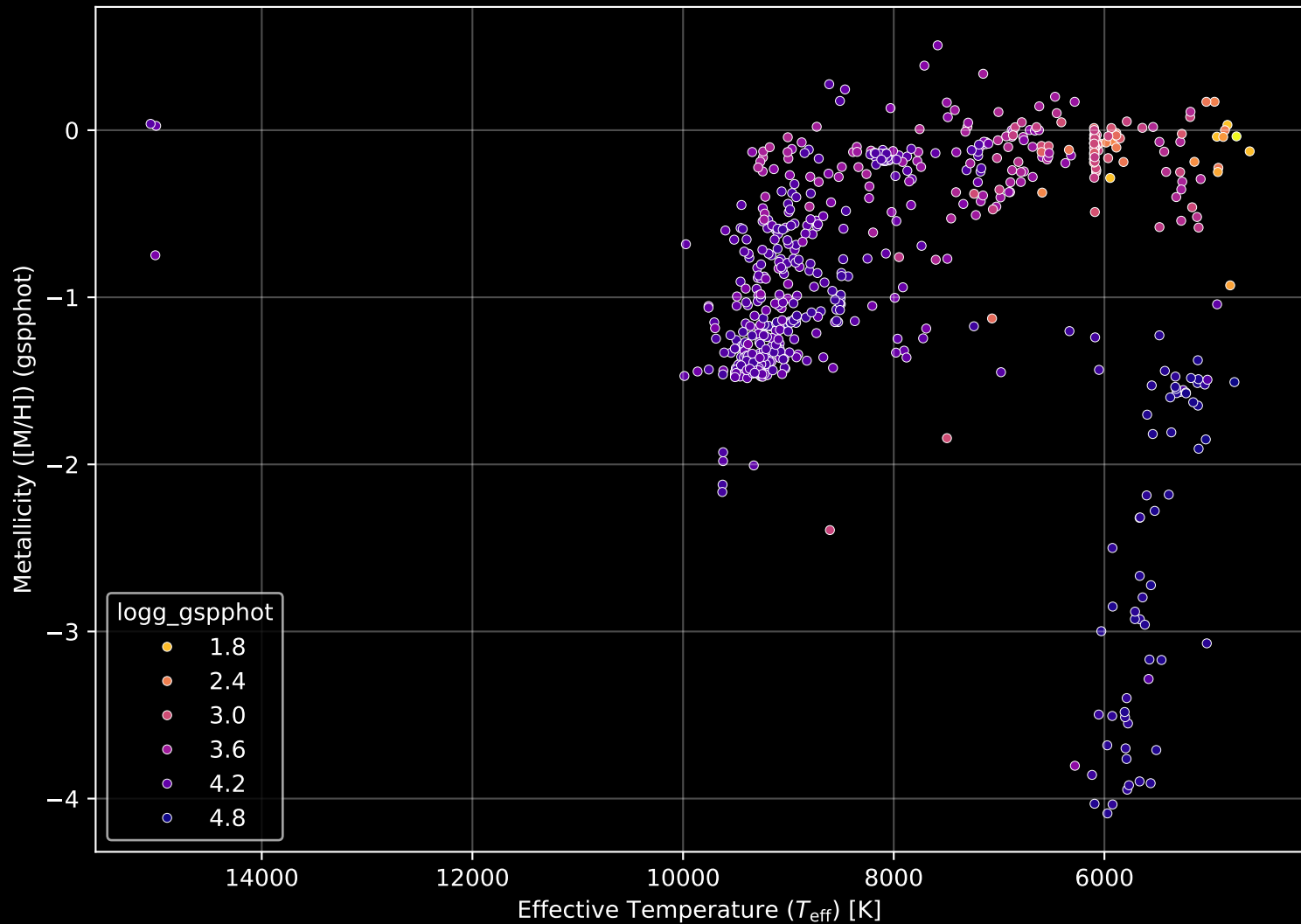
Gaia Cluster: [IC_166] Stellar Population Parameters (n= 656)
