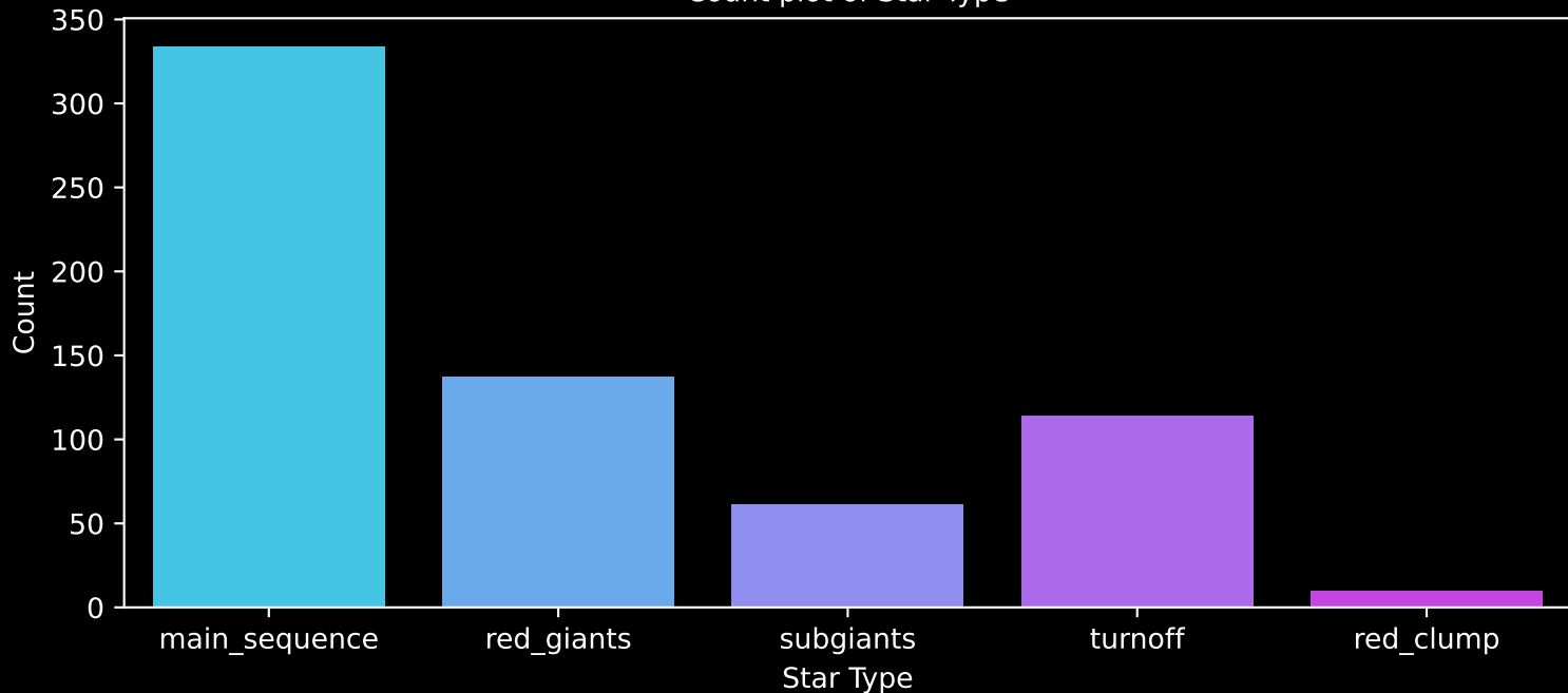
Gaia Cluster: [IC_166] Count plot of Star Type
