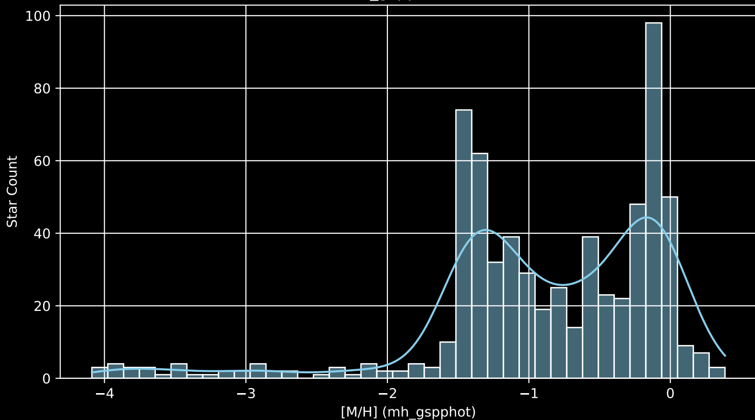
Gaia Cluster: [IC_166 [M/H] (mh_gspphot) (n= 655)
