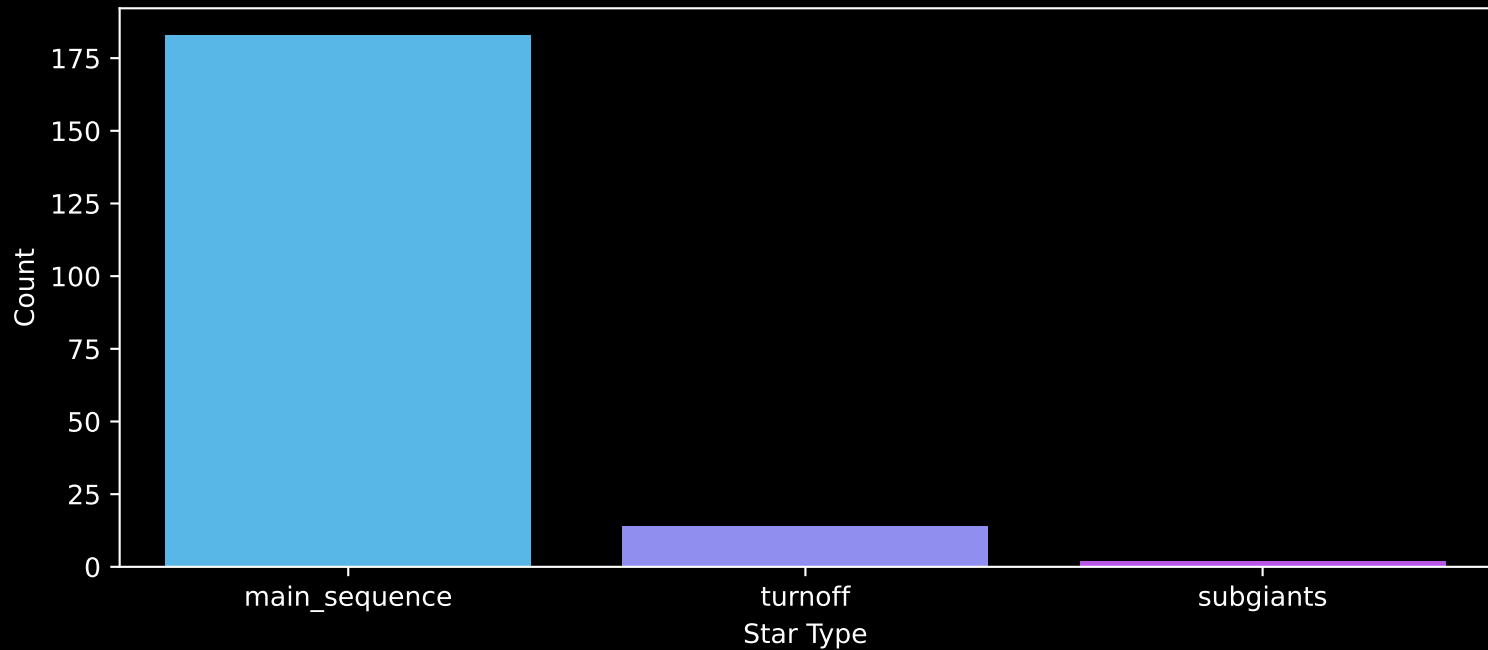
Gaia Cluster: [IC_2391] Count plot of Star Type
