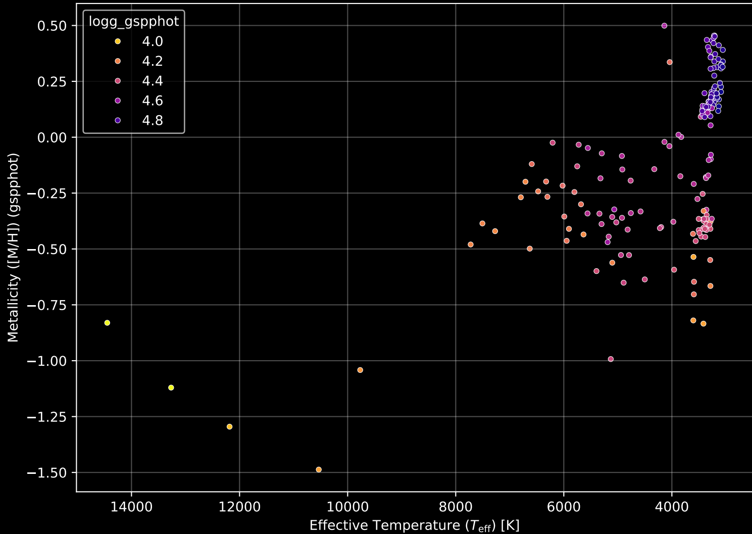
Gaia Cluster: [IC_2391] Stellar Population Parameters (n= 199)
