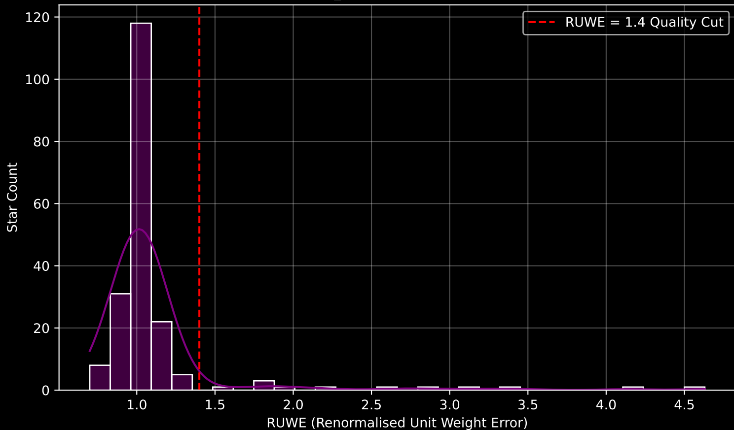
Gaia Cluster: [IC_2391] RUWE Distribution (n= 196)
