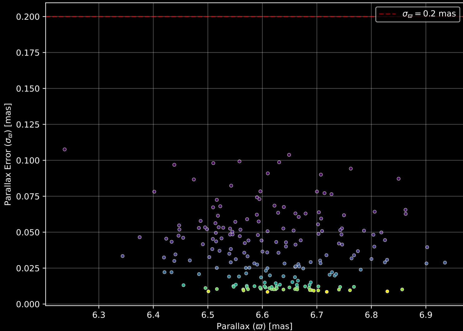
Gaia Cluster: [IC_2391] Parallax Quality (n= 199)
