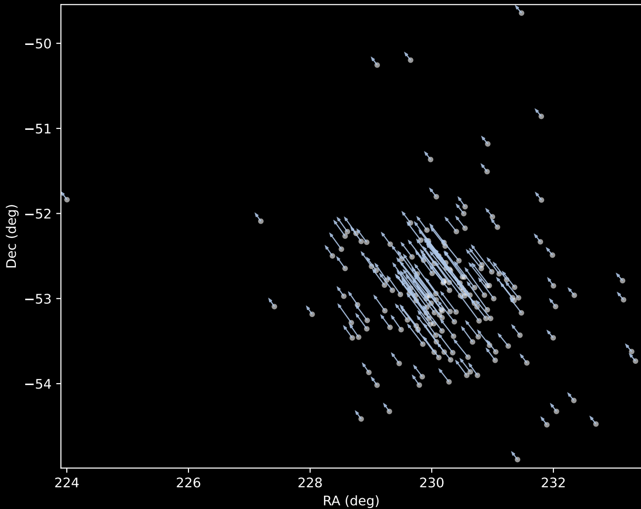
Gaia DR3 Cluster 1 Proper Motion Vectors (n=168)
