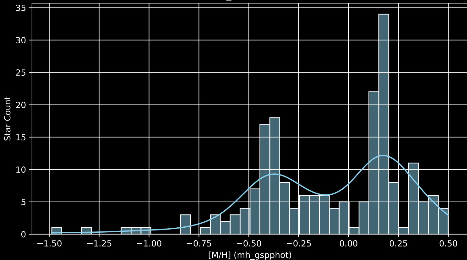
Gaia Cluster: [IC_2391 [M/H] (mh_gspphot) (n= 199)
