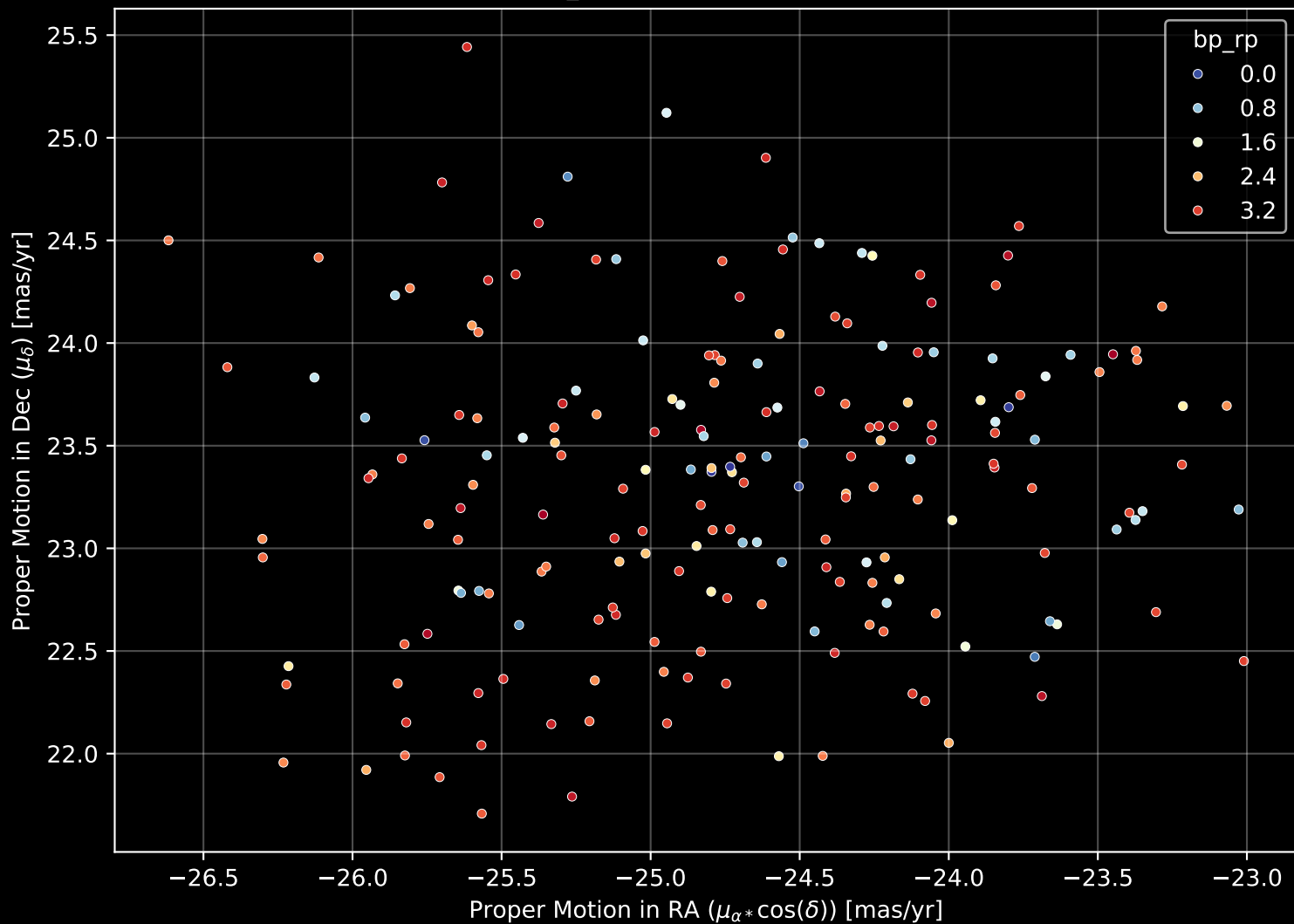
Gaia Cluster: [IC_2391] Proper Motion Diagram (n= 199)
