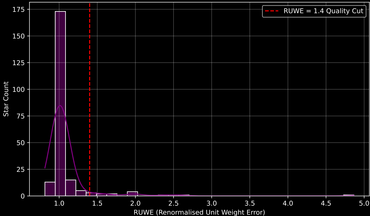
Gaia Cluster: [IC_2395] RUWE Distribution (n= 221)
