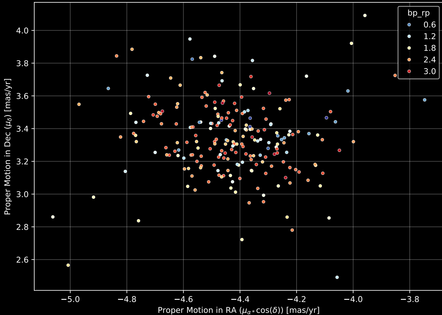
Gaia Cluster: [IC_2395] Proper Motion Diagram (n= 222)
