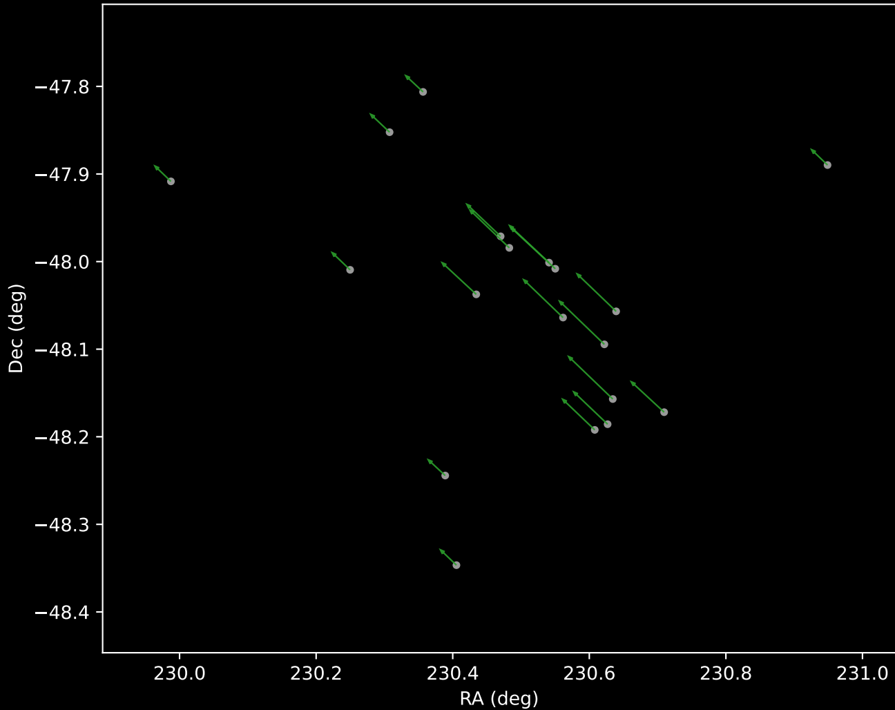
Gaia DR3 Cluster 4 Proper Motion Vectors (n=19)
