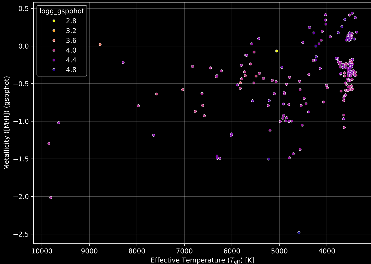
Gaia Cluster: [IC_2395] Stellar Population Parameters (n= 222)
