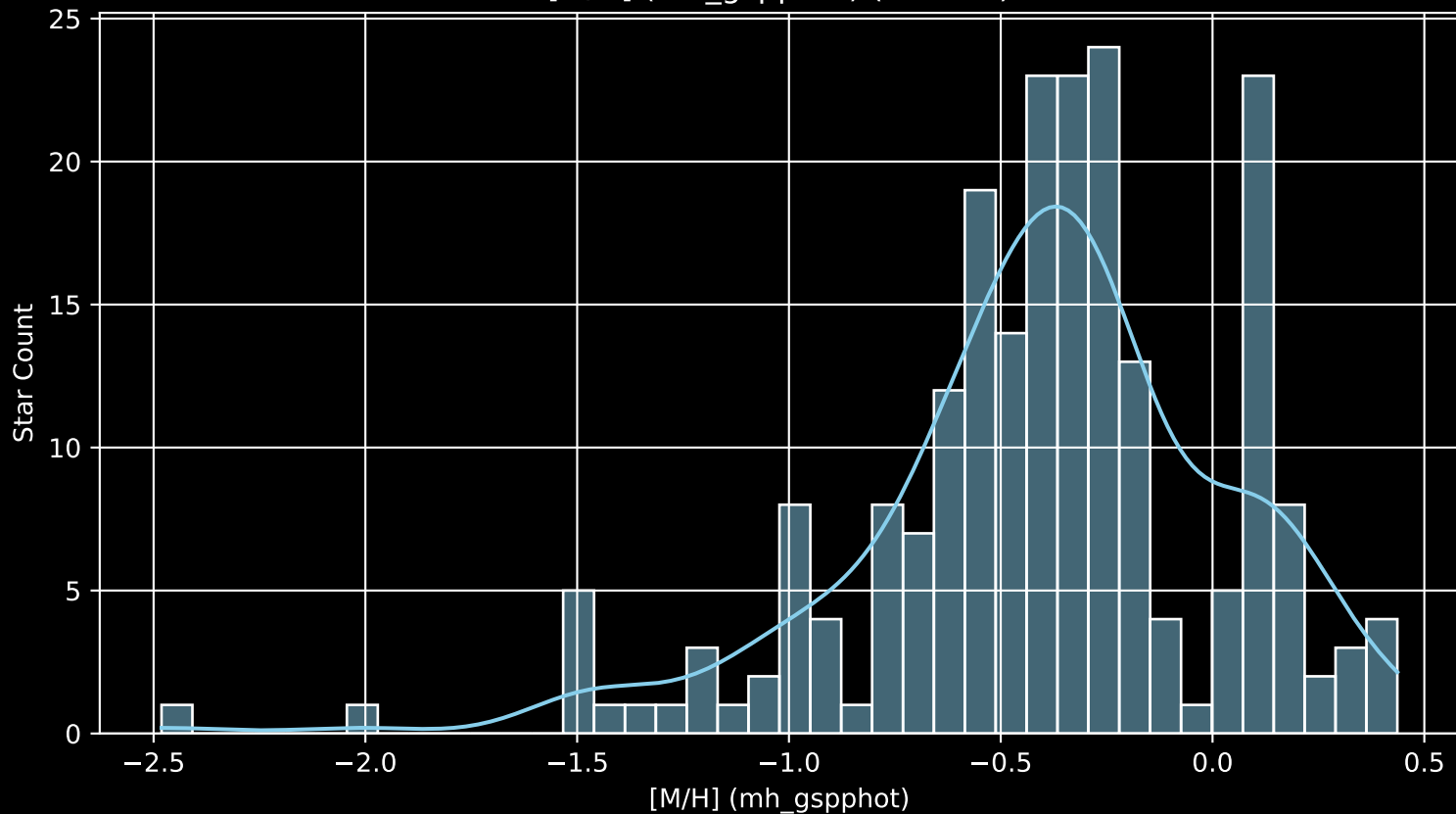
Gaia Cluster: [IC_2395 [M/H] (mh_gspphot) (n= 222)
