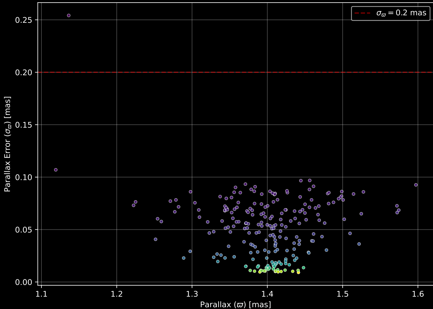
Gaia Cluster: [IC 2395] Parallax Quality (n= 222)
