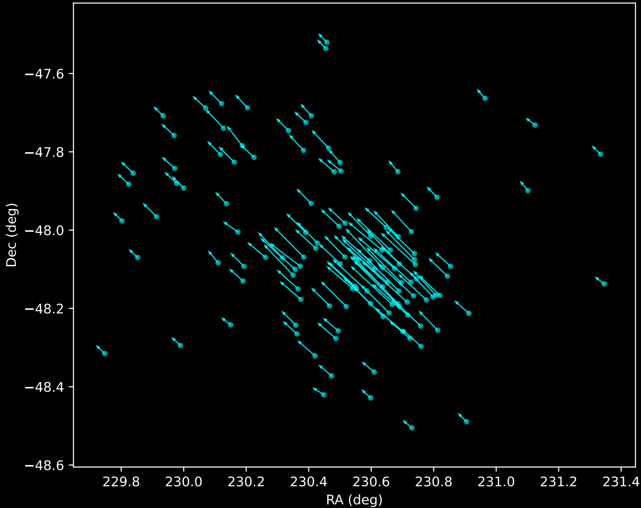
Gaia DR3 Noise Stream Proper Motion Vectors (n=119)
