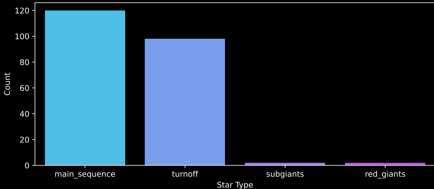
Gaia Cluster: [IC_2395] Count plot of Star Type
