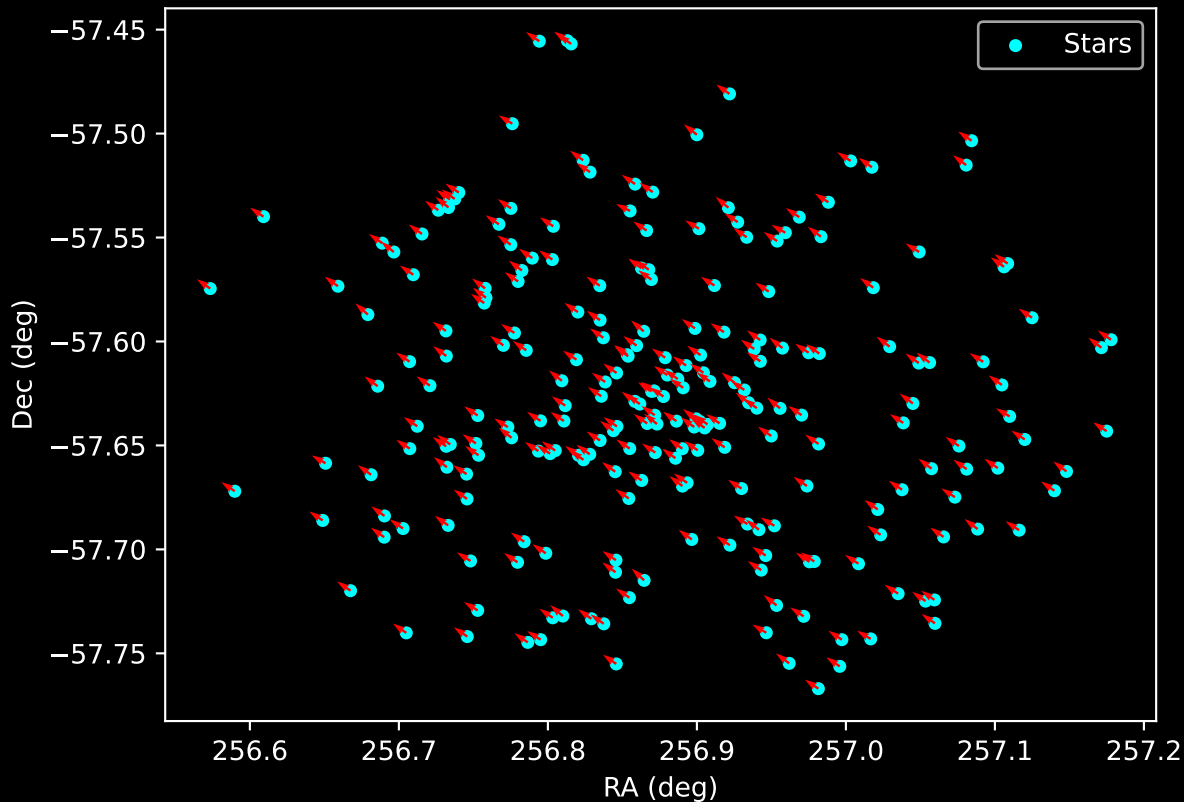
Gaia Cluster: [IC_2581] Proper Motion Vectors for Gaia Star Field (n= 230)
