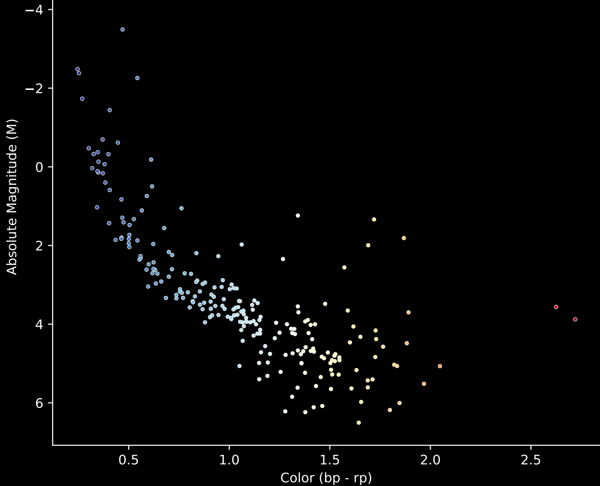
Gaia Cluster: [IC 2581] Stars (n= 230) Hertzsprung-Russel Diagram
