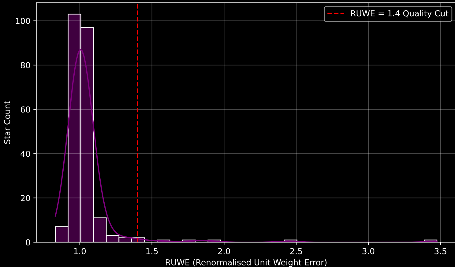
Gaia Cluster: [IC_2581] RUWE Distribution (n= 230)
