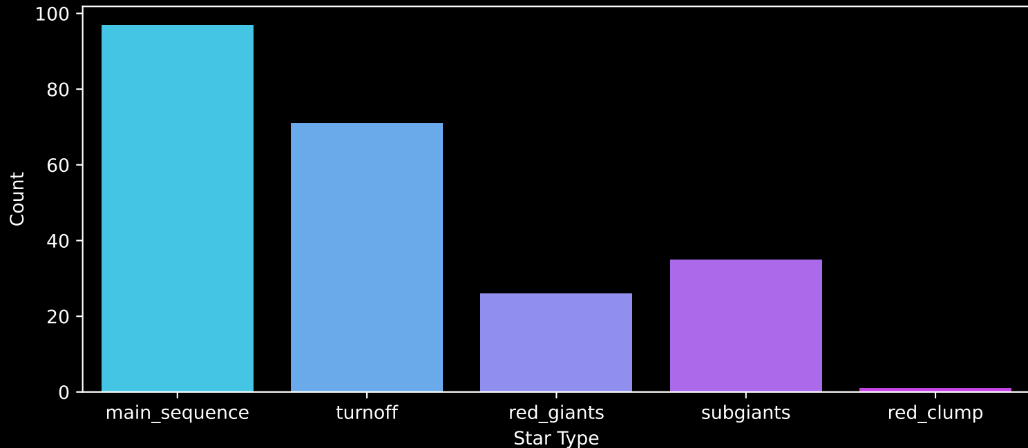
Gaia Cluster: [IC_2581] Count plot of Star Type
