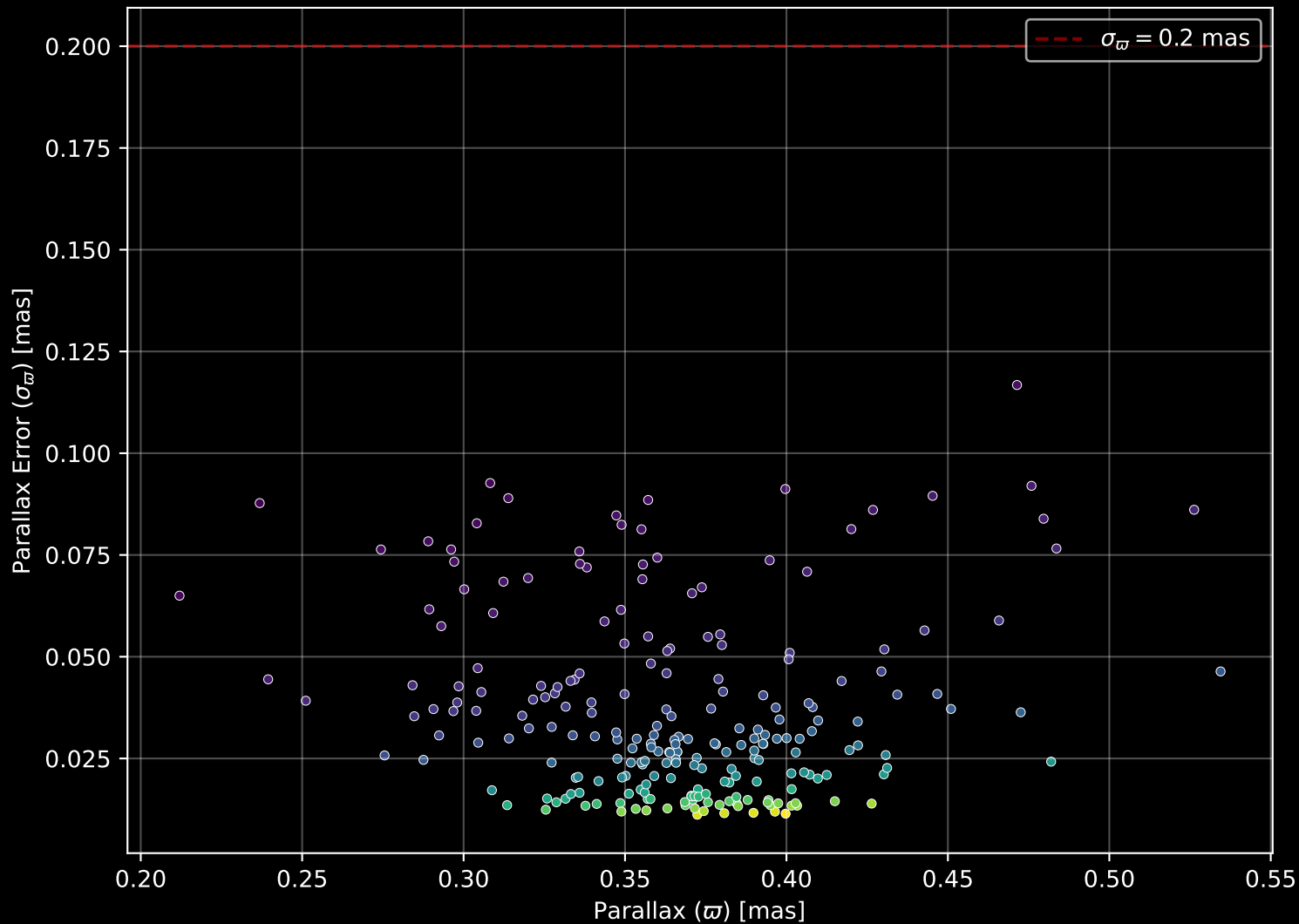
Gaia Cluster: [IC_2581] Parallax Quality (n= 230)
