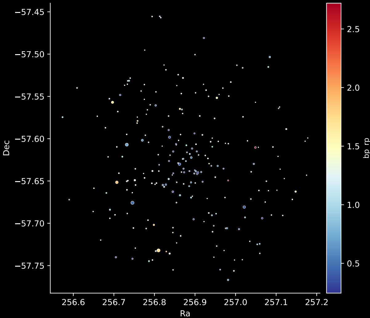
Gaia Cluster: [IC_2581] Stars: 230
