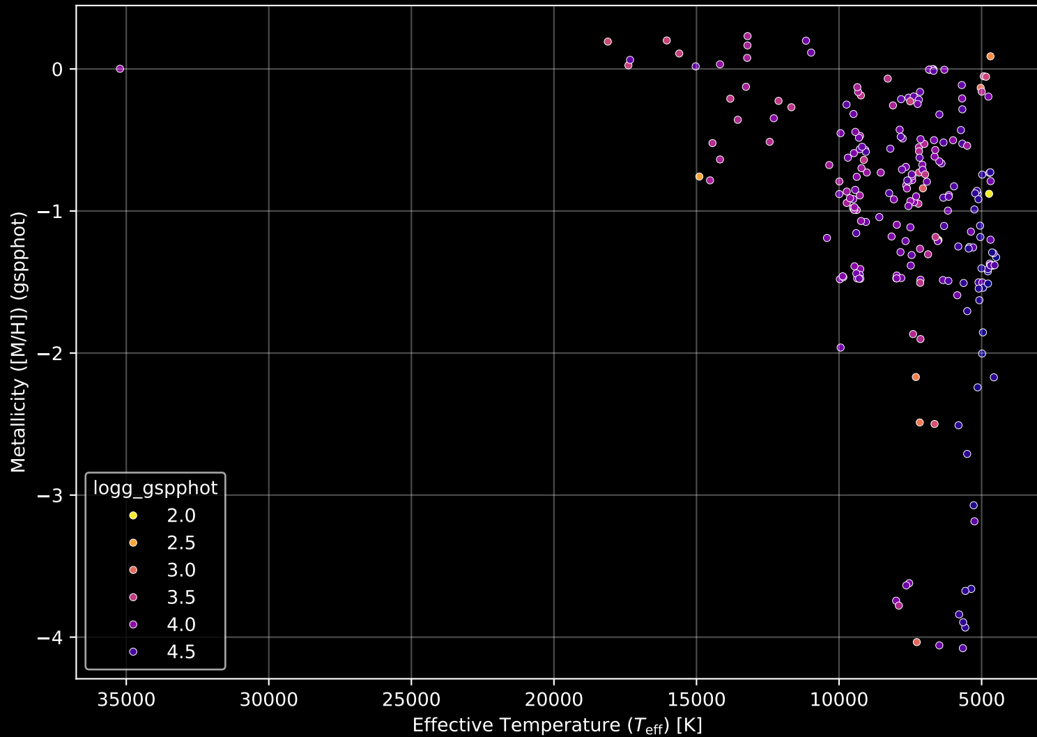
Gaia Cluster: [IC_2581] Stellar Population Parameters (n= 230)
