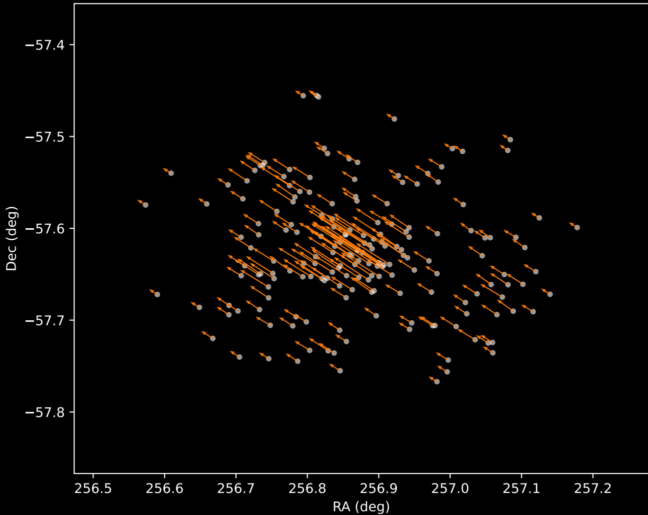
Gaia DR3 Cluster 2 Proper Motion Vectors (n=183)
