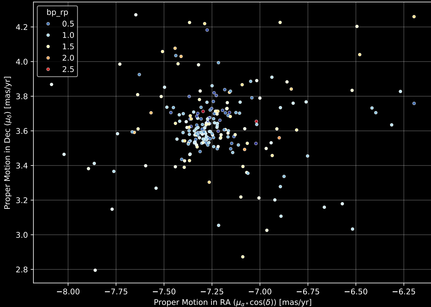
Gaia Cluster: [IC_2581] Proper Motion Diagram (n= 230)
