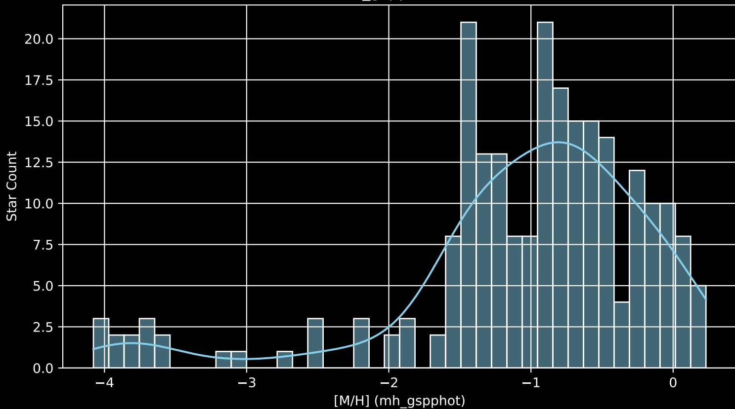
Gaia Cluster: [IC_2581 [M/H] (mh_gspphot) (n= 230)
