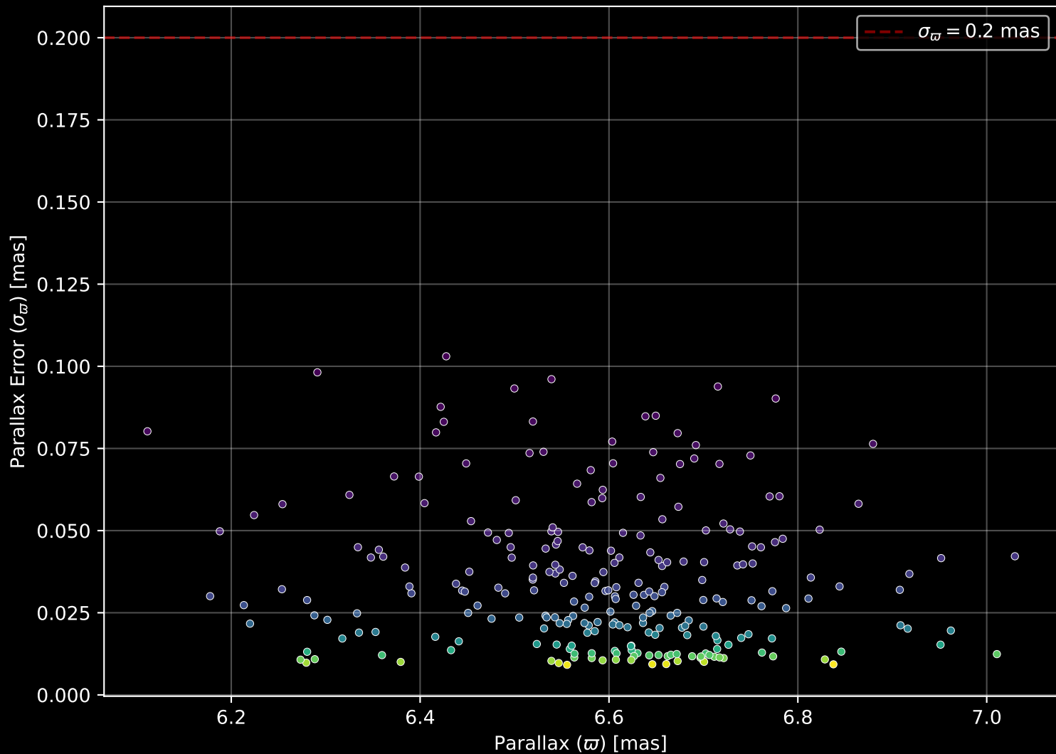
Gaia Cluster: [IC_2602] Parallax Quality (n= 252)
