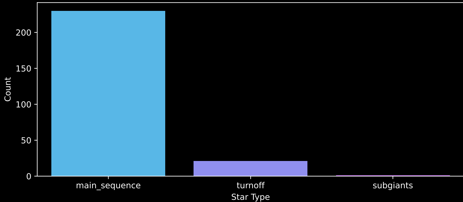
Gaia Cluster: [IC_2602] Count plot of Star Type
