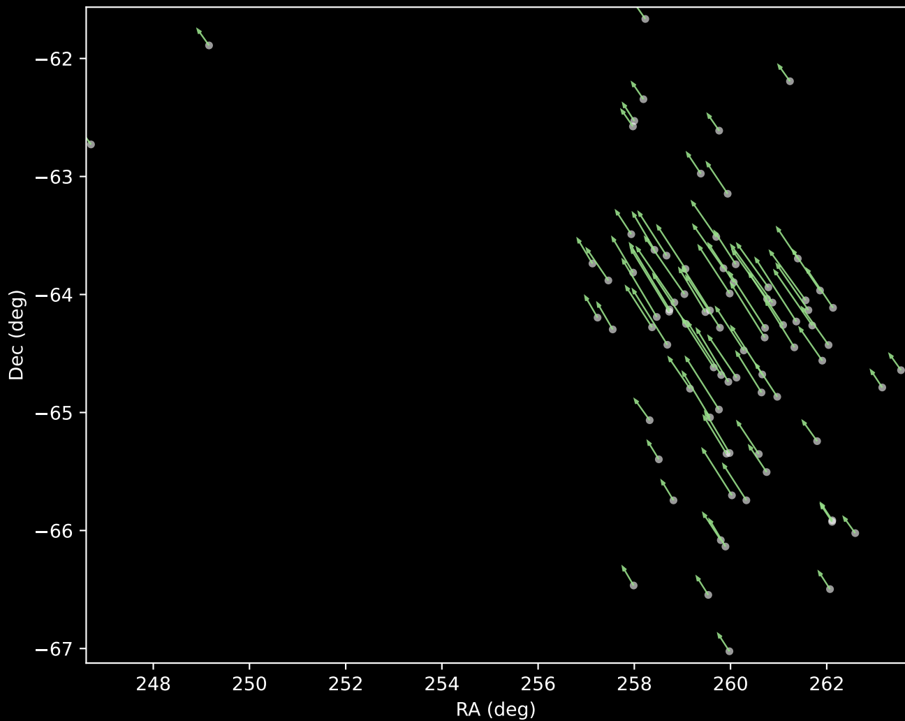
Gaia DR3 Cluster 5 Proper Motion Vectors (n=83)
