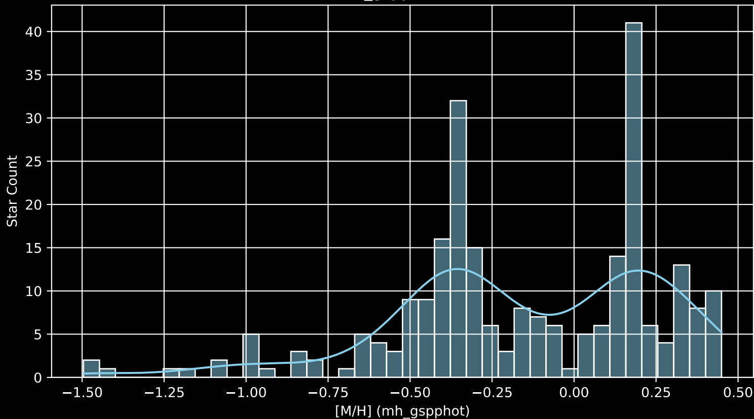
Gaia Cluster: [IC_2602 [M/H] (mh_gspphot) (n= 250)
