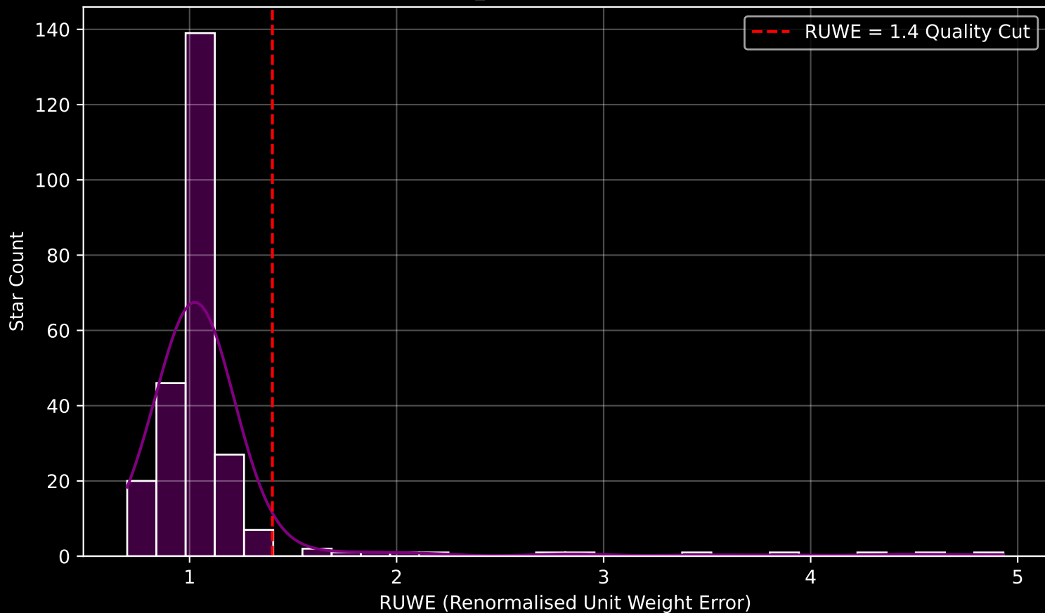
Gaia Cluster: [IC_2602] RUWE Distribution (n= 252)
