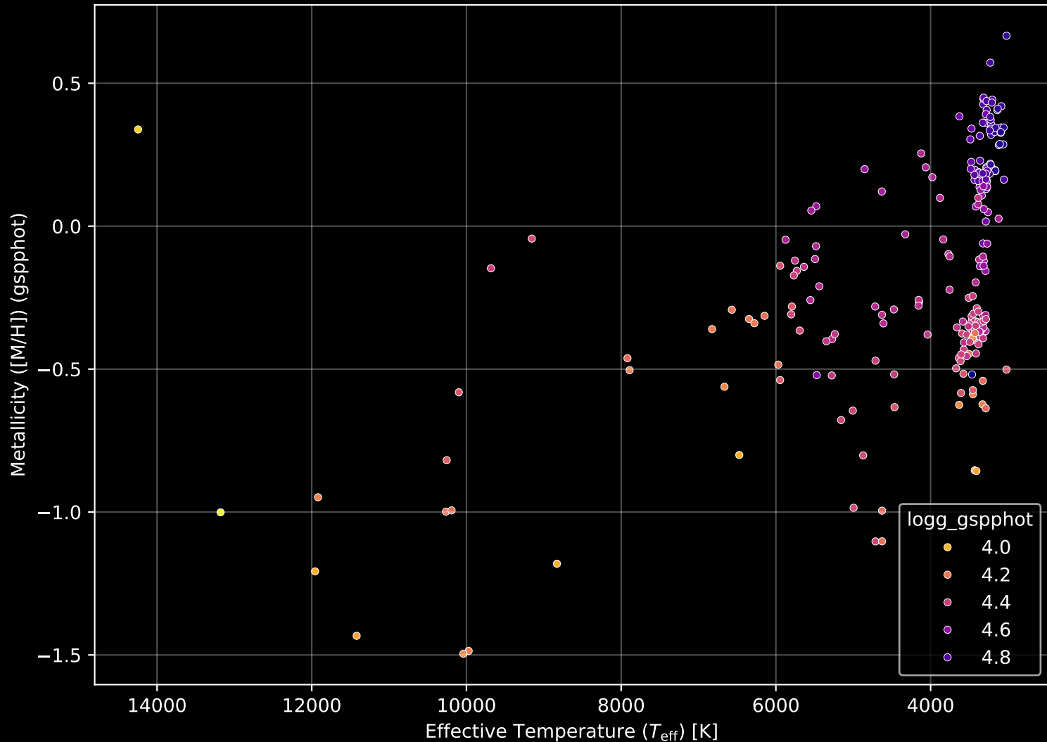
Gaia Cluster: [IC_2602] Stellar Population Parameters (n= 252)
