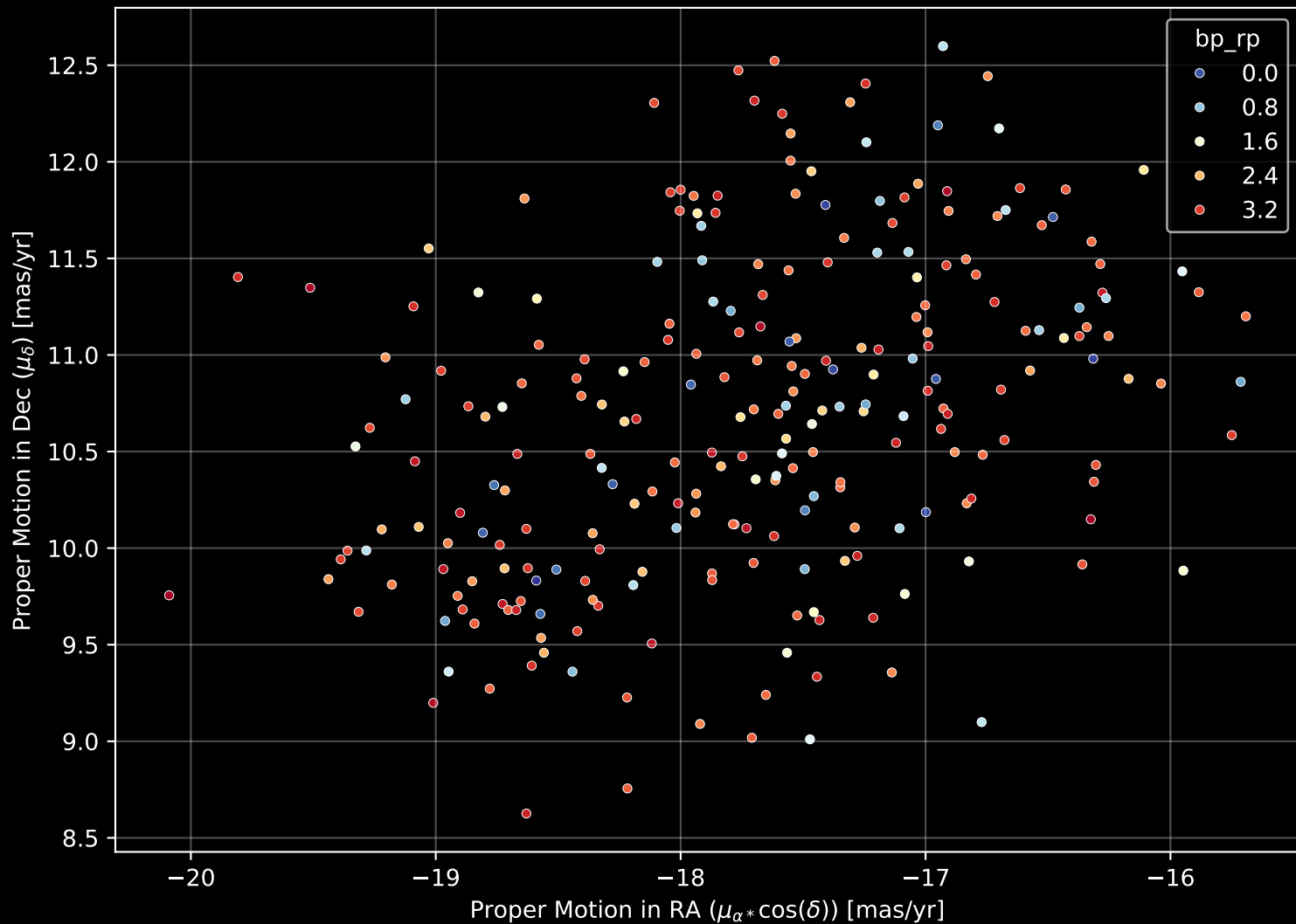
Gaia Cluster: [IC_2602] Proper Motion Diagram (n= 252)
