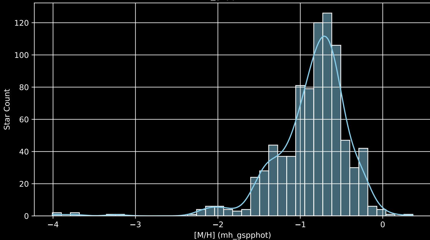
Gaia Cluster: [IC_2714 [M/H] (mh_gspphot) (n= 847)
