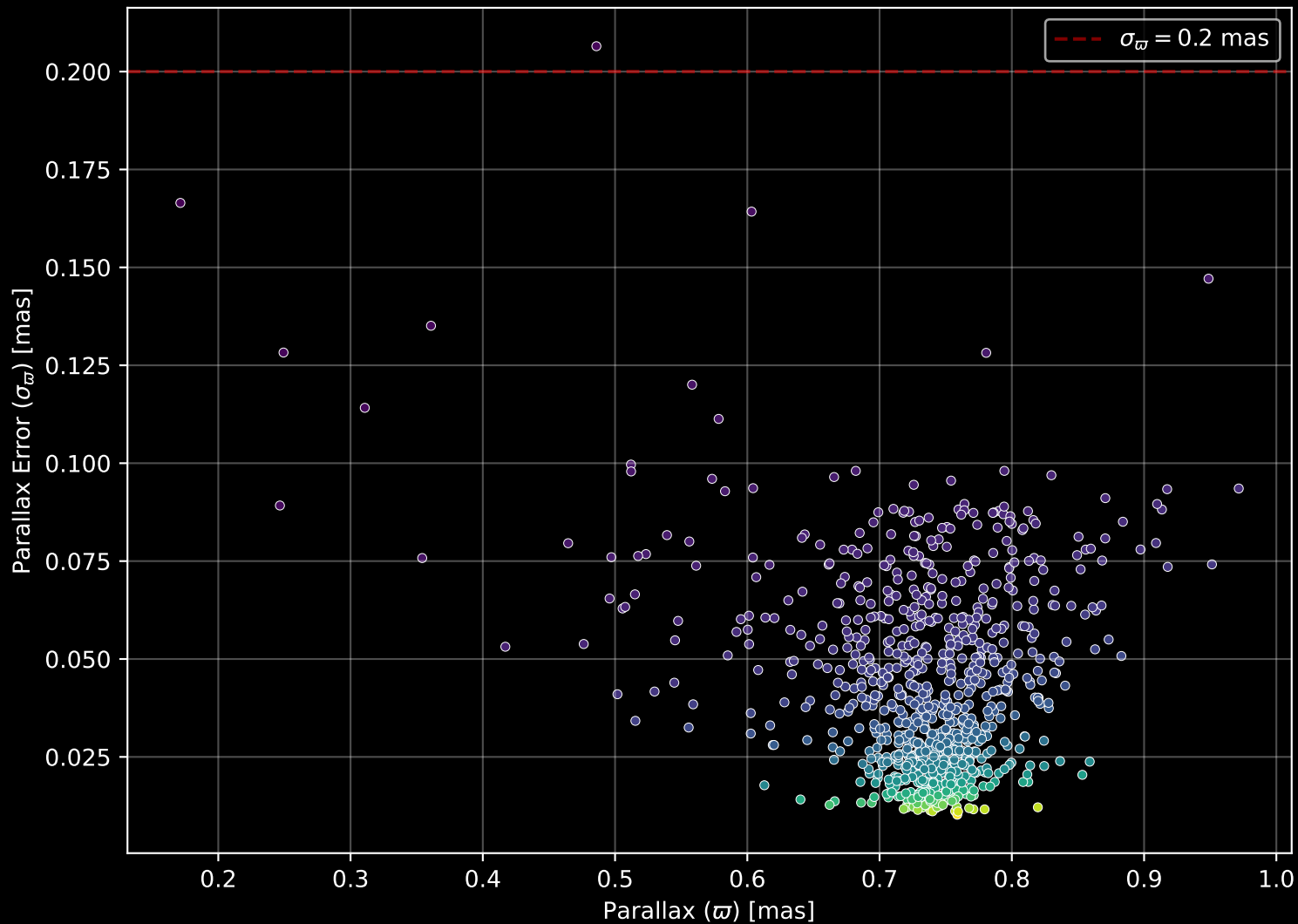
Gaia Cluster: [IC_2714] Parallax Quality (n= 848)
