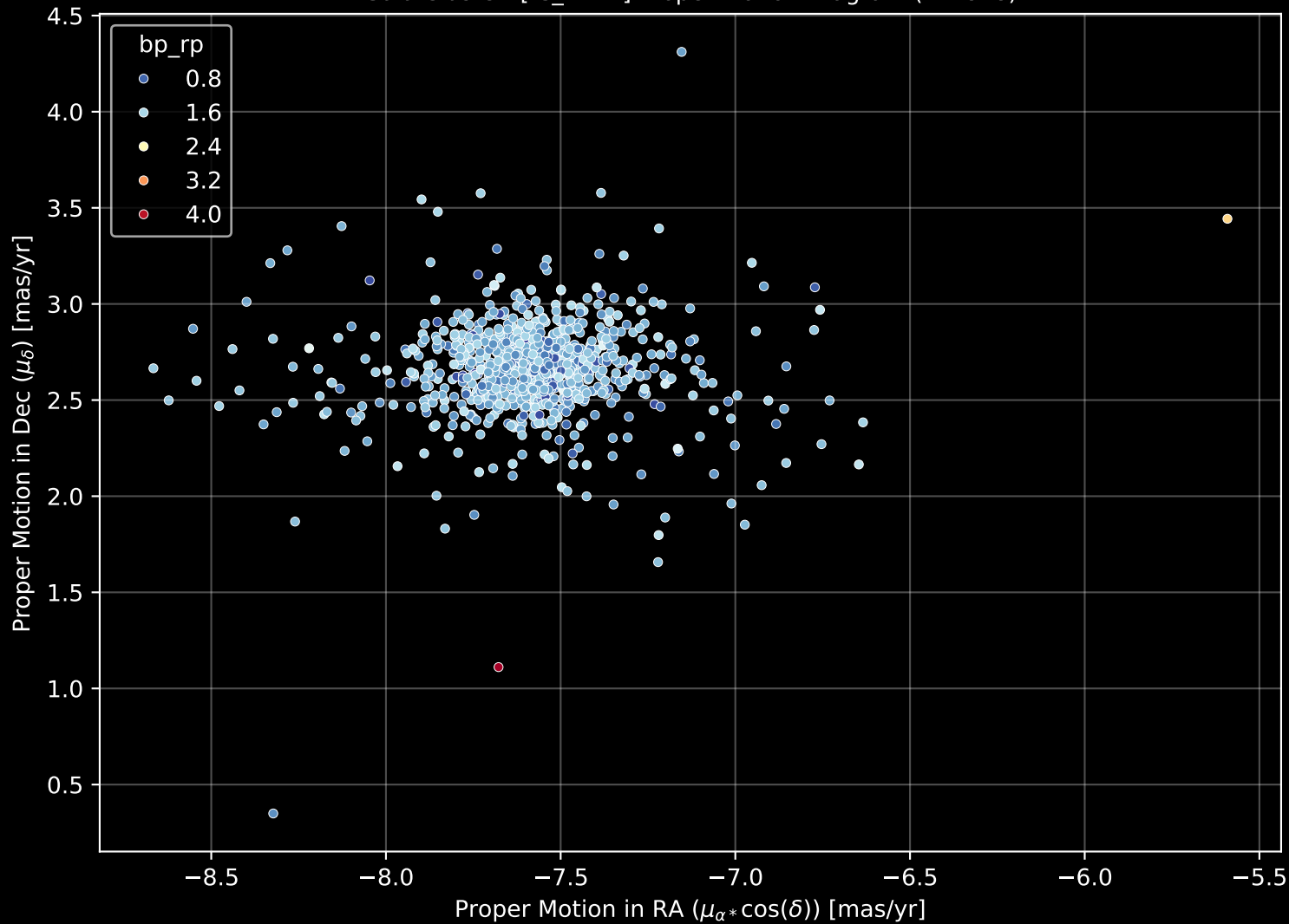
Gaia Cluster: [IC_2714] Proper Motion Diagram (n= 848)
