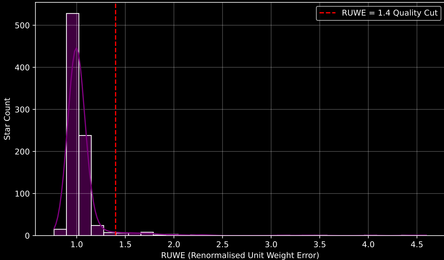
Gaia Cluster: [IC_2714] RUWE Distribution (n= 846)
