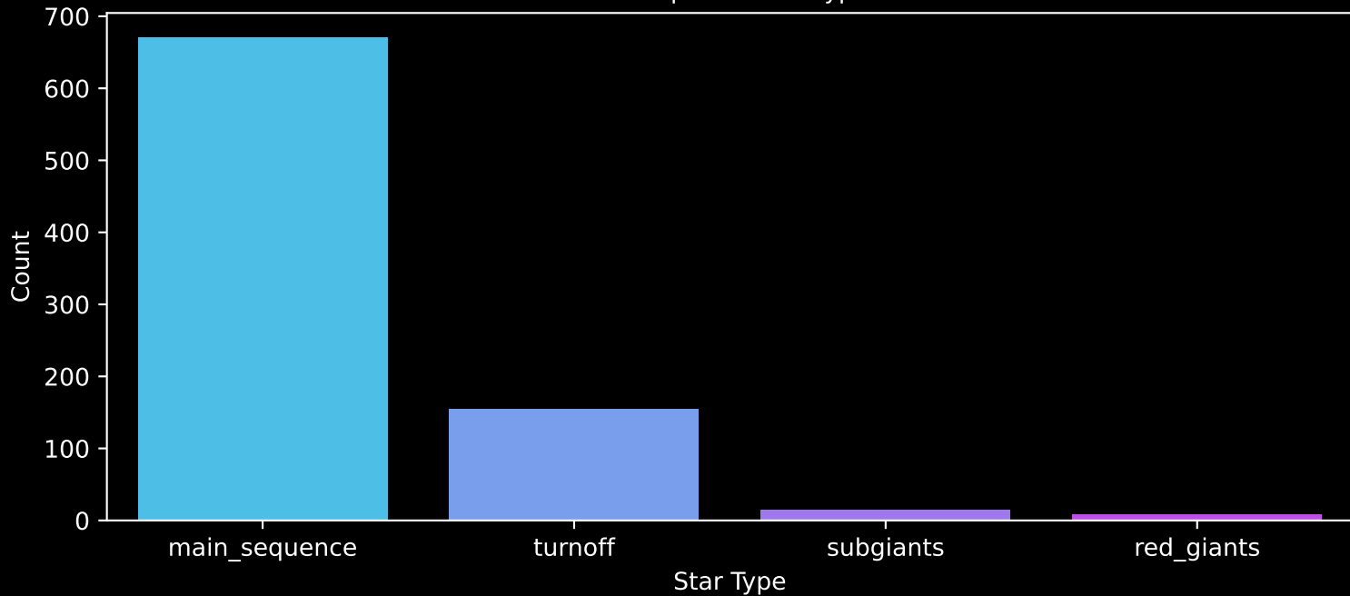
Gaia Cluster: [IC_2714] Count plot of Star Type
