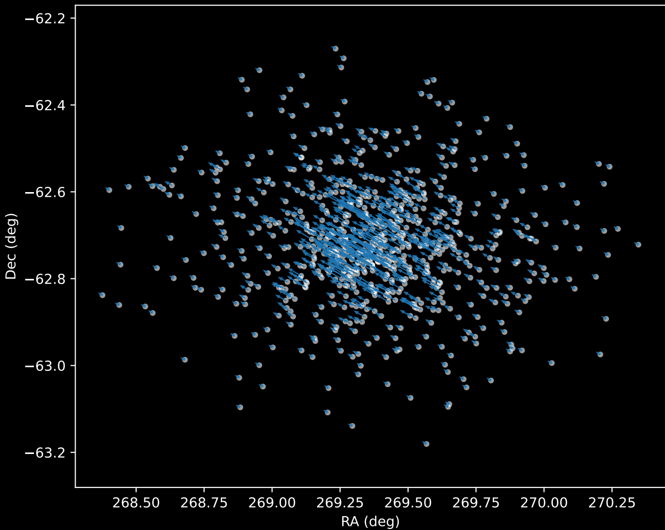
Gaia DR3 Cluster 0 Proper Motion Vectors (n=744)
