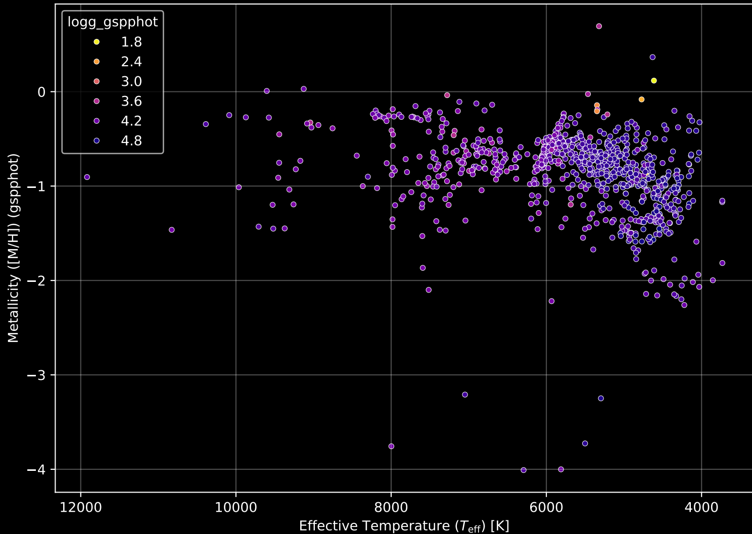
Gaia Cluster: [IC_2714] Stellar Population Parameters (n= 848)
