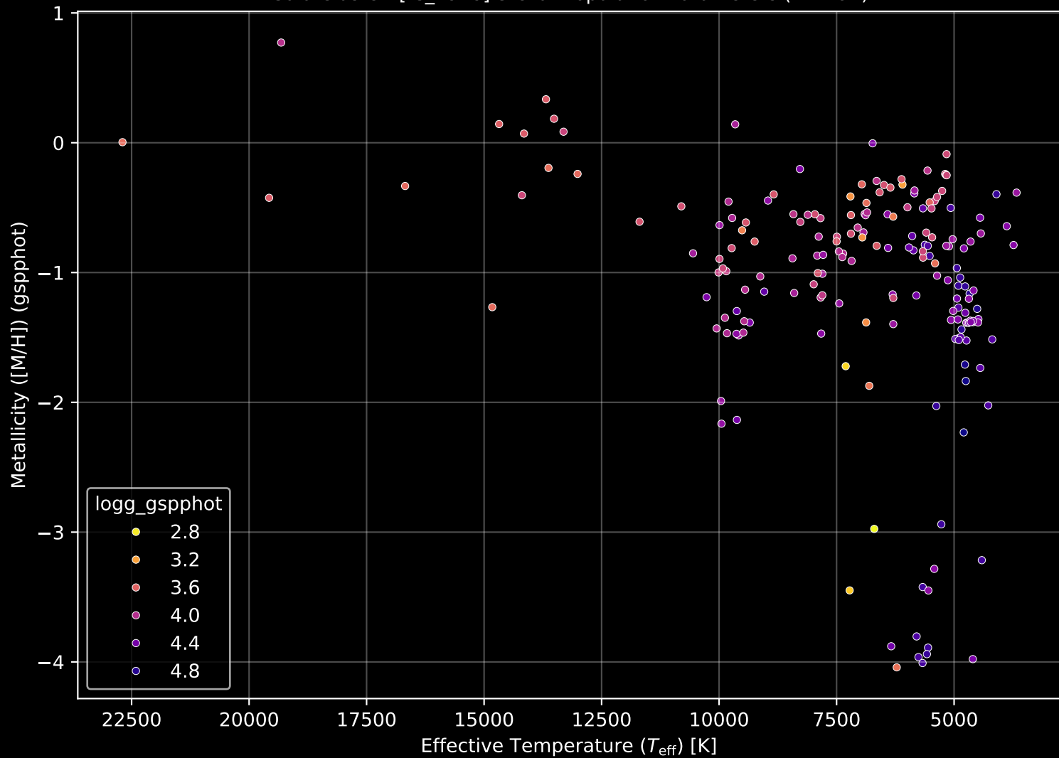
Gaia Cluster: [IC_2948] Stellar Population Parameters (n= 191)
