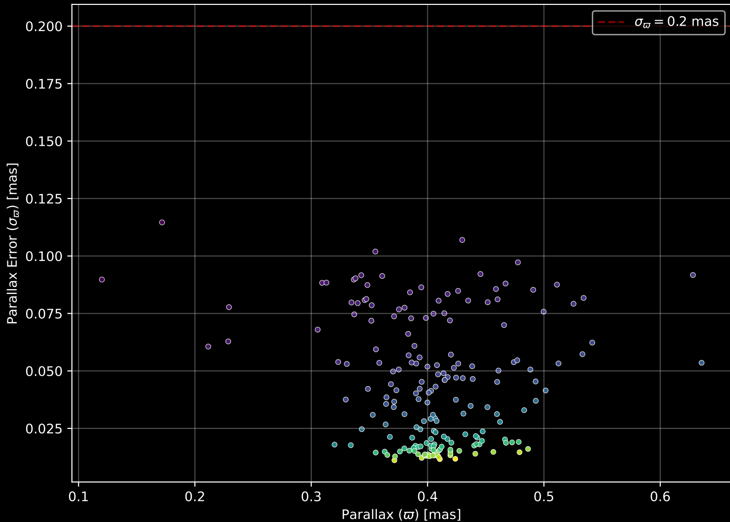
Gaia Cluster: [IC_2948] Parallax Quality (n= 191)
