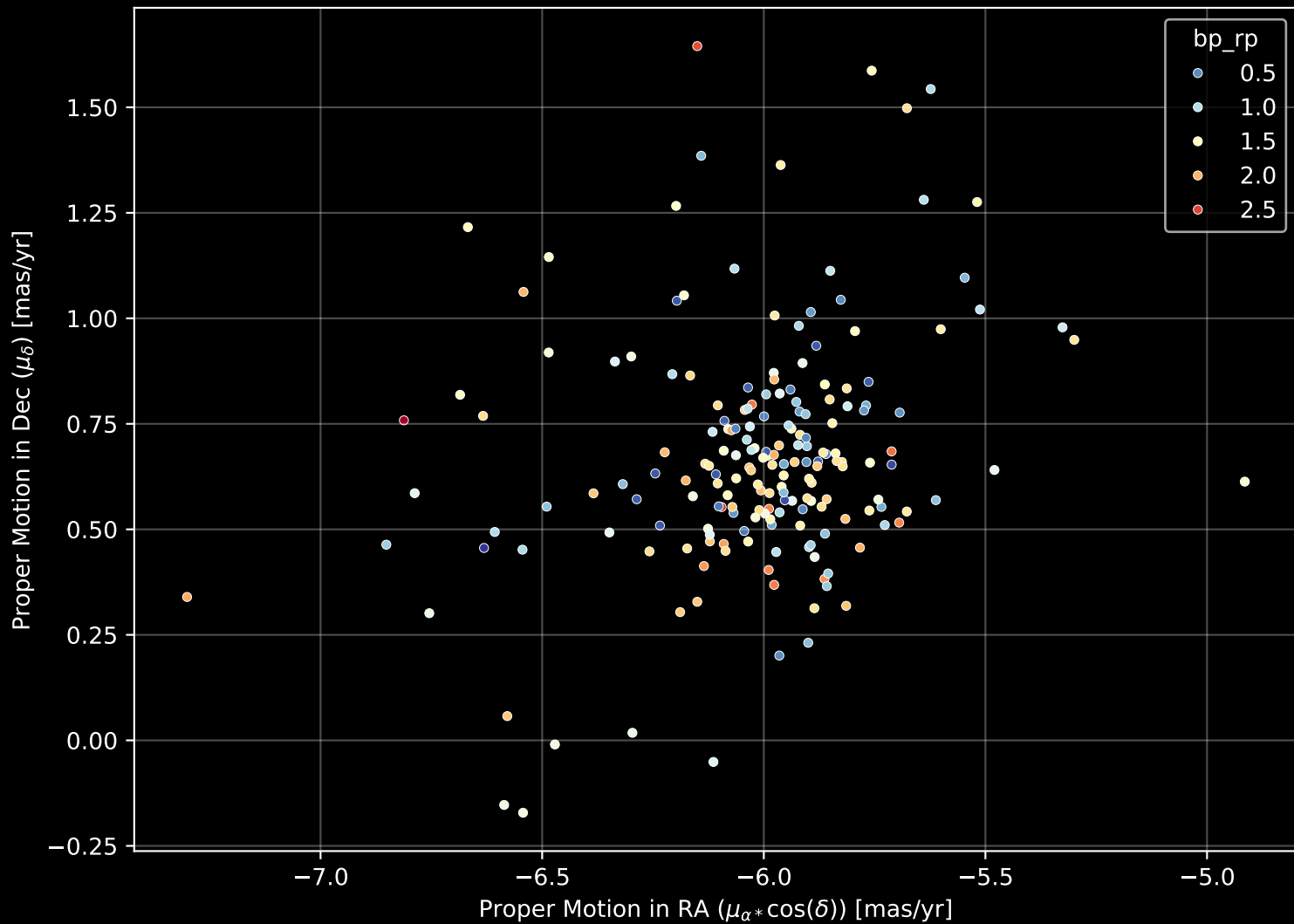
Gaia Cluster: [IC_2948] Proper Motion Diagram (n= 191)
