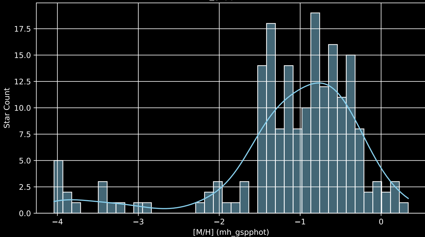
Gaia Cluster: [IC_2948 [M/H] (mh_gspphot) (n= 190)
