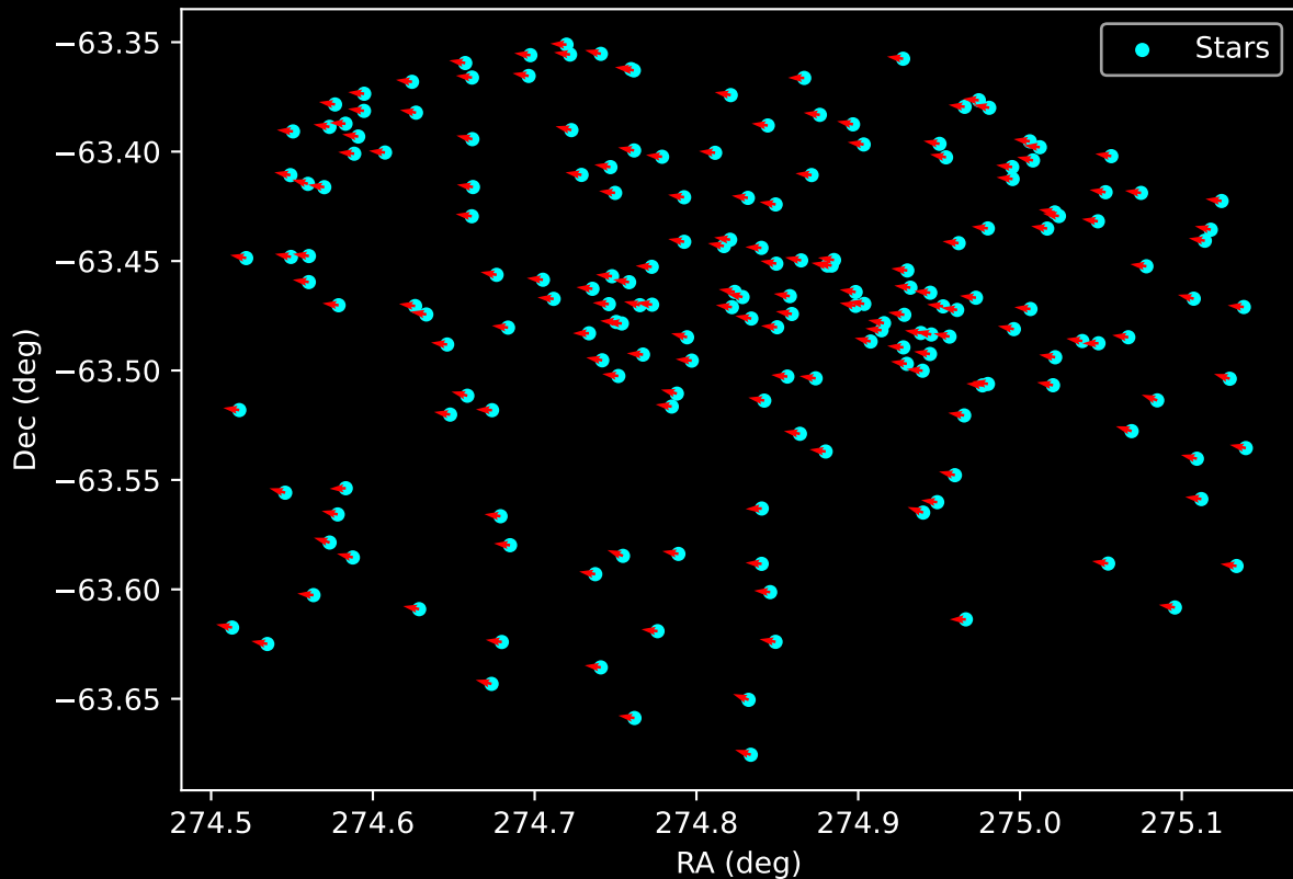
Gaia Cluster: [IC_2948] Proper Motion Vectors for Gaia Star Field (n= 191)
