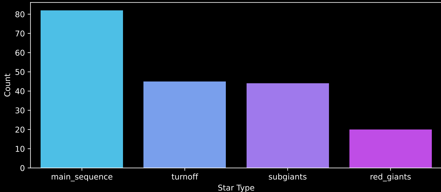
Gaia Cluster: [IC_2948] Count plot of Star Type
