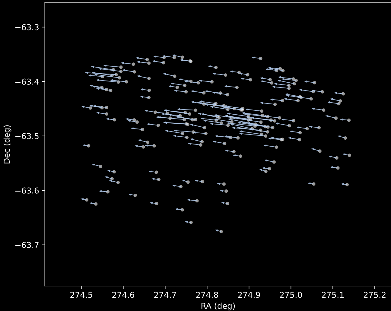
Gaia DR3 Cluster 1 Proper Motion Vectors (n=180)
