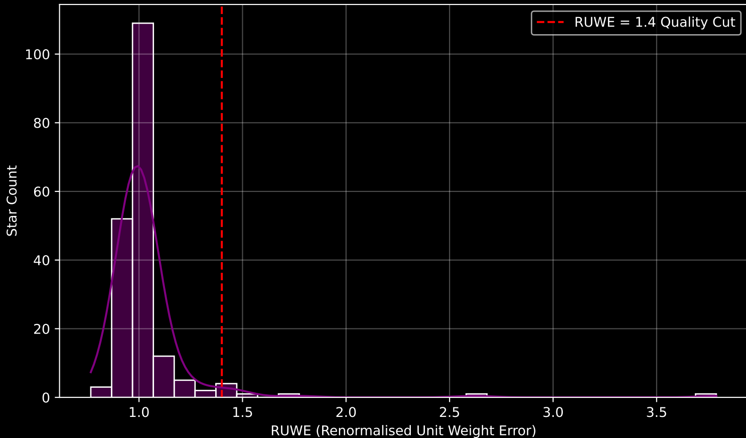
Gaia Cluster: [IC_2948] RUWE Distribution (n= 191)
