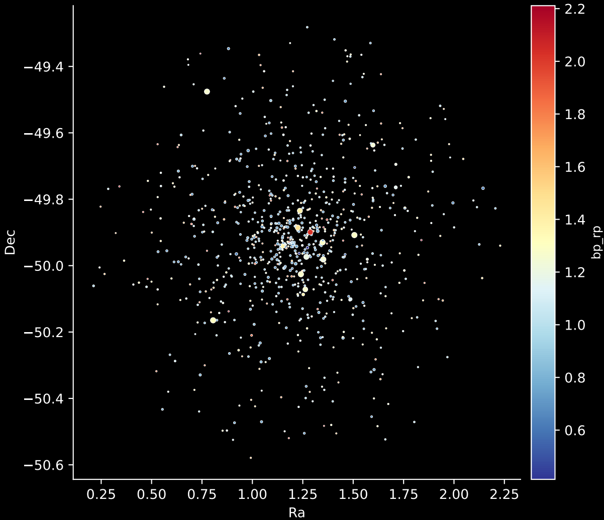
Gaia Cluster: [IC_4651] Stars: 835
