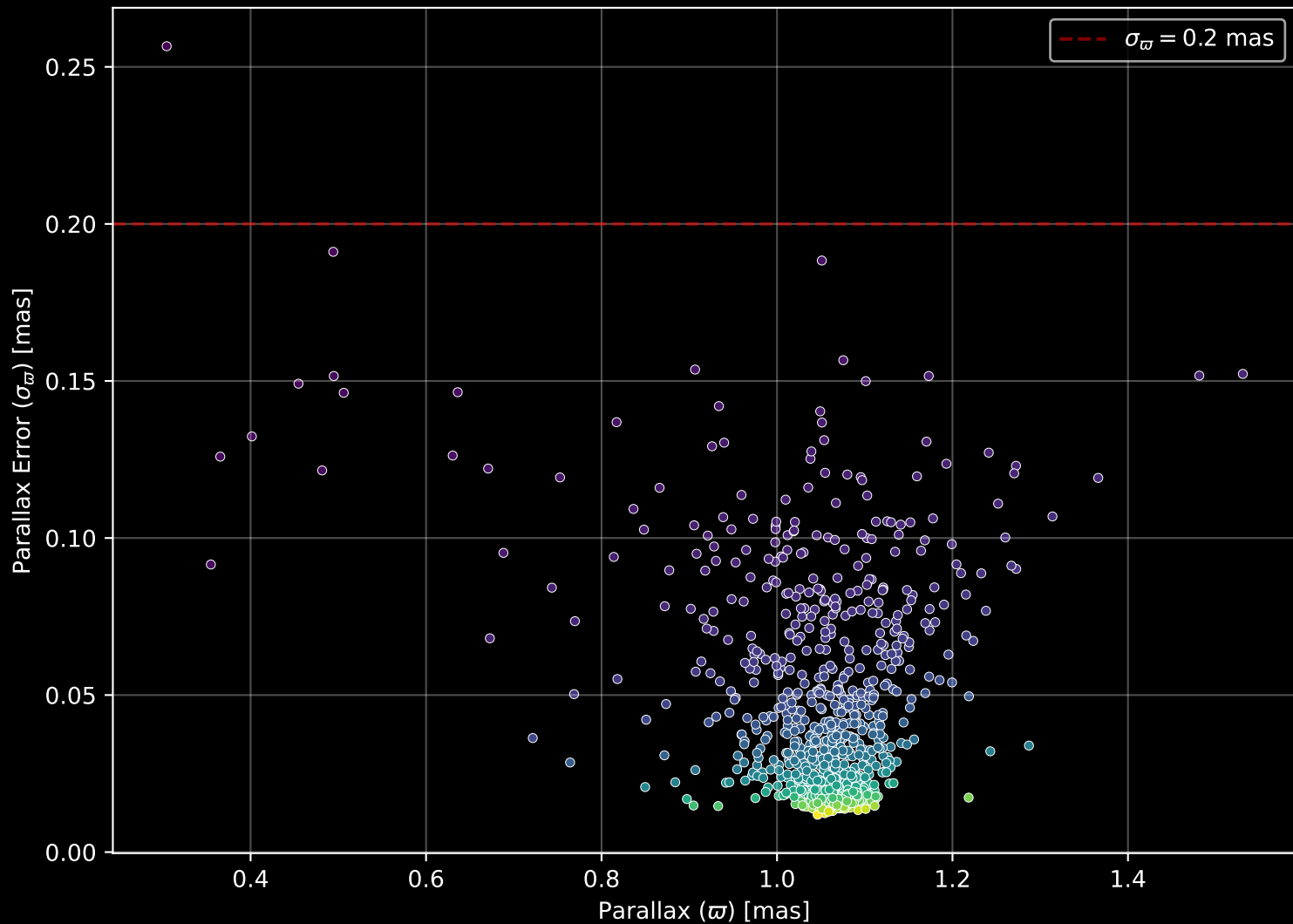
Gaia Cluster: [IC_4651] Parallax Quality (n= 835)
