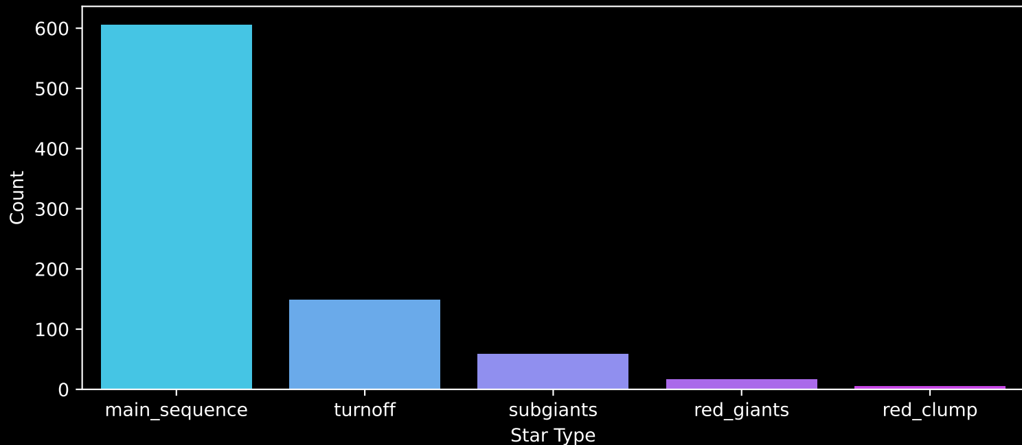
Gaia Cluster: [IC_4651] Count plot of Star Type
