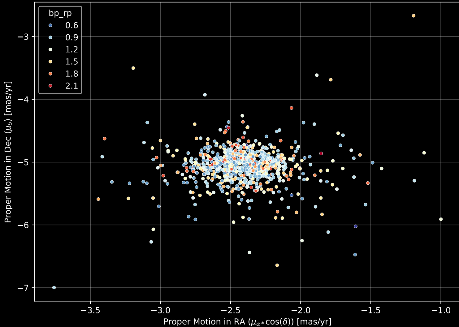
Gaia Cluster: [IC_4651] Proper Motion Diagram (n= 835)
