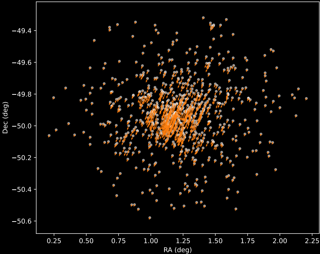
Gaia DR3 Cluster 2 Proper Motion Vectors (n=720)
