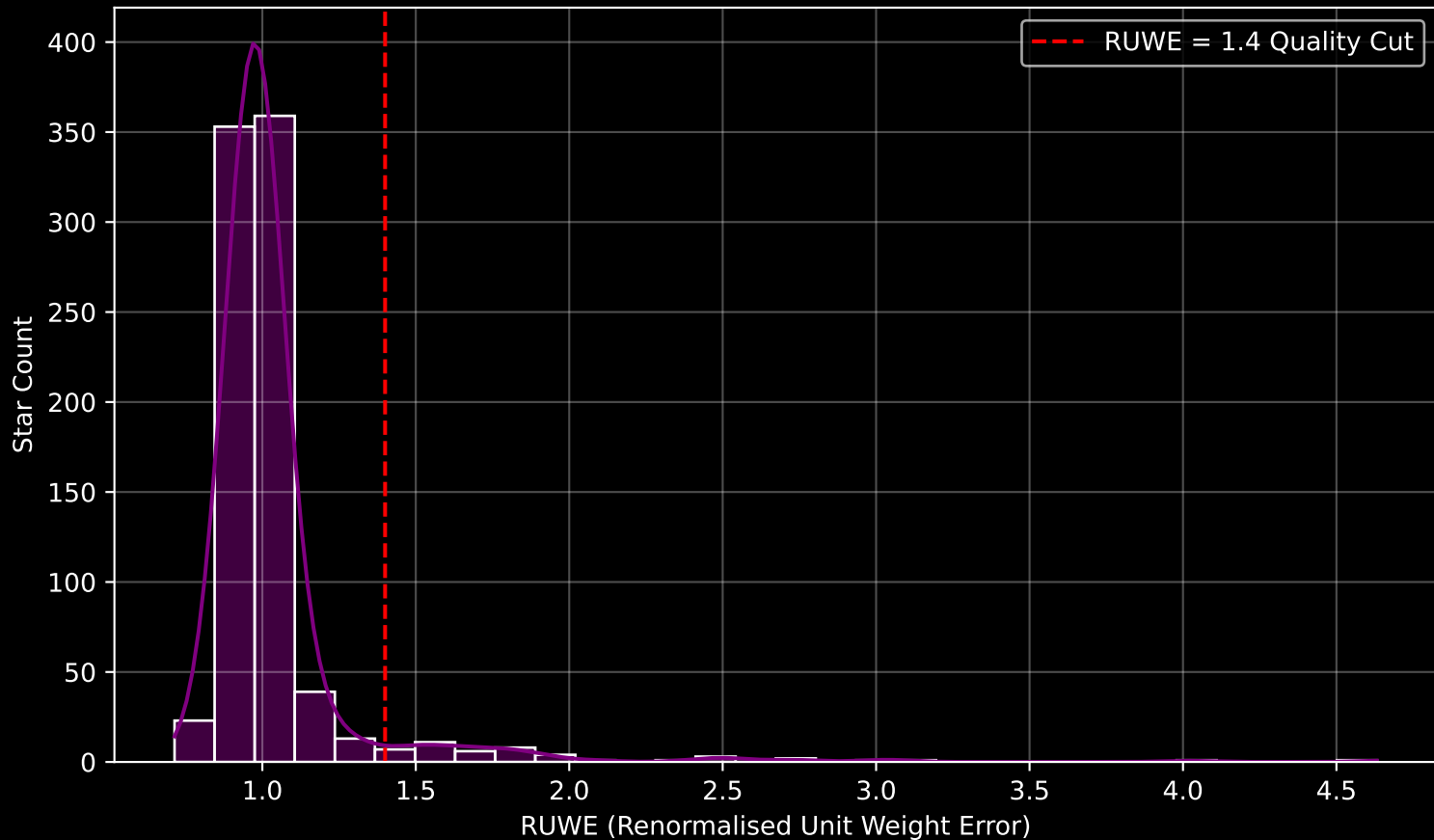
Gaia Cluster: [IC_4651] RUWE Distribution (n= 834)
