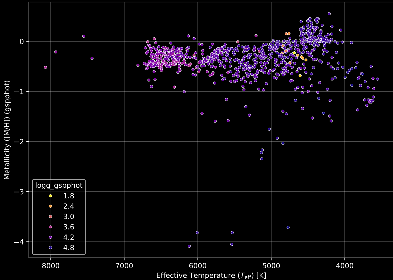
Gaia Cluster: [IC_4651] Stellar Population Parameters (n= 835)
