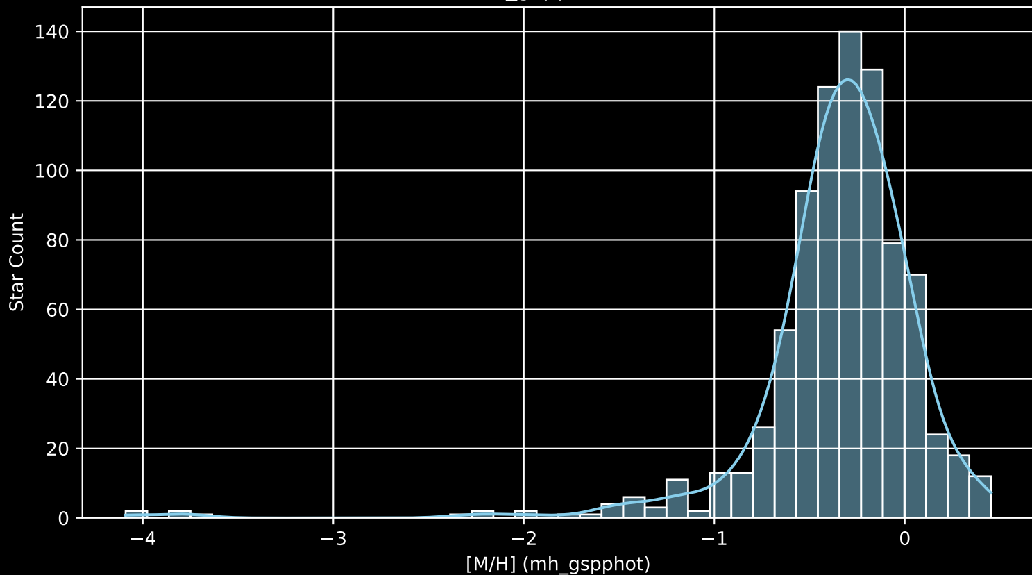
Gaia Cluster: [IC_4651 [M/H] (mh_gspphot) (n= 834)
