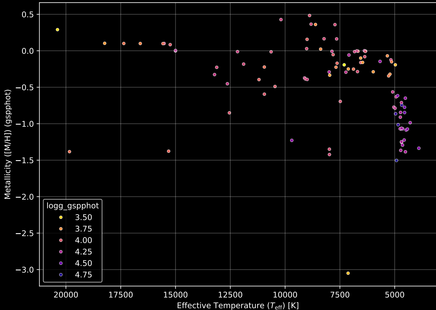
Gaia Cluster: [IC_4996] Stellar Population Parameters (n= 99)
