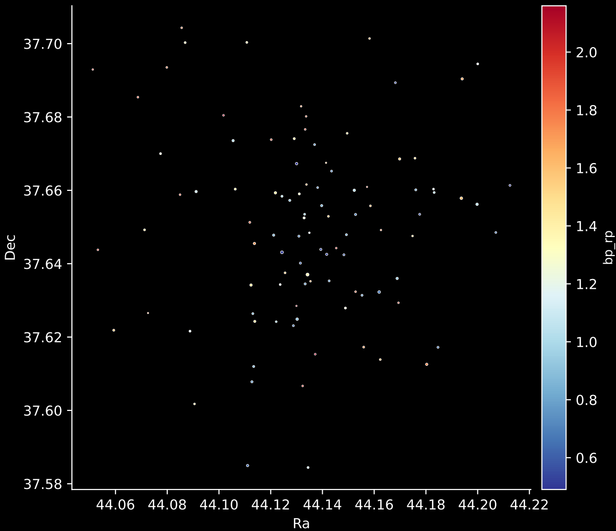
Gaia Cluster: [IC_4996] Stars: 99
