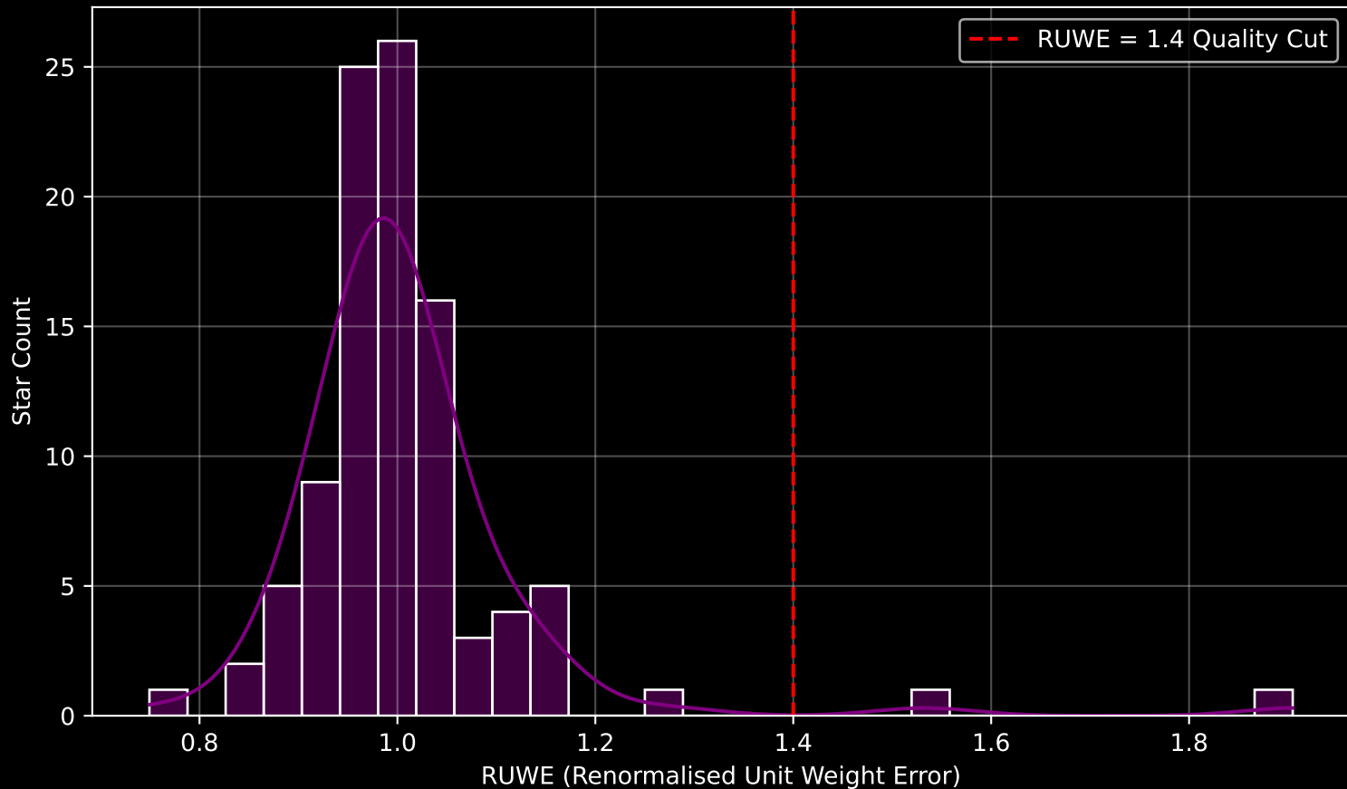
Gaia Cluster: [IC_4996] RUWE Distribution (n= 99)
