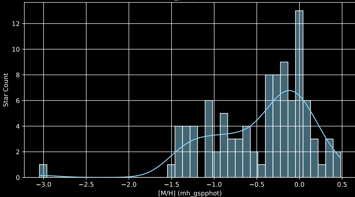
Gaia Cluster: [IC_4996 [M/H] (mh_gspphot) (n= 99)
