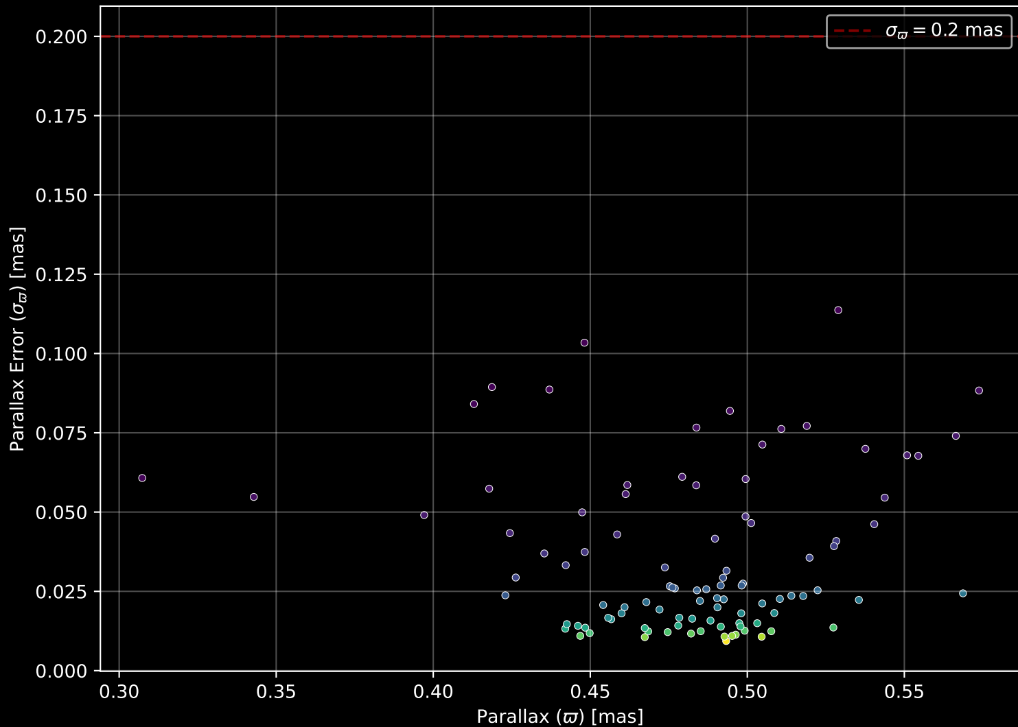
Gaia Cluster: [IC_4996] Parallax Quality (n= 99)
