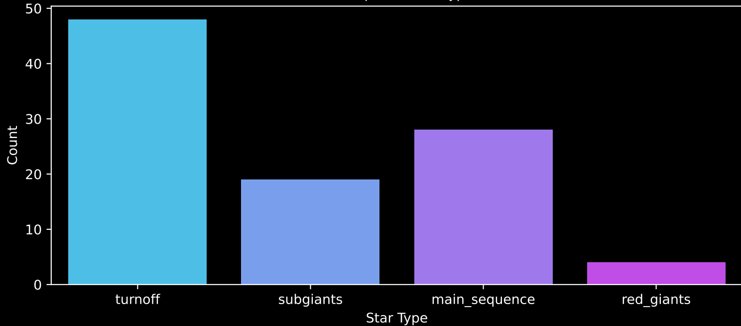
Gaia Cluster: [IC_4996] Count plot of Star Type
