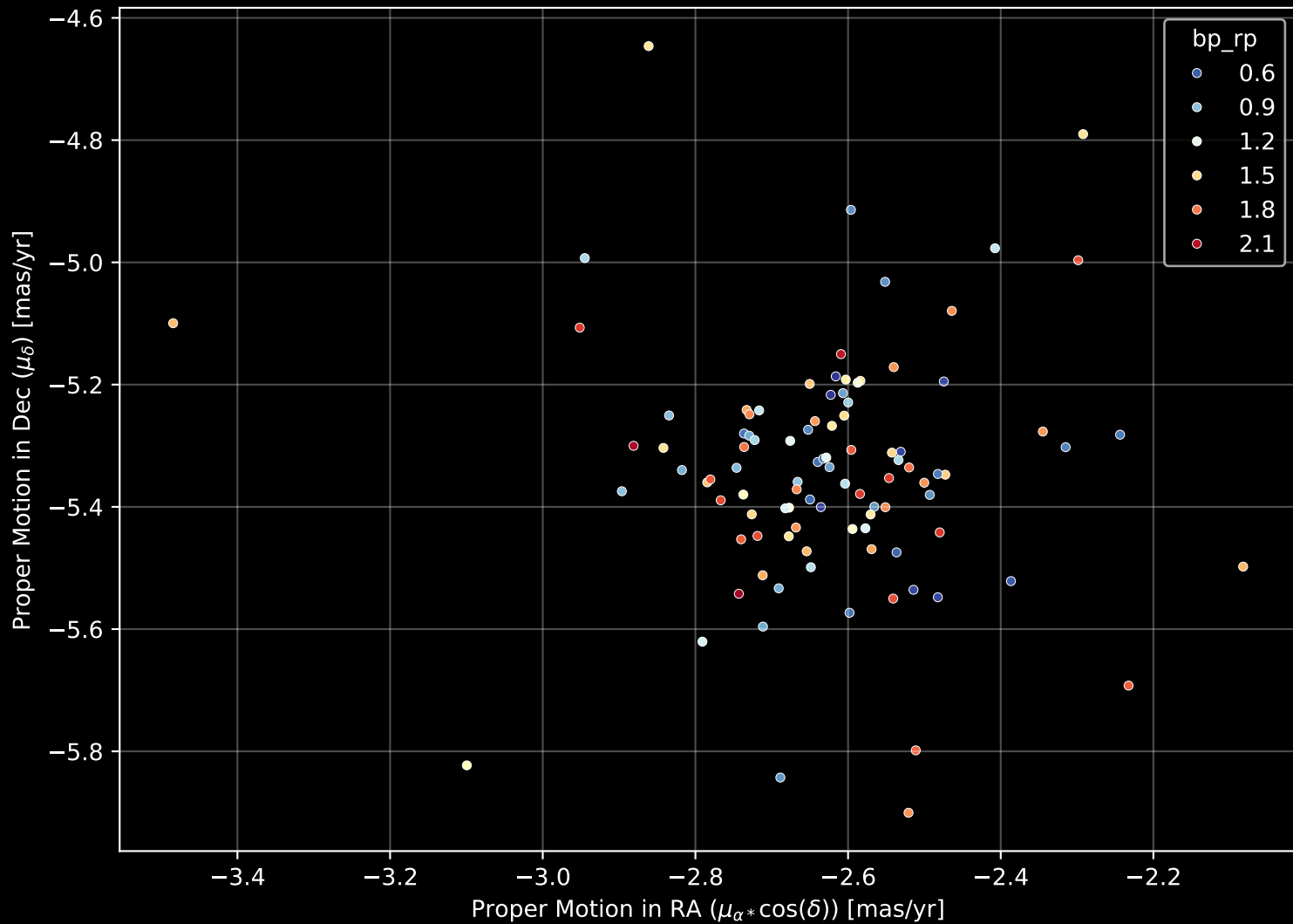
Gaia Cluster: [IC_4996] Proper Motion Diagram (n= 99)
