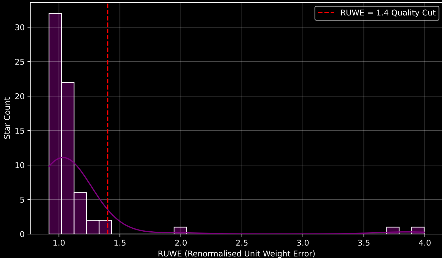
Gaia Cluster: [Ivanov_4] RUWE Distribution (n= 67)
