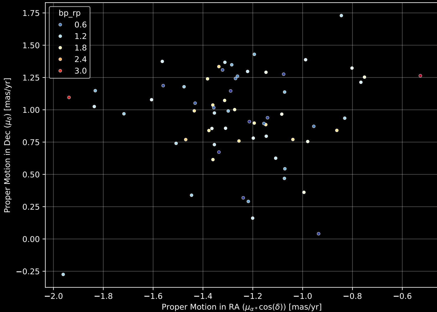
Gaia Cluster: [Ivanov_4] Proper Motion Diagram (n= 67)
