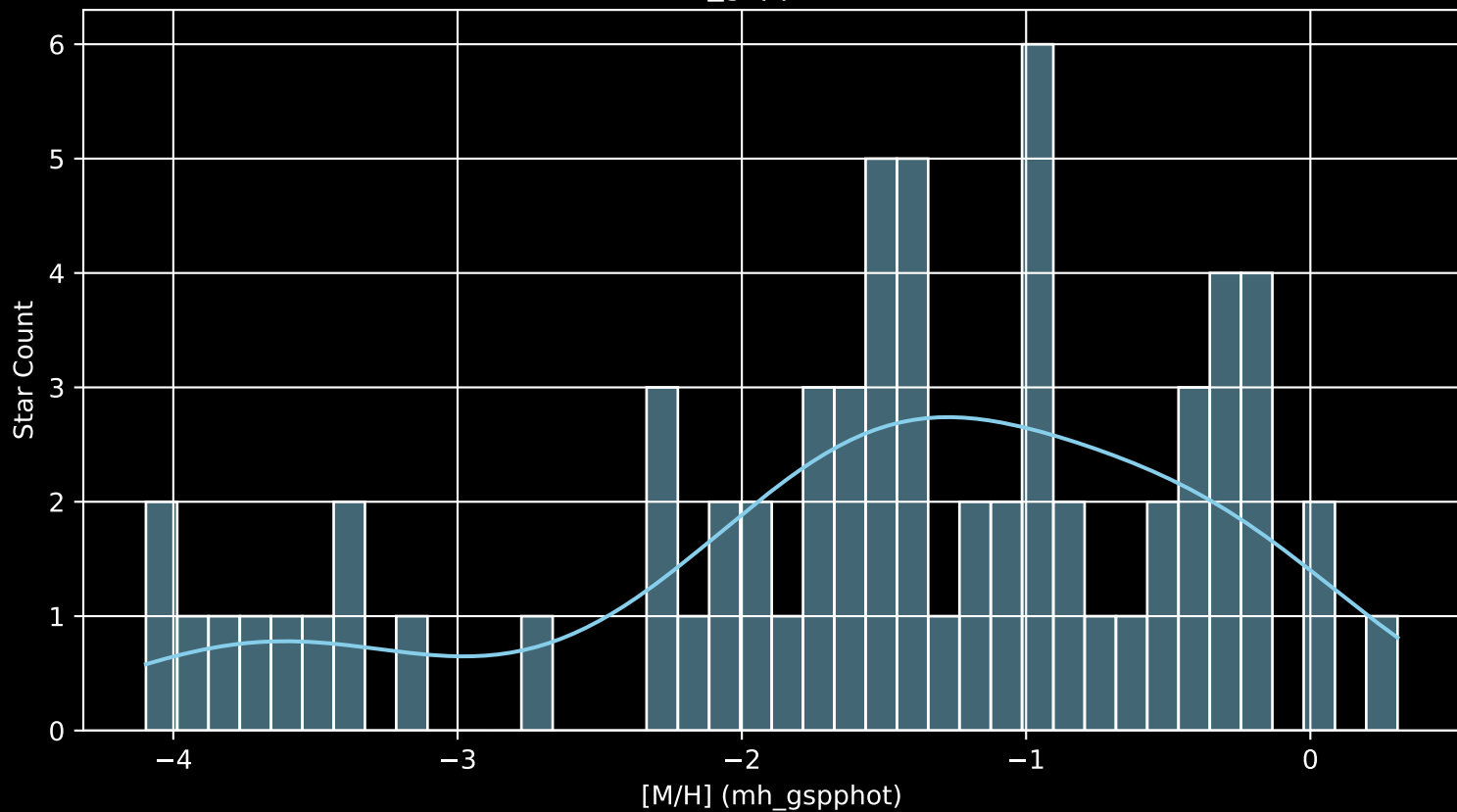
Gaia Cluster: [Ivanov_4 [M/H] (mh_gspphot) (n= 67)
