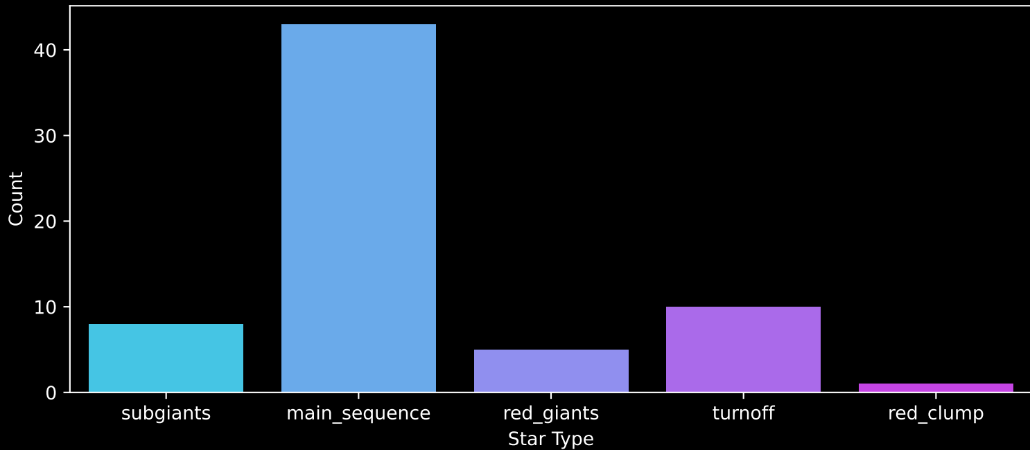
Gaia Cluster: [Ivanov_4] Count plot of Star Type
