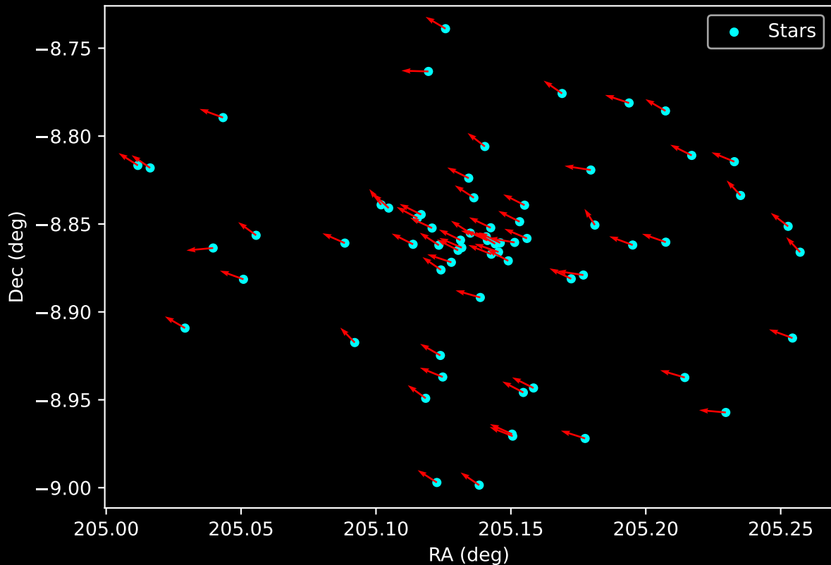
Gaia Cluster: [Ivanov_4] Proper Motion Vectors for Gaia Star Field (n= 67)
