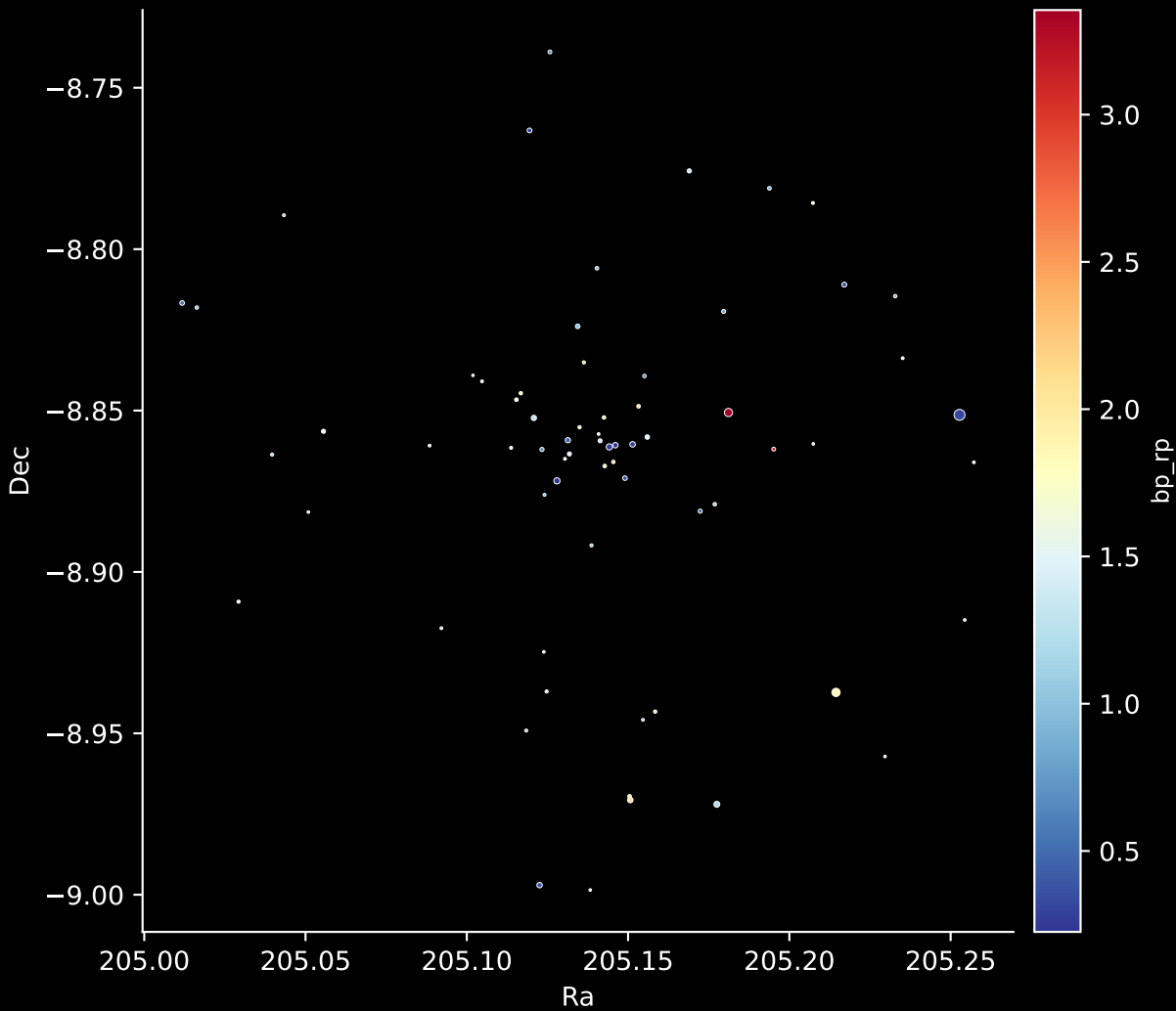
Gaia Cluster: [Ivanov_4] Stars: 67
