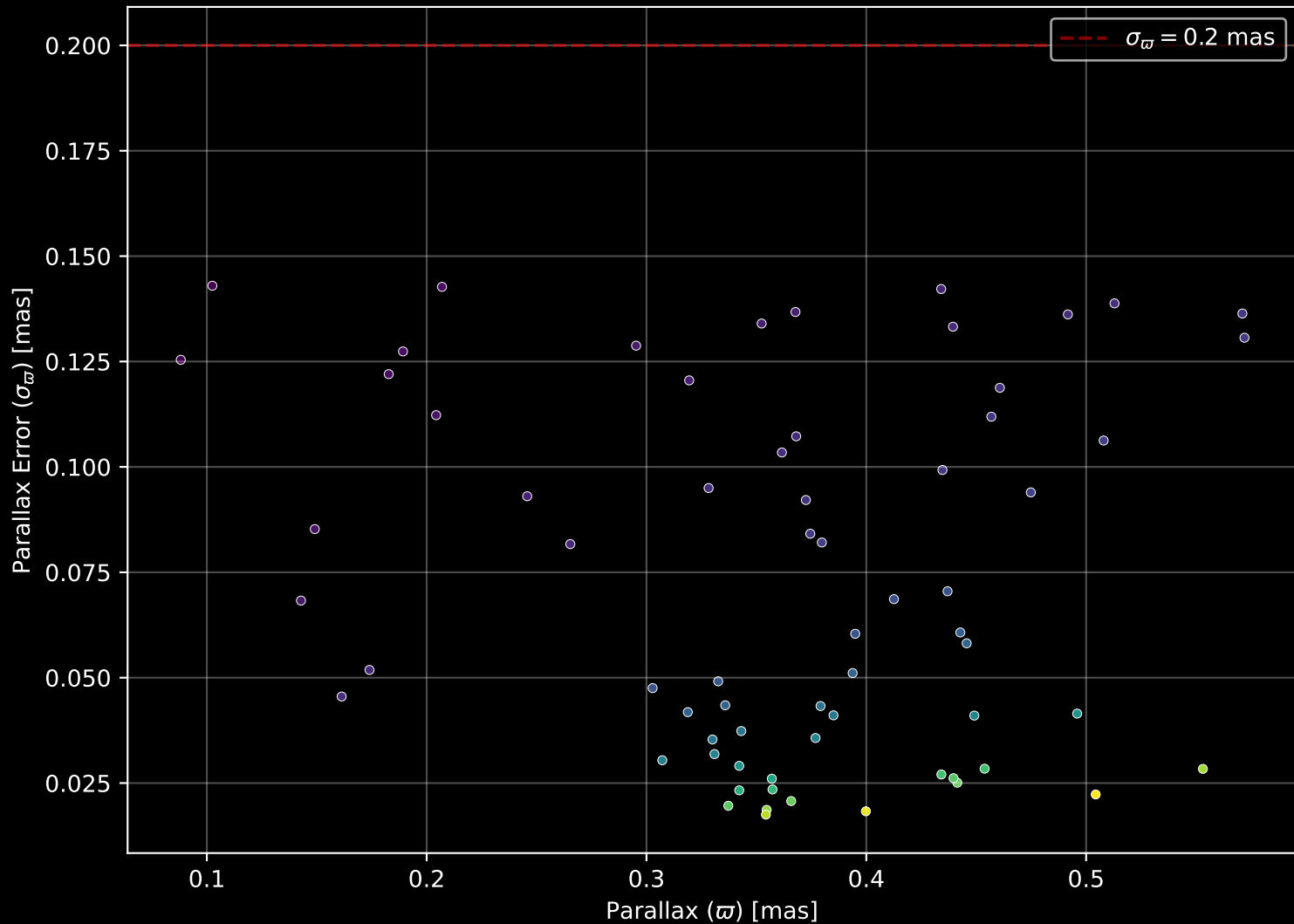
Gaia Cluster: [Ivanov_4] Parallax Quality (n= 67)
