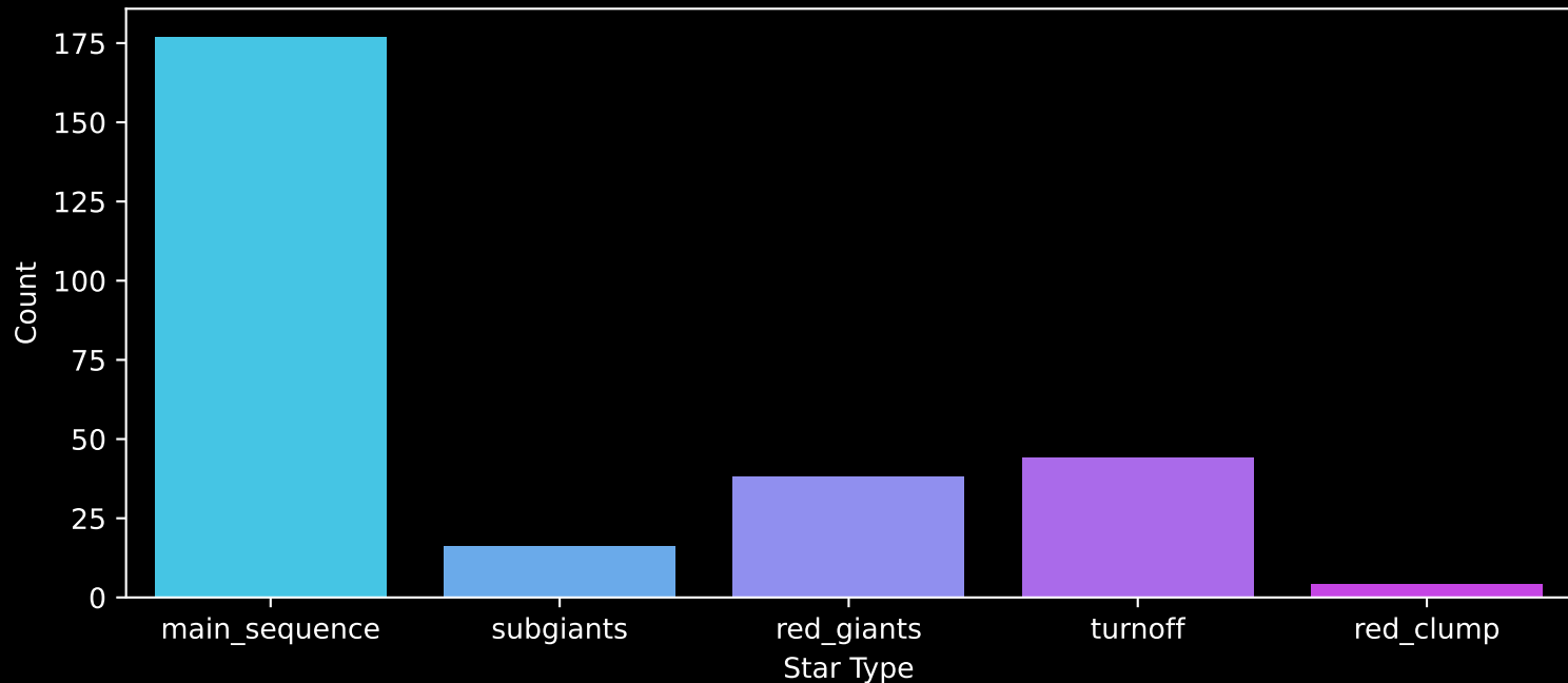
Gaia Cluster: [Juchert_13] Count plot of Star Type
