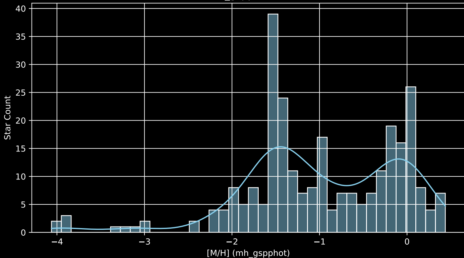
Gaia Cluster: [Juchert_13 [M/H] (mh_gspphot) (n= 273)
