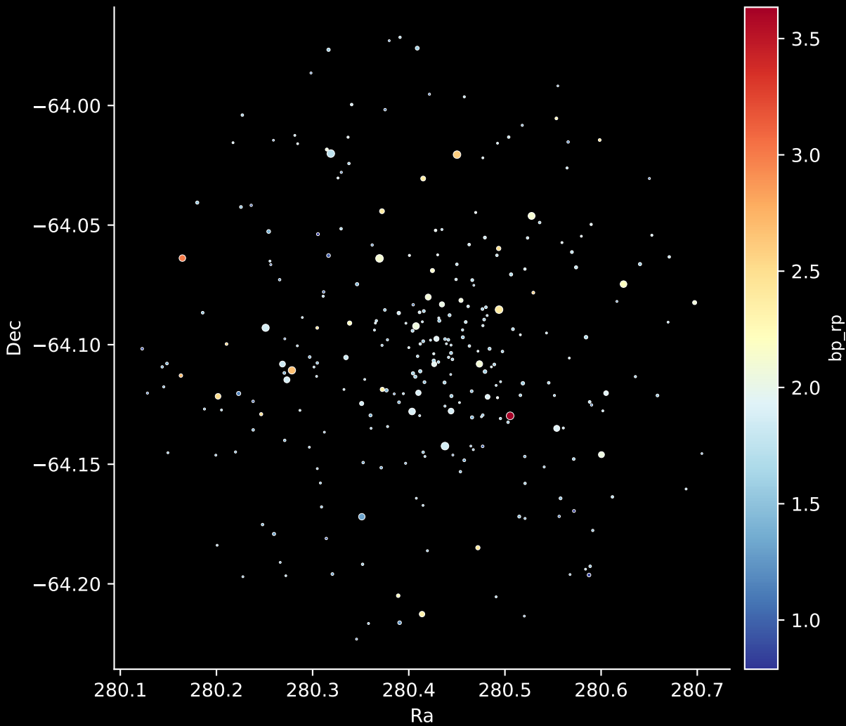
Gaia Cluster: [Juchert_13] Stars: 279
