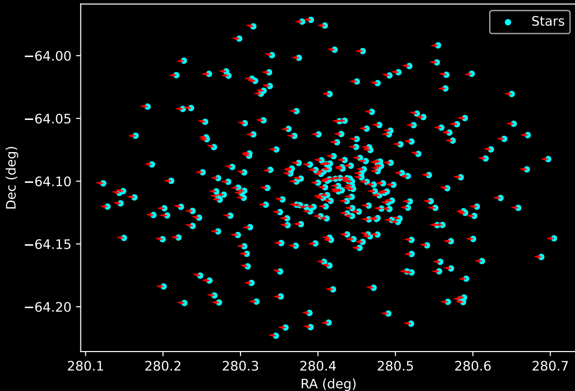
Gaia Cluster: [Juchert_13] Proper Motion Vectors for Gaia Star Field (n= 279)
