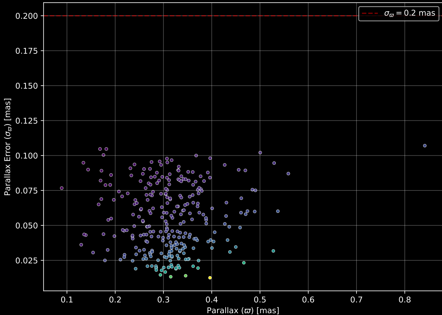
Gaia Cluster: [Juchert_13] Parallax Quality (n= 279)
