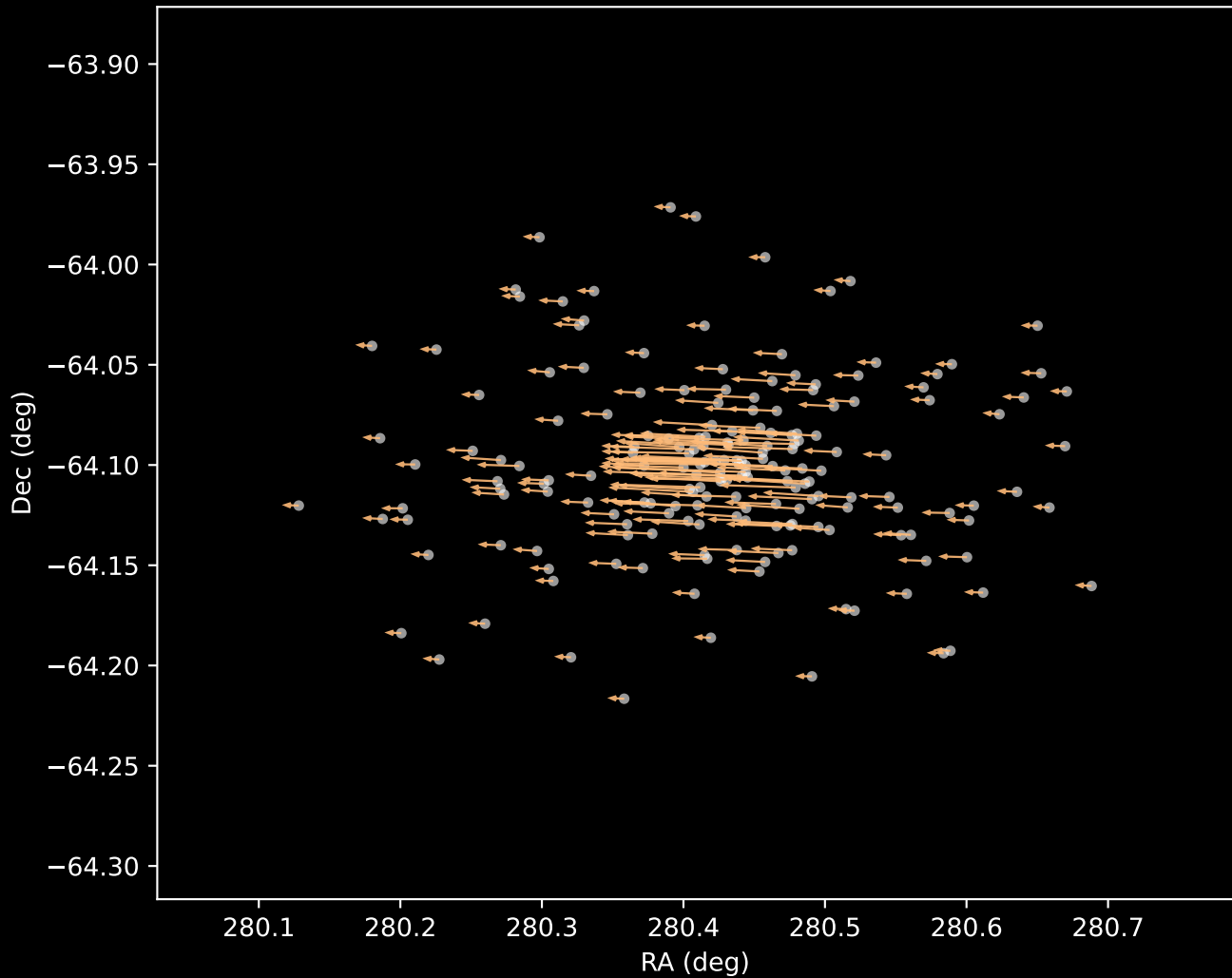
Gaia DR3 Cluster 3 Proper Motion Vectors (n=189)
