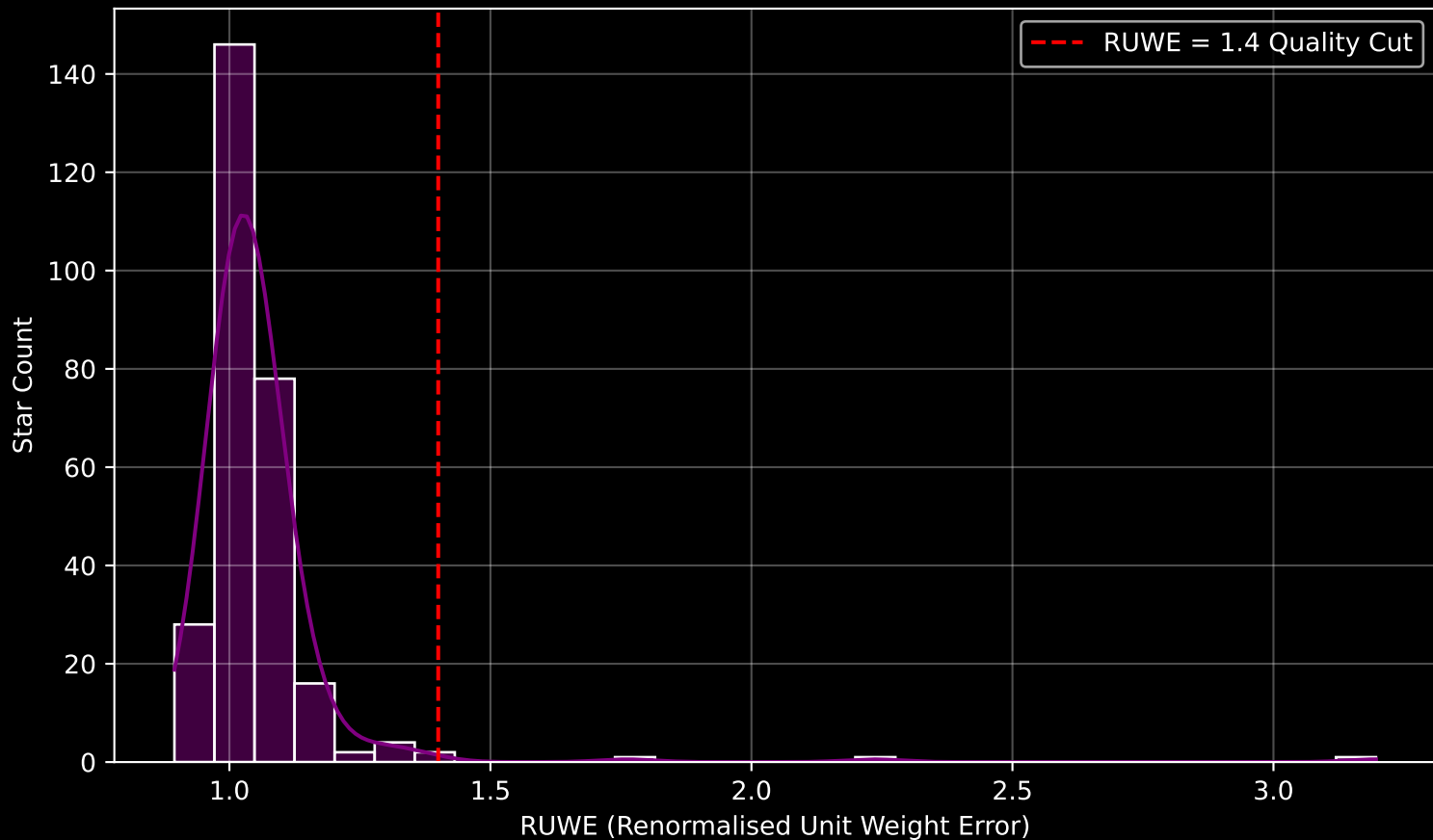
Gaia Cluster: [Juchert_13] RUWE Distribution (n= 279)
