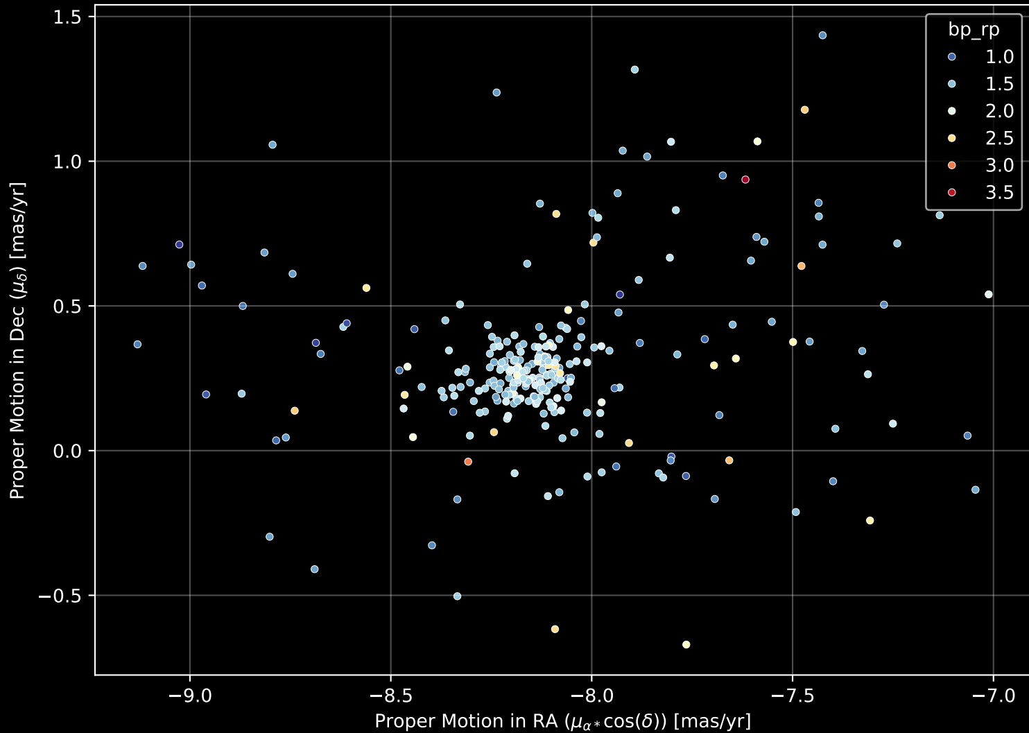
Gaia Cluster: [Juchert_13] Proper Motion Diagram (n= 279)
