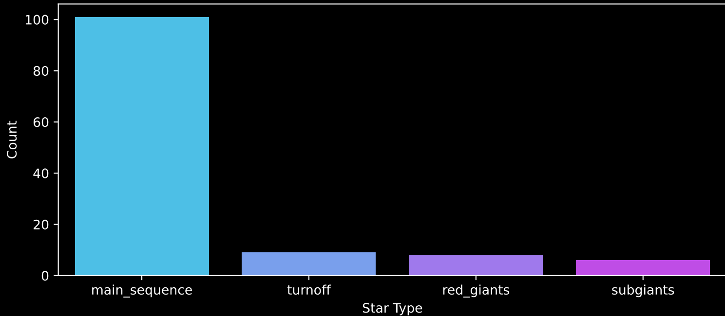
Gaia Cluster: [Juchert_20] Count plot of Star Type
