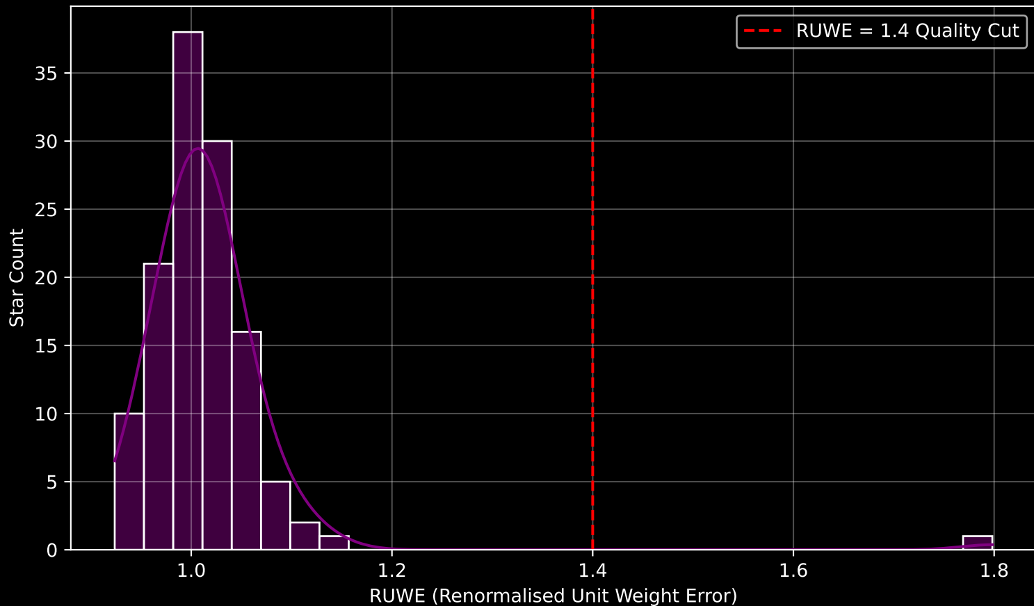
Gaia Cluster: [Juchert_20] RUWE Distribution (n= 124)
