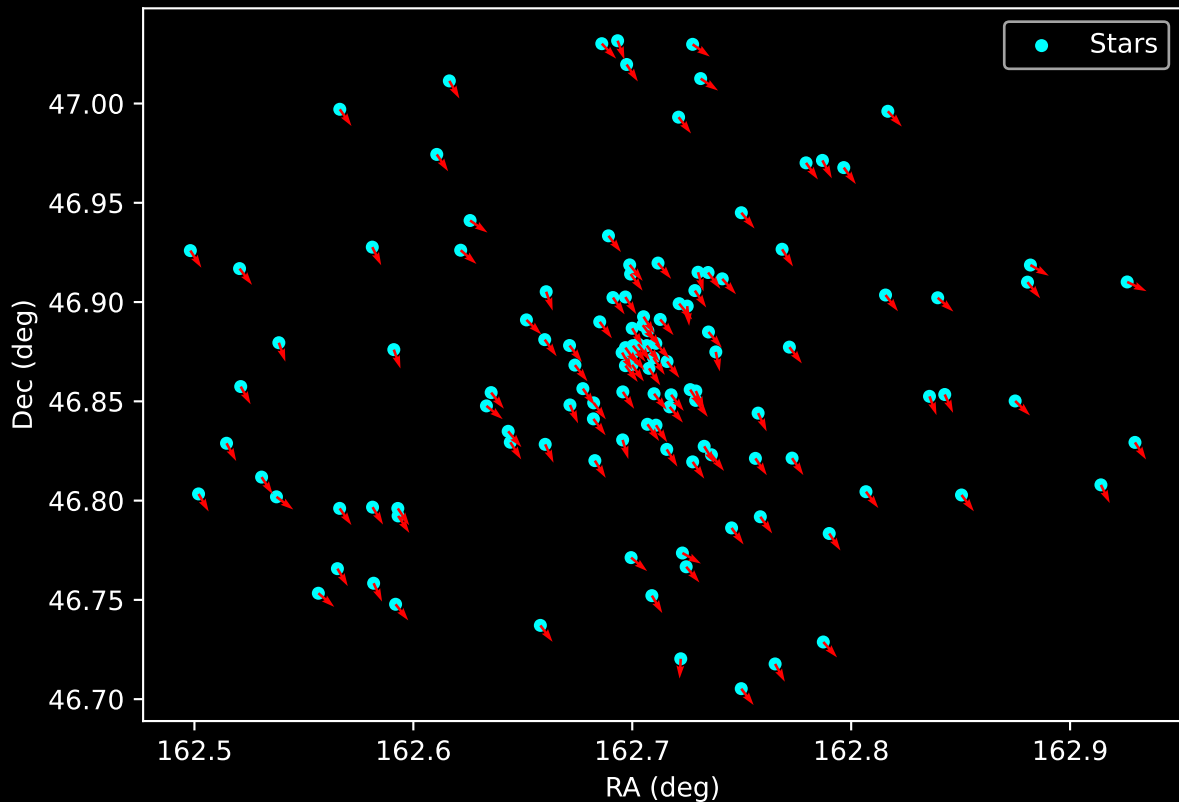
Gaia Cluster: [Juchert_20] Proper Motion Vectors for Gaia Star Field (n= 124)
