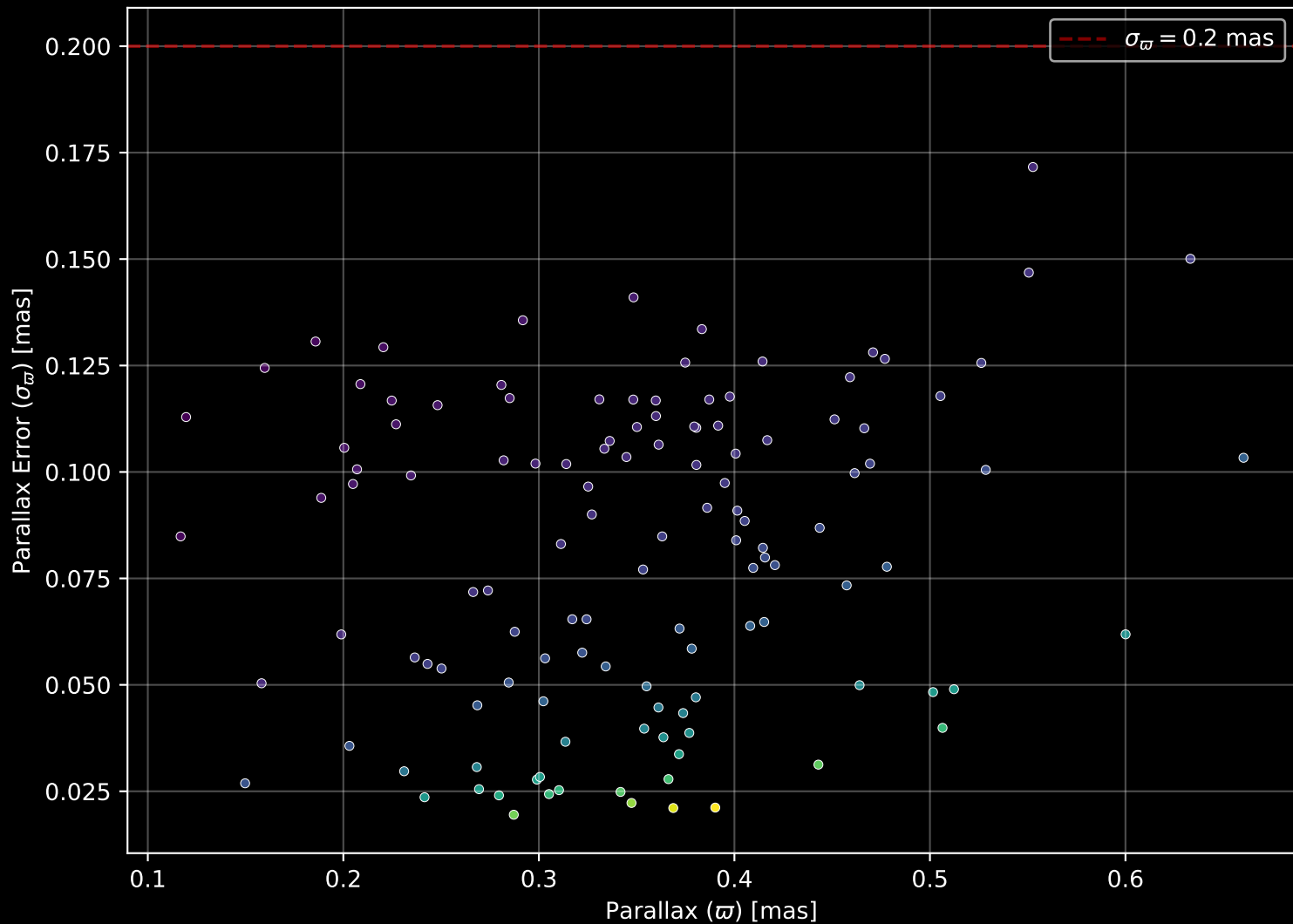
Gaia Cluster: [Juchert_20] Parallax Quality (n= 124)
