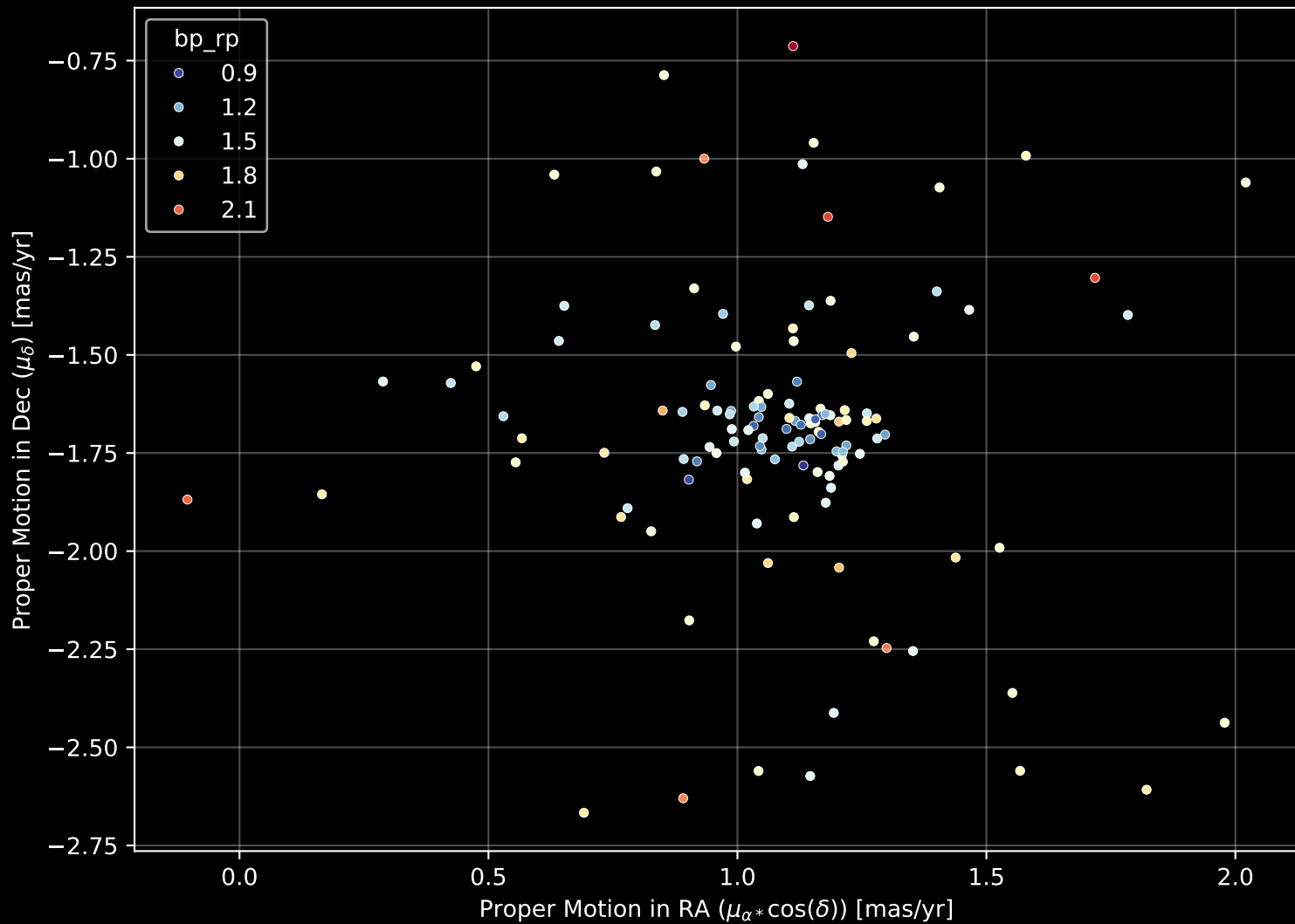
Gaia Cluster: [Juchert_20] Proper Motion Diagram (n= 124)
