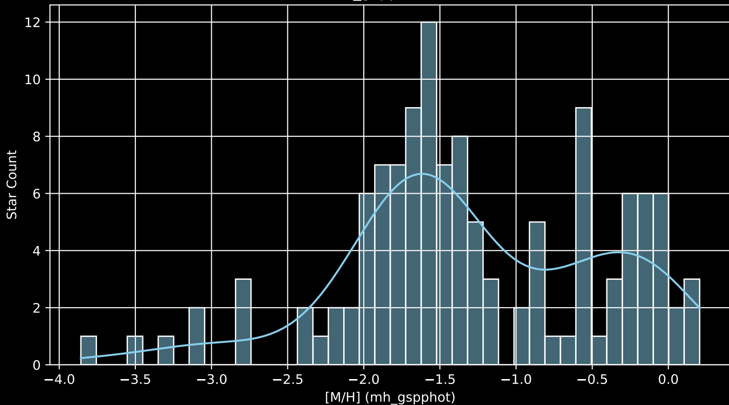
Gaia Cluster: [Juchert_20 [M/H] (mh_gspphot) (n= 124)
