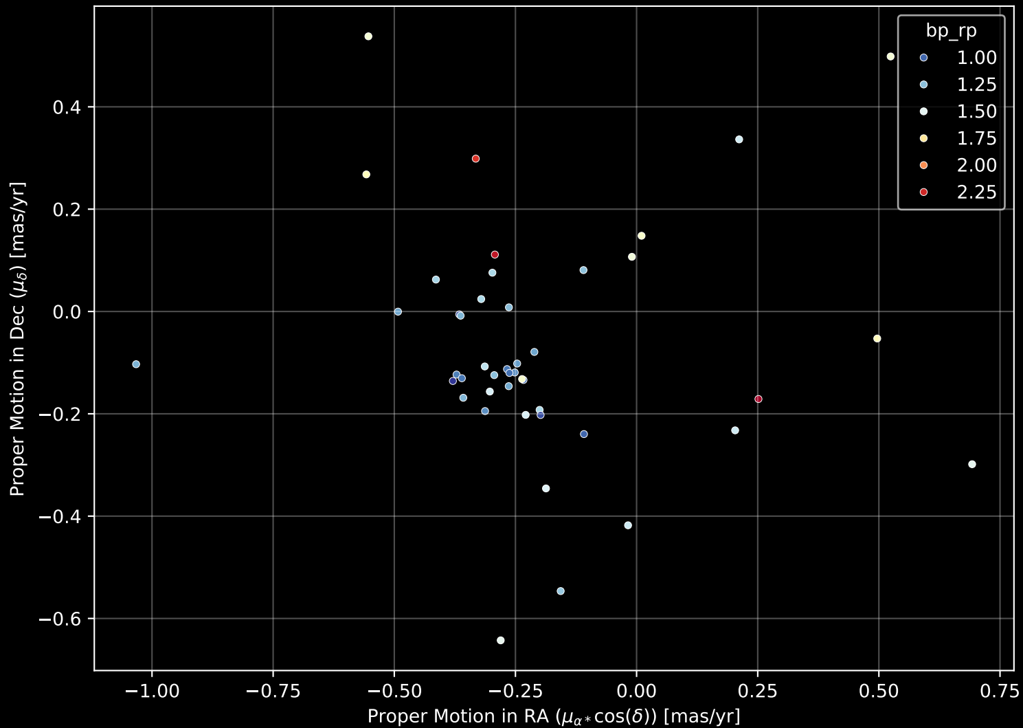
Gaia Cluster: [Juchert_9] Proper Motion Diagram (n= 45)
