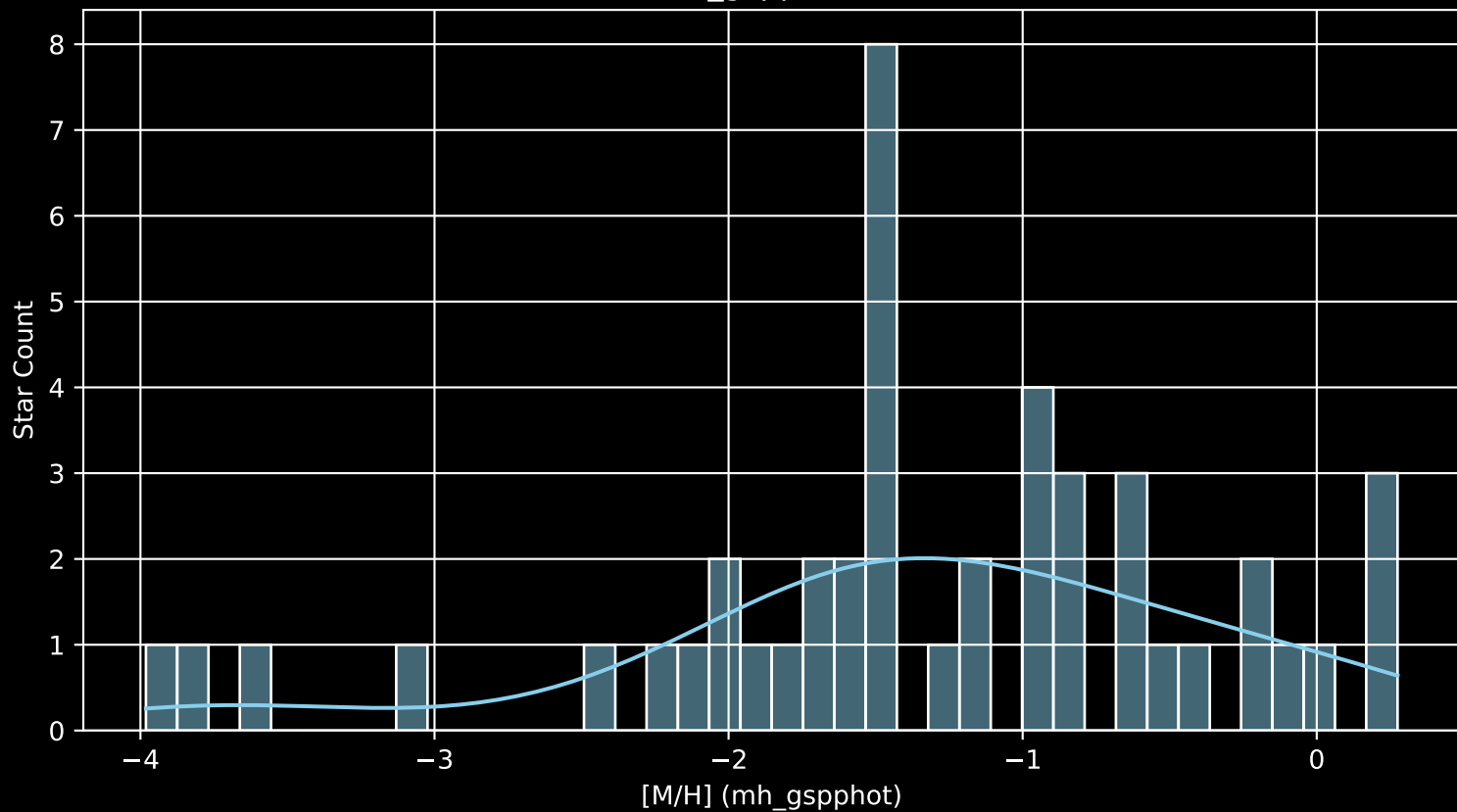
Gaia Cluster: [Juchert_9 [M/H] (mh_gspphot) (n= 45)
