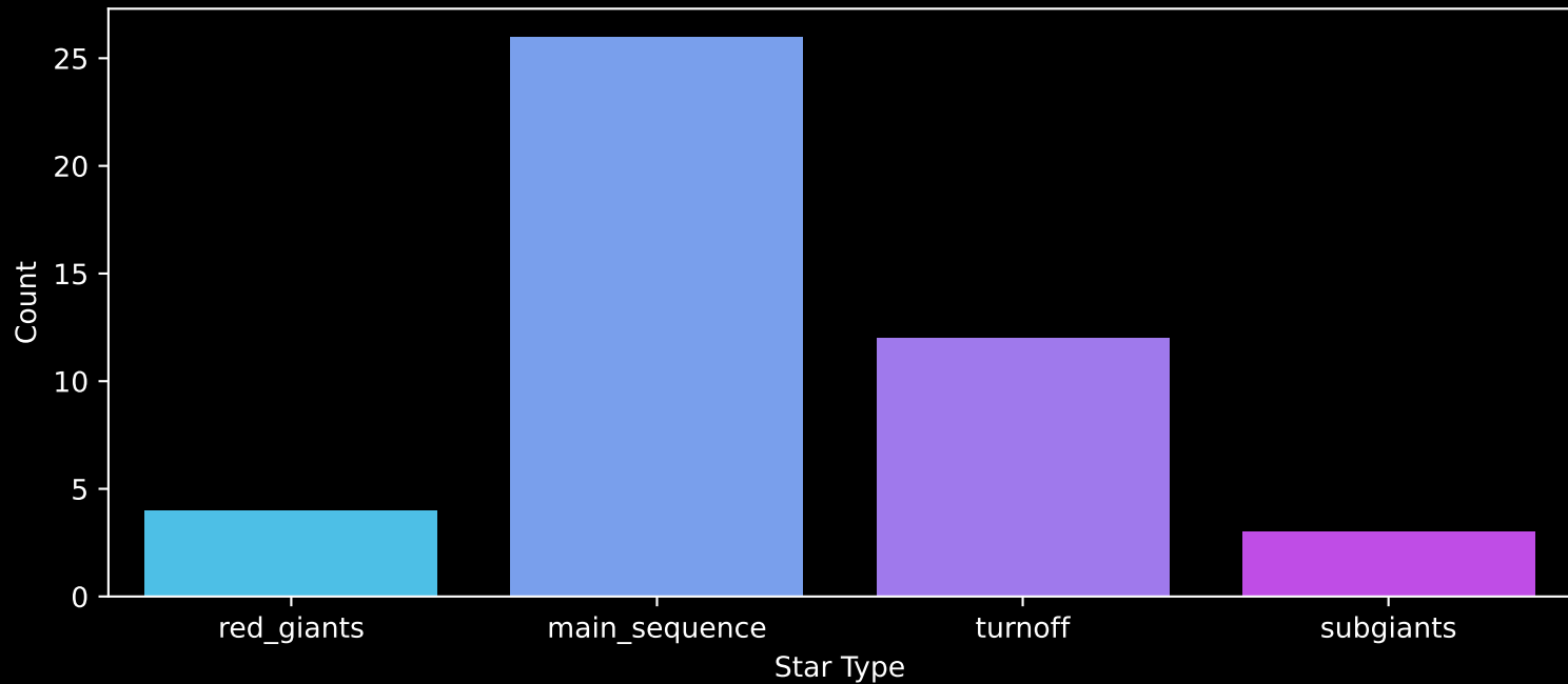
Gaia Cluster: [Juchert_9] Count plot of Star Type
