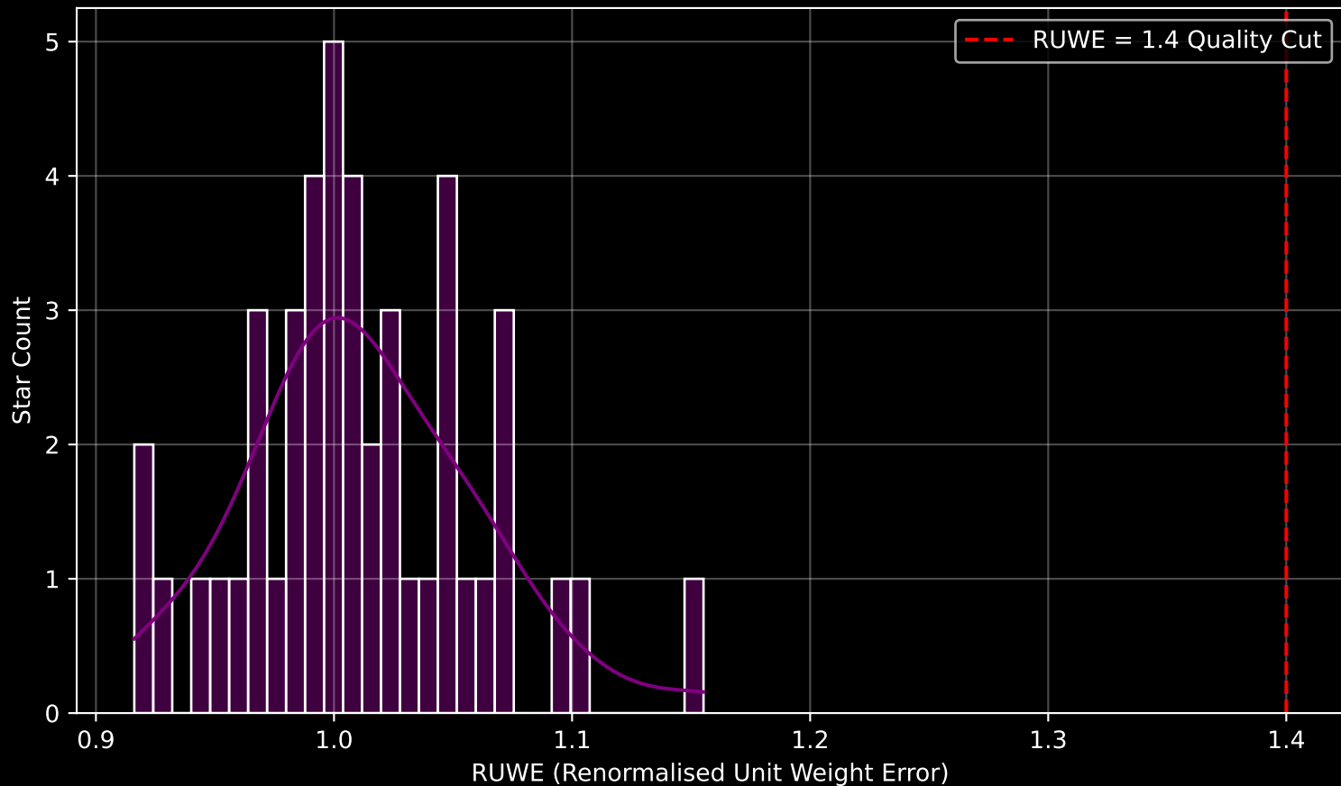
Gaia Cluster: [Juchert_9] RUWE Distribution (n= 45)
