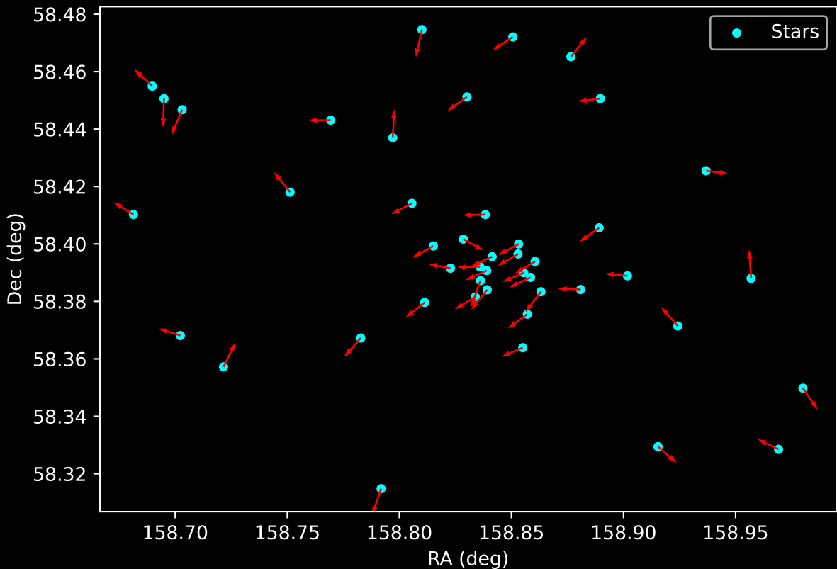
Gaia Cluster: [Juchert_9] Proper Motion Vectors for Gaia Star Field (n= 45)
