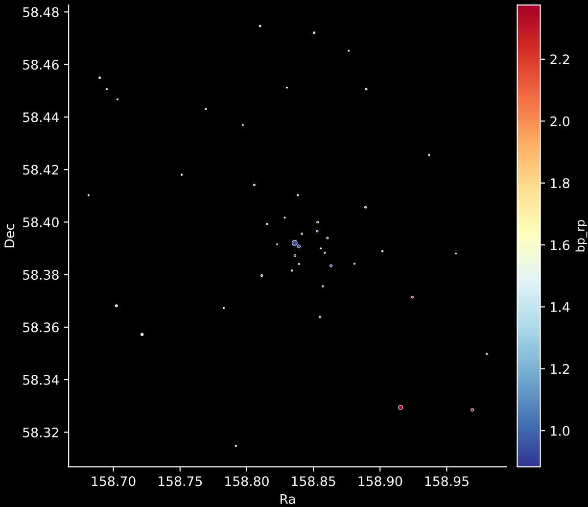
Gaia Cluster: [Juchert_9] Stars: 45
