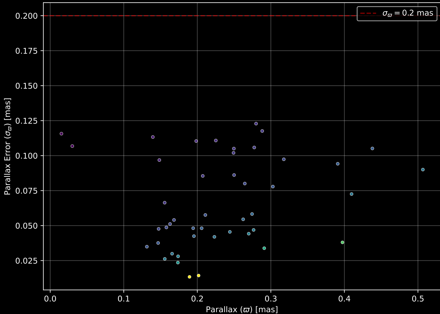
Gaia Cluster: [Juchert_9] Parallax Quality (n= 45)
