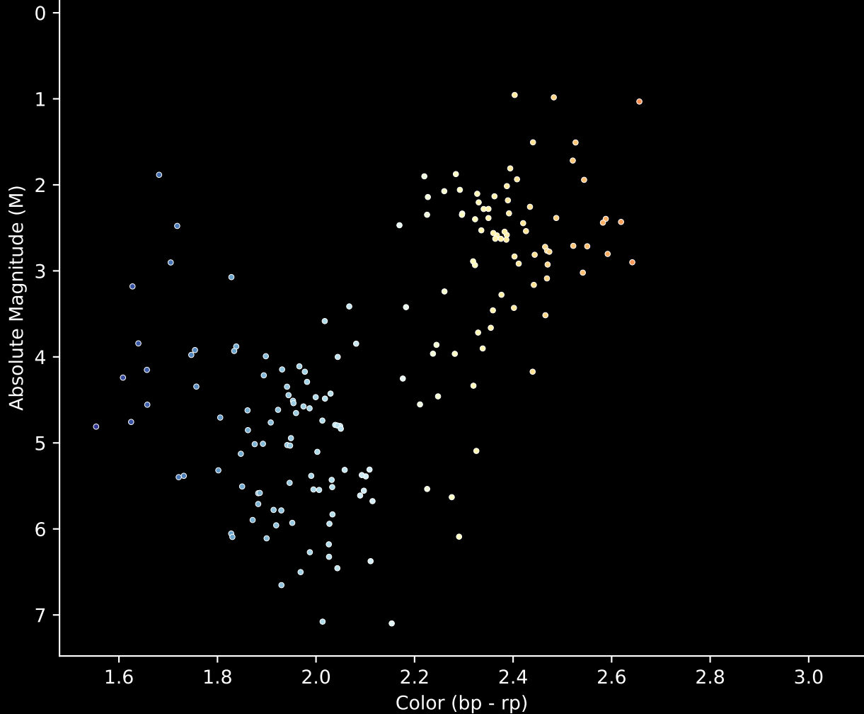
Gaia Cluster: [King_11] Stars (n= 173) Hertzsprung-Russel Diagram
