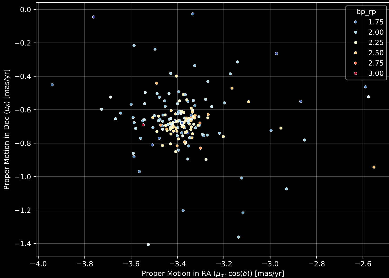
Gaia Cluster: [King_11] Proper Motion Diagram (n= 173)
