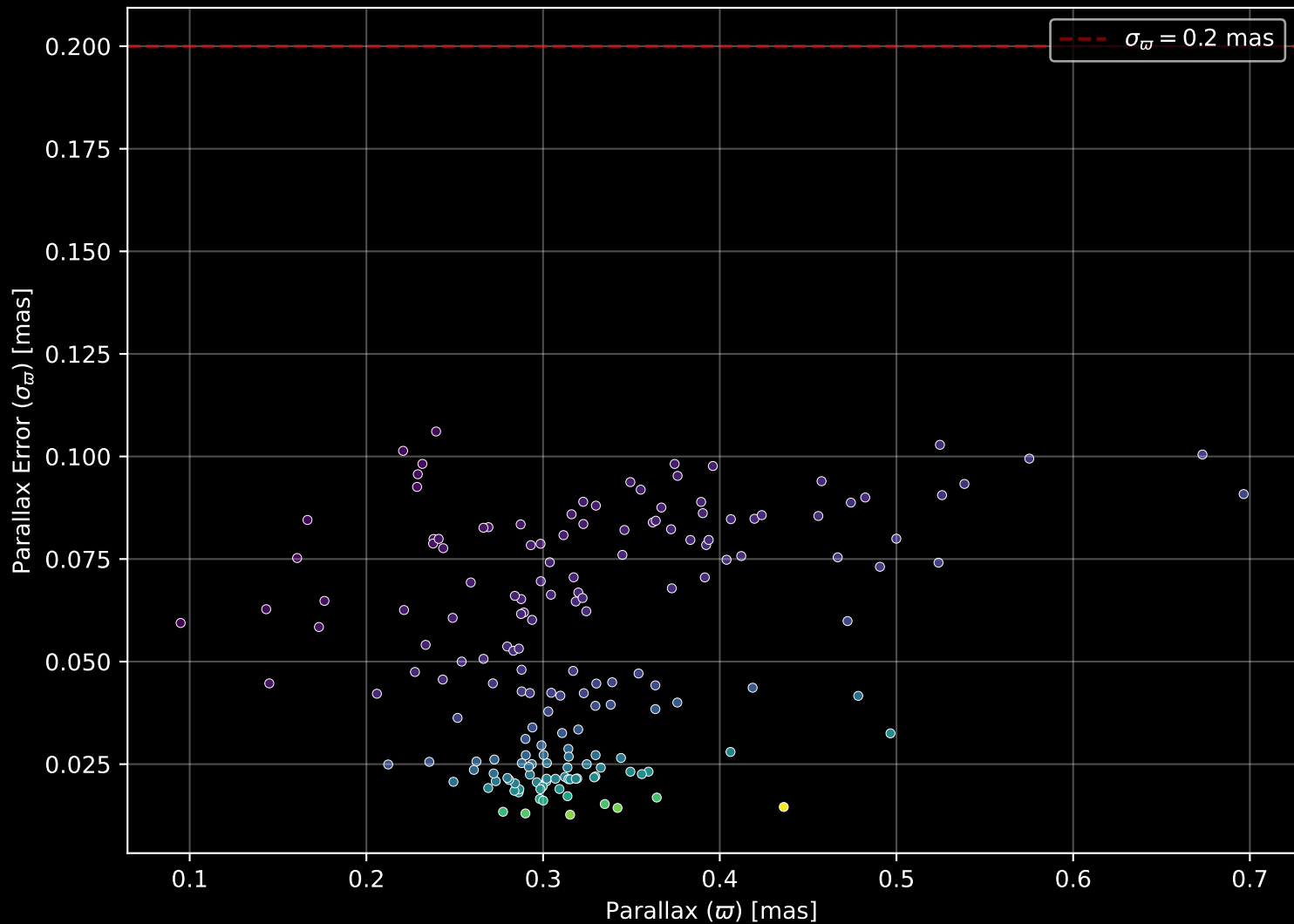
Gaia Cluster: [King_11] Parallax Quality (n= 173)
