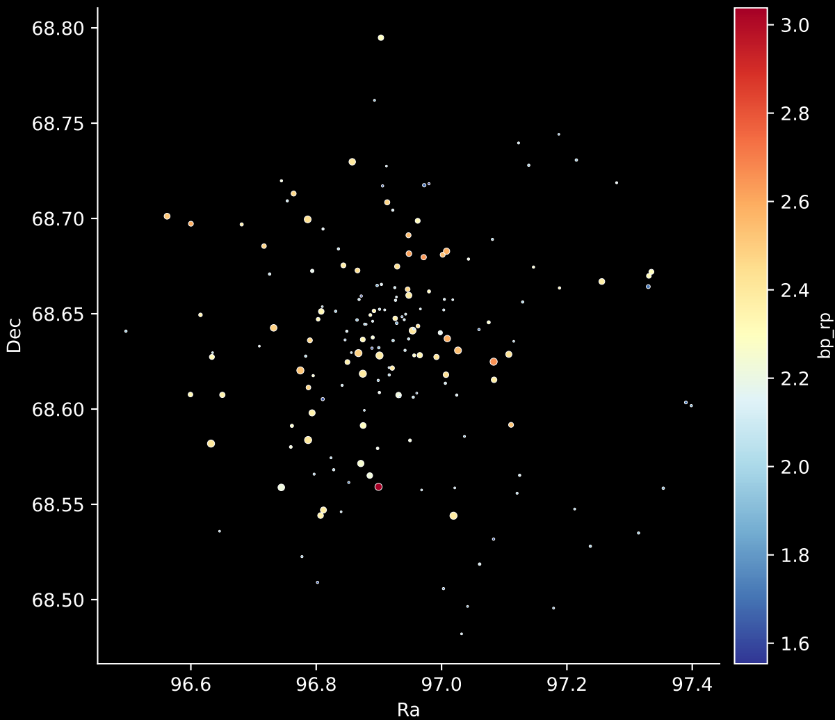
Gaia Cluster: [King_11] Stars: 173
