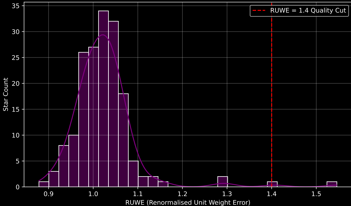
Gaia Cluster: [King_11] RUWE Distribution (n= 173)
