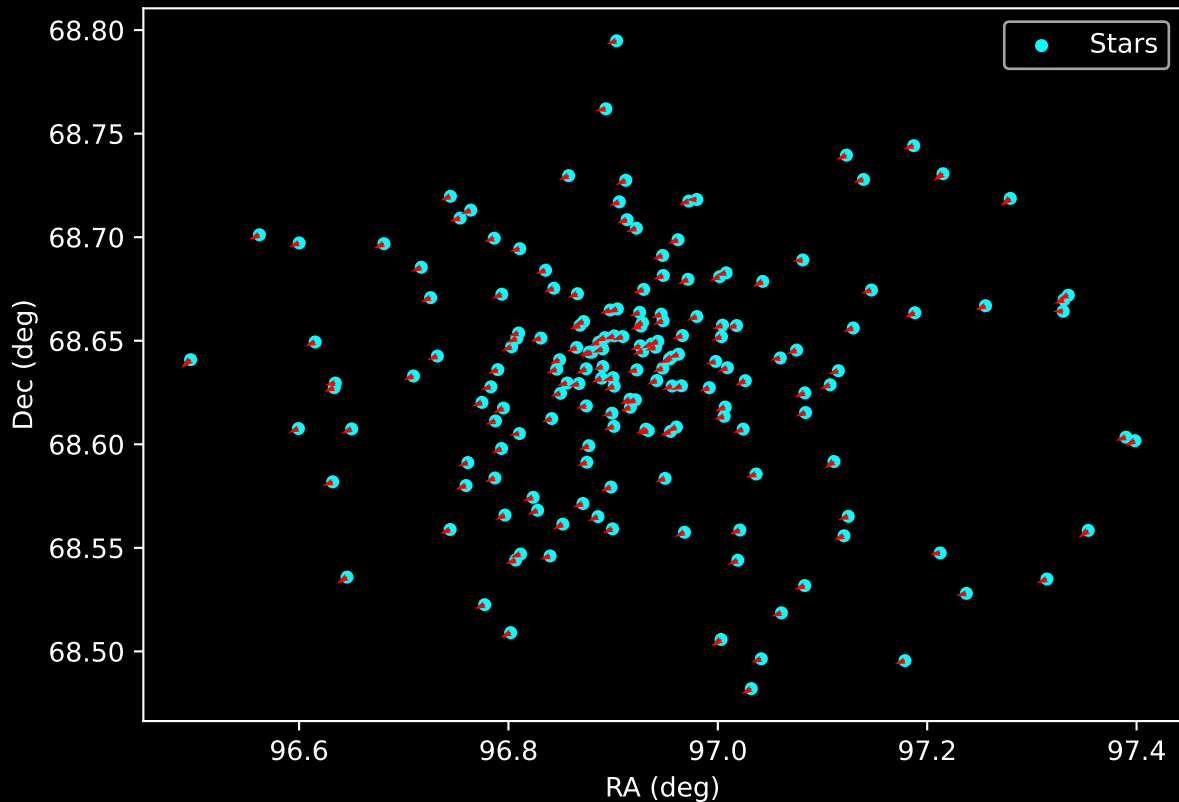
Gaia Cluster: [King_11] Proper Motion Vectors for Gaia Star Field (n= 173)
