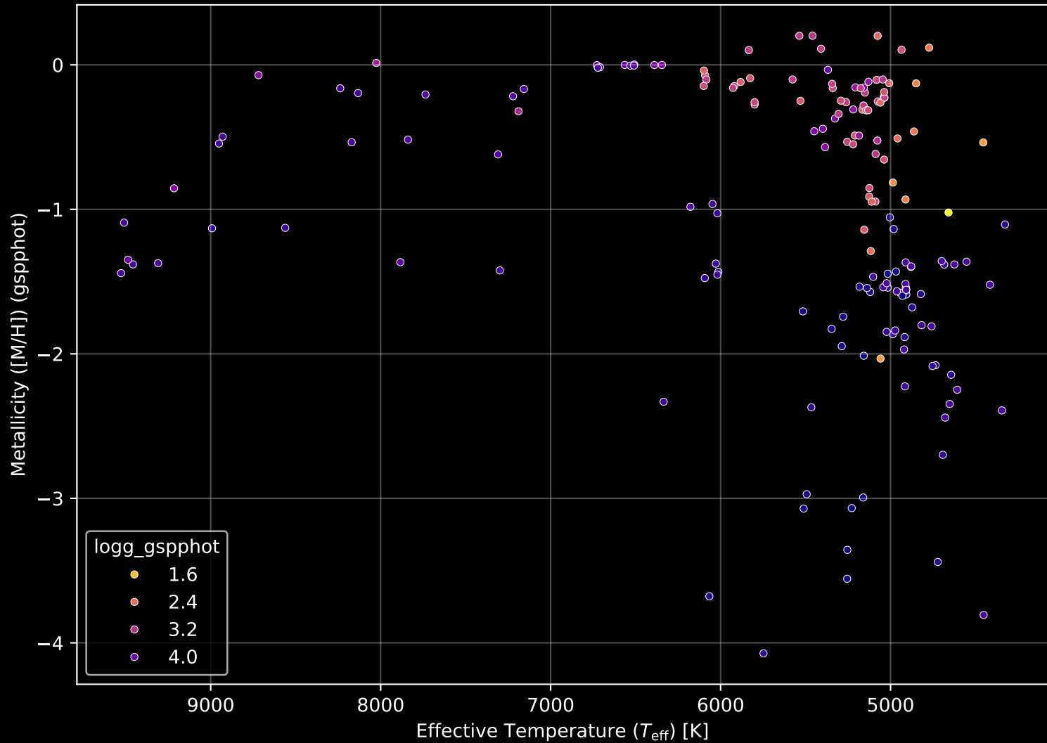
Gaia Cluster: [King_11] Stellar Population Parameters (n= 173)
