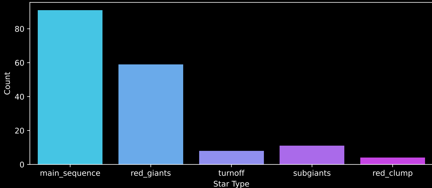
Gaia Cluster: [King_11] Count plot of Star Type
