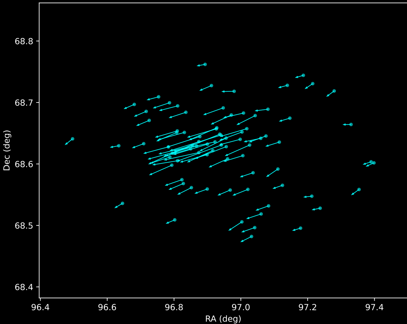
Gaia DR3 Noise Stream Proper Motion Vectors (n=80)
