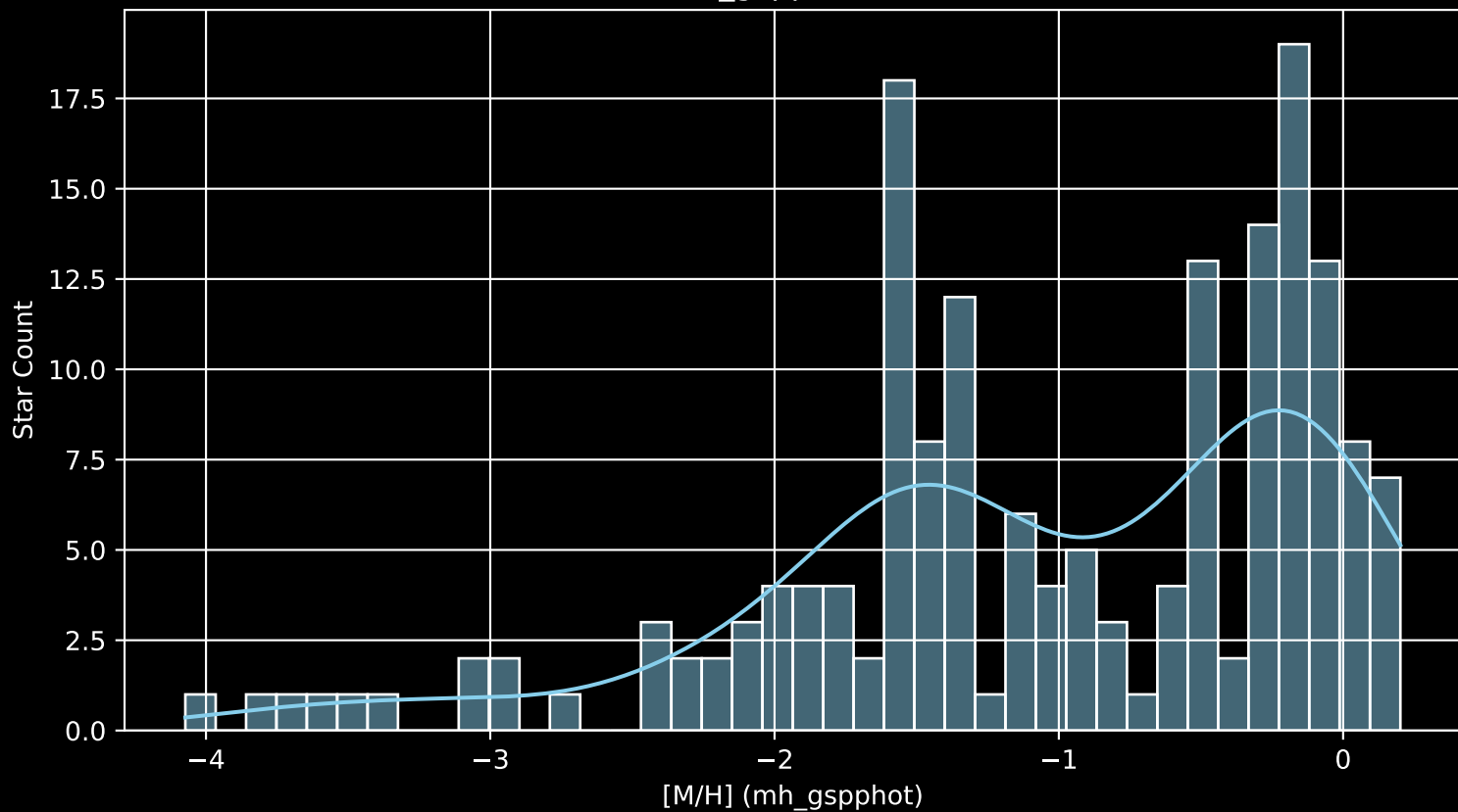
Gaia Cluster: [King_11 [M/H] (mh_gspphot) (n= 173)
