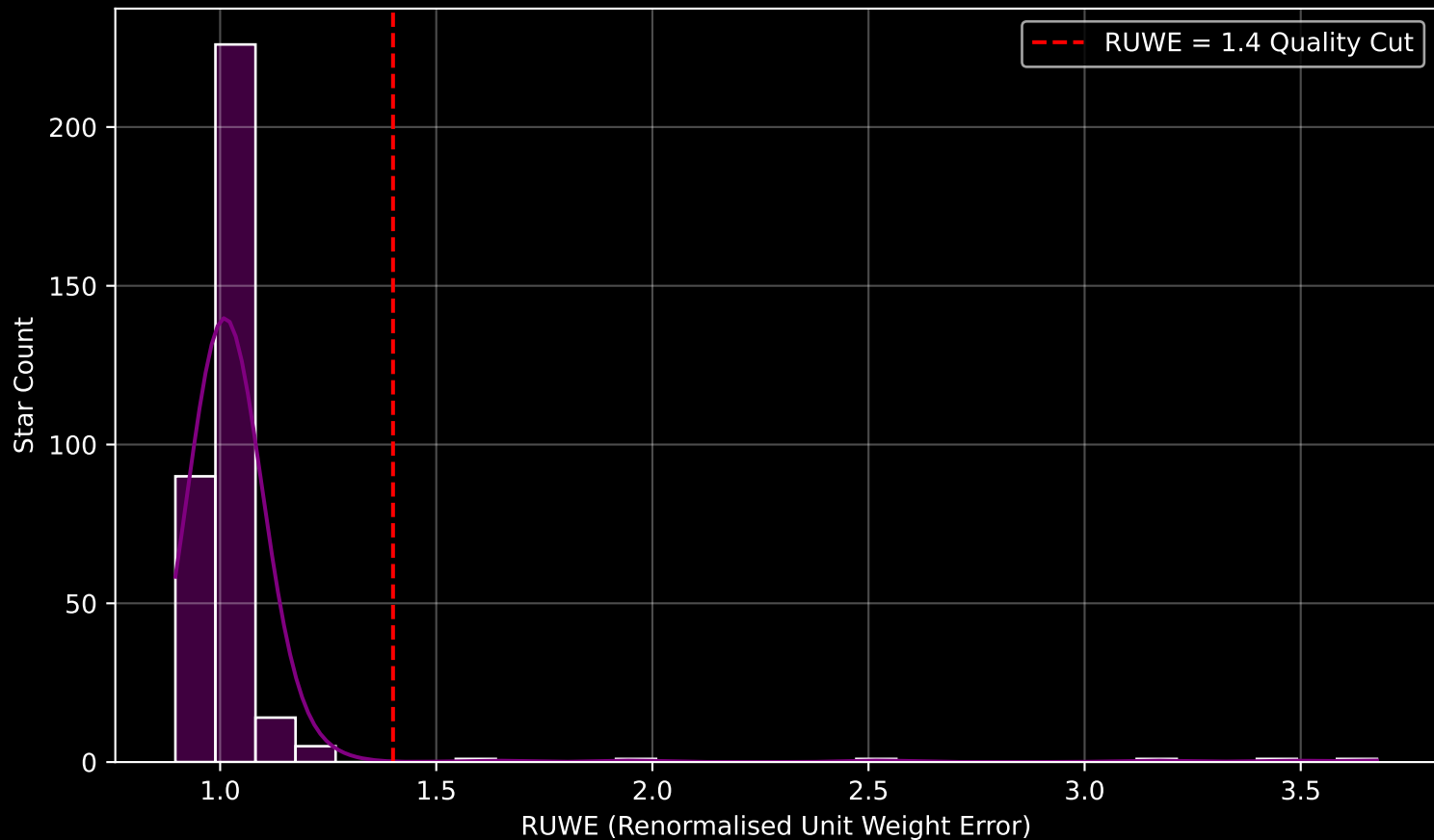
Gaia Cluster: [King_13] RUWE Distribution (n= 341)
