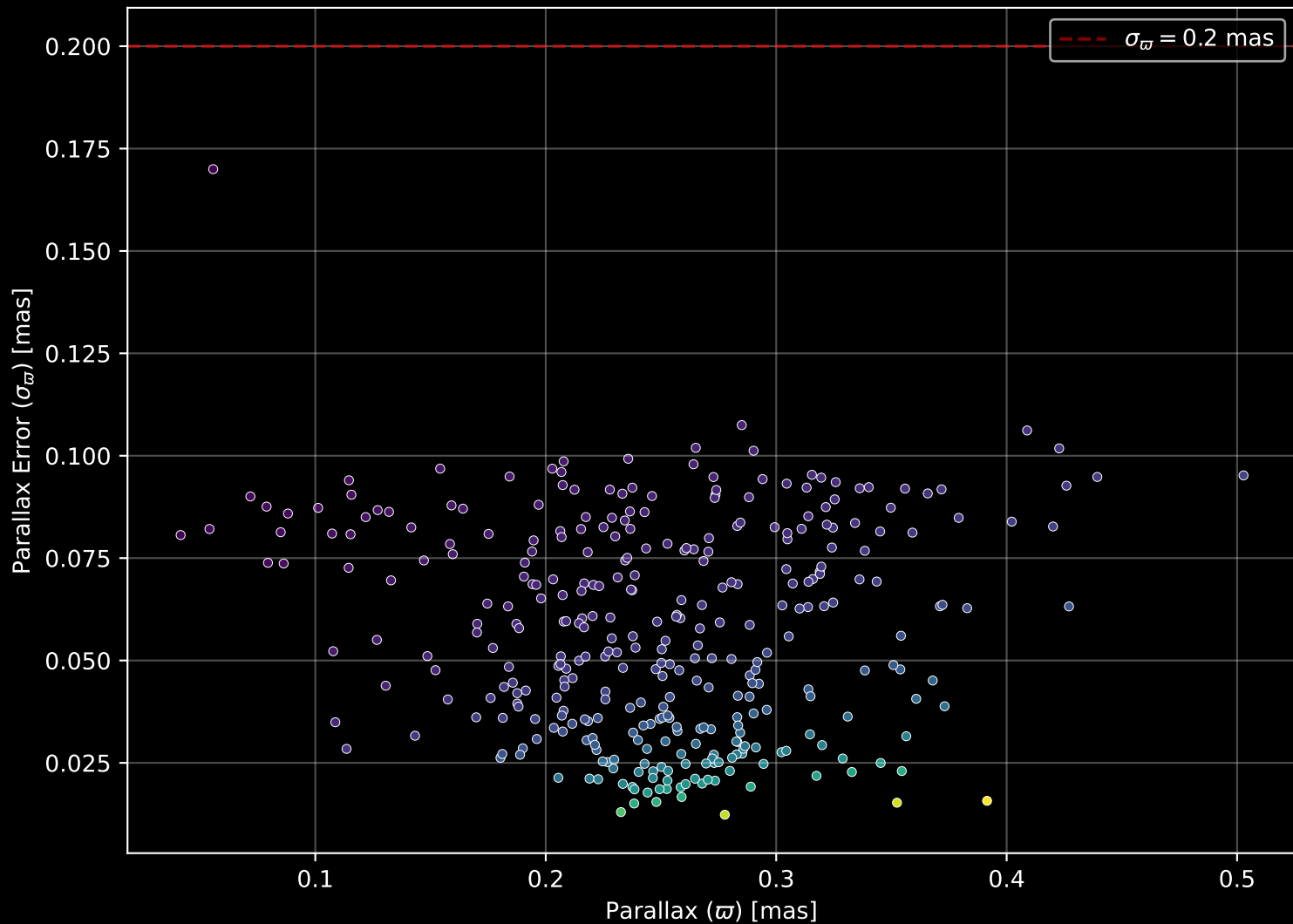
Gaia Cluster: [King_13] Parallax Quality (n= 341)
