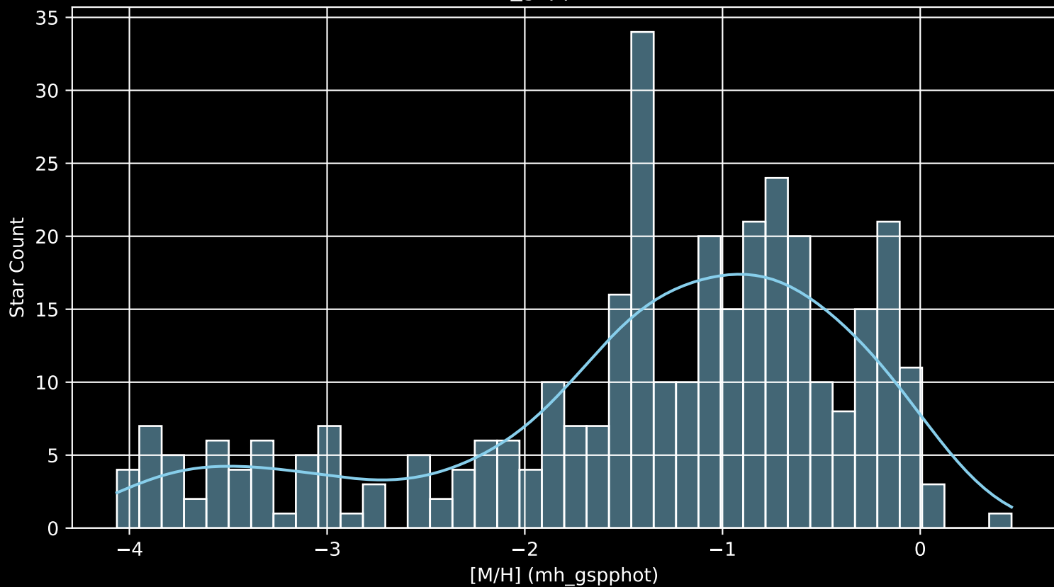
Gaia Cluster: [King_13 [M/H] (mh_gspphot) (n= 341)
