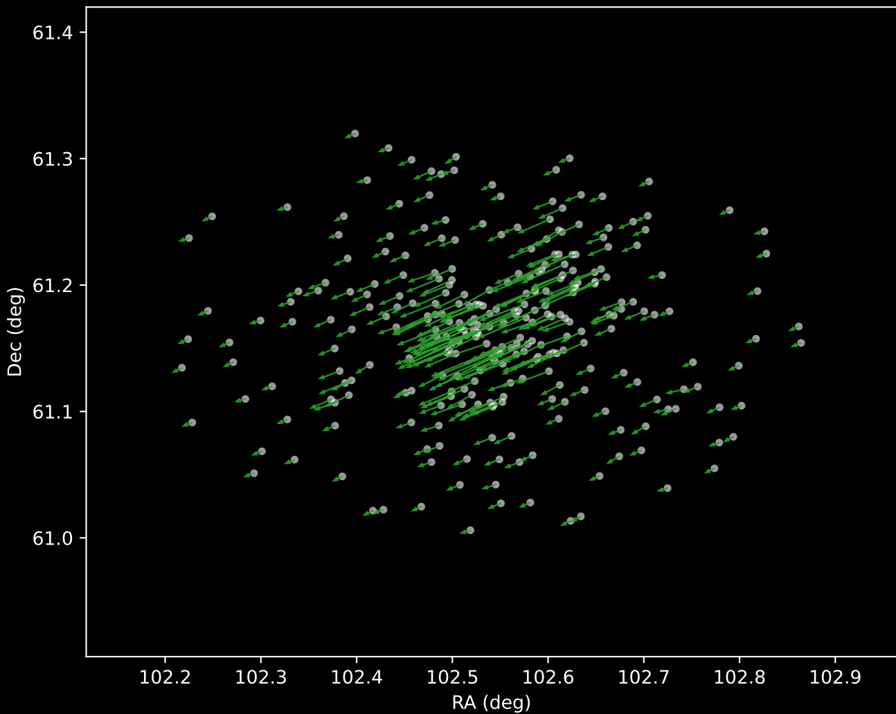
Gaia DR3 Cluster 4 Proper Motion Vectors (n=282)
