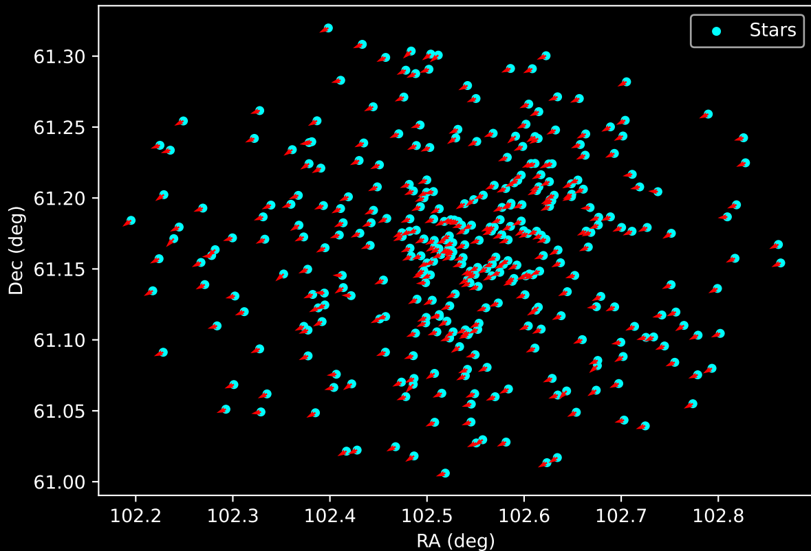
Gaia Cluster: [King_13] Proper Motion Vectors for Gaia Star Field (n= 341)
