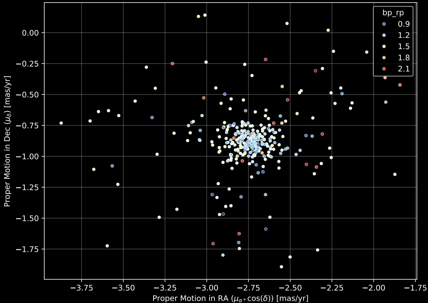
Gaia Cluster: [King_13] Proper Motion Diagram (n= 341)
