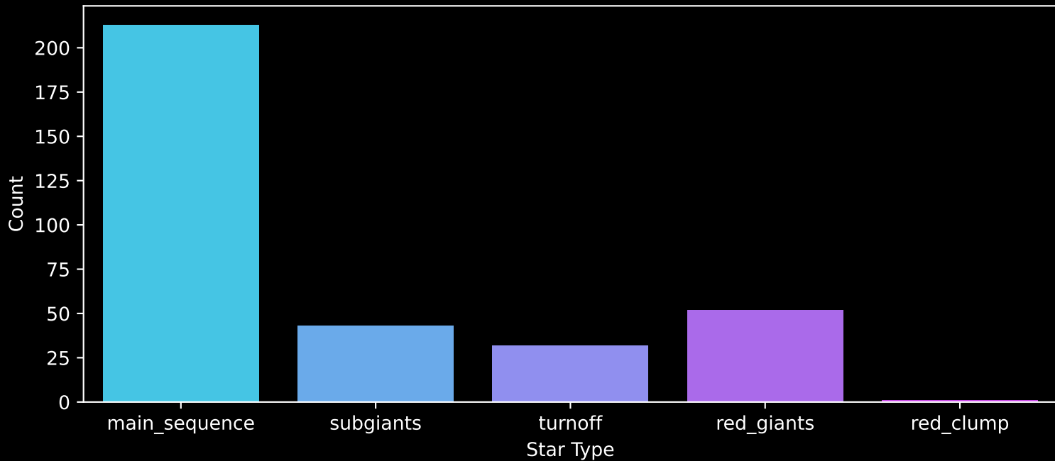
Gaia Cluster: [King_13] Count plot of Star Type
