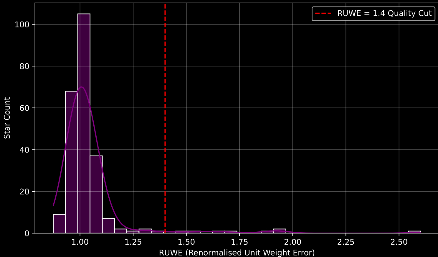
Gaia Cluster: [King_14] RUWE Distribution (n= 240)
