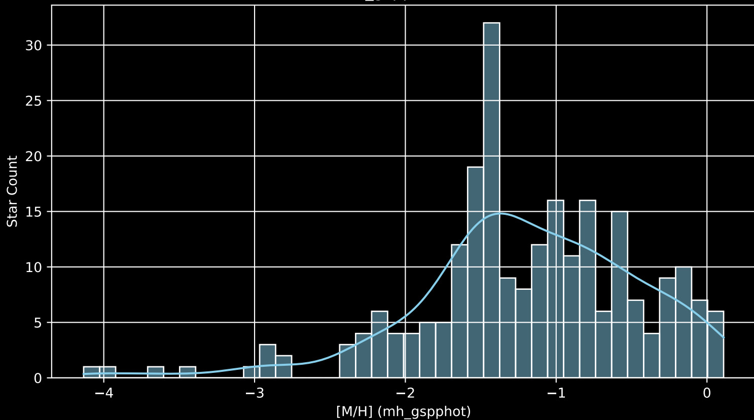
Gaia Cluster: [King_14 [M/H] (mh_gspphot) (n= 240)
