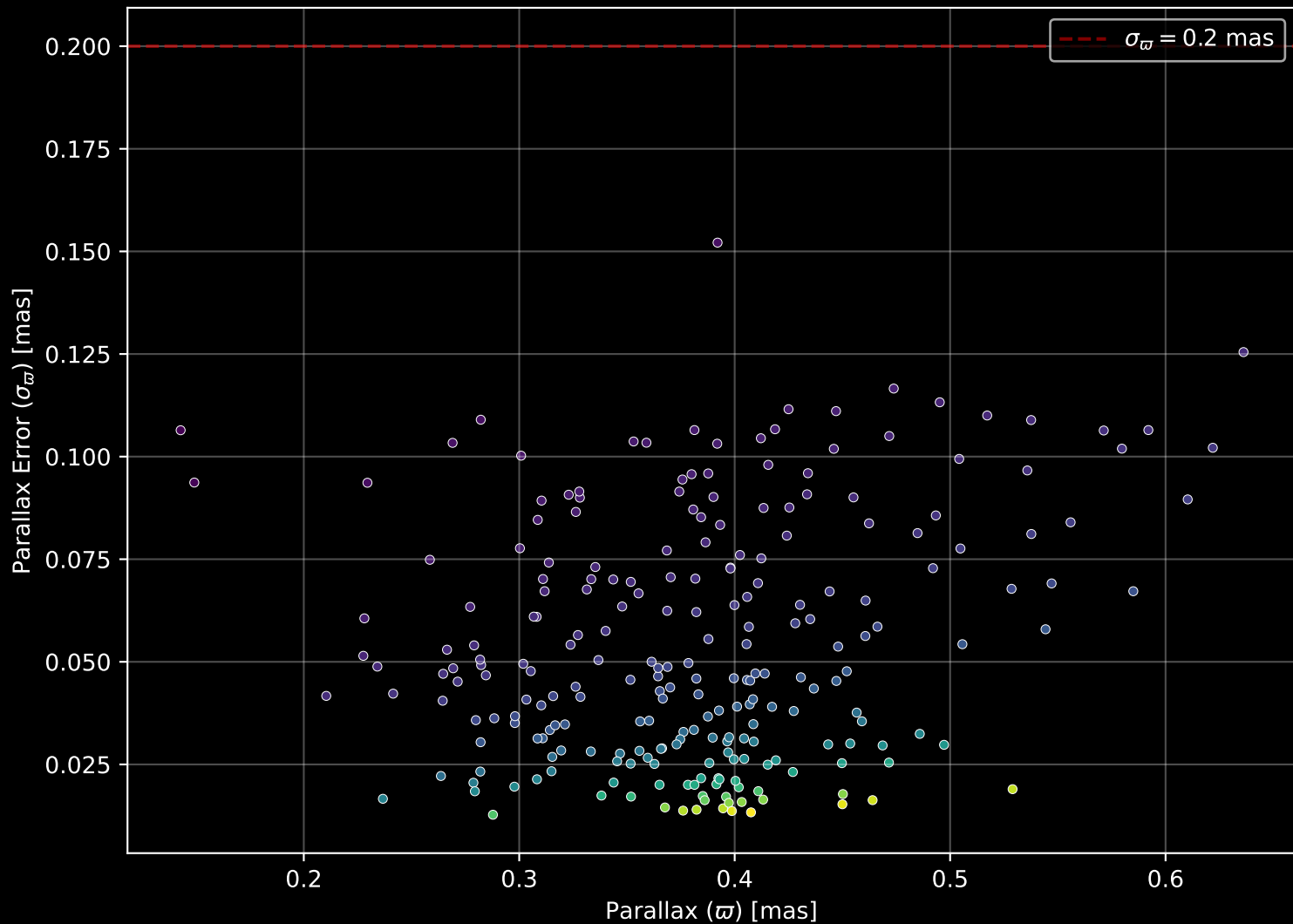
Gaia Cluster: [King_14] Parallax Quality (n= 240)
