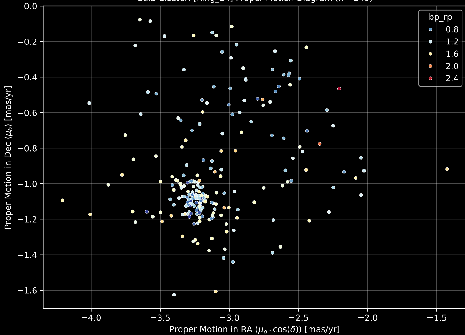
Gaia Cluster: [King_14] Proper Motion Diagram (n= 240)
