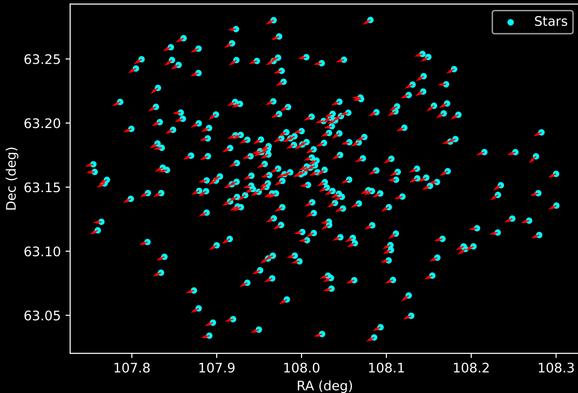
Gaia Cluster: [King_14] Proper Motion Vectors for Gaia Star Field (n= 240)
