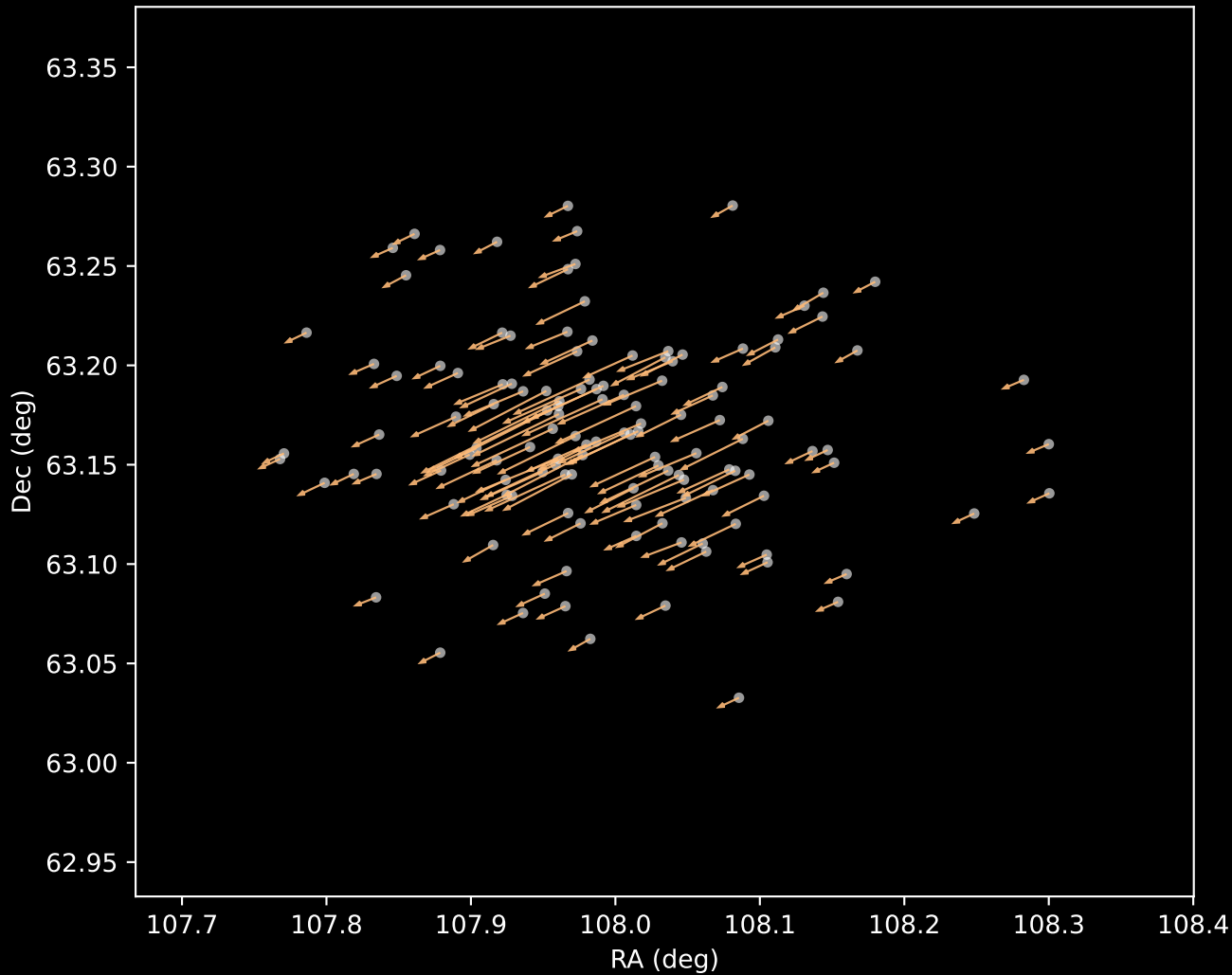
Gaia DR3 Cluster 3 Proper Motion Vectors (n=130)
