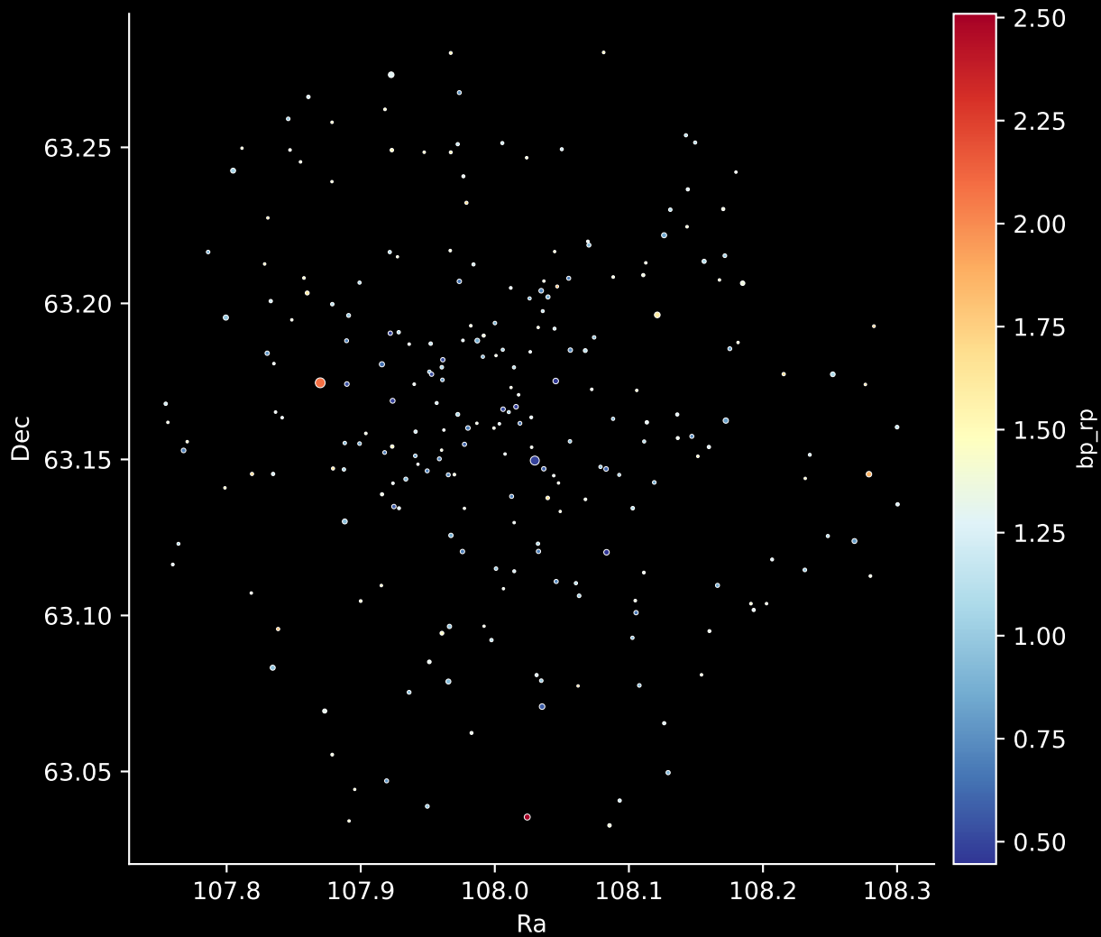
Gaia Cluster: [King_14] Stars: 240
