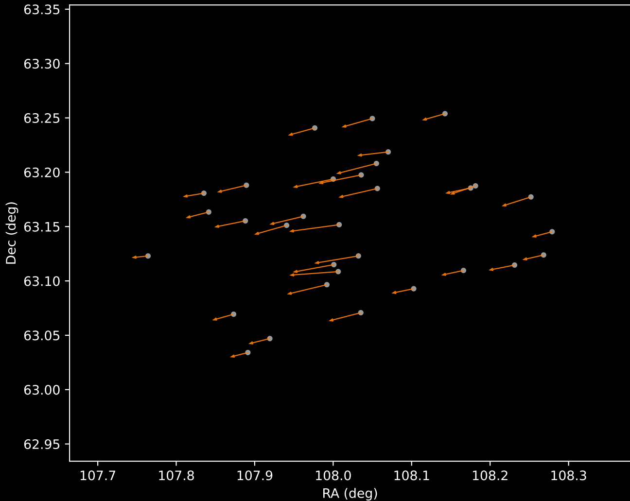
Gaia DR3 Cluster 2 Proper Motion Vectors (n=32)
