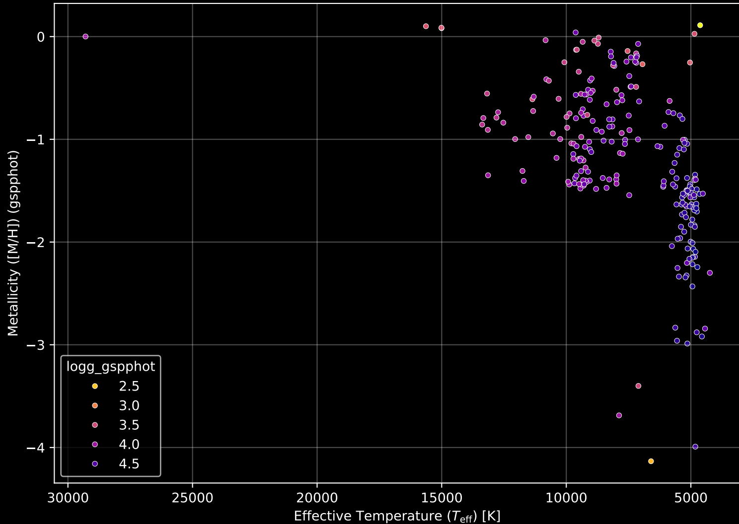
Gaia Cluster: [King_14] Stellar Population Parameters (n= 240)
