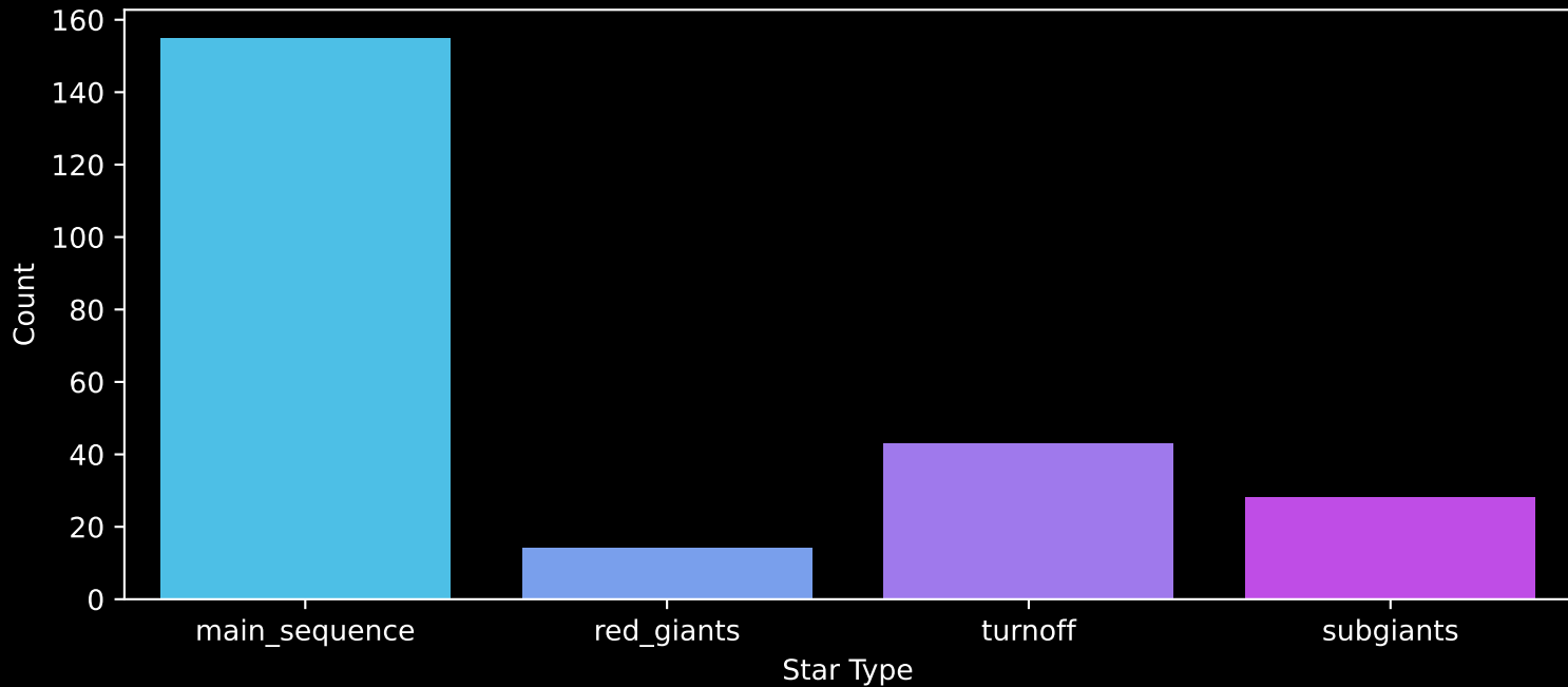
Gaia Cluster: [King_14] Count plot of Star Type
