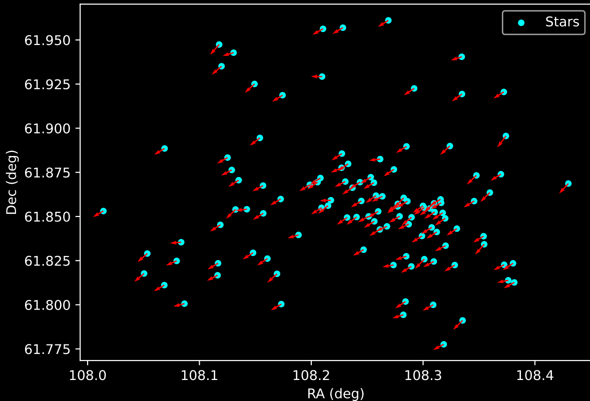
Gaia Cluster: [King_15] Proper Motion Vectors for Gaia Star Field (n= 111)
