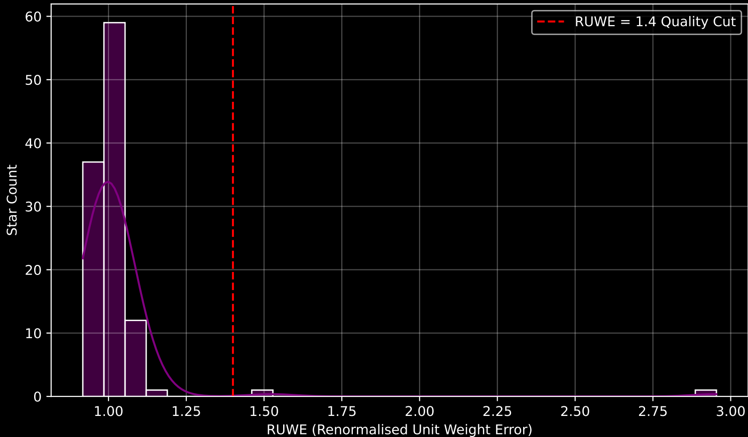
Gaia Cluster: [King_15] RUWE Distribution (n= 111)
