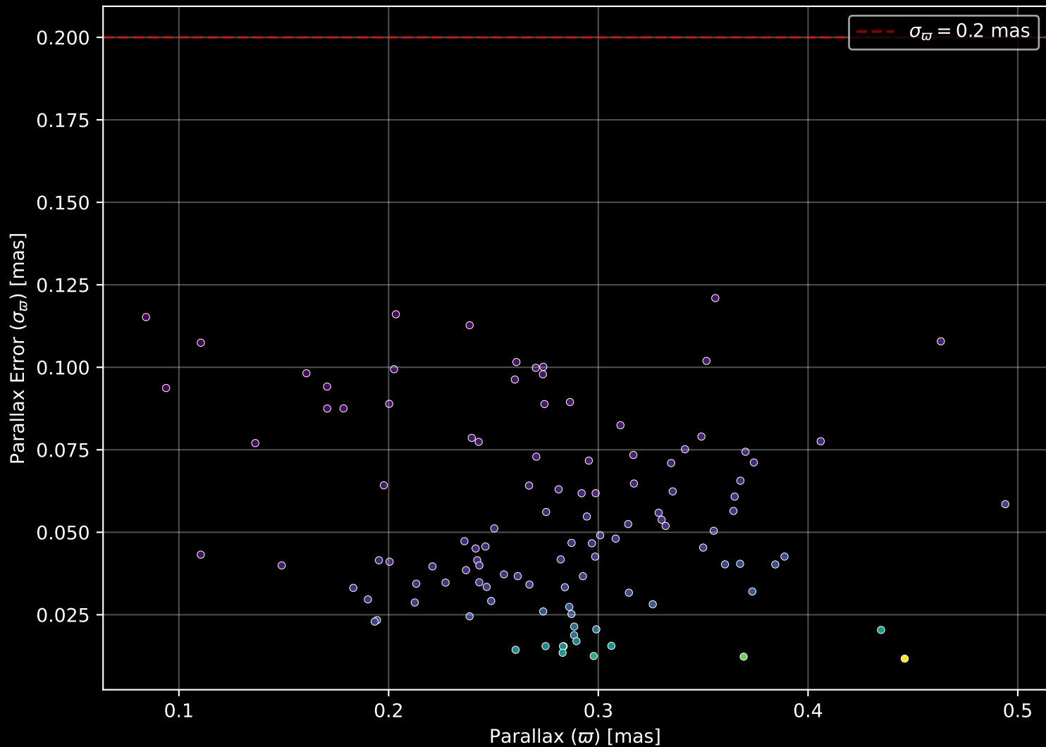
Gaia Cluster: [King_15] Parallax Quality (n= 111)
