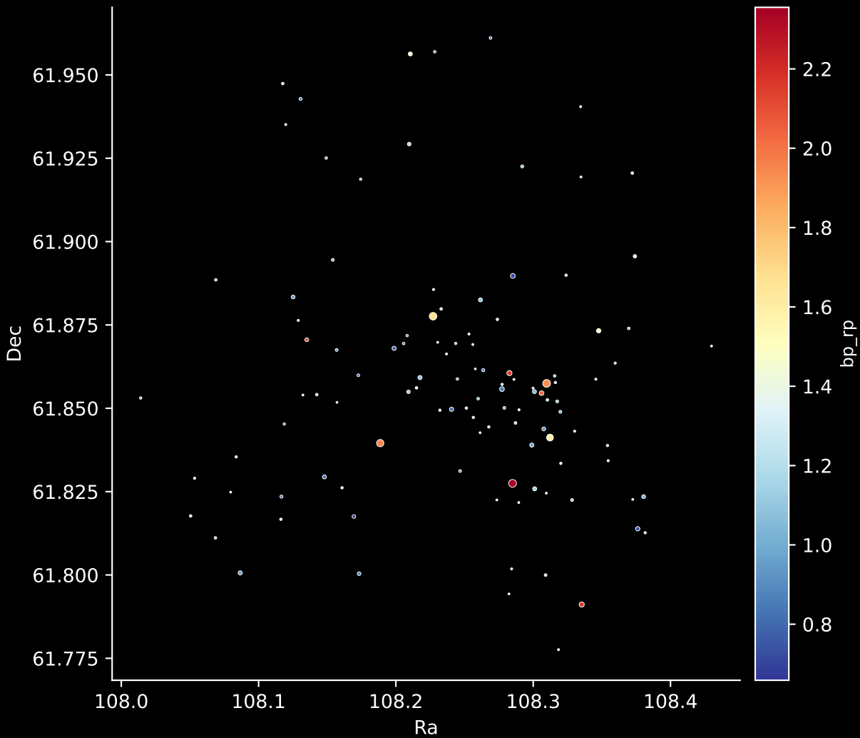
Gaia Cluster: [King_15] Stars: 111
