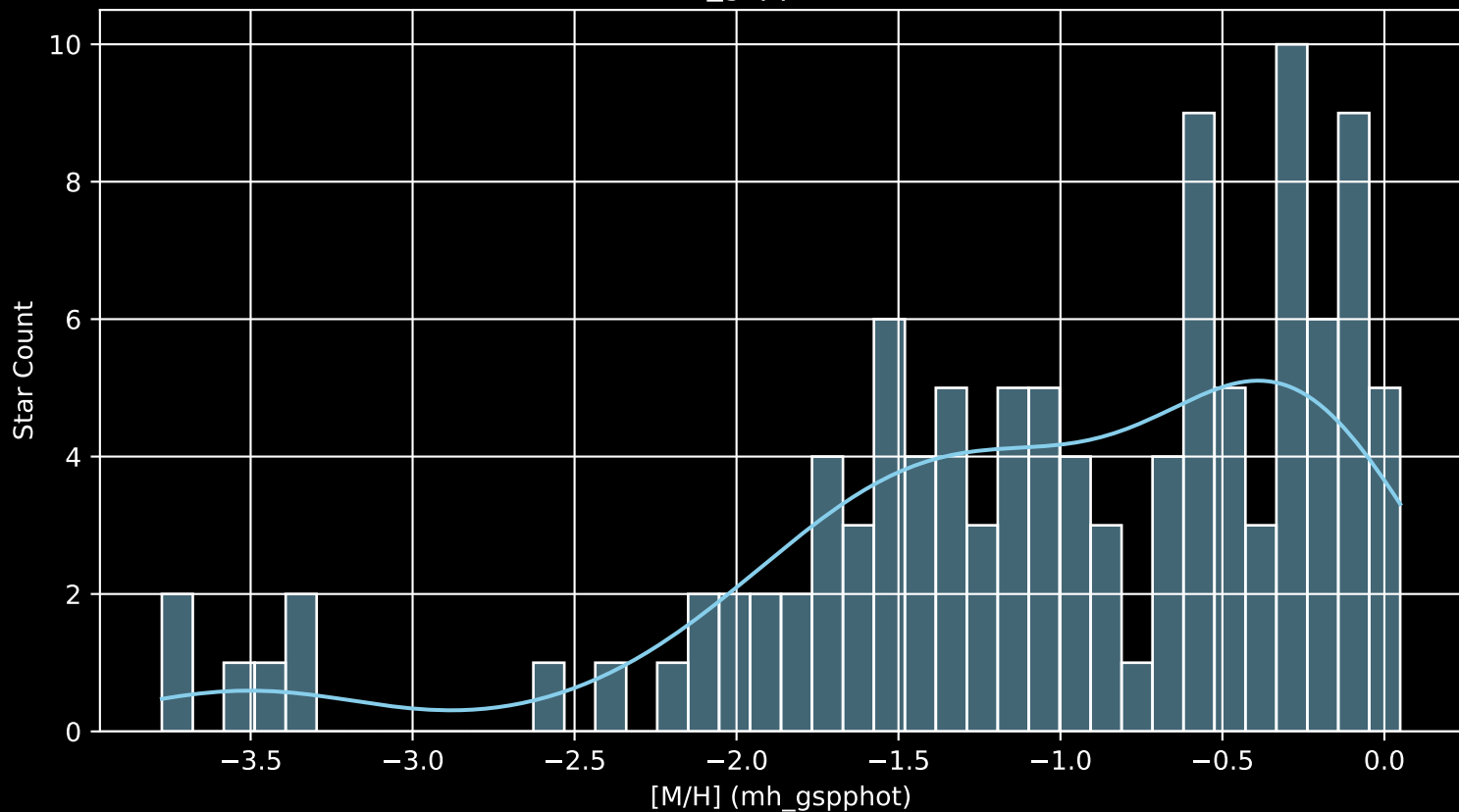
Gaia Cluster: [King_15 [M/H] (mh_gspphot) (n= 111)
