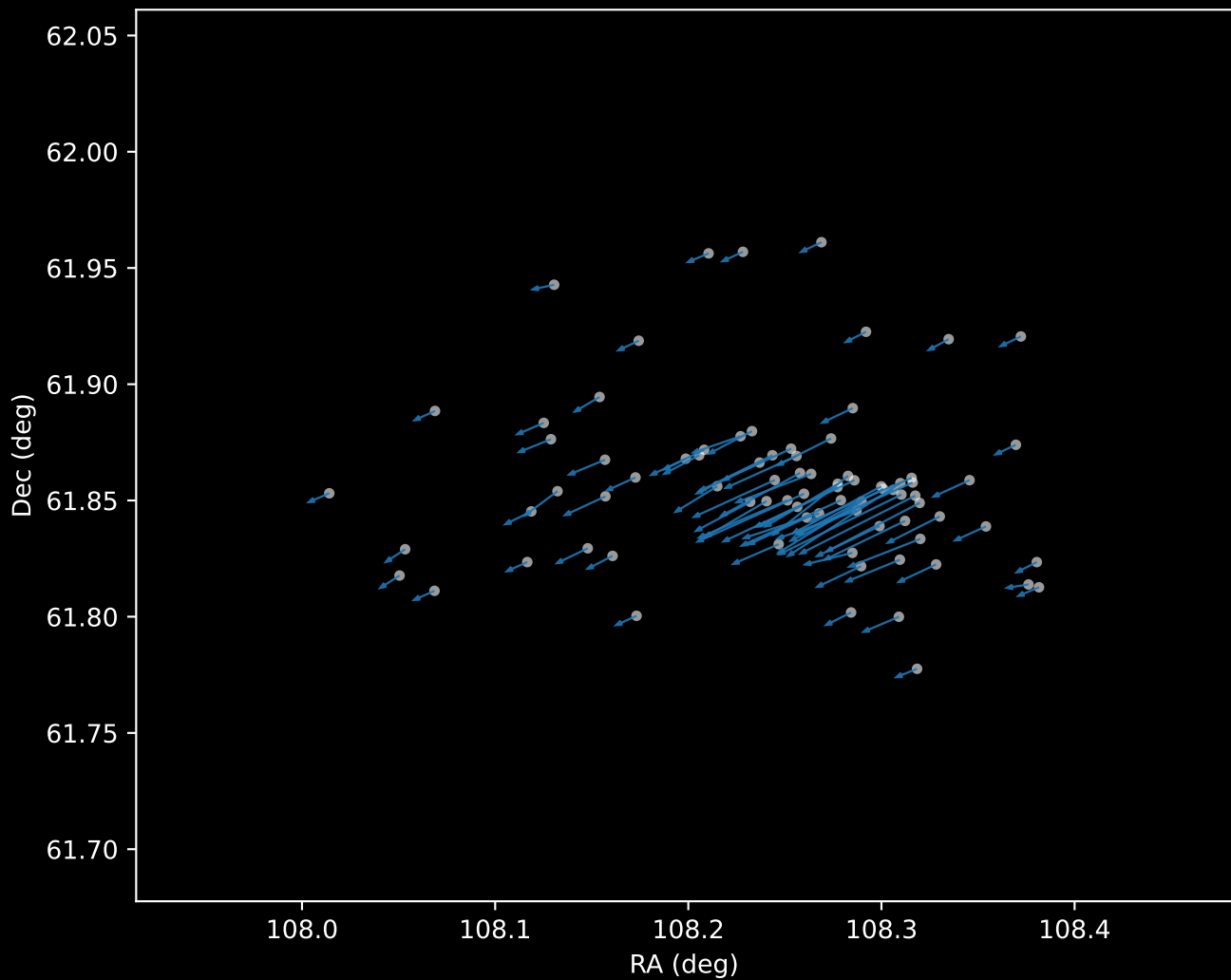
Gaia DR3 Cluster 0 Proper Motion Vectors (n=81)
