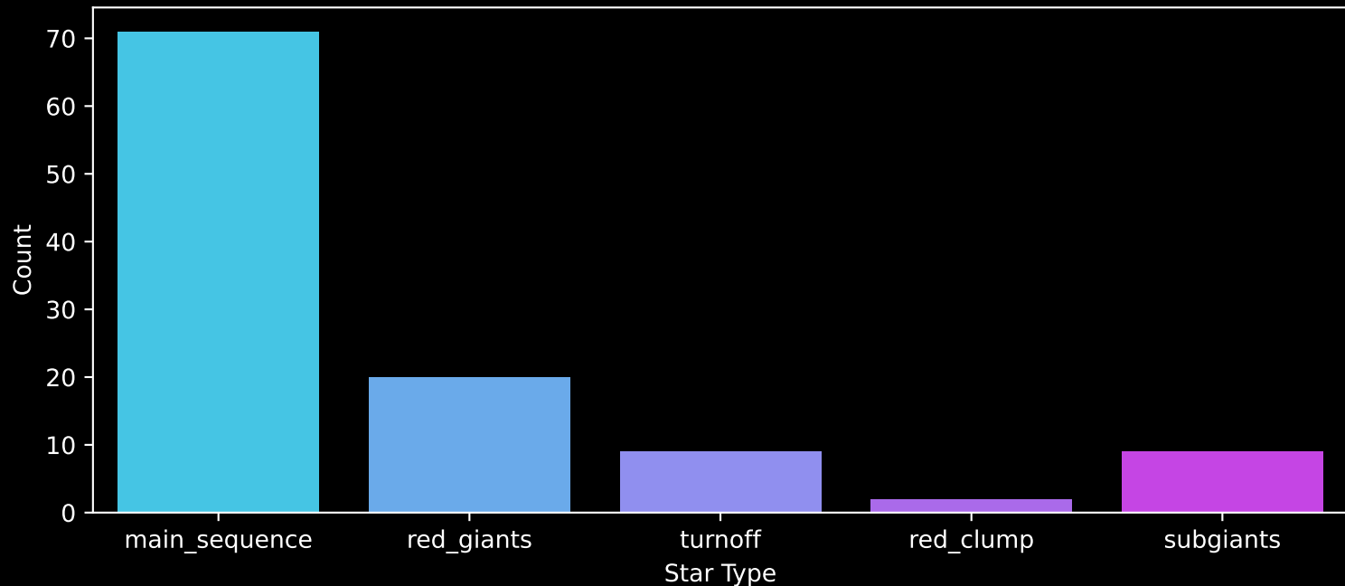
Gaia Cluster: [King_15] Count plot of Star Type
