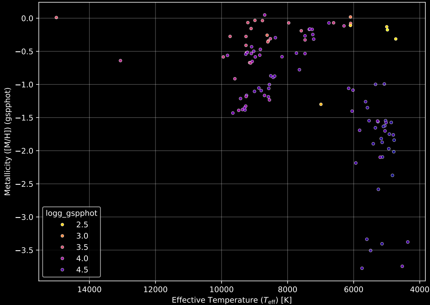
Gaia Cluster: [King_15] Stellar Population Parameters (n= 111)
