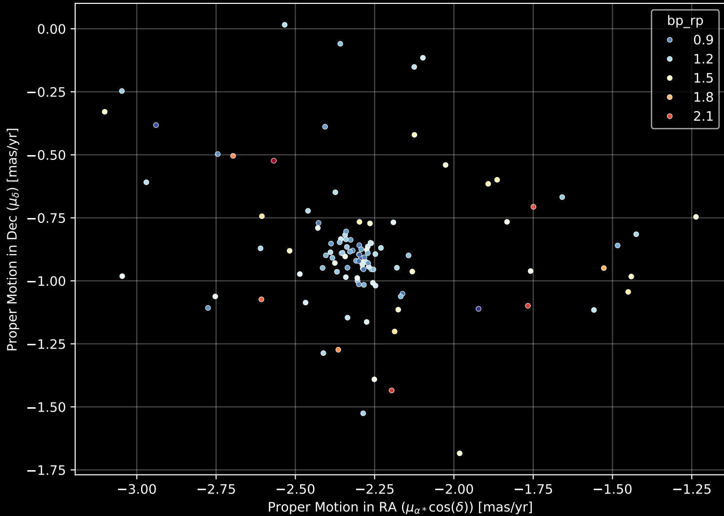
Gaia Cluster: [King_15] Proper Motion Diagram (n= 111)
