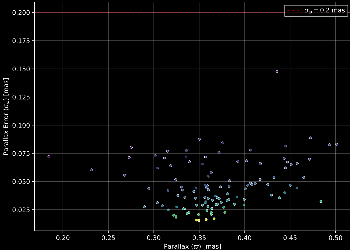
Gaia Cluster: [King_19] Parallax Quality (n= 114)
