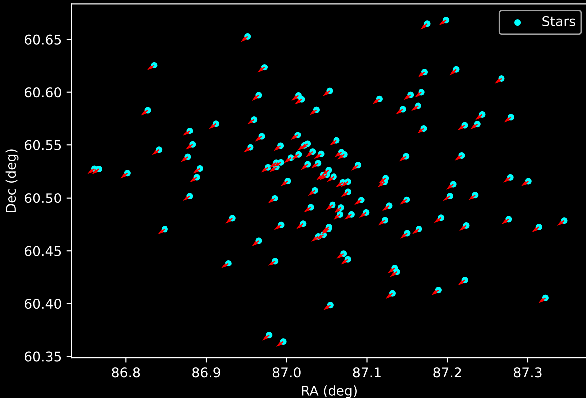
Gaia Cluster: [King_19] Proper Motion Vectors for Gaia Star Field (n= 114)
