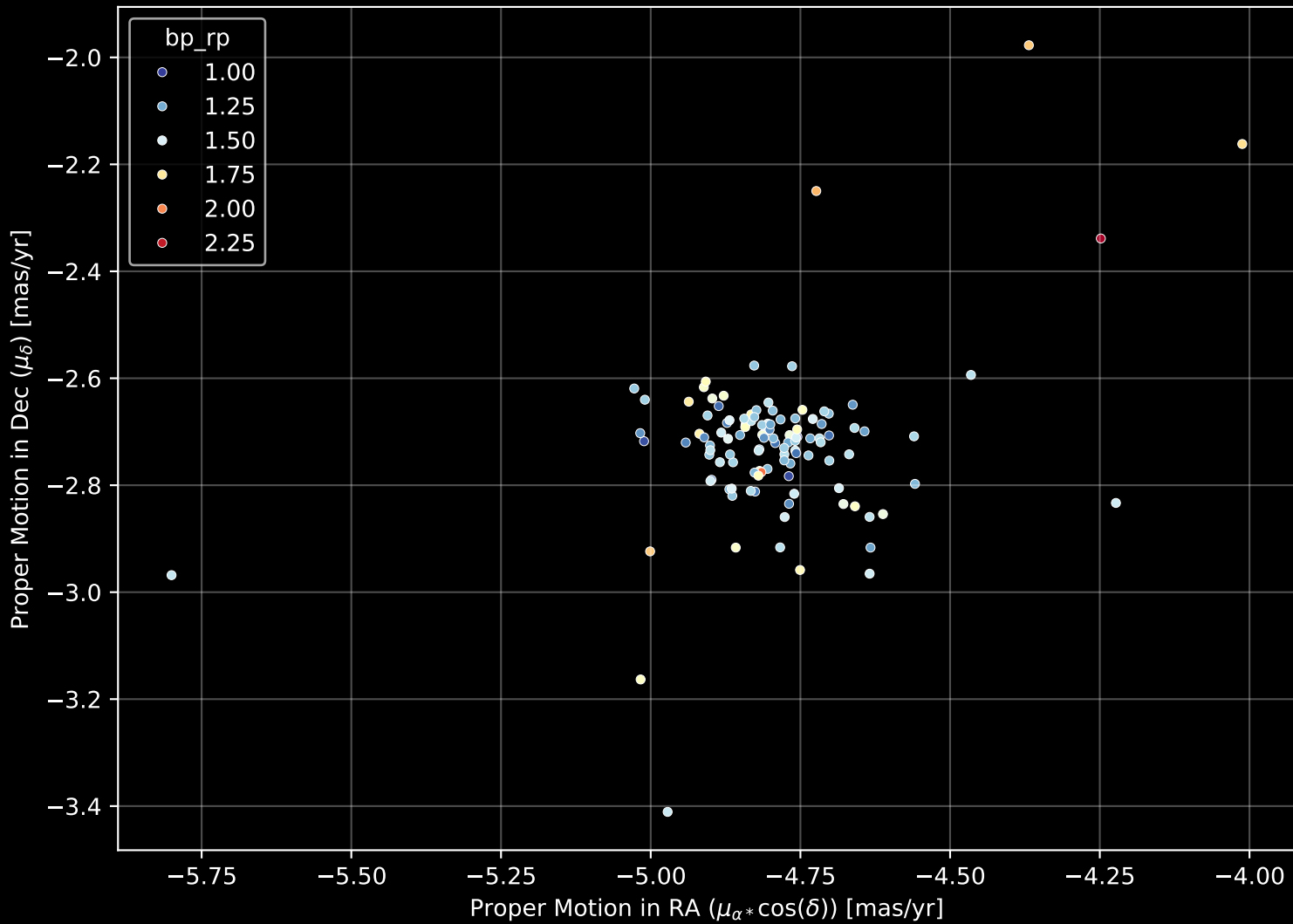
Gaia Cluster: [King_19] Proper Motion Diagram (n= 114)
