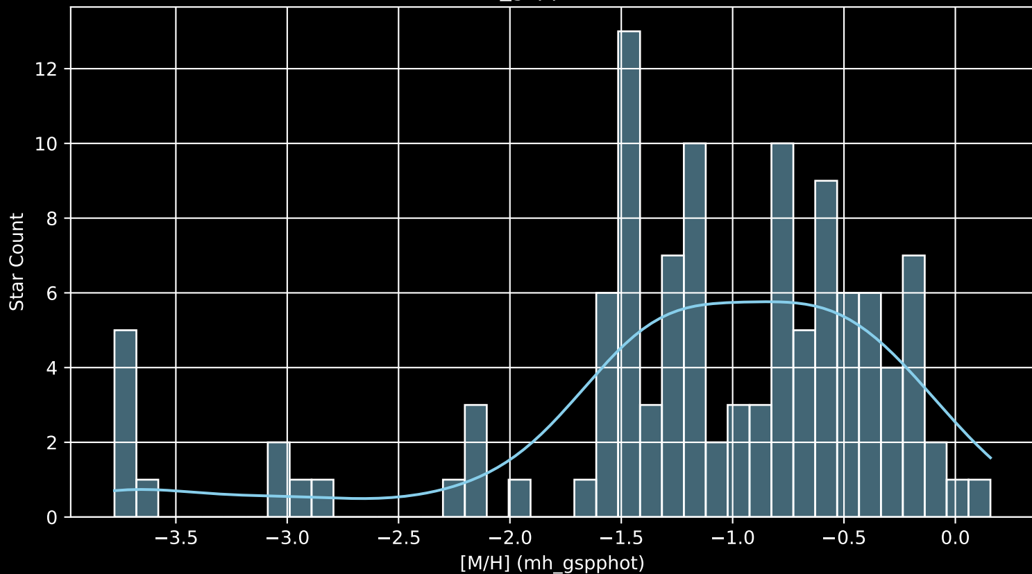
Gaia Cluster: [King_19 [M/H] (mh_gspphot) (n= 114)
