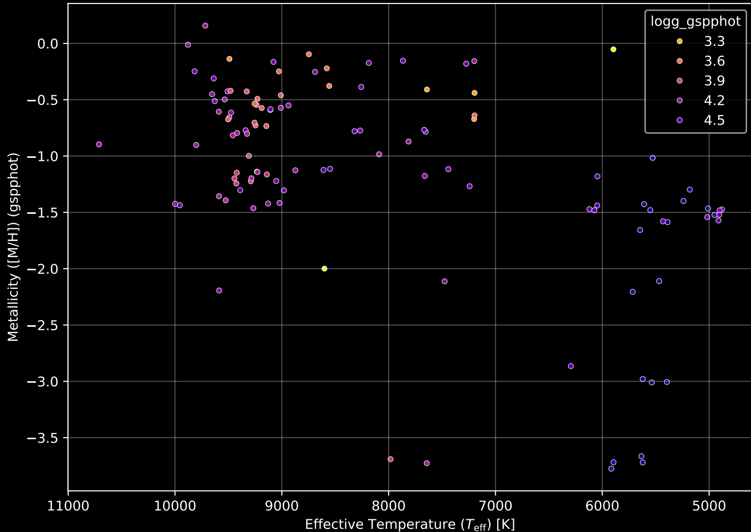
Gaia Cluster: [King_19] Stellar Population Parameters (n= 114)
