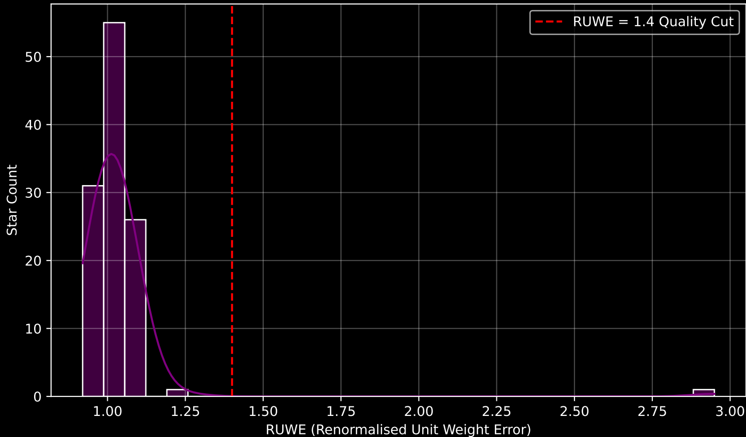
Gaia Cluster: [King_19] RUWE Distribution (n= 114)
