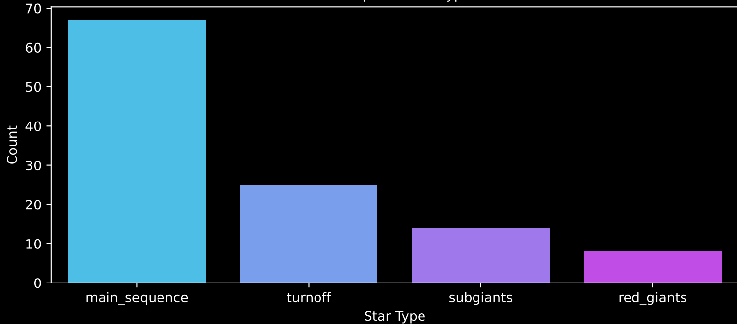
Gaia Cluster: [King_19] Count plot of Star Type
