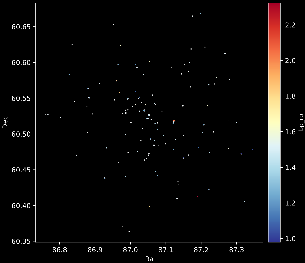
Gaia Cluster: [King_19] Stars: 114
