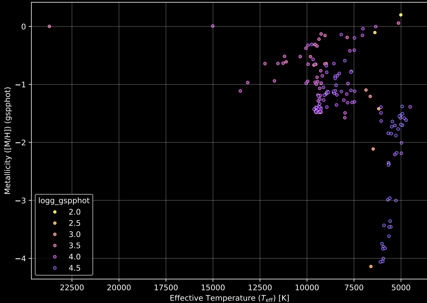
Gaia Cluster: [King_21] Stellar Population Parameters (n= 163)
