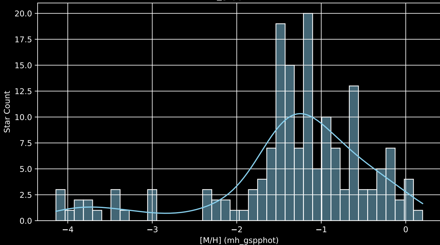
Gaia Cluster: [King_21 [M/H] (mh_gspphot) (n= 163)
