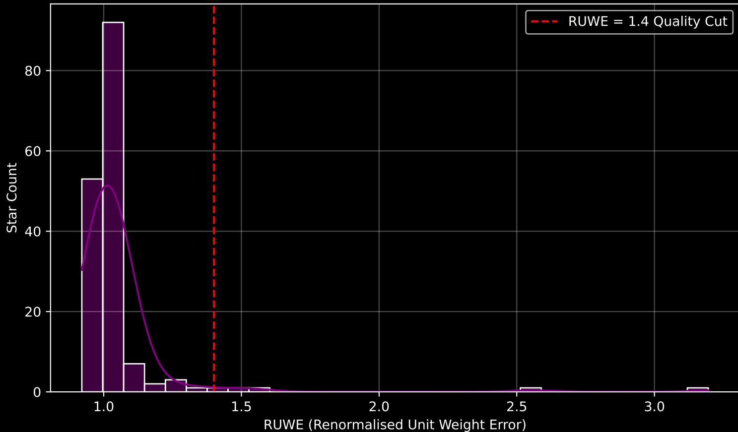
Gaia Cluster: [King_21] RUWE Distribution (n= 163)
