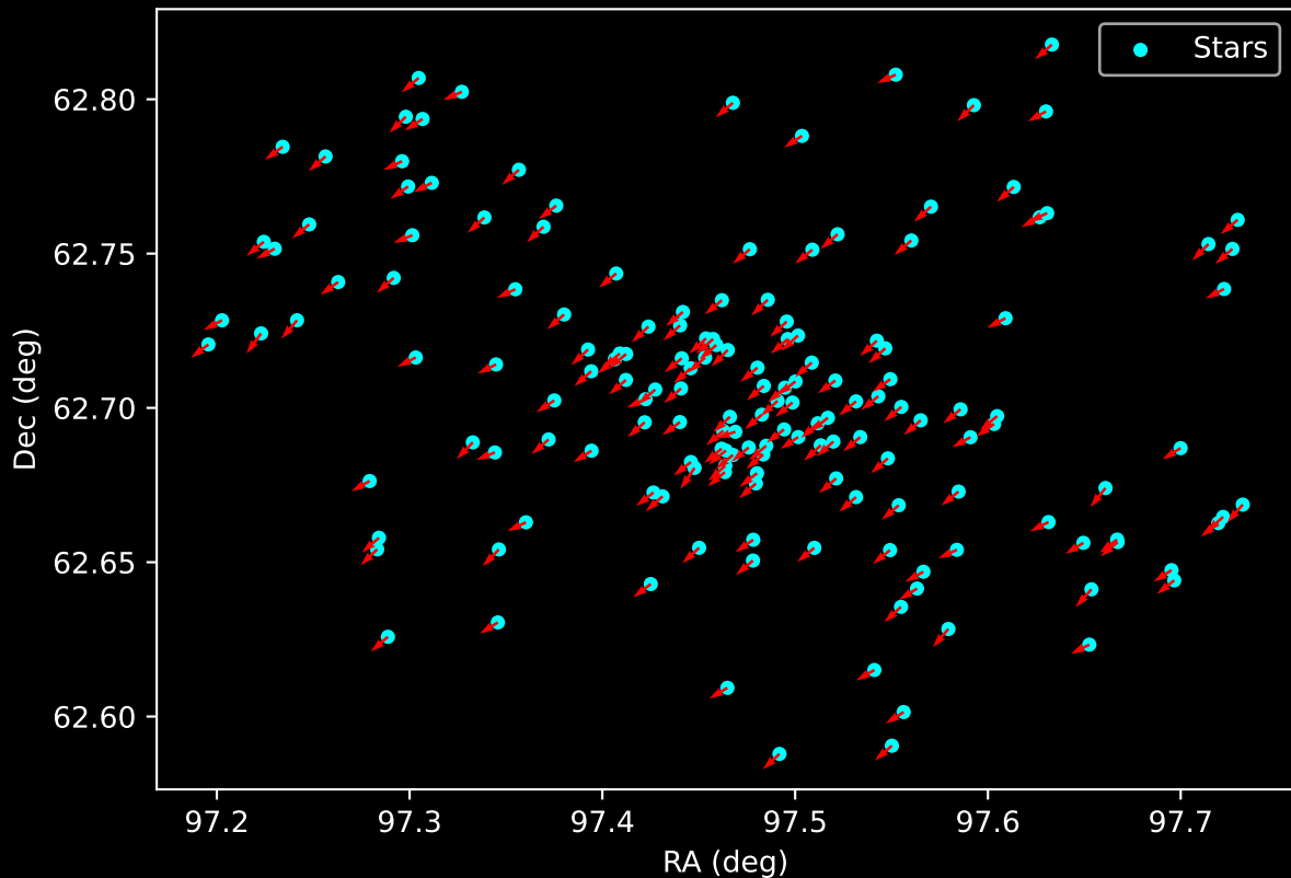
Gaia Cluster: [King_21] Proper Motion Vectors for Gaia Star Field (n= 163)
