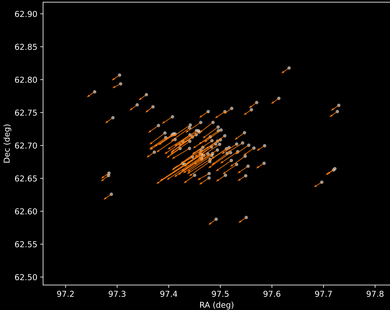
Gaia DR3 Cluster 2 Proper Motion Vectors (n=95)
