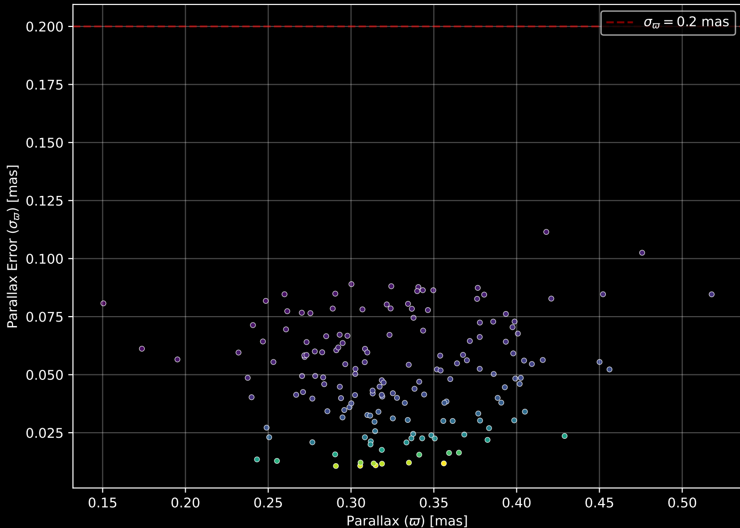
Gaia Cluster: [King_21] Parallax Quality (n= 163)
