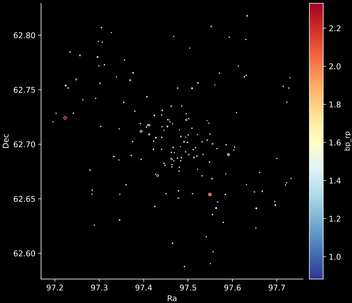
Gaia Cluster: [King_21] Stars: 163
