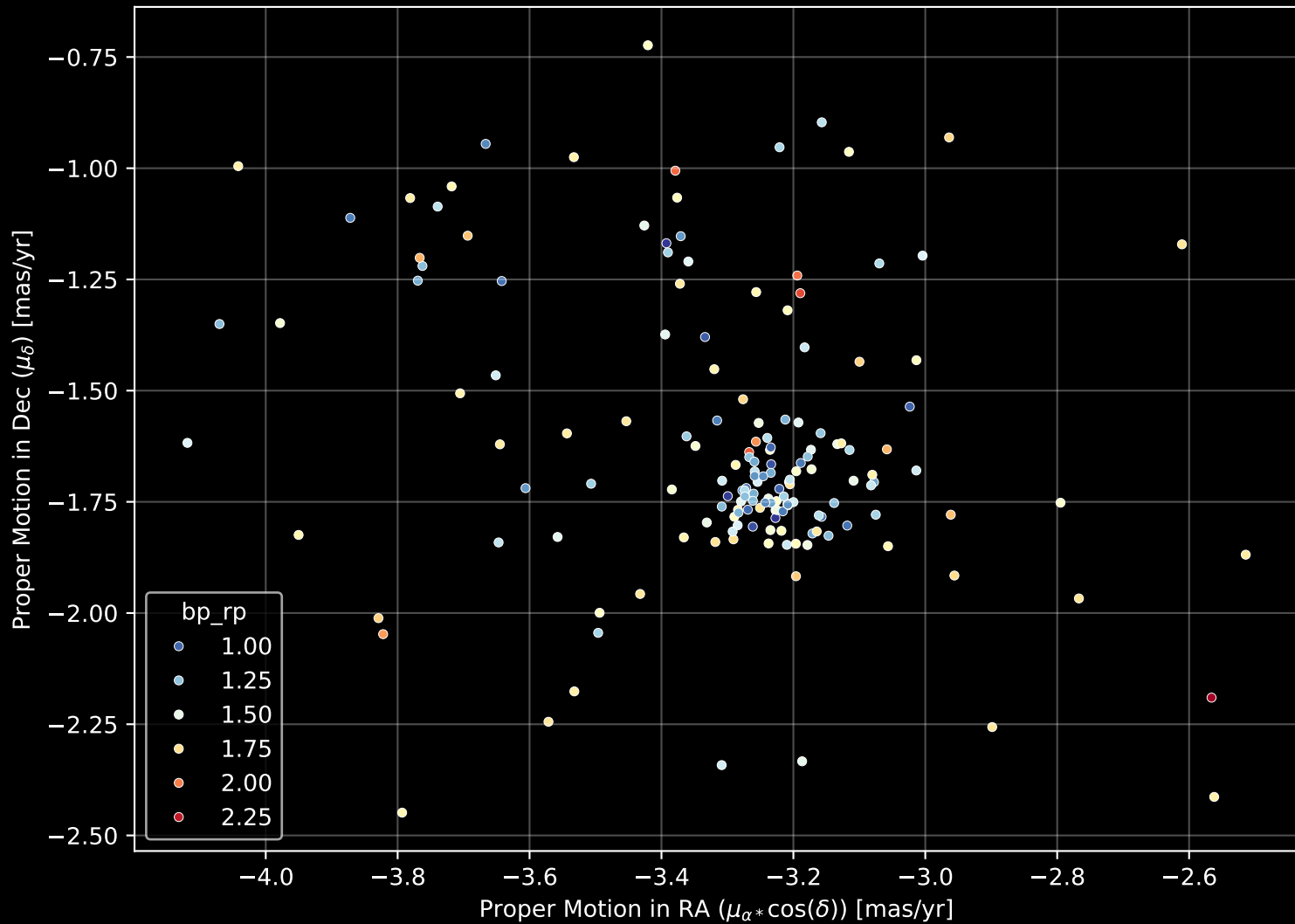
Gaia Cluster: [King_21] Proper Motion Diagram (n= 163)
