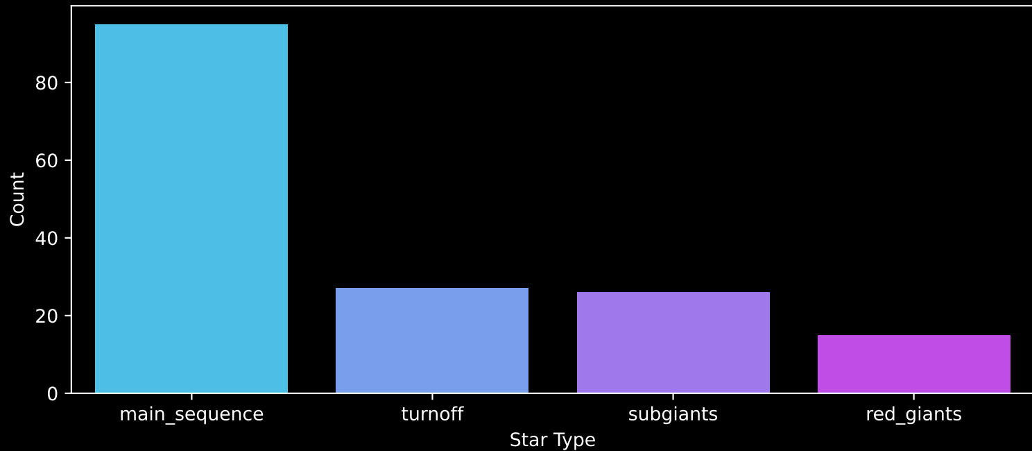
Gaia Cluster: [King_21] Count plot of Star Type
