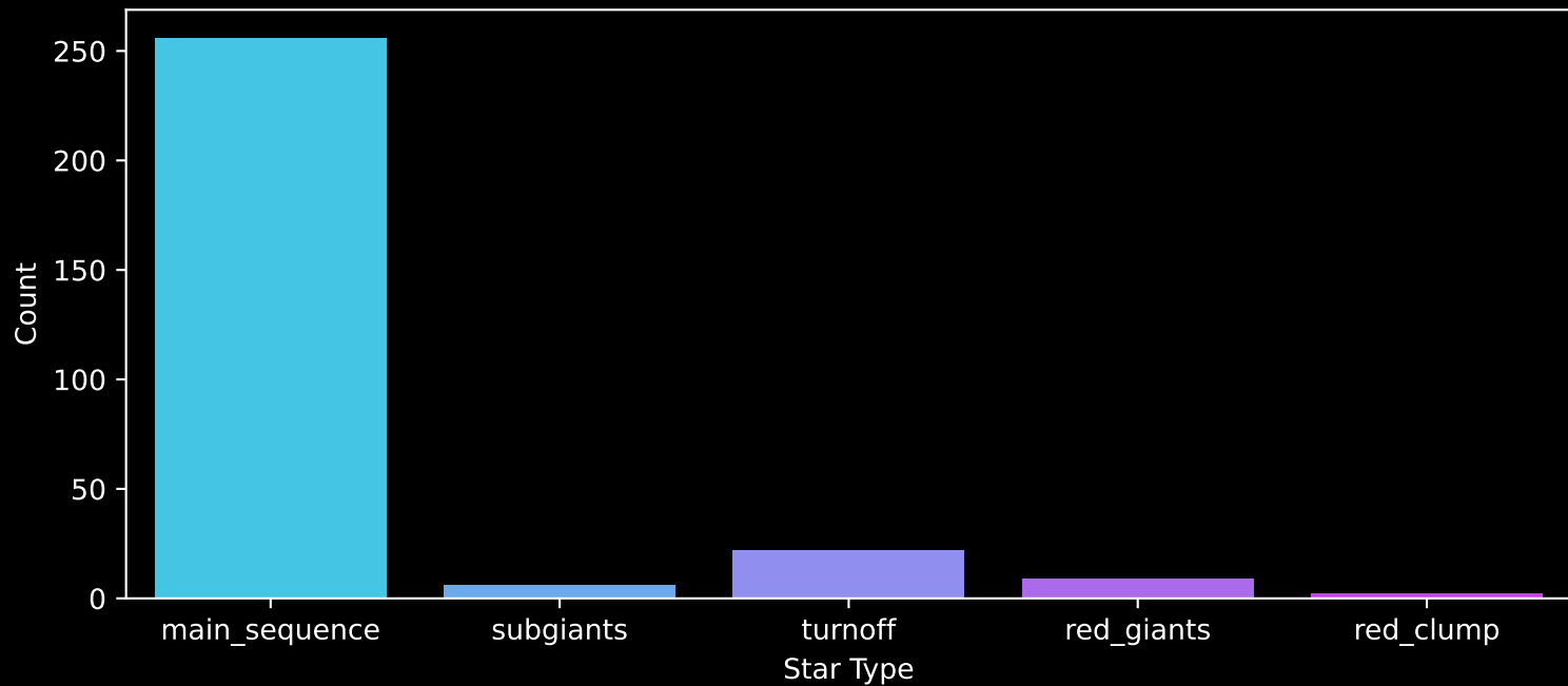
Gaia Cluster: [King_23] Count plot of Star Type
