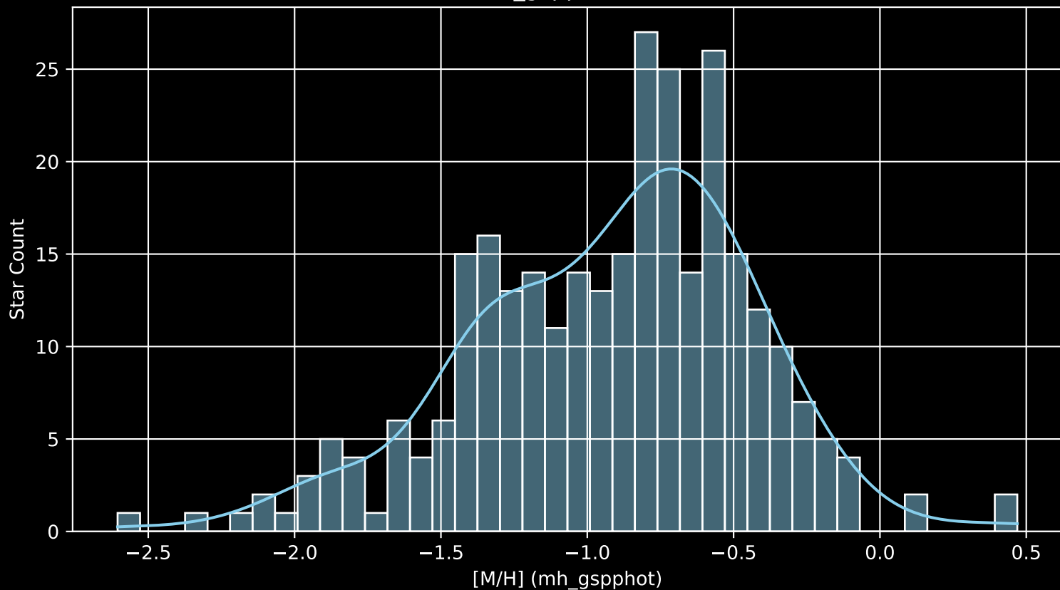
Gaia Cluster: [King_23 [M/H] (mh_gspphot) (n= 295)
