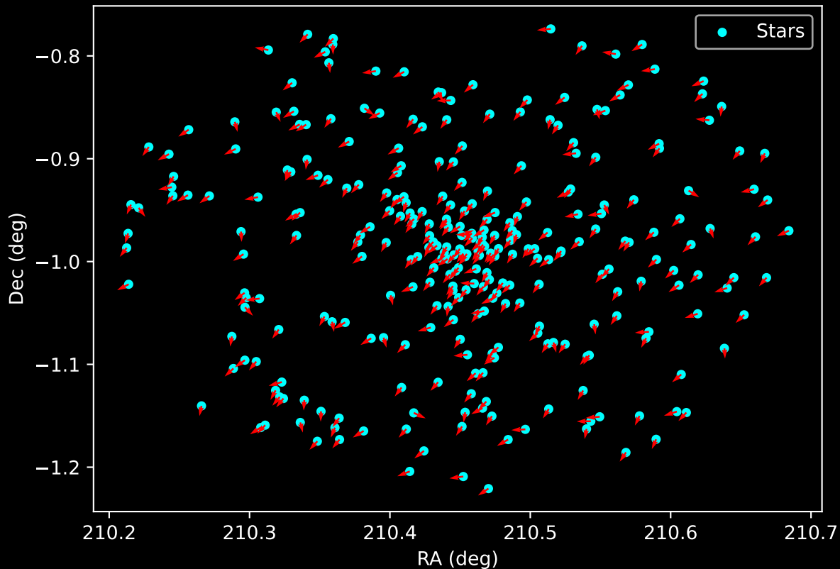
Gaia Cluster: [King_23] Proper Motion Vectors for Gaia Star Field (n= 295)
