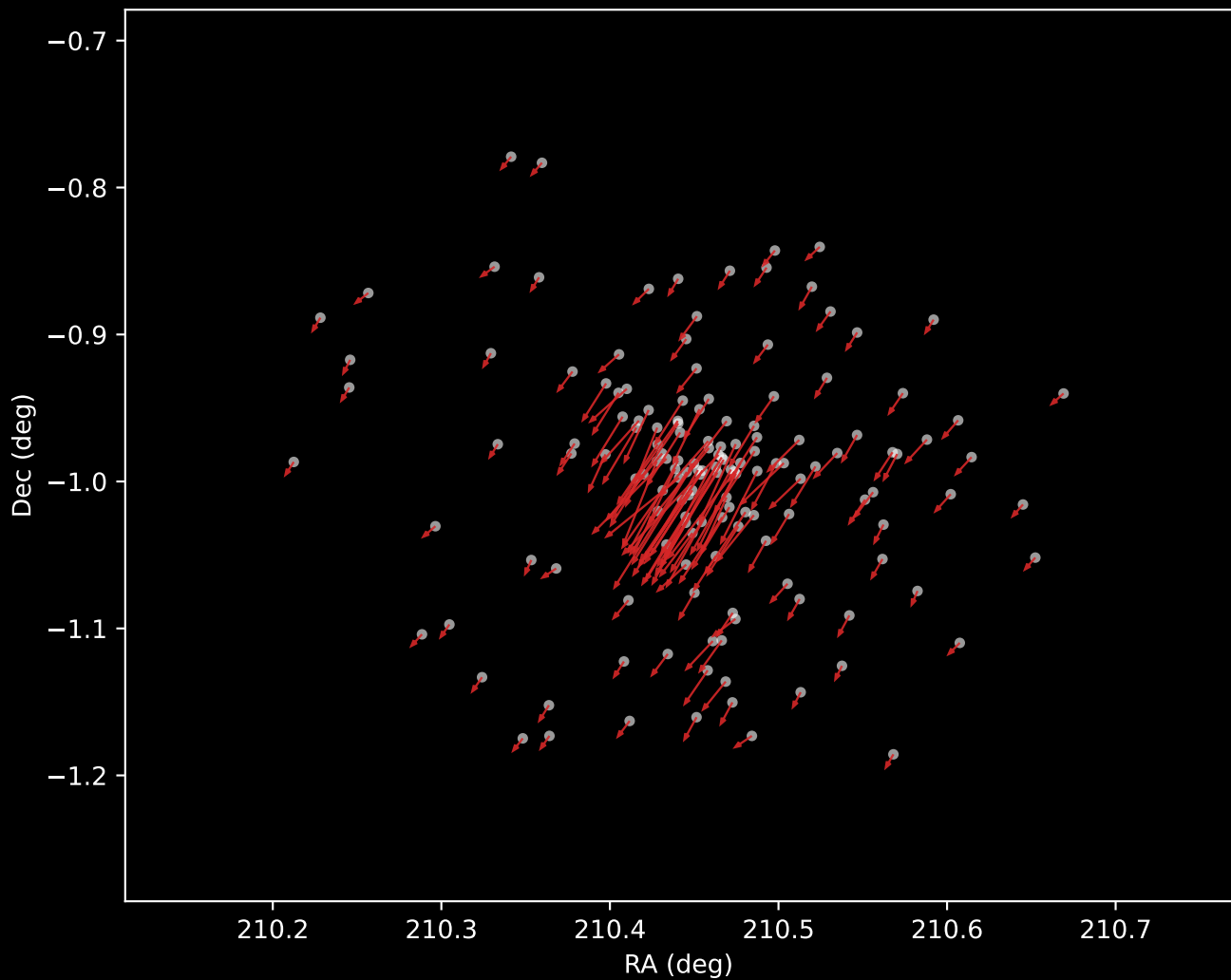
Gaia DR3 Cluster 6 Proper Motion Vectors (n=150)
