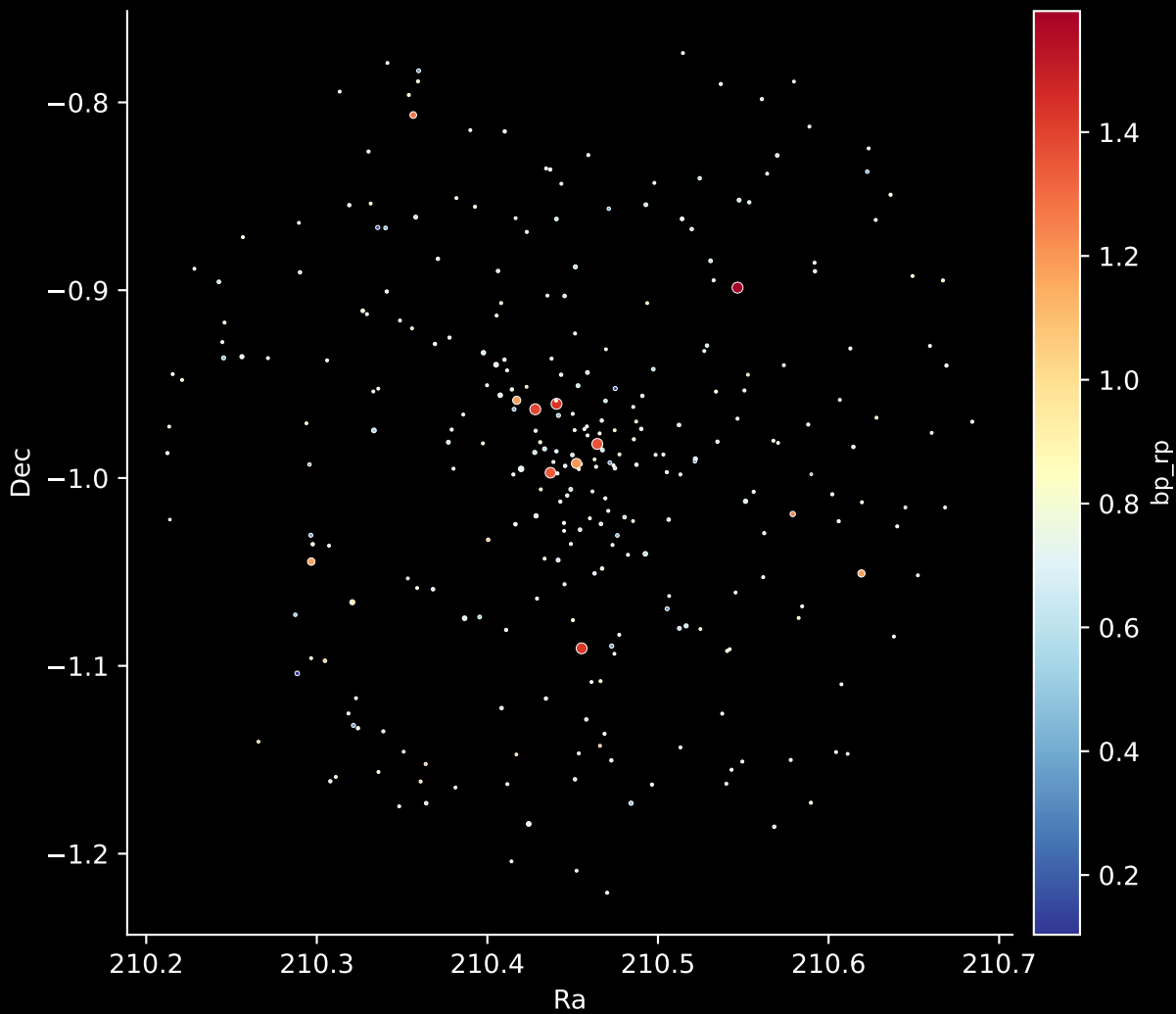
Gaia Cluster: [King_23] Stars: 295
