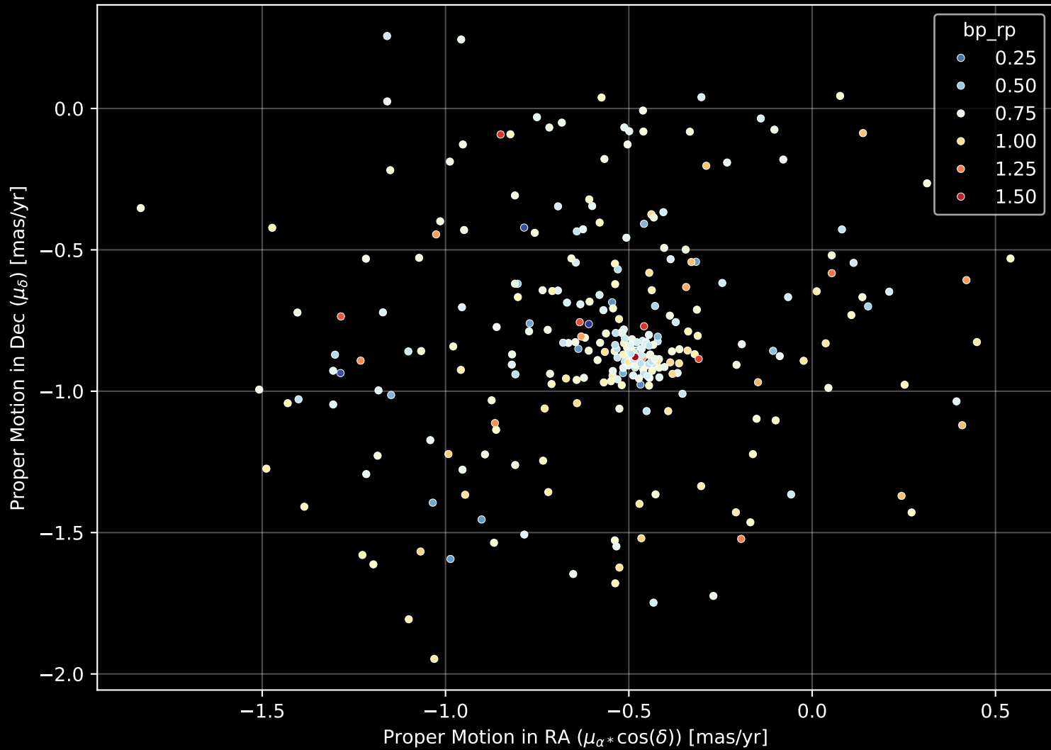
Gaia Cluster: [King_23] Proper Motion Diagram (n= 295)
