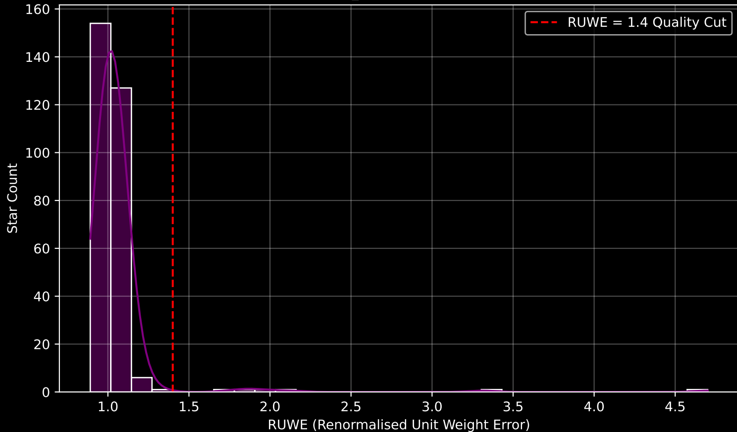
Gaia Cluster: [King_23] RUWE Distribution (n= 294)
