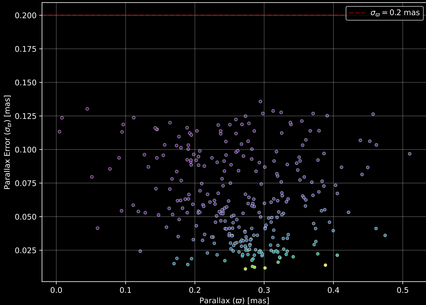
Gaia Cluster: [King_23] Parallax Quality (n= 295)
