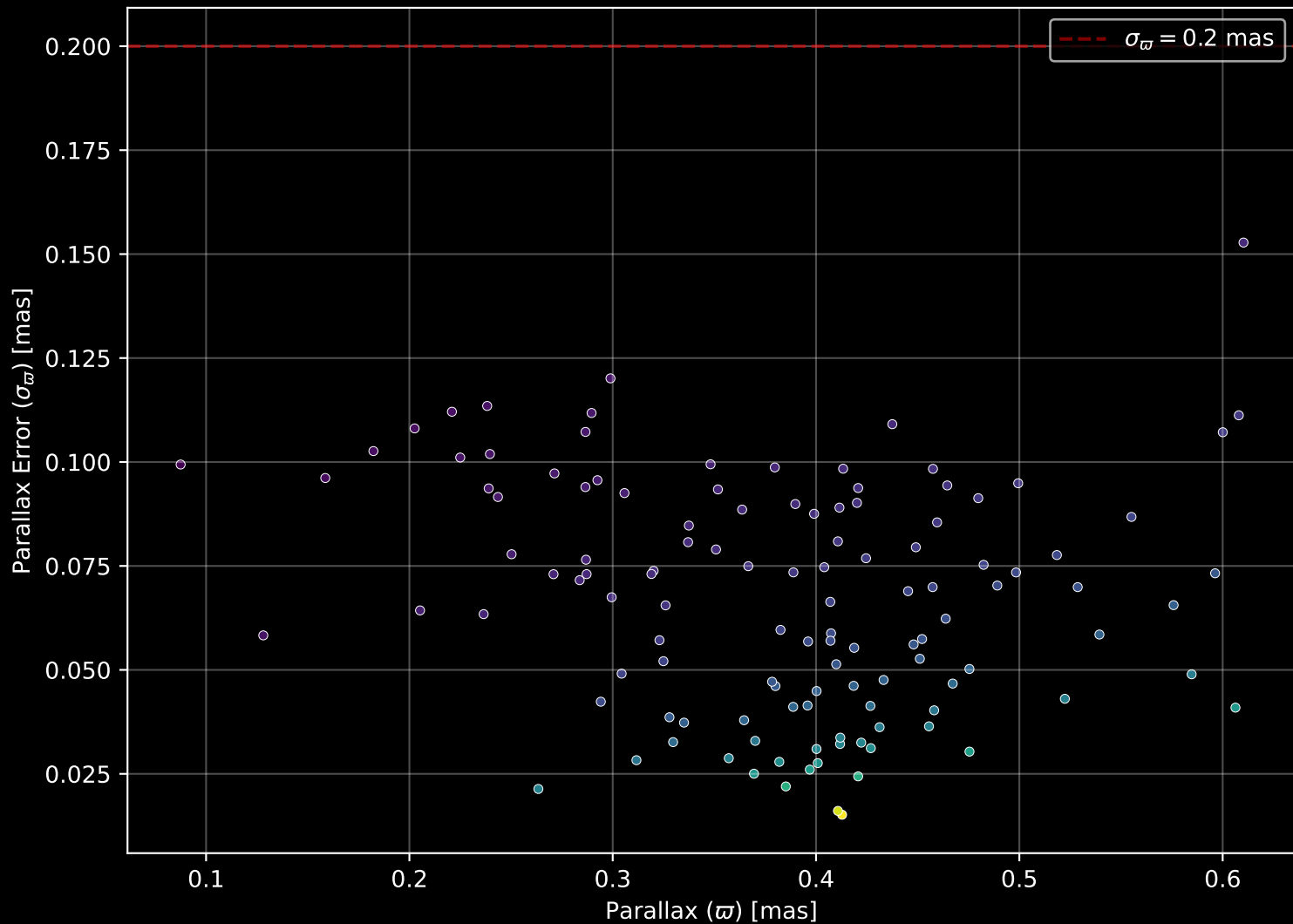
Gaia Cluster: [King_26] Parallax Quality (n= 121)
