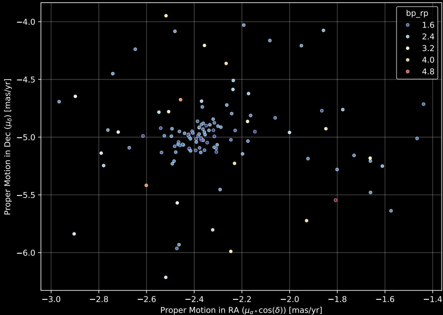
Gaia Cluster: [King_26] Proper Motion Diagram (n= 121)
