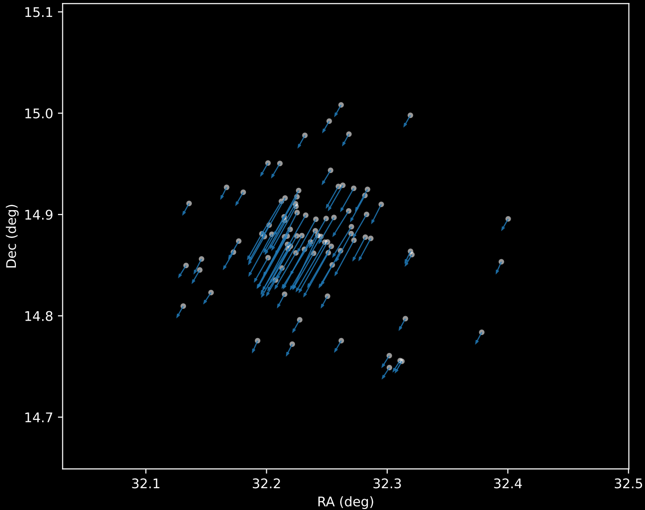
Gaia DR3 Cluster 0 Proper Motion Vectors (n=88)
