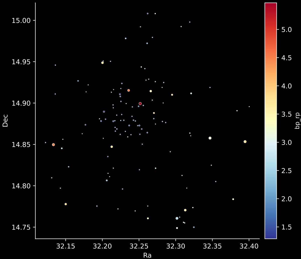
Gaia Cluster: [King_26] Stars: 121
