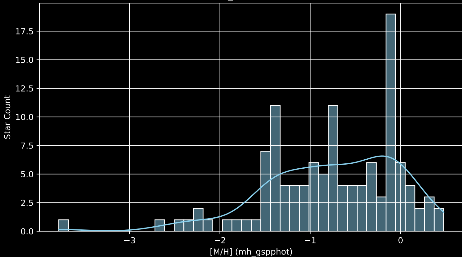
Gaia Cluster: [King_26 [M/H] (mh_gspphot) (n= 120)
