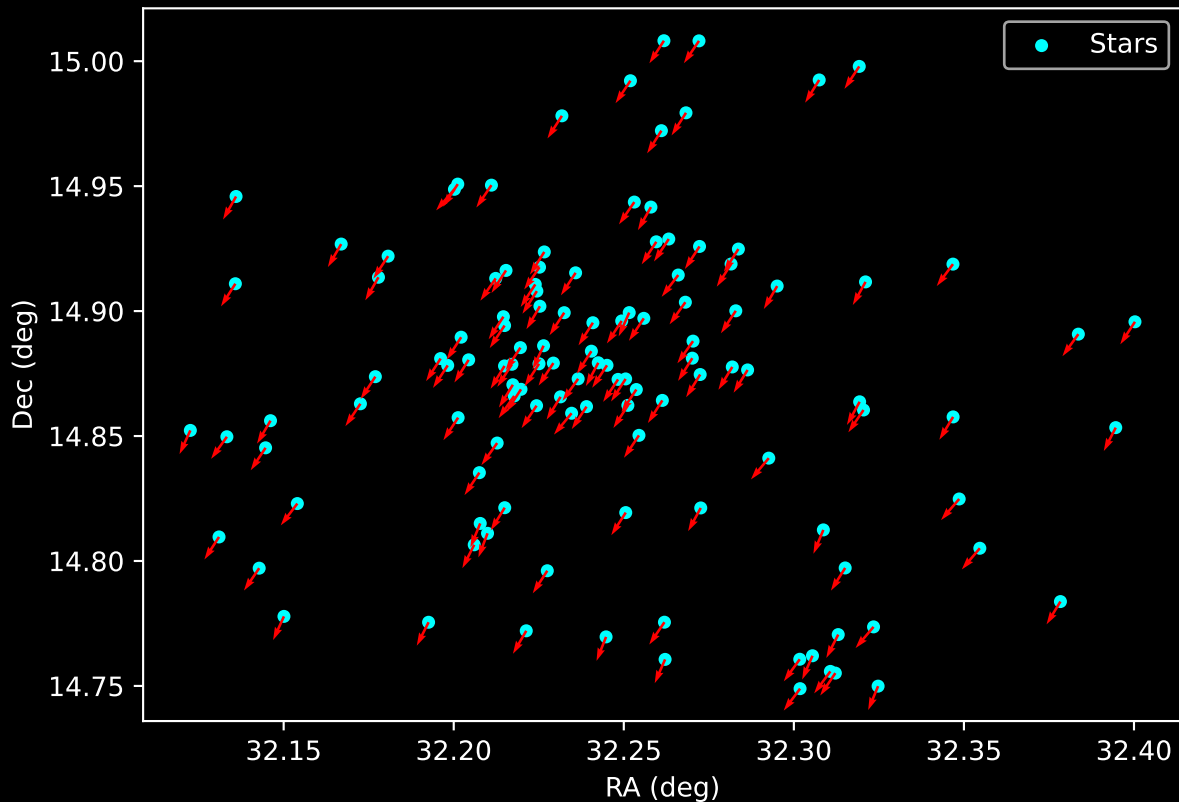
Gaia Cluster: [King_26] Proper Motion Vectors for Gaia Star Field (n= 121)
