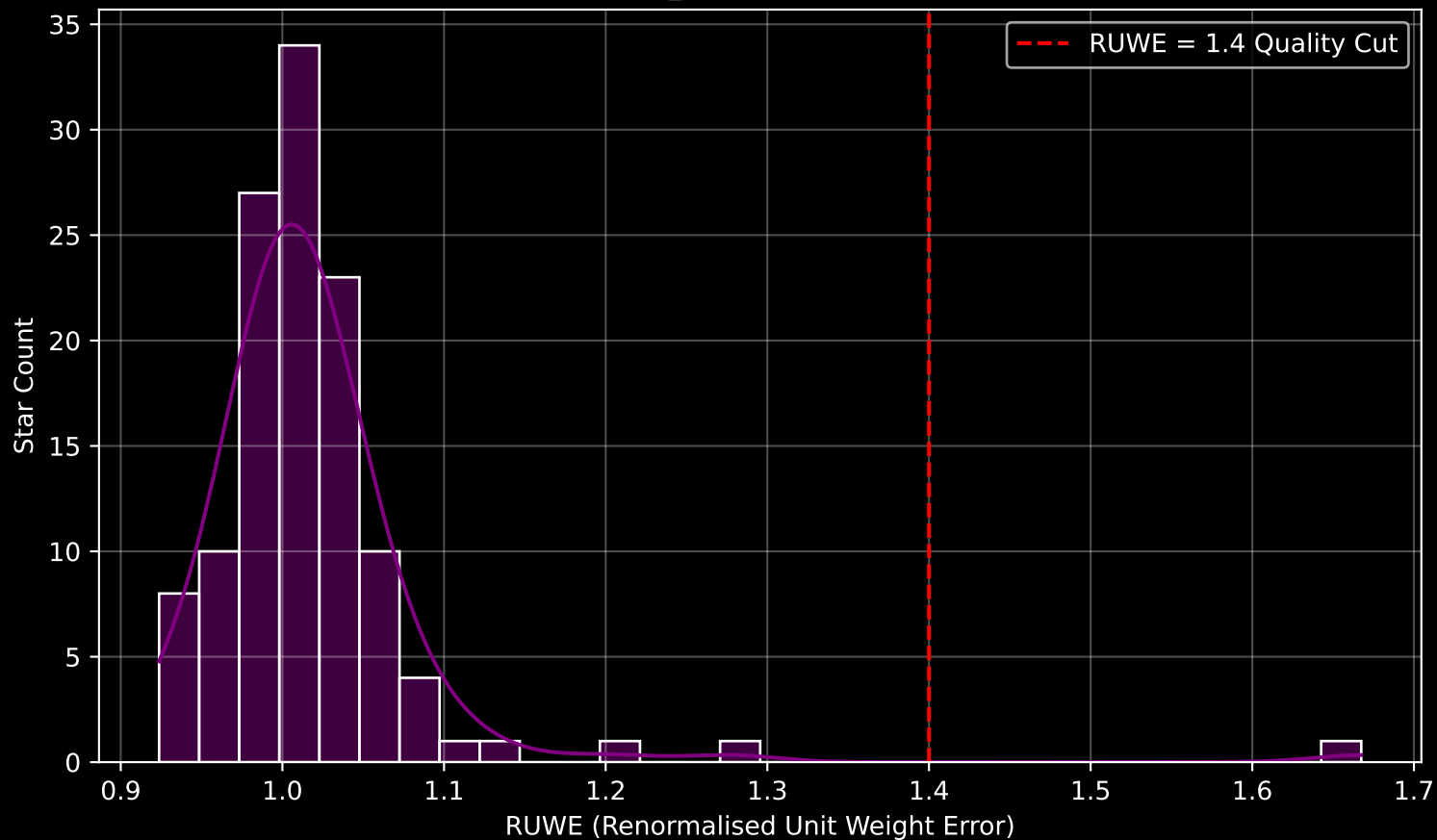
Gaia Cluster: [King_26] RUWE Distribution (n= 121)
