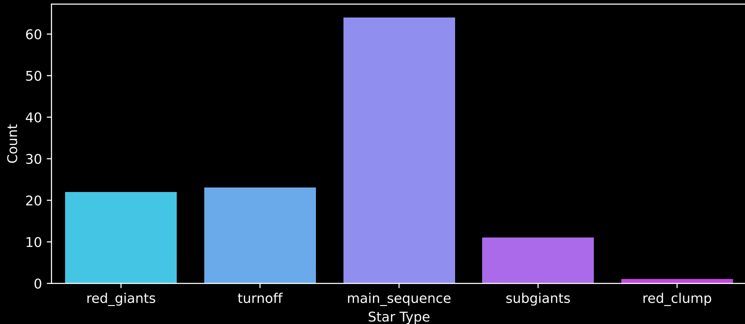
Gaia Cluster: [King_26] Count plot of Star Type
