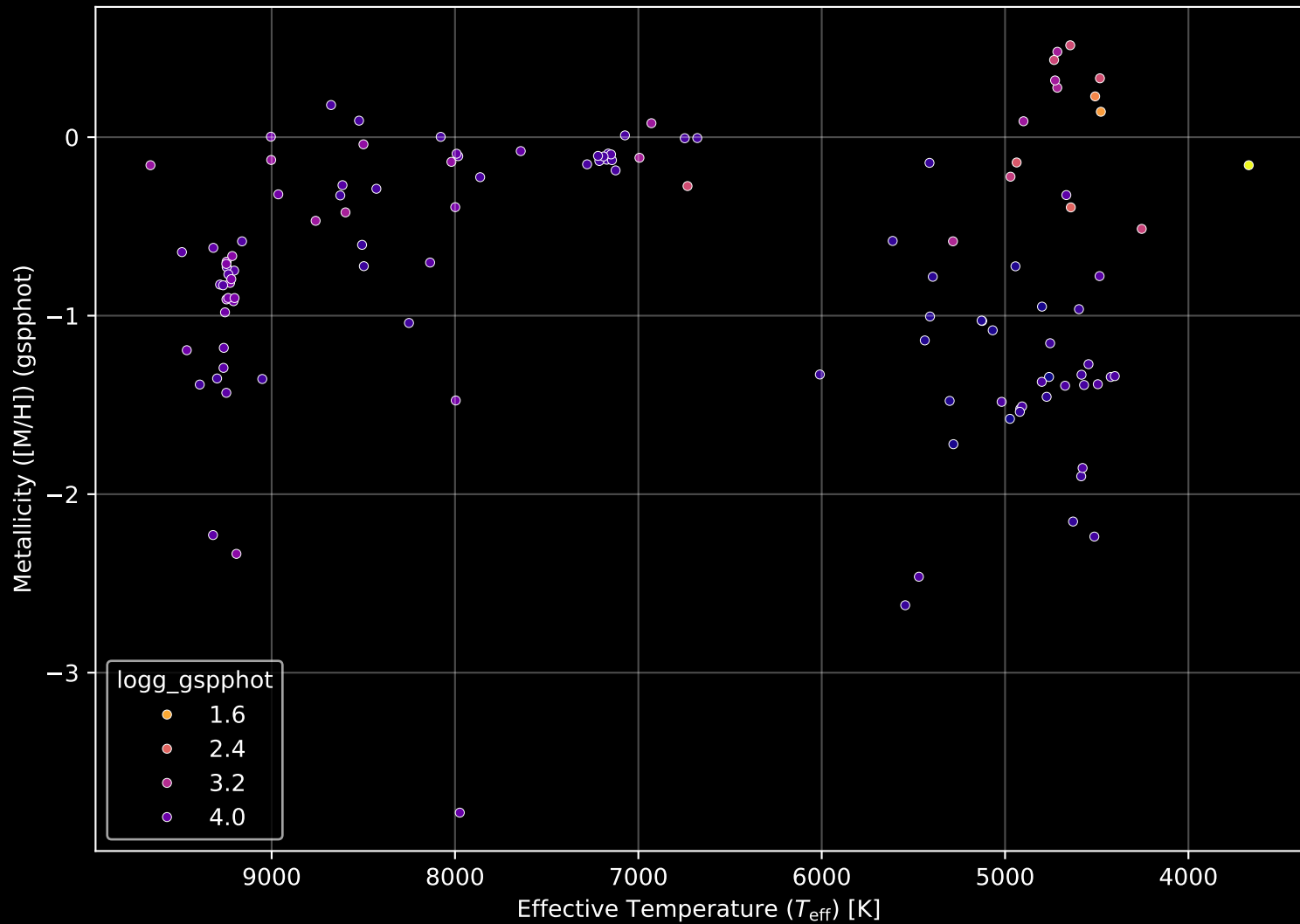
Gaia Cluster: [King_26] Stellar Population Parameters (n= 121)
