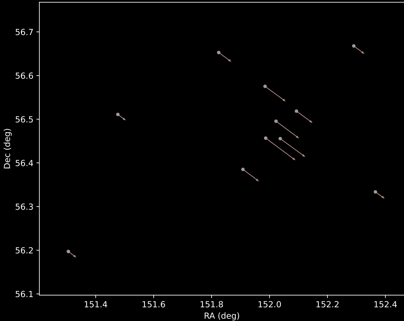
Gaia DR3 Cluster 11 Proper Motion Vectors (n=11)
