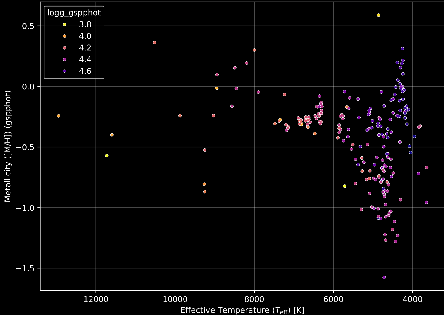
Gaia Cluster: [King_6] Stellar Population Parameters (n= 213)
