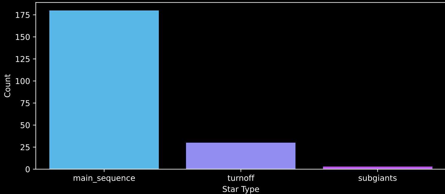
Gaia Cluster: [King_6] Count plot of Star Type
