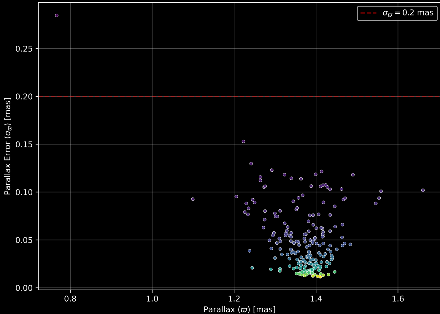
Gaia Cluster: [King_6] Parallax Quality (n= 213)
