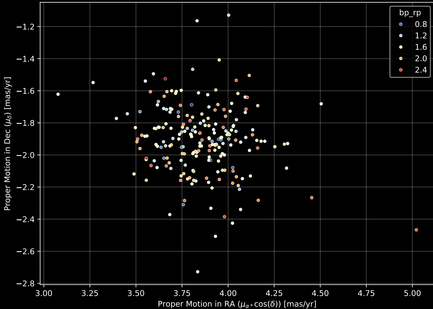
Gaia Cluster: [King_6] Proper Motion Diagram (n= 213)
