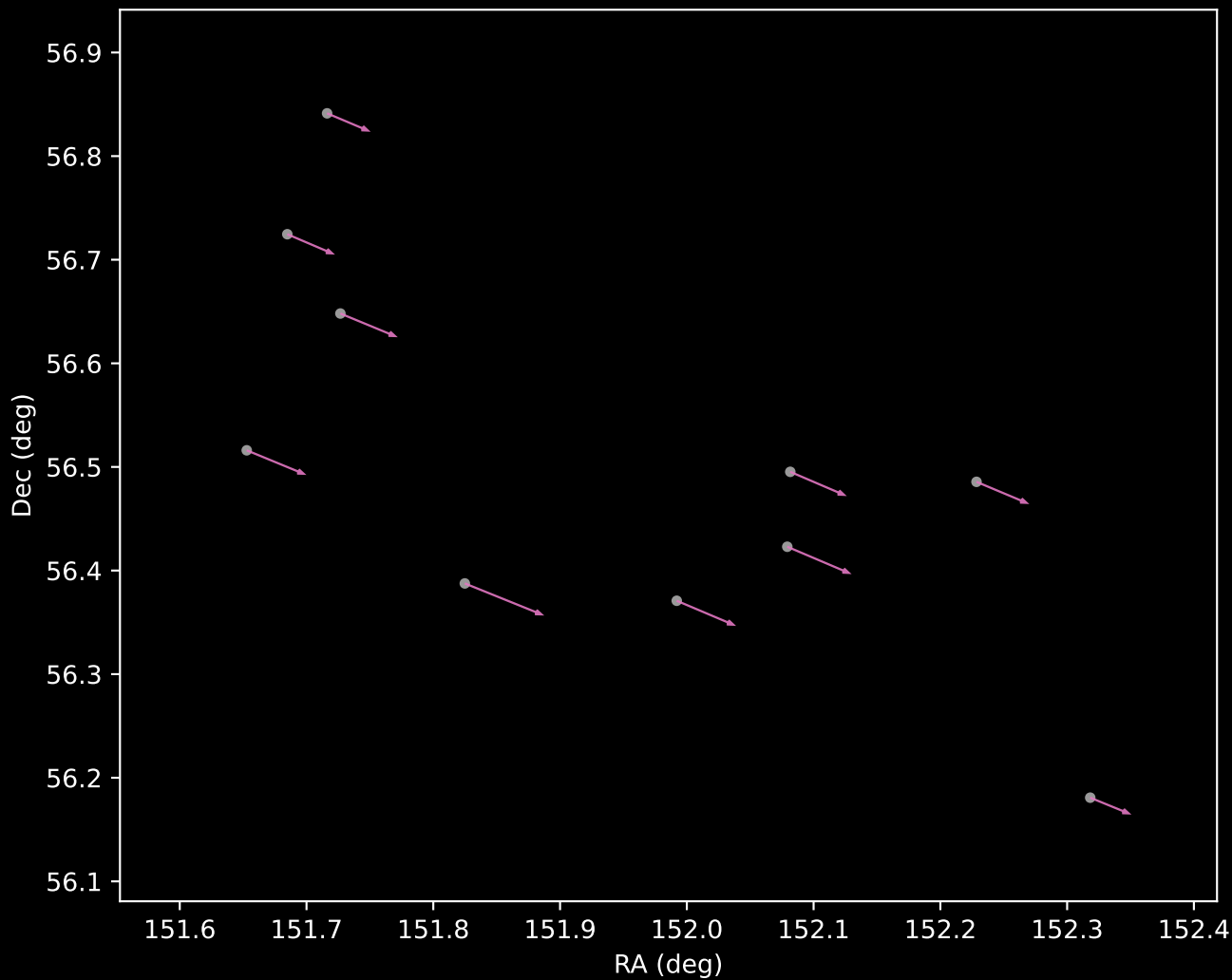
Gaia DR3 Cluster 12 Proper Motion Vectors (n=10)
