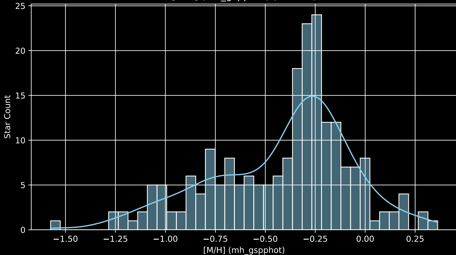
Gaia Cluster: [King_6 [M/H] (mh_gspphot) (n= 212)
