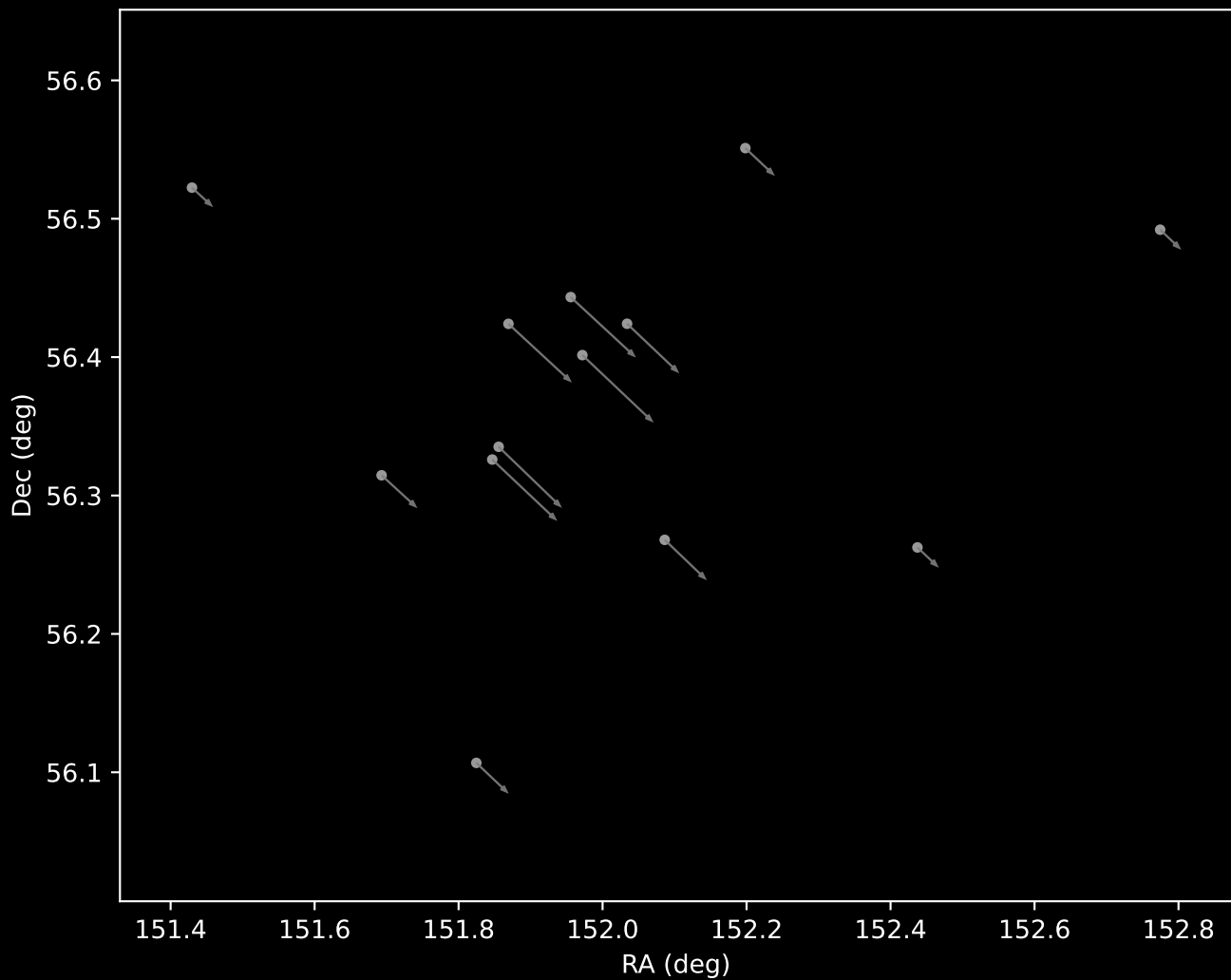
Gaia DR3 Cluster 14 Proper Motion Vectors (n=13)
