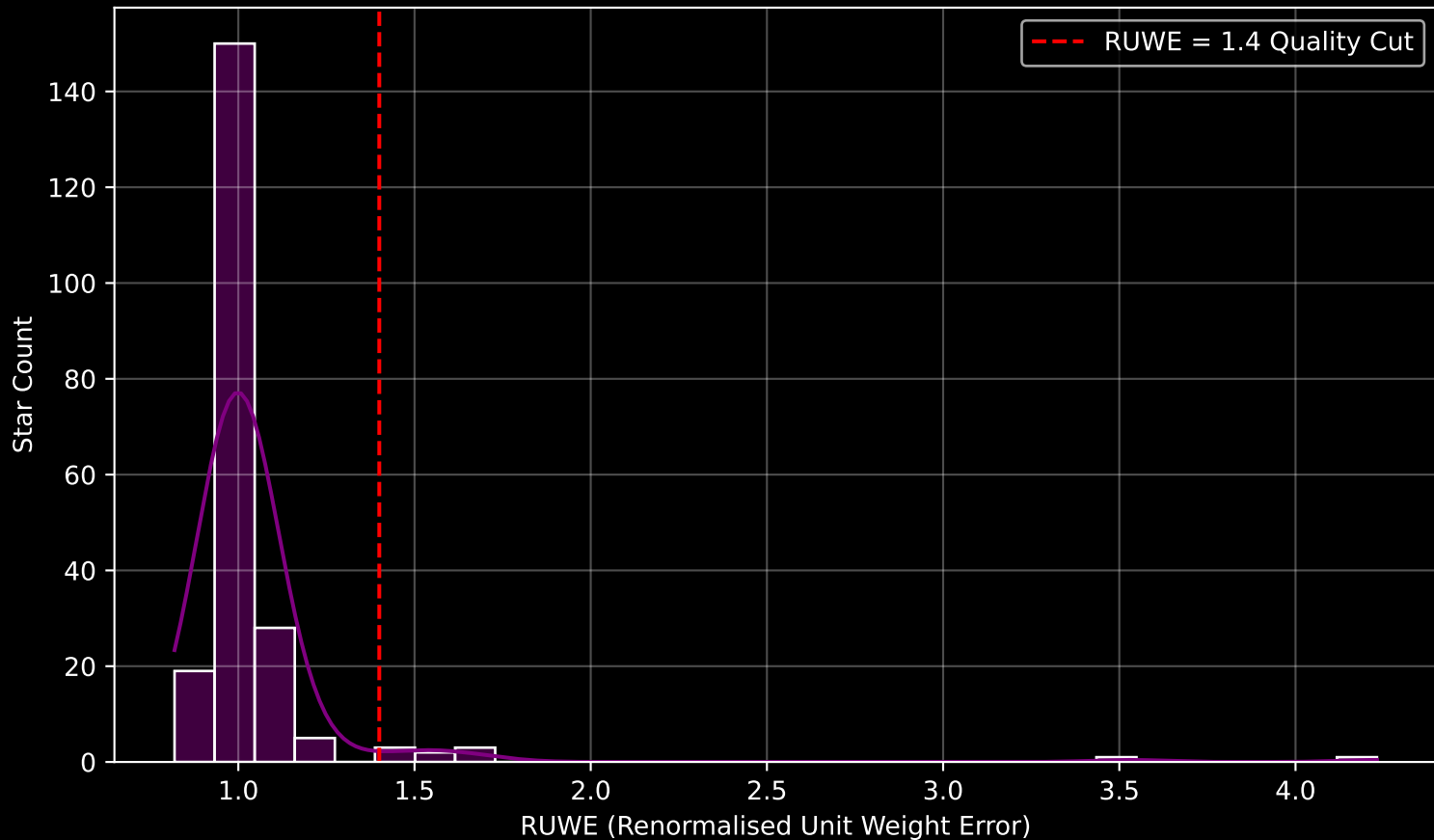
Gaia Cluster: [King_6] RUWE Distribution (n= 212)
