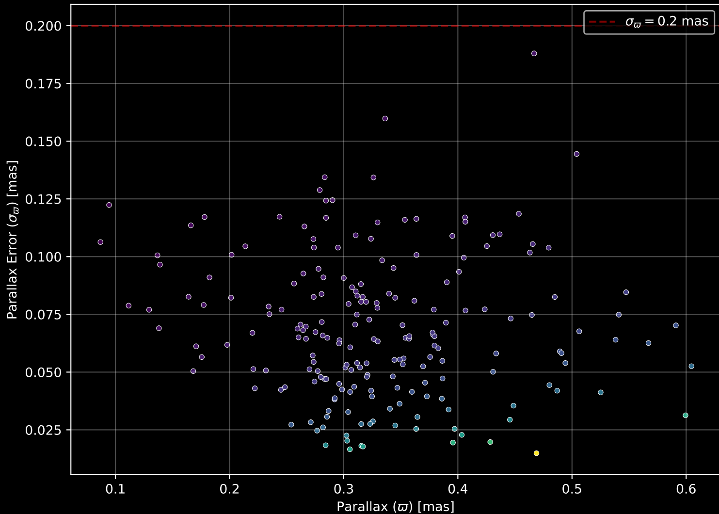
Gaia Cluster: [King_7] Parallax Quality (n= 200)
