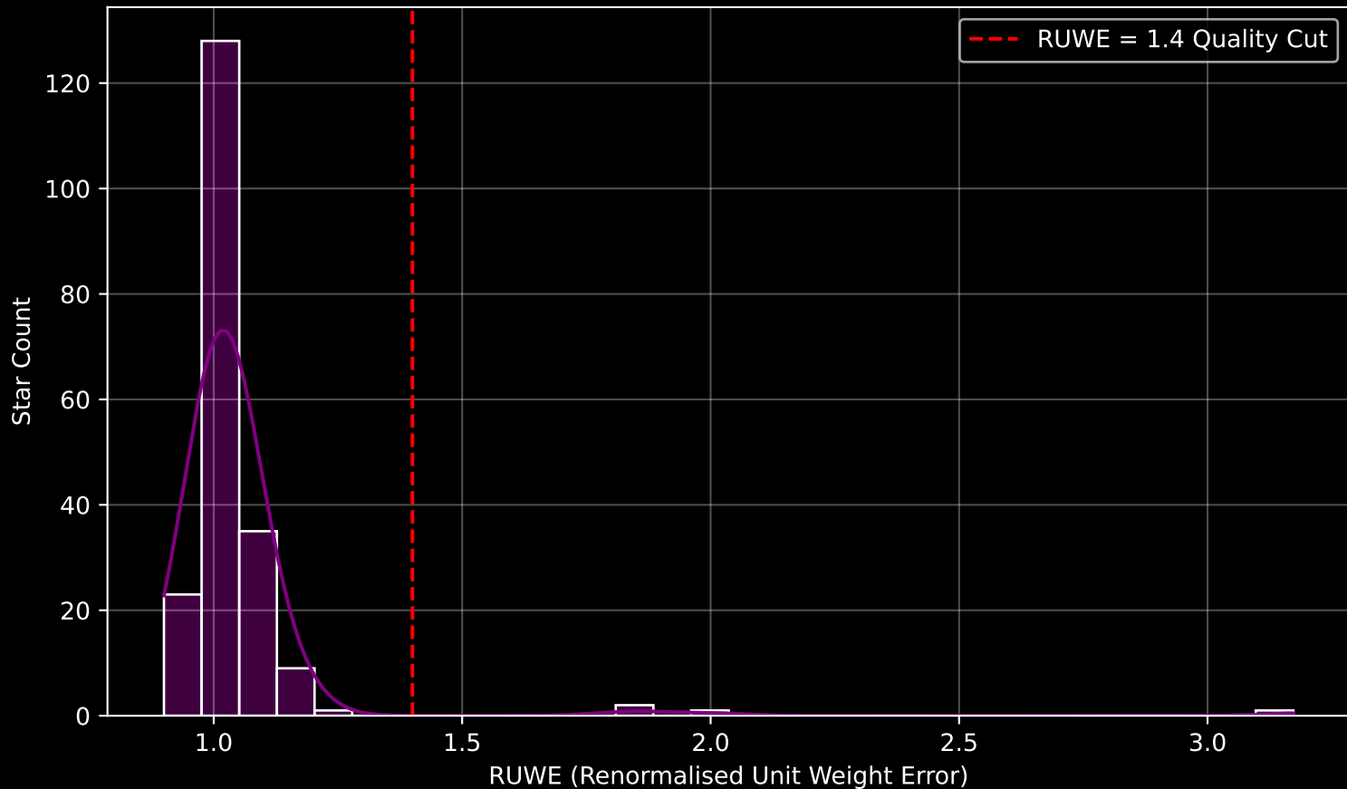
Gaia Cluster: [King_7] RUWE Distribution (n= 200)
