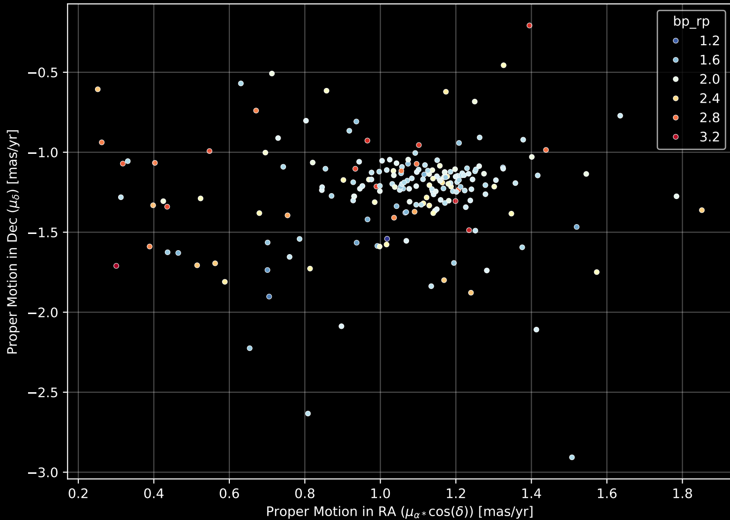
Gaia Cluster: [King_7] Proper Motion Diagram (n= 200)
