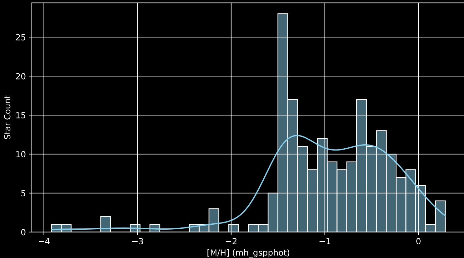
Gaia Cluster: [King_7 [M/H] (mh_gspphot) (n= 198)
