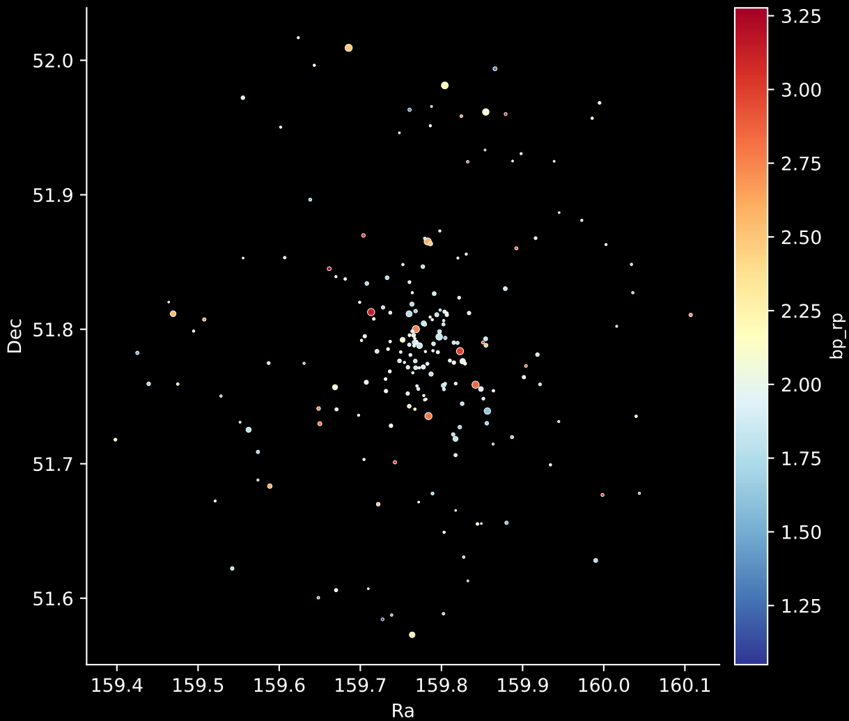
Gaia Cluster: [King_7] Stars: 200
