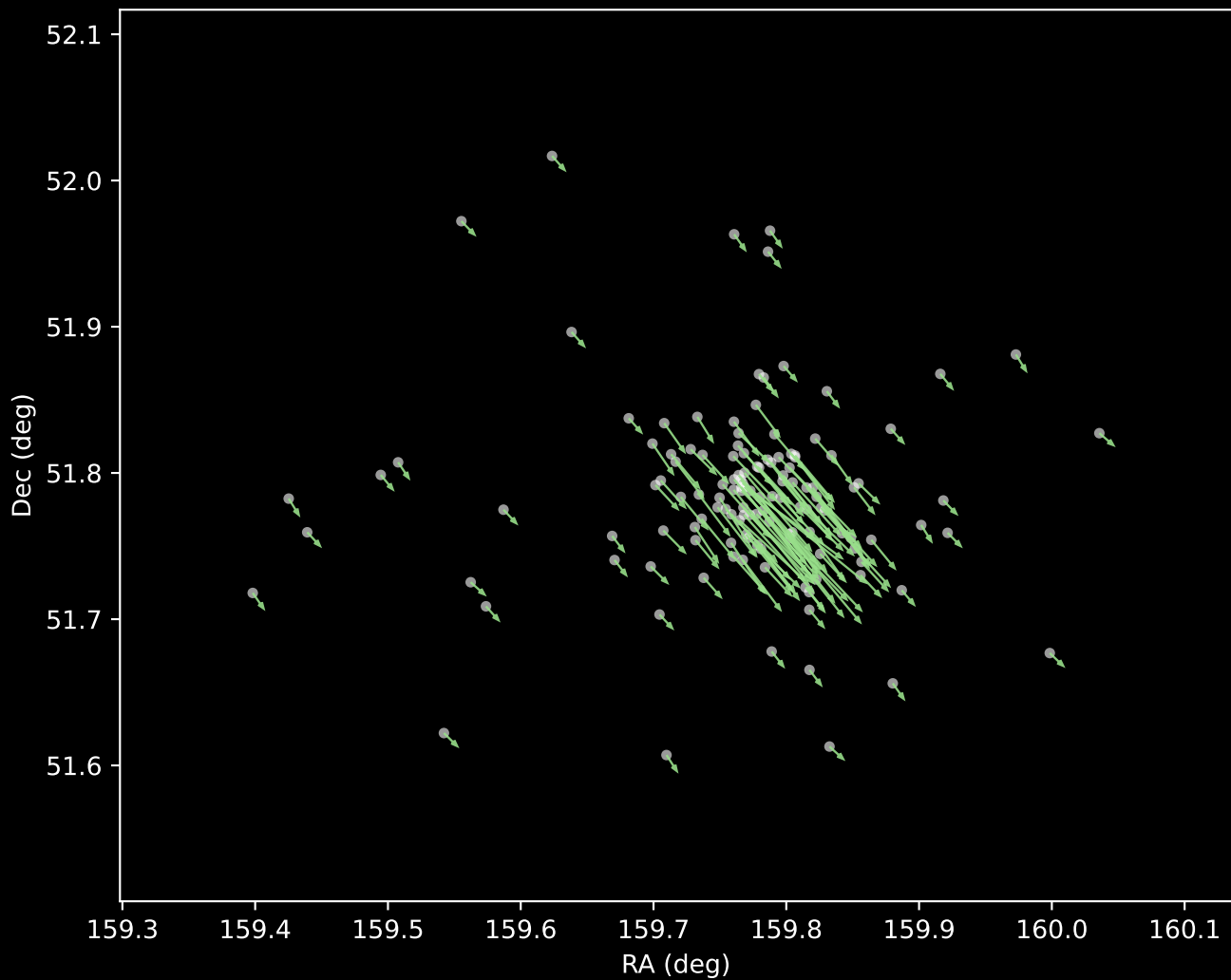
Gaia DR3 Cluster 5 Proper Motion Vectors (n=132)
