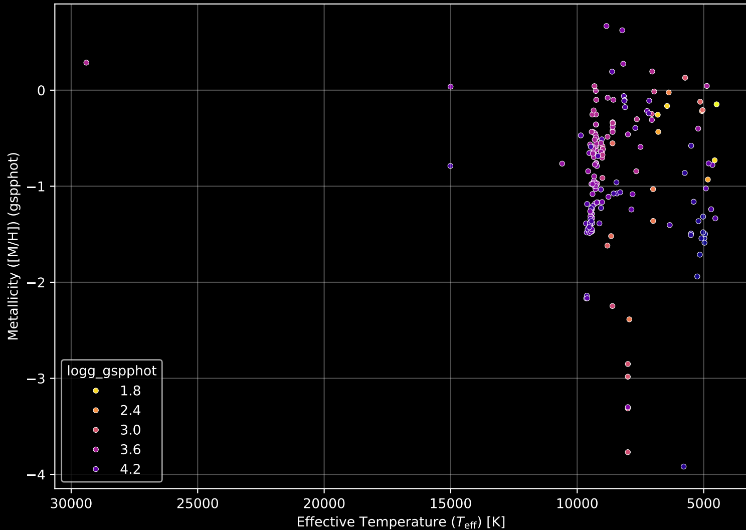
Gaia Cluster: [King_7] Stellar Population Parameters (n= 200)
