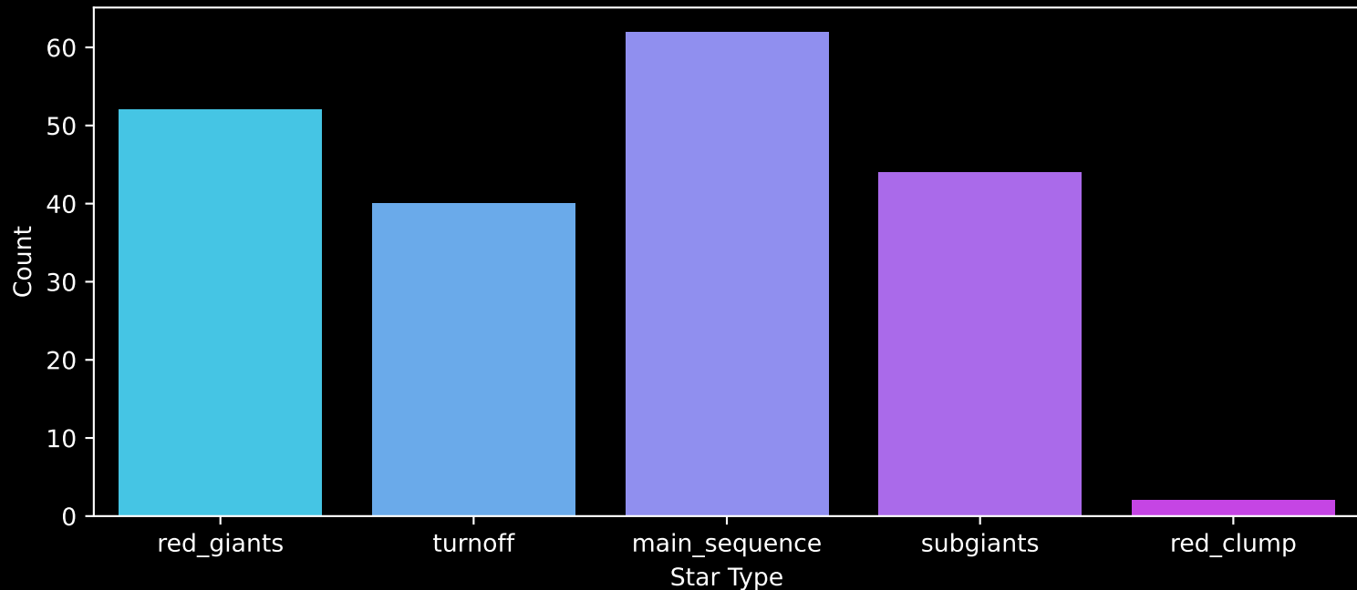
Gaia Cluster: [King_7] Count plot of Star Type
