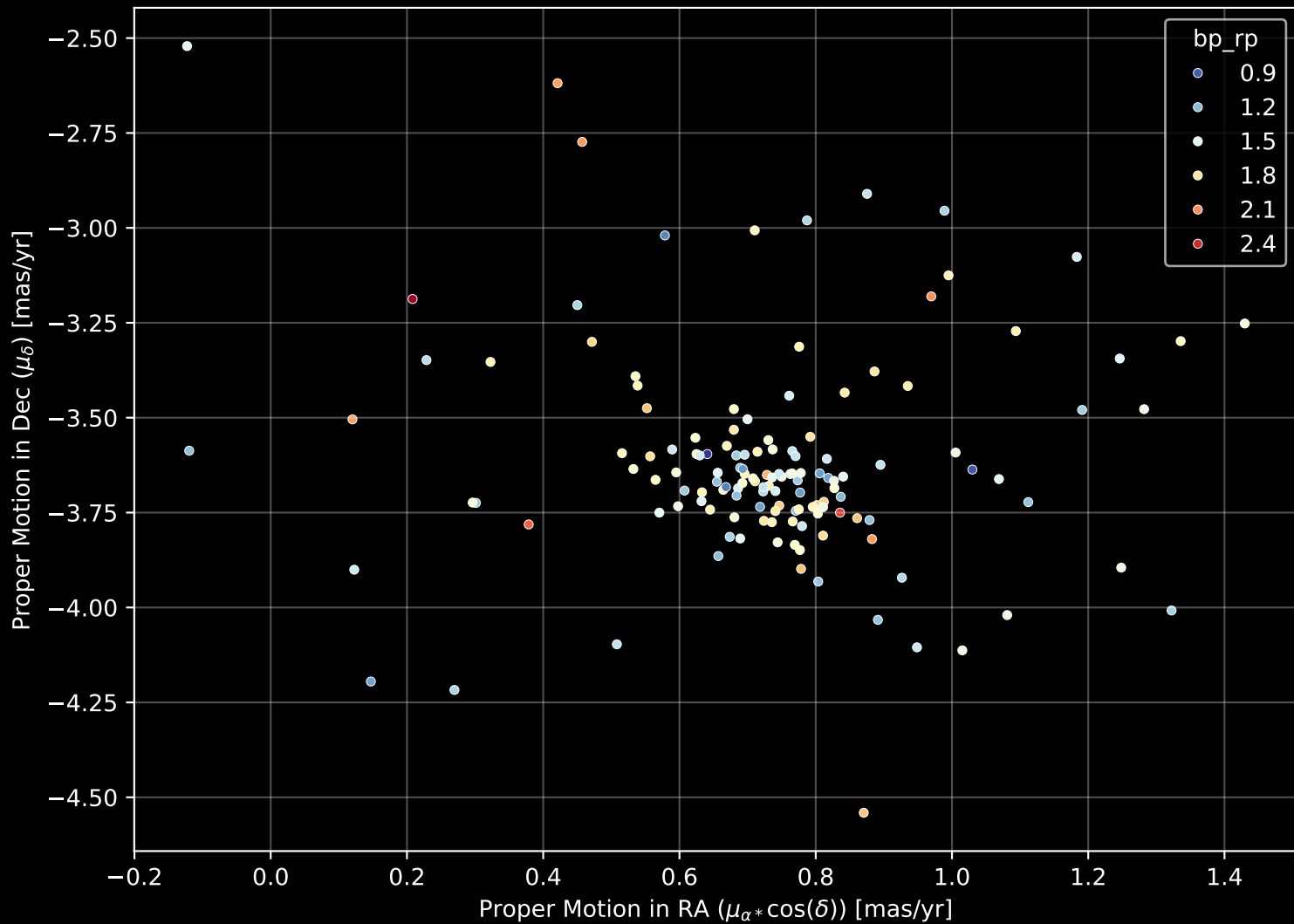
Gaia Cluster: [Koposov_36] Proper Motion Diagram (n= 140)
