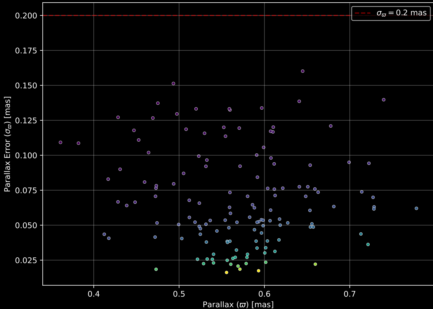
Gaia Cluster: [Koposov_36] Parallax Quality (n= 140)
