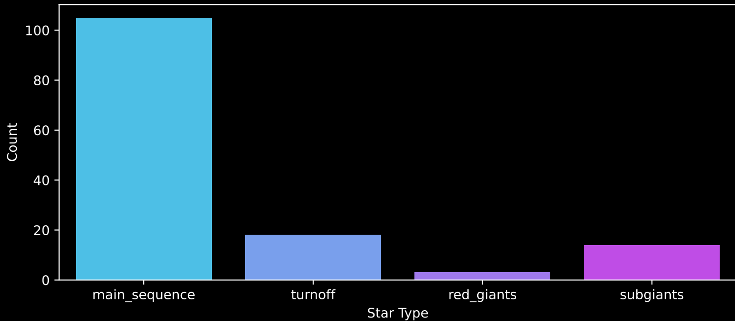
Gaia Cluster: [Koposov_36] Count plot of Star Type
