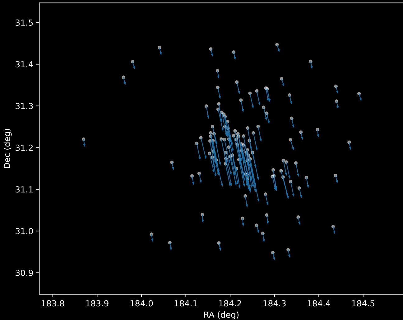
Gaia DR3 Cluster 0 Proper Motion Vectors (n=112)
