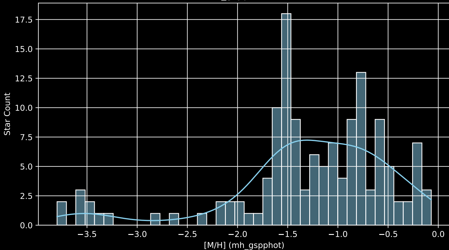
Gaia Cluster: [Koposov_36 [M/H] (mh_gspphot) (n= 139)
