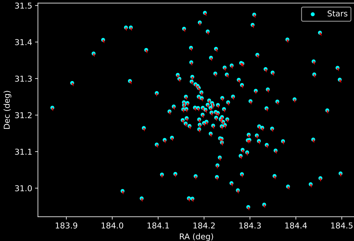
Gaia Cluster: [Koposov_36] Proper Motion Vectors for Gaia Star Field (n= 140)
