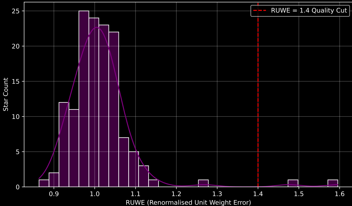
Gaia Cluster: [Koposov_36] RUWE Distribution (n= 139)
