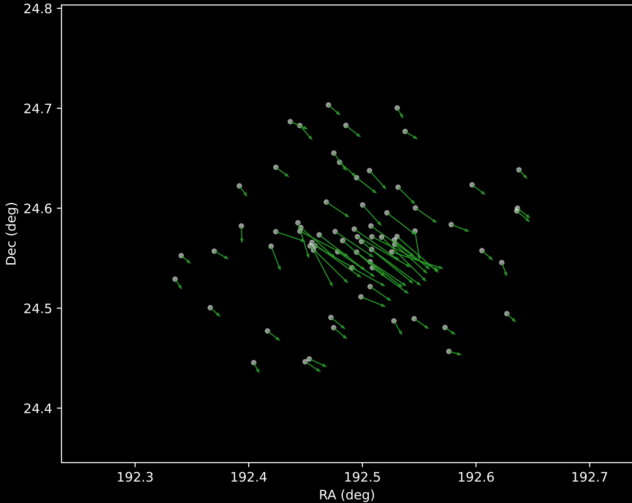
Gaia DR3 Cluster 4 Proper Motion Vectors (n=71)
