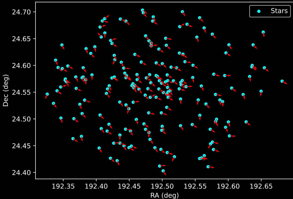
Gaia Cluster: [Koposov_63] Proper Motion Vectors for Gaia Star Field (n= 186)
