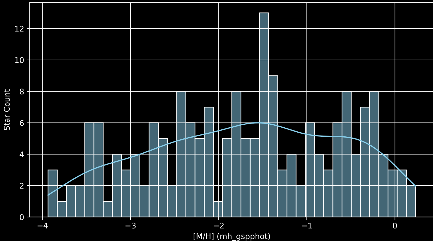
Gaia Cluster: [Koposov_63 [M/H] (mh_gspphot) (n= 186)
