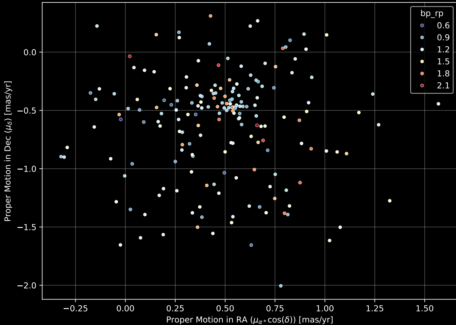
Gaia Cluster: [Koposov_63] Proper Motion Diagram (n= 186)
