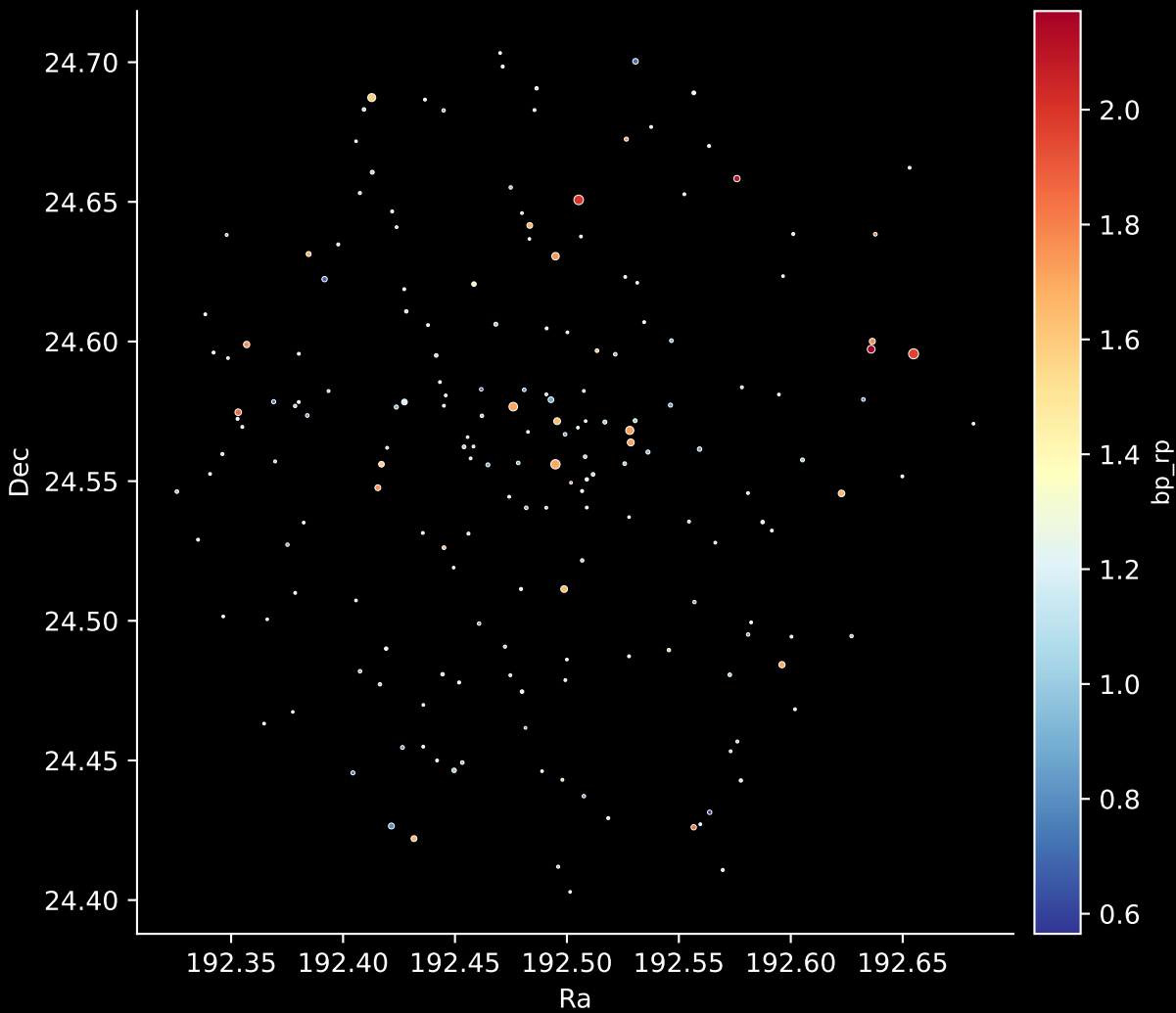
Gaia Cluster: [Koposov_63] Stars: 186
