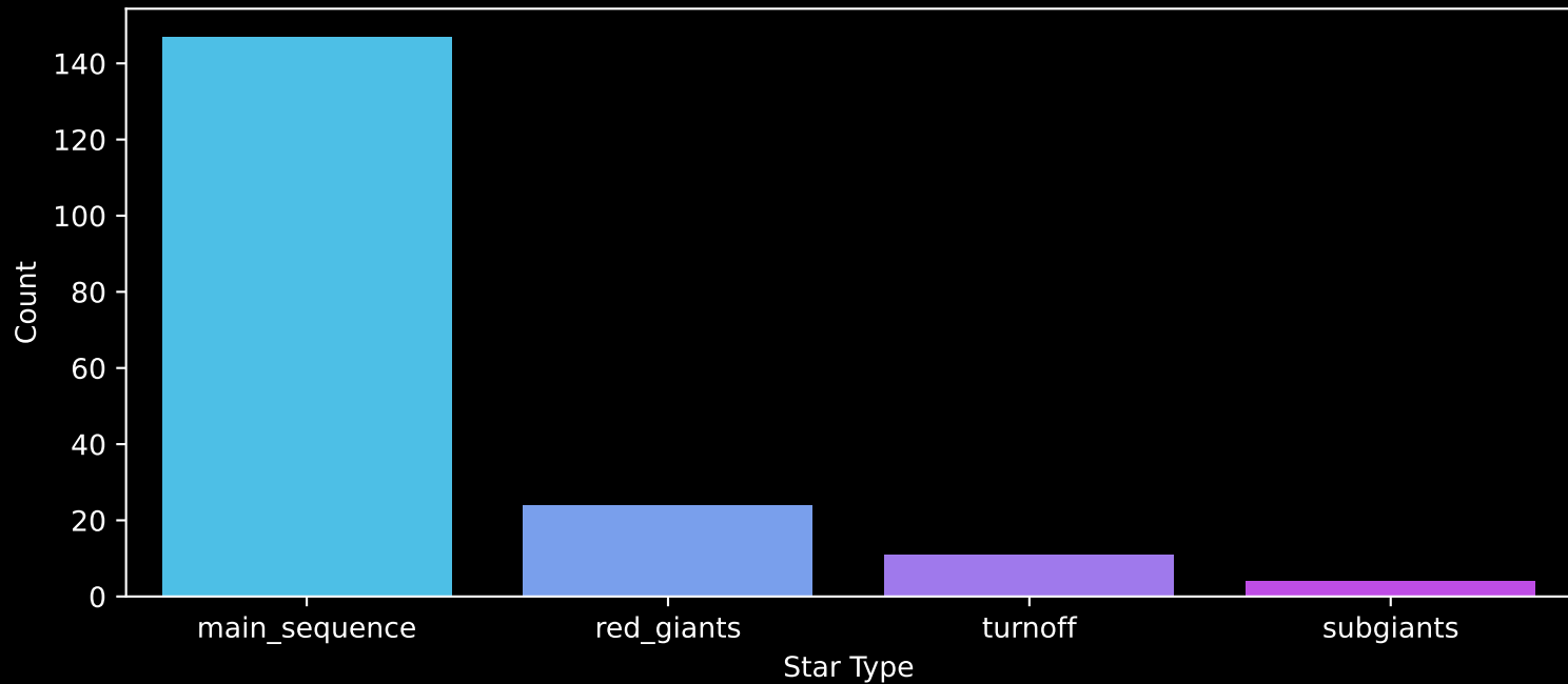
Gaia Cluster: [Koposov_63] Count plot of Star Type
