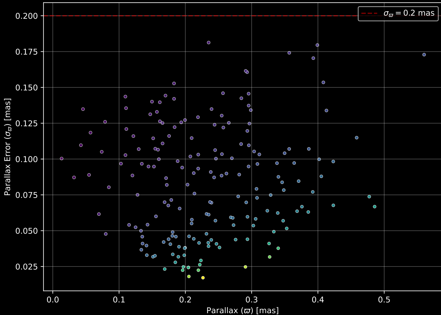
Gaia Cluster: [Koposov_63] Parallax Quality (n= 186)
