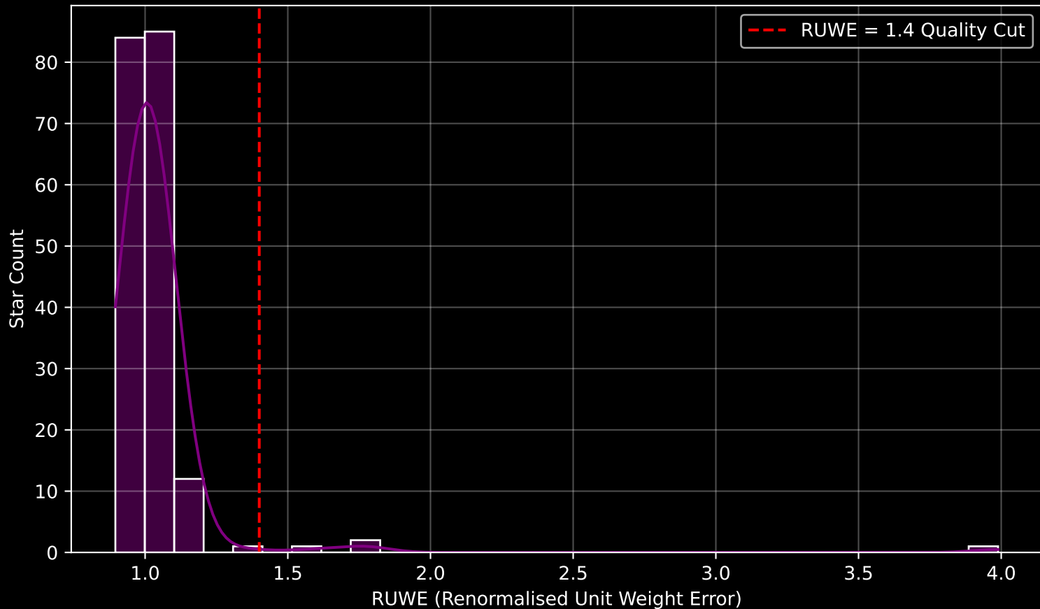
Gaia Cluster: [Koposov_63] RUWE Distribution (n= 186)
