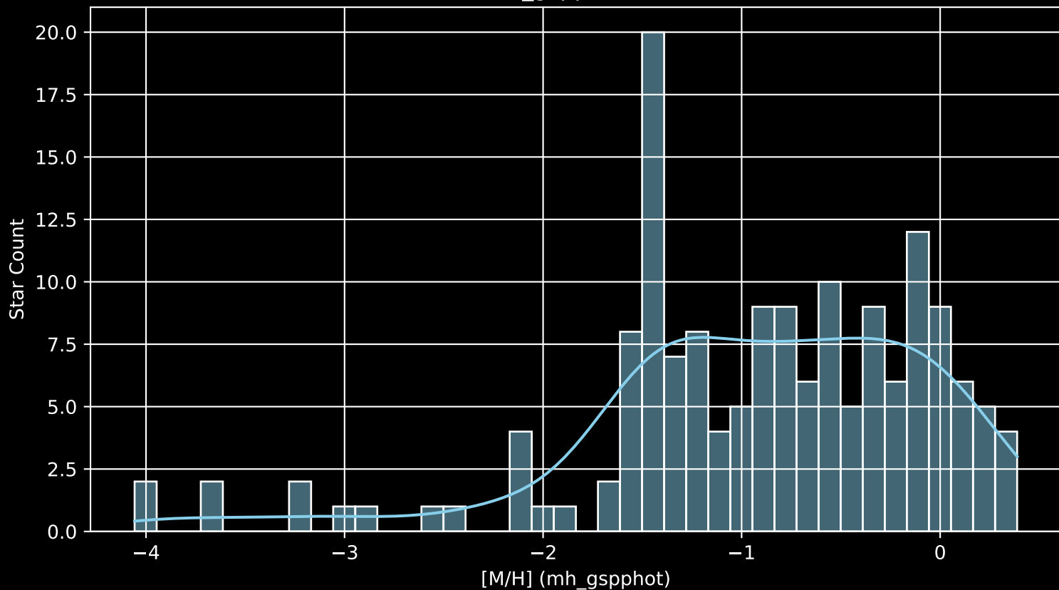
Gaia Cluster: [Kronberger_52 [M/H] (mh_gspphot) (n= 160)
