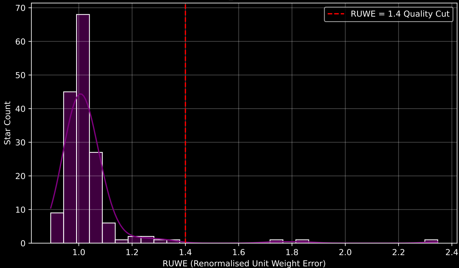
Gaia Cluster: [Kronberger_52] RUWE Distribution (n= 165)
