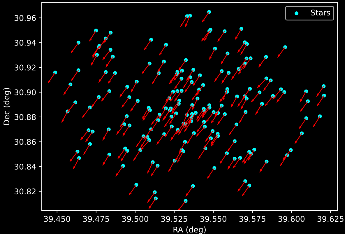
Gaia Cluster: [Kronberger_52] Proper Motion Vectors for Gaia Star Field (n= 165)
