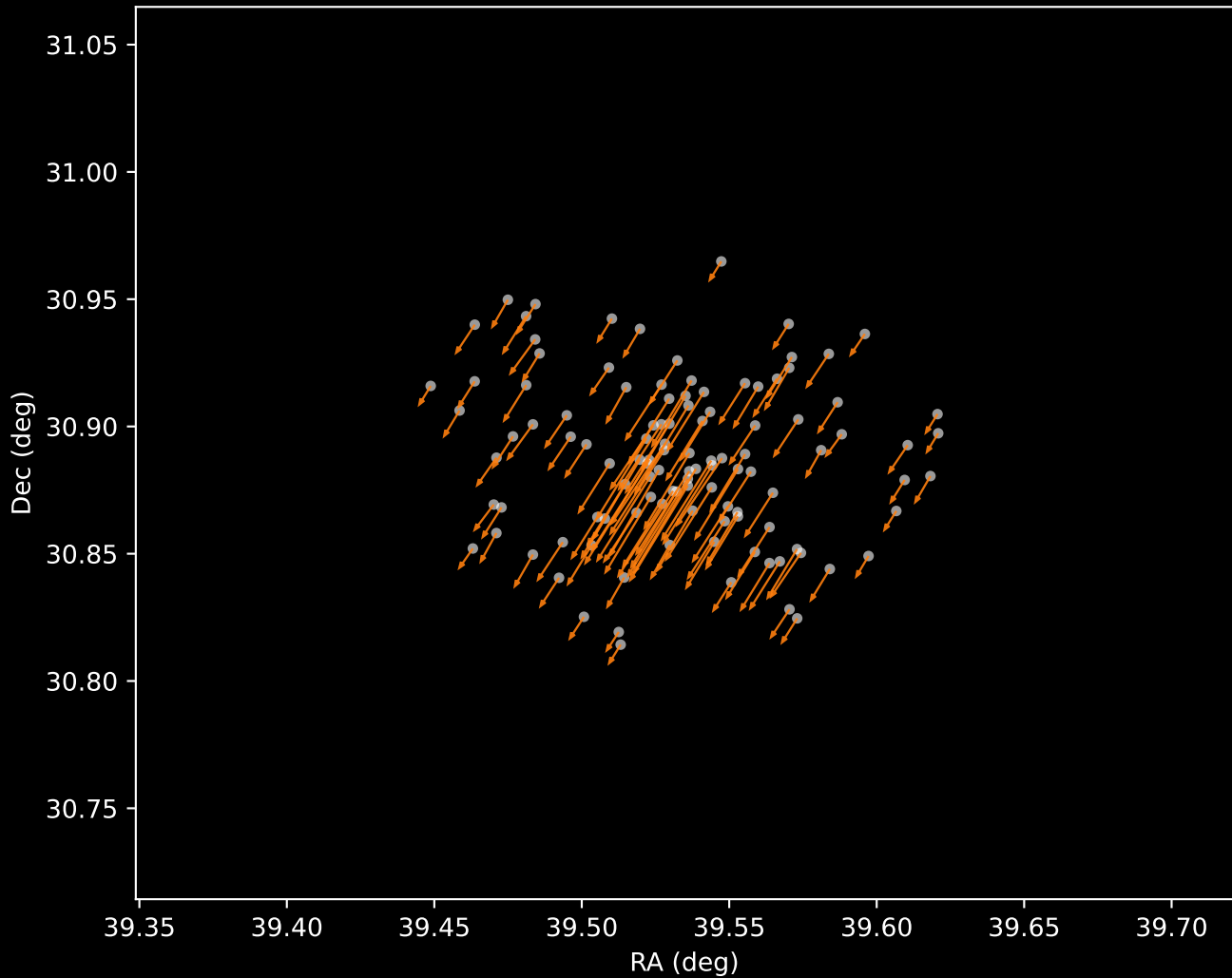
Gaia DR3 Cluster 2 Proper Motion Vectors (n=112)
