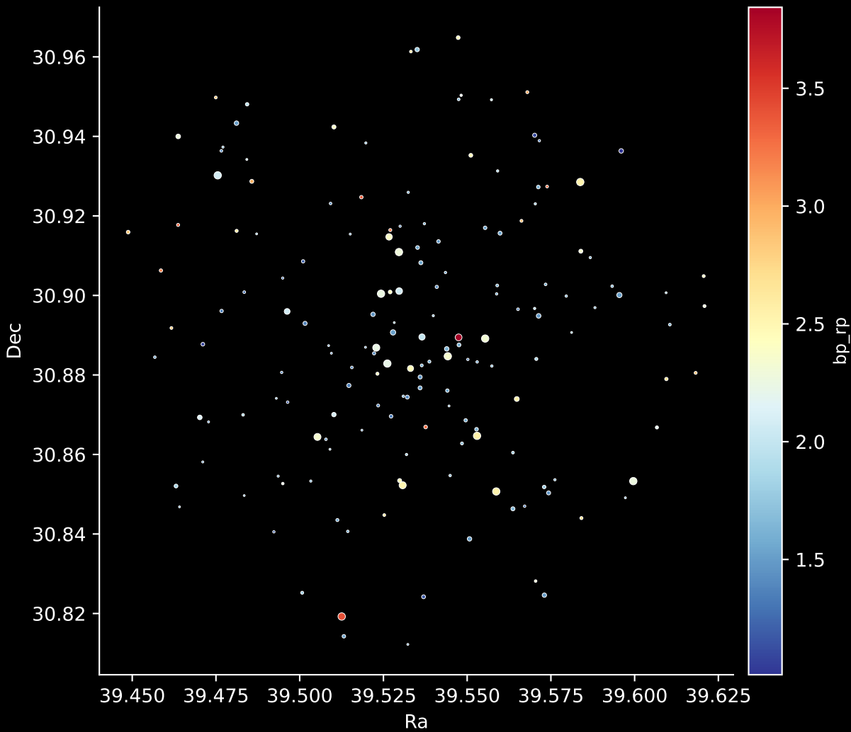
Gaia Cluster: [Kronberger_52] Stars: 165
