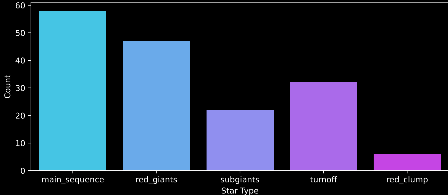
Gaia Cluster: [Kronberger_52] Count plot of Star Type
