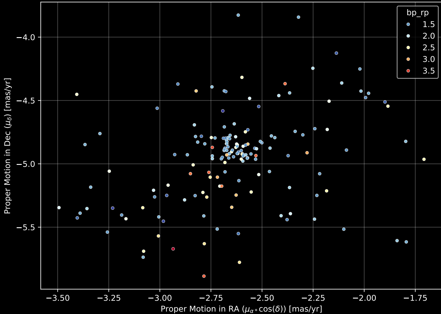
Gaia Cluster: [Kronberger_52] Proper Motion Diagram (n= 165)
