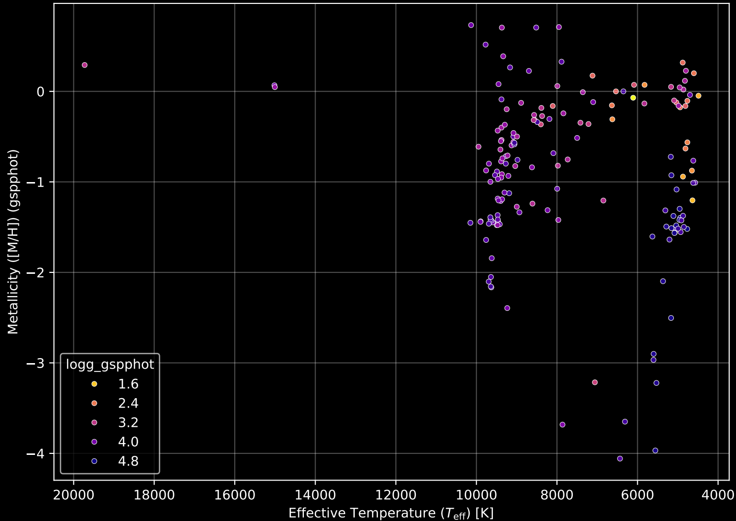
Gaia Cluster: [Kronberger_52] Stellar Population Parameters (n= 165)
