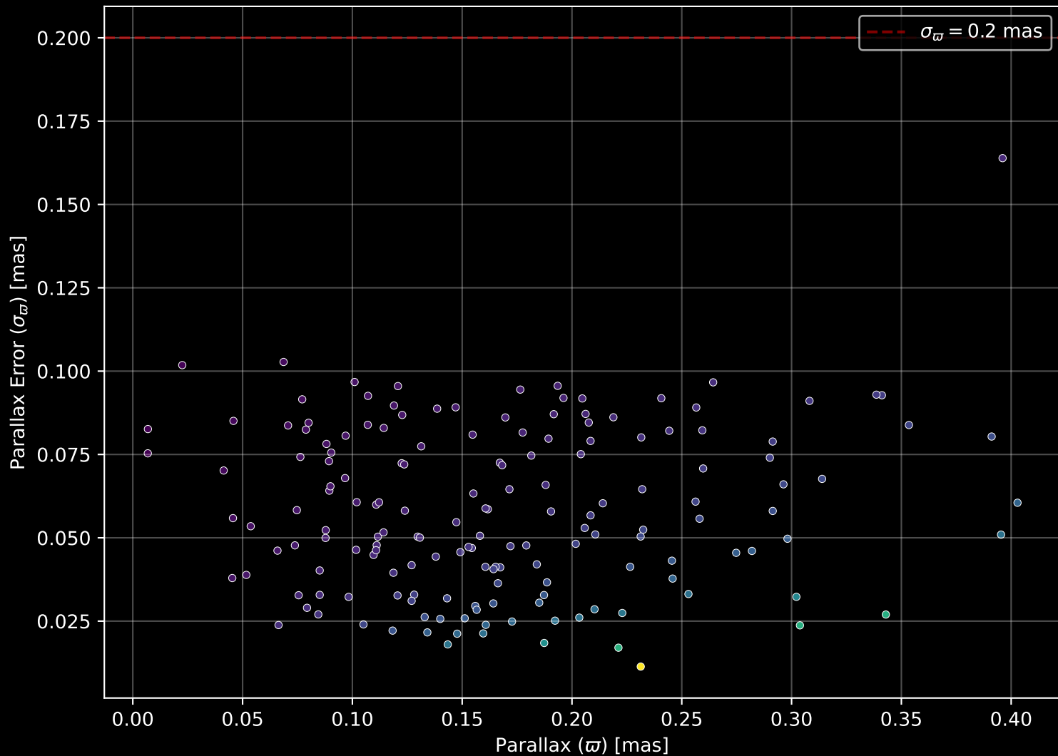
Gaia Cluster: [Kronberger_52] Parallax Quality (n= 165)
