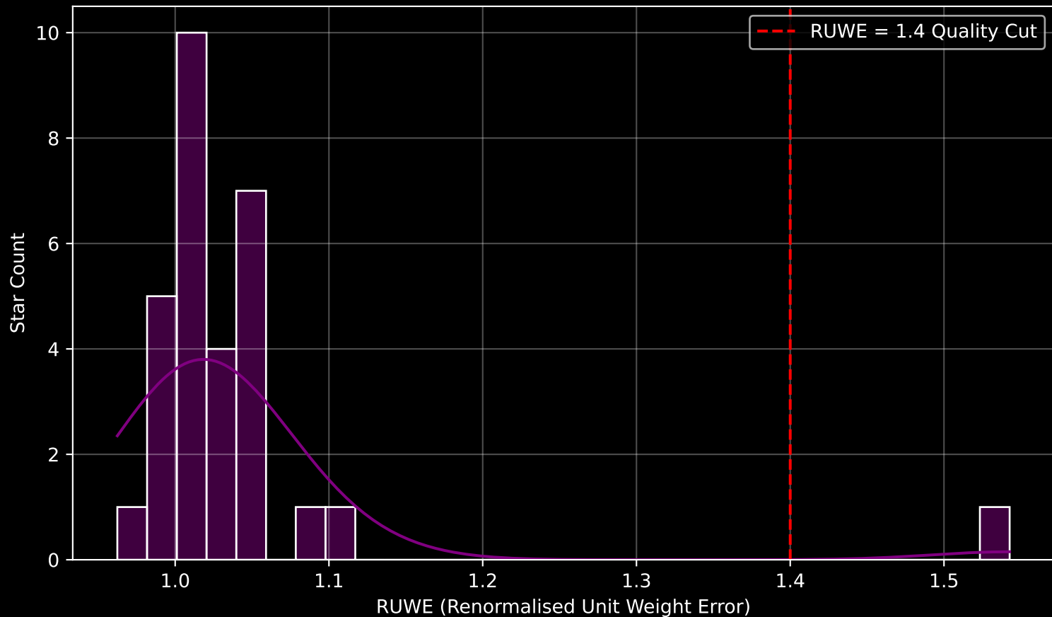
Gaia Cluster: [Kronberger_54] RUWE Distribution (n= 30)
