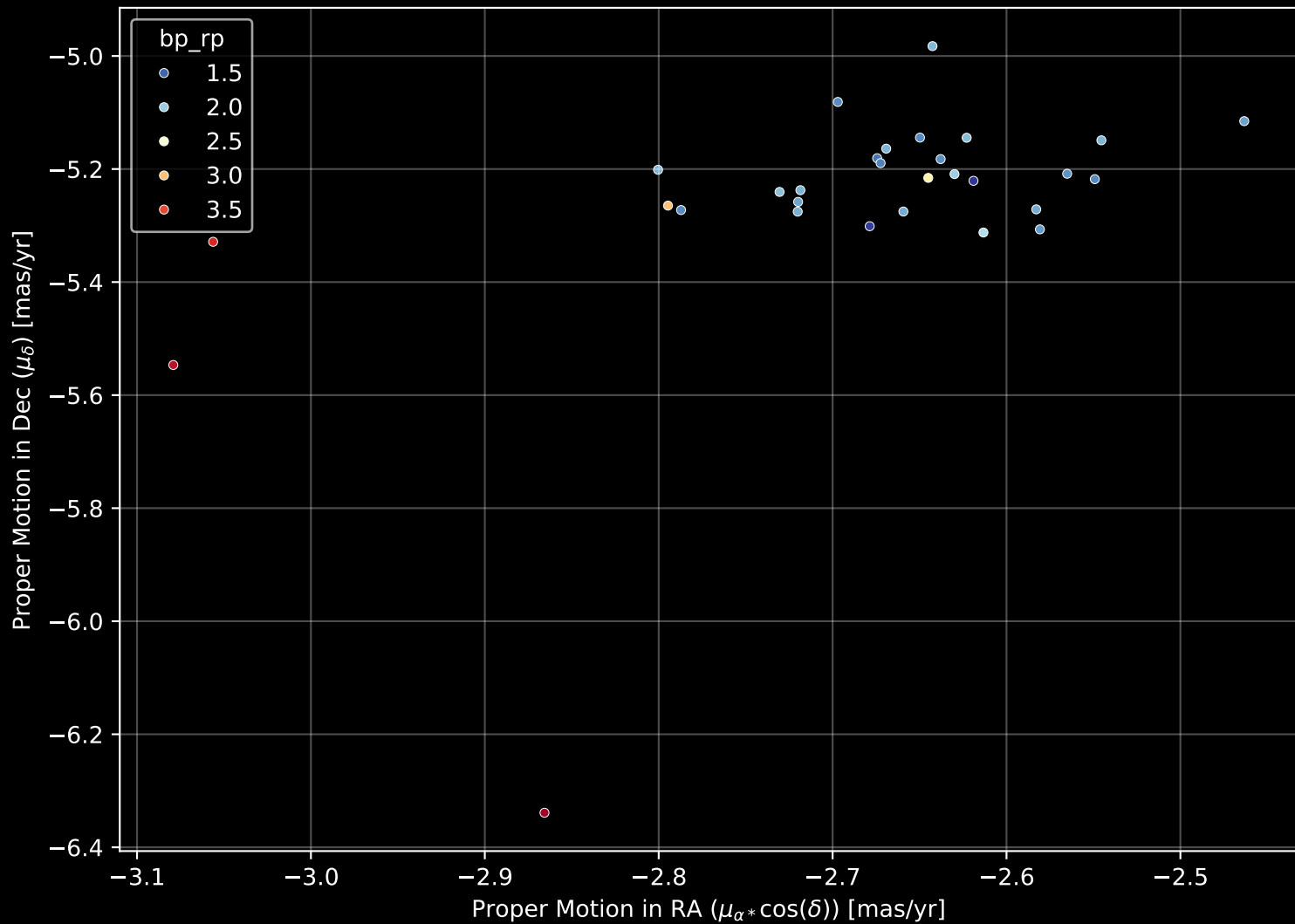
Gaia Cluster: [Kronberger_54] Proper Motion Diagram (n= 30)
