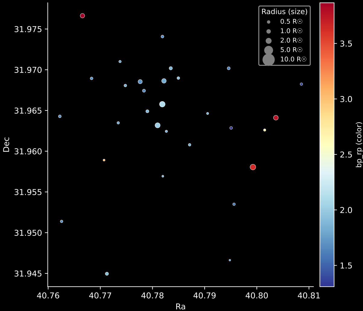
Gaia Cluster: [Kronberger_54] Stars: 30
