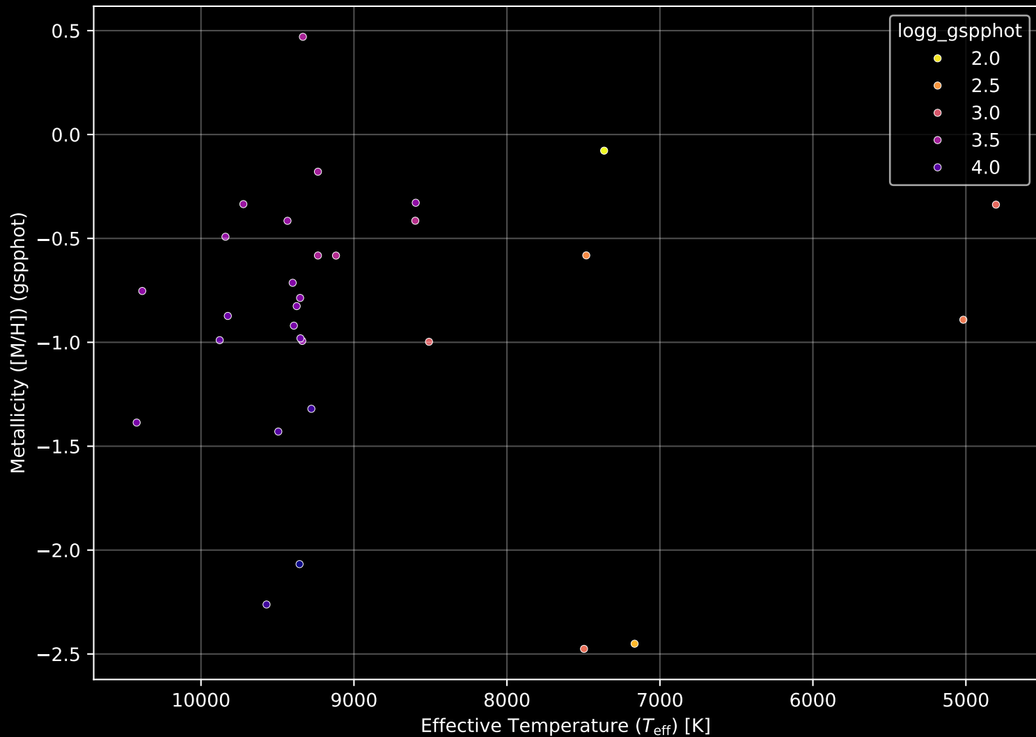
Gaia Cluster: [Kronberger_54] Stellar Population Parameters (n= 30)
