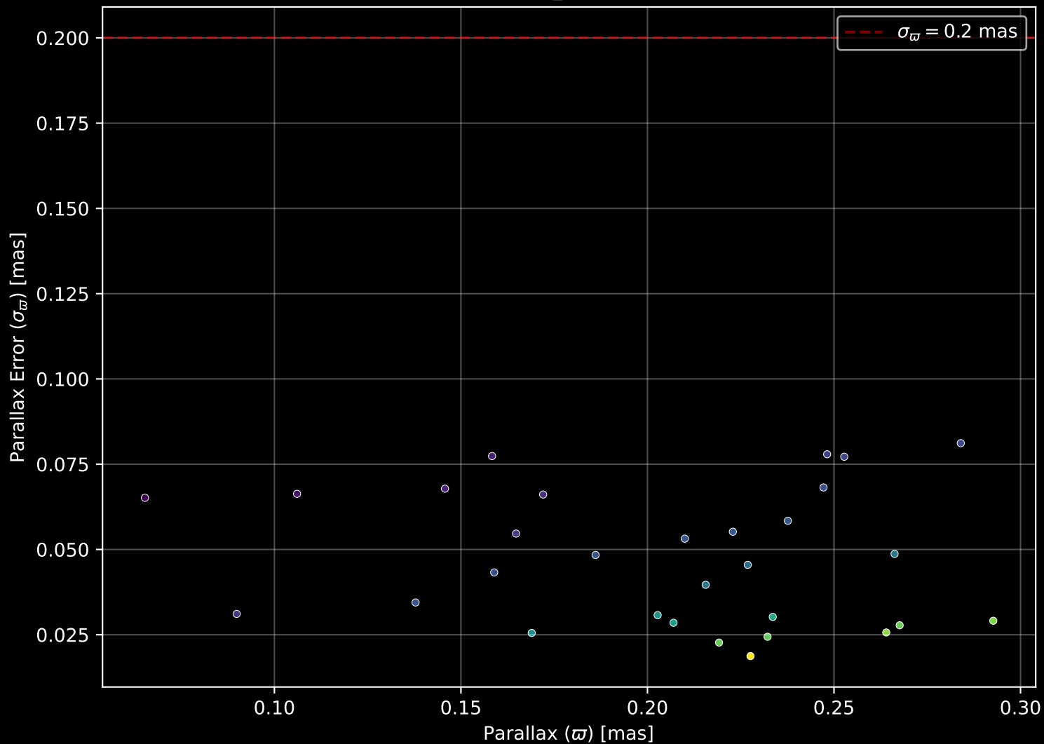
Gaia Cluster: [Kronberger_54] Parallax Quality (n= 30)
