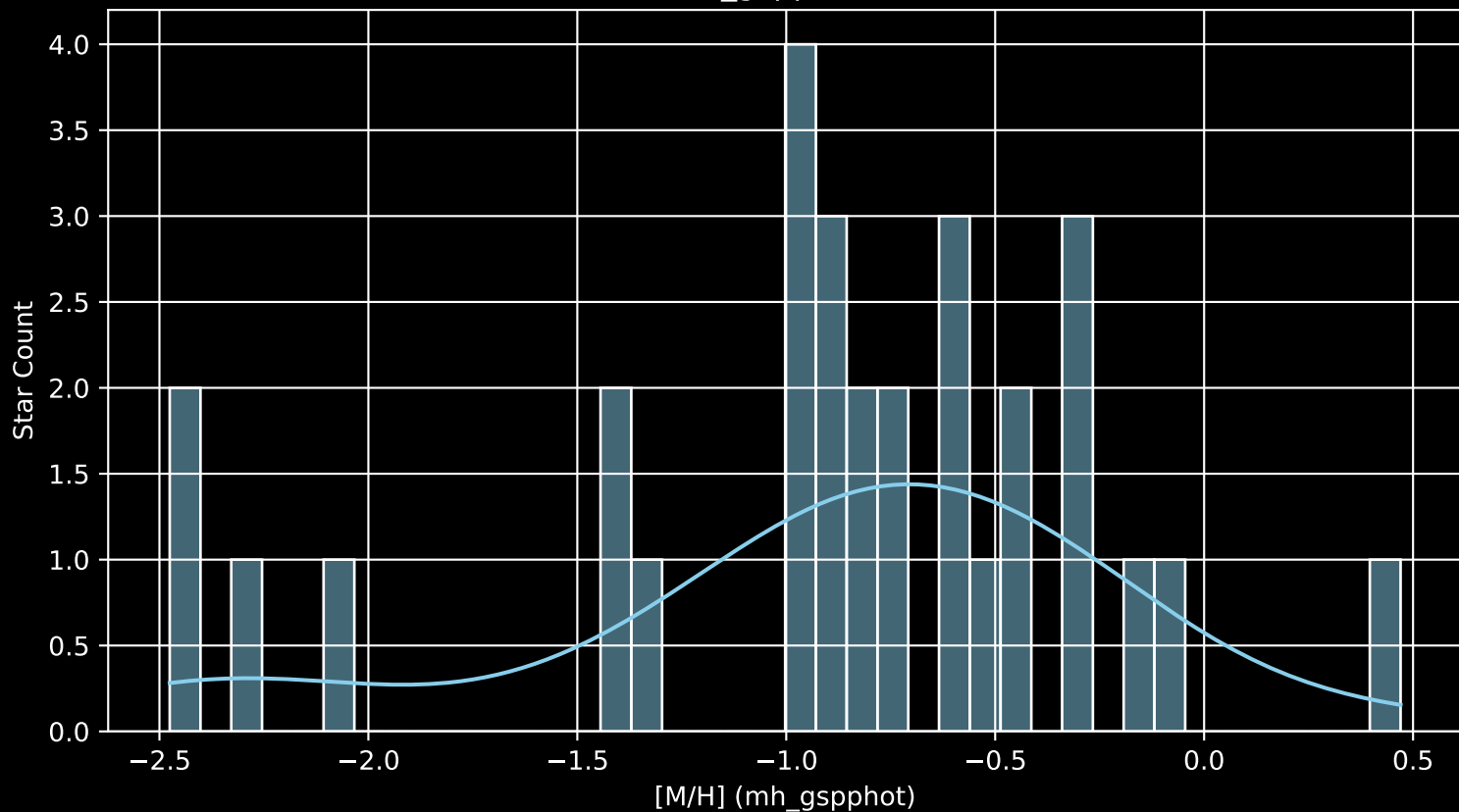
Gaia Cluster: [Kronberger_54 [M/H] (mh_gspphot) (n= 30)
