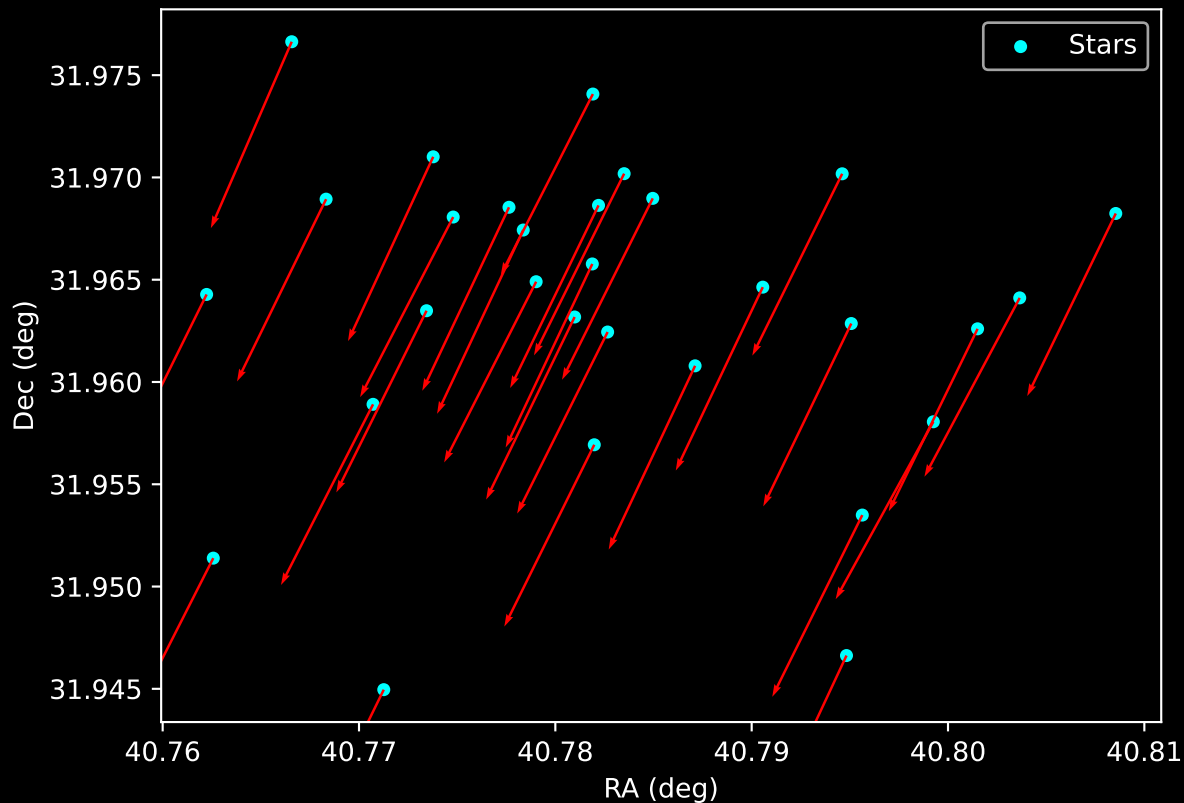
Gaia Cluster: [Kronberger_54] Proper Motion Vectors for Gaia Star Field (n= 30)
