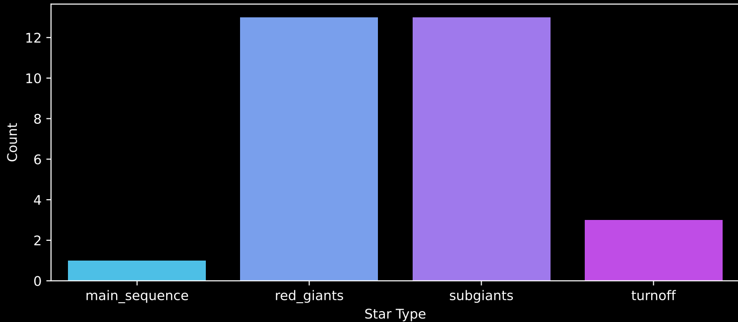
Gaia Cluster: [Kronberger_54] Count plot of Star Type
