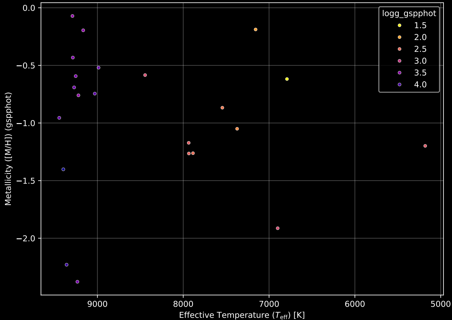
Gaia Cluster: [Kronberger_57] Stellar Population Parameters (n= 22)
