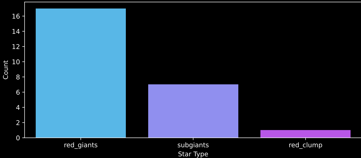
Gaia Cluster: [Kronberger_80] Count plot of Star Type
