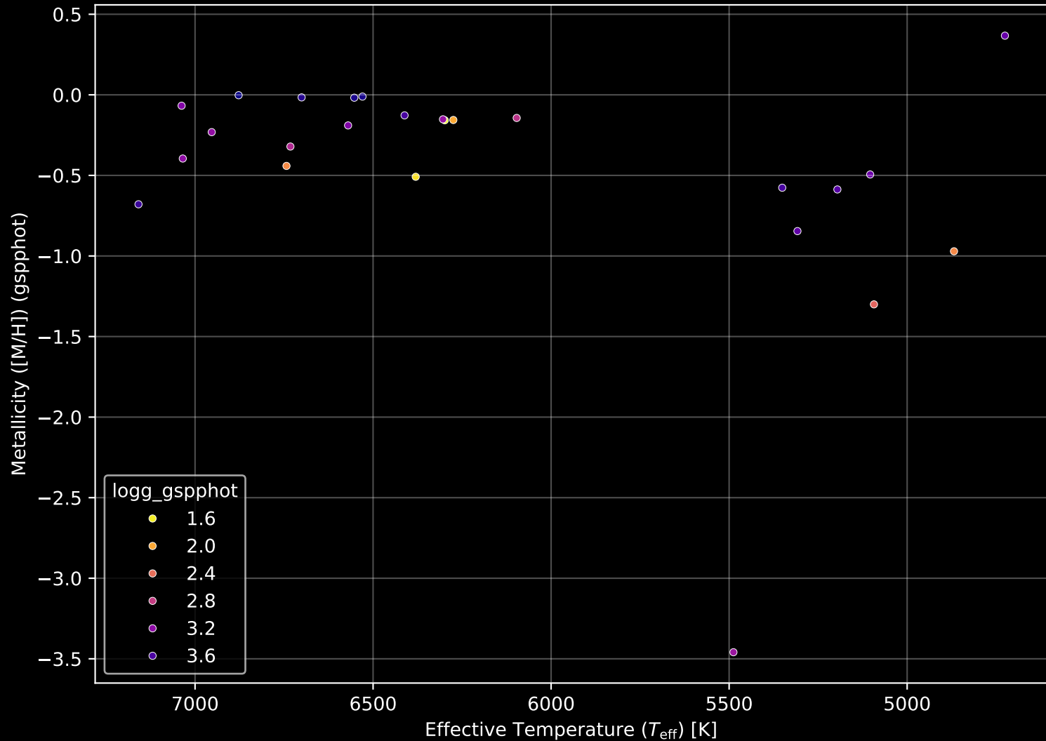
Gaia Cluster: [Kronberger_80] Stellar Population Parameters (n= 25)
