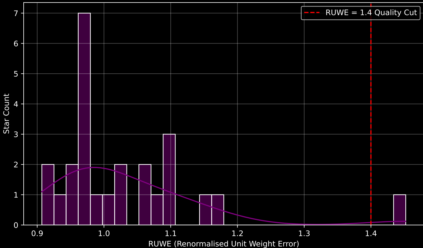
Gaia Cluster: [Kronberger_80] RUWE Distribution (n= 25)
