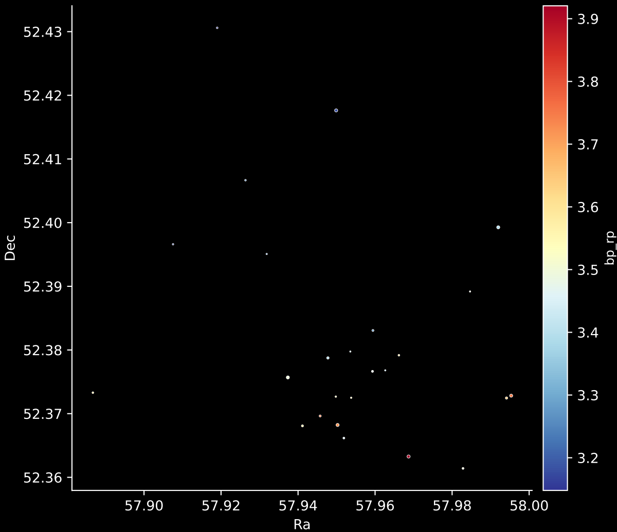
Gaia Cluster: [Kronberger_80] Stars: 25
