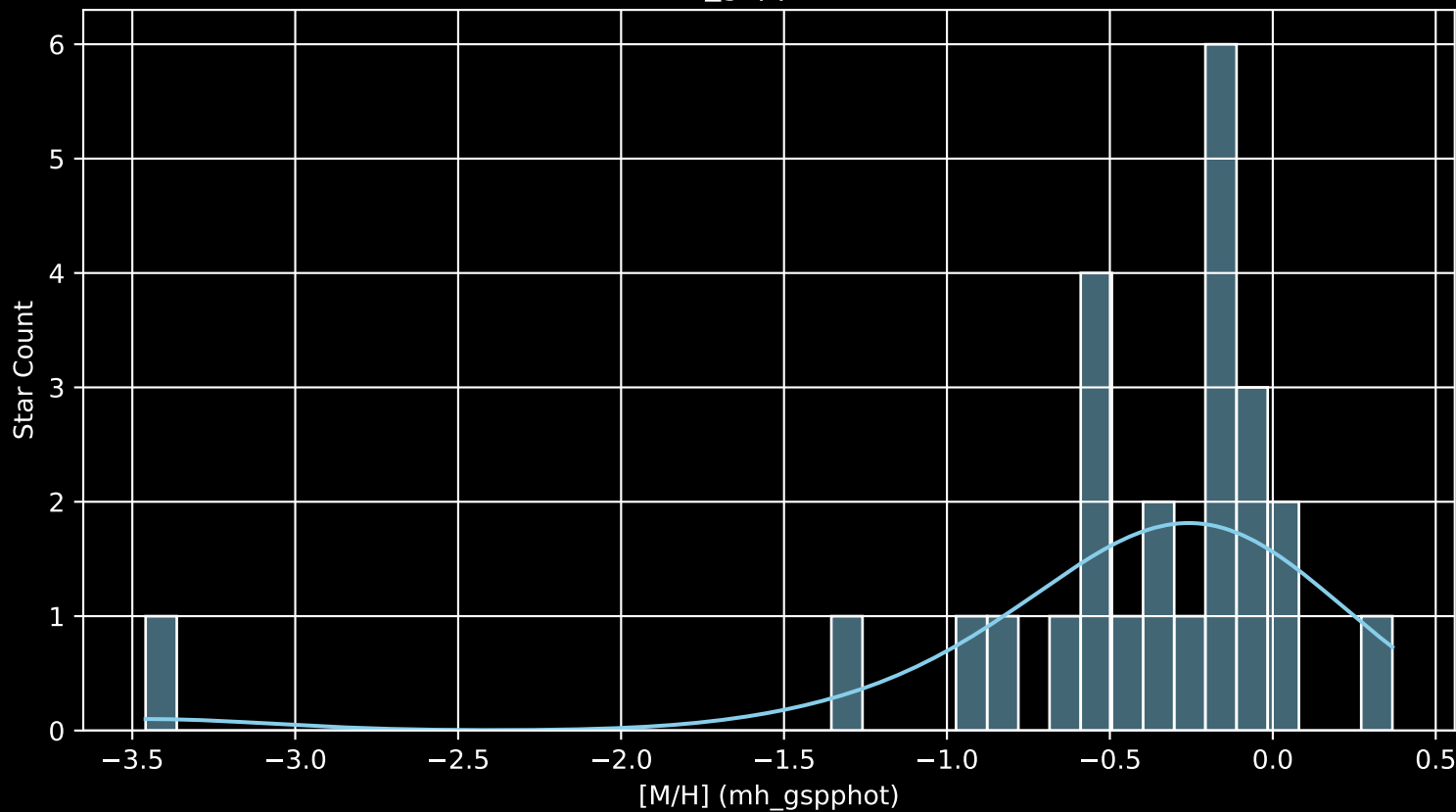
Gaia Cluster: [Kronberger_80 [M/H] (mh_gspphot) (n= 25)
