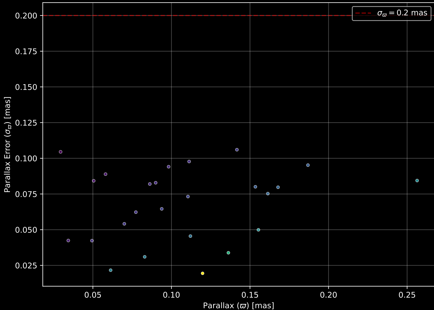
Gaia Cluster: [Kronberger_80] Parallax Quality (n= 25)
