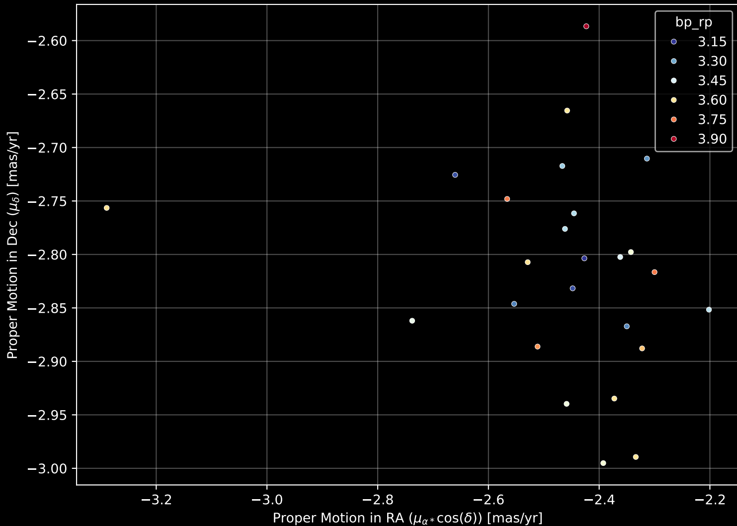
Gaia Cluster: [Kronberger_80] Proper Motion Diagram (n= 25)
