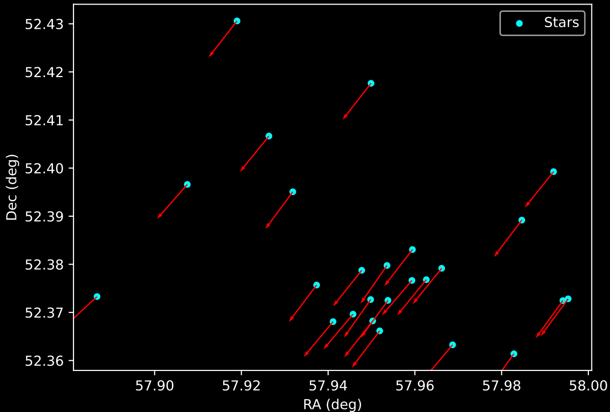
Gaia Cluster: [Kronberger_80] Proper Motion Vectors for Gaia Star Field (n= 25)
